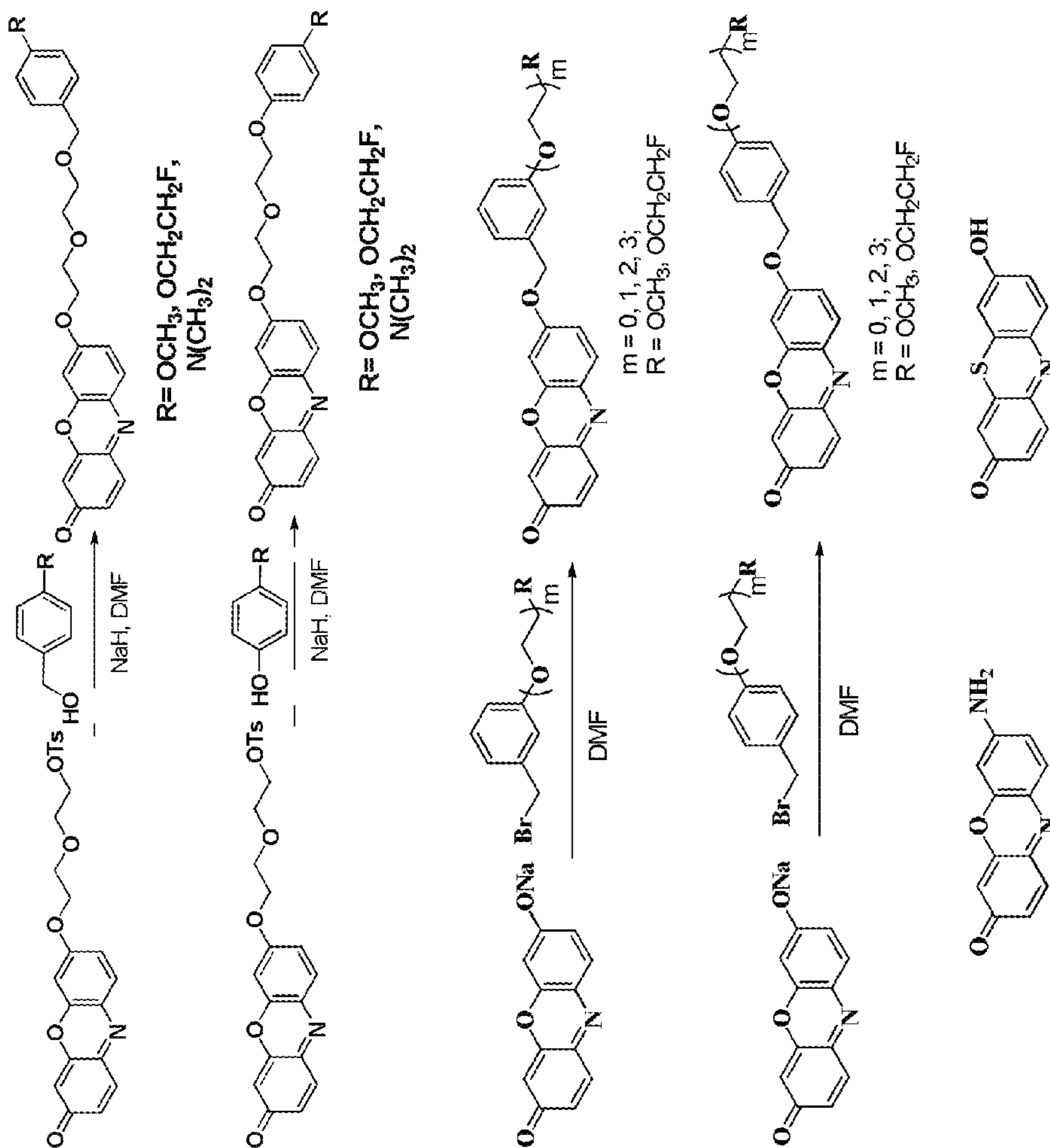
7-Amino-3H-Phenoxazin-3-one
