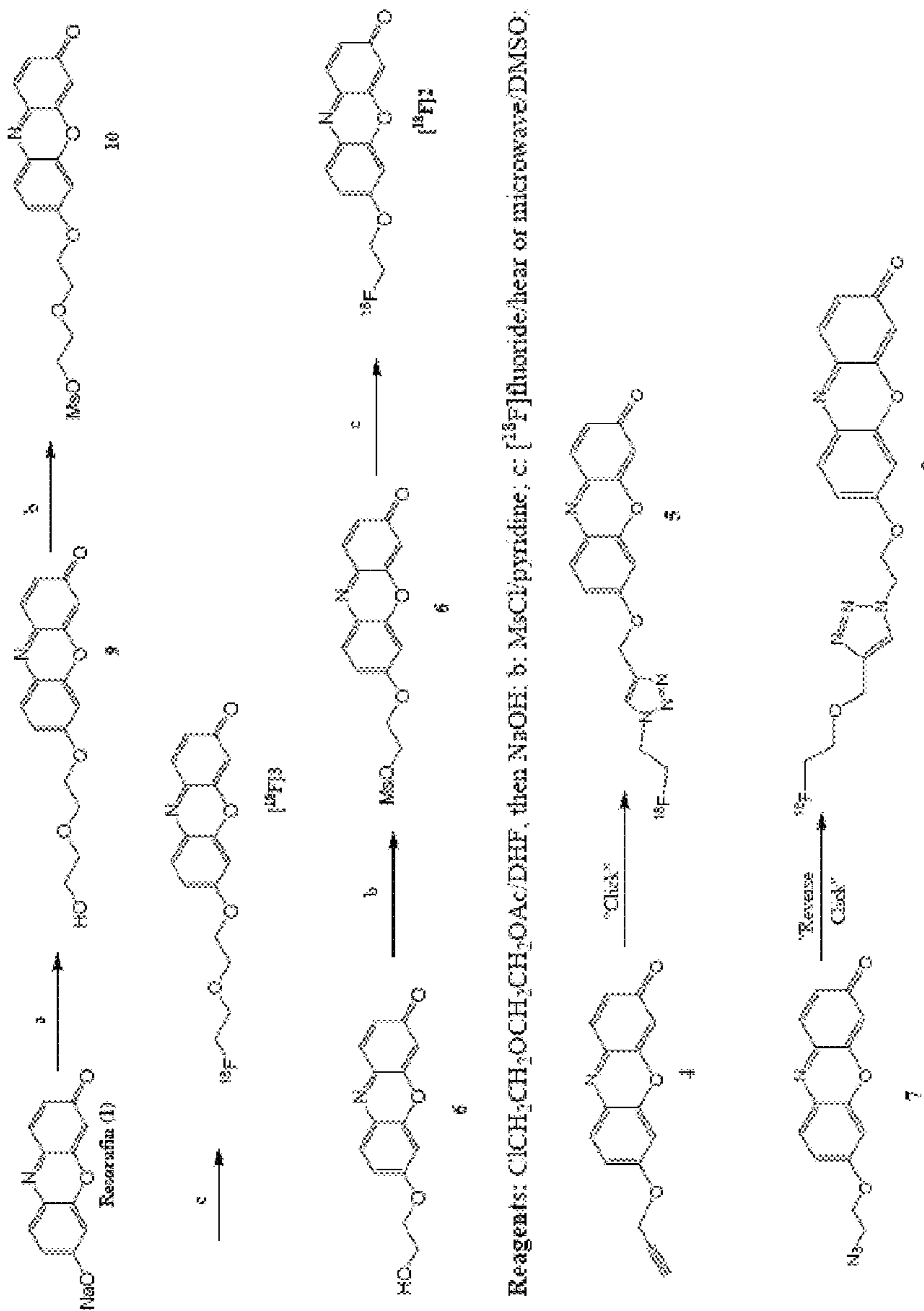
Synthesis of 18 F-resorufin analogs.
