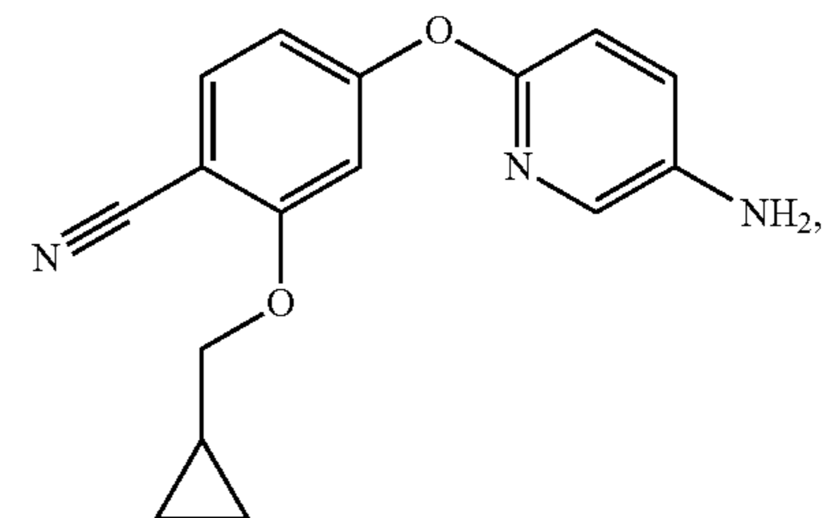
4-[[5-amino-2-pyridinyl]oxy]-2-[(cyclopropylmethyl)oxy]benzonitrile
