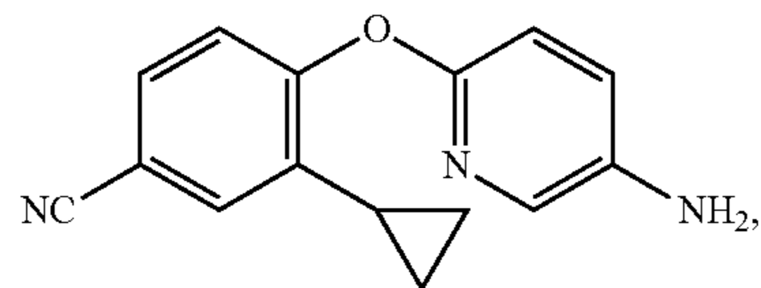
4-[[5-amino-2-pyridinyl]oxy]-3-cyclopropylbenzonitrile
