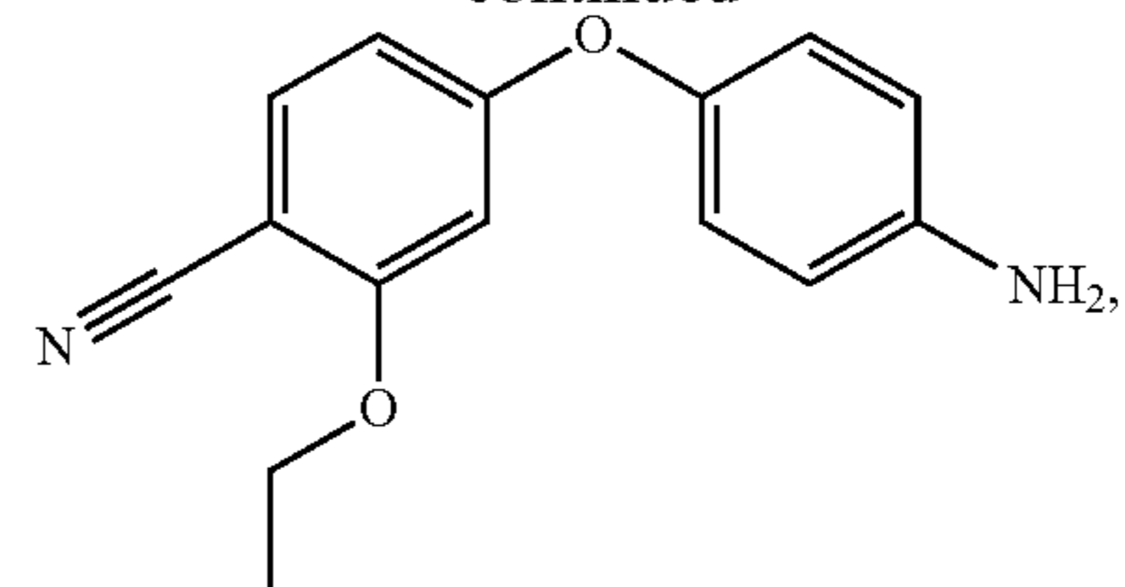
4-[[4-aminophenyl]oxy]-2-(ethoxy)benzonitrile
