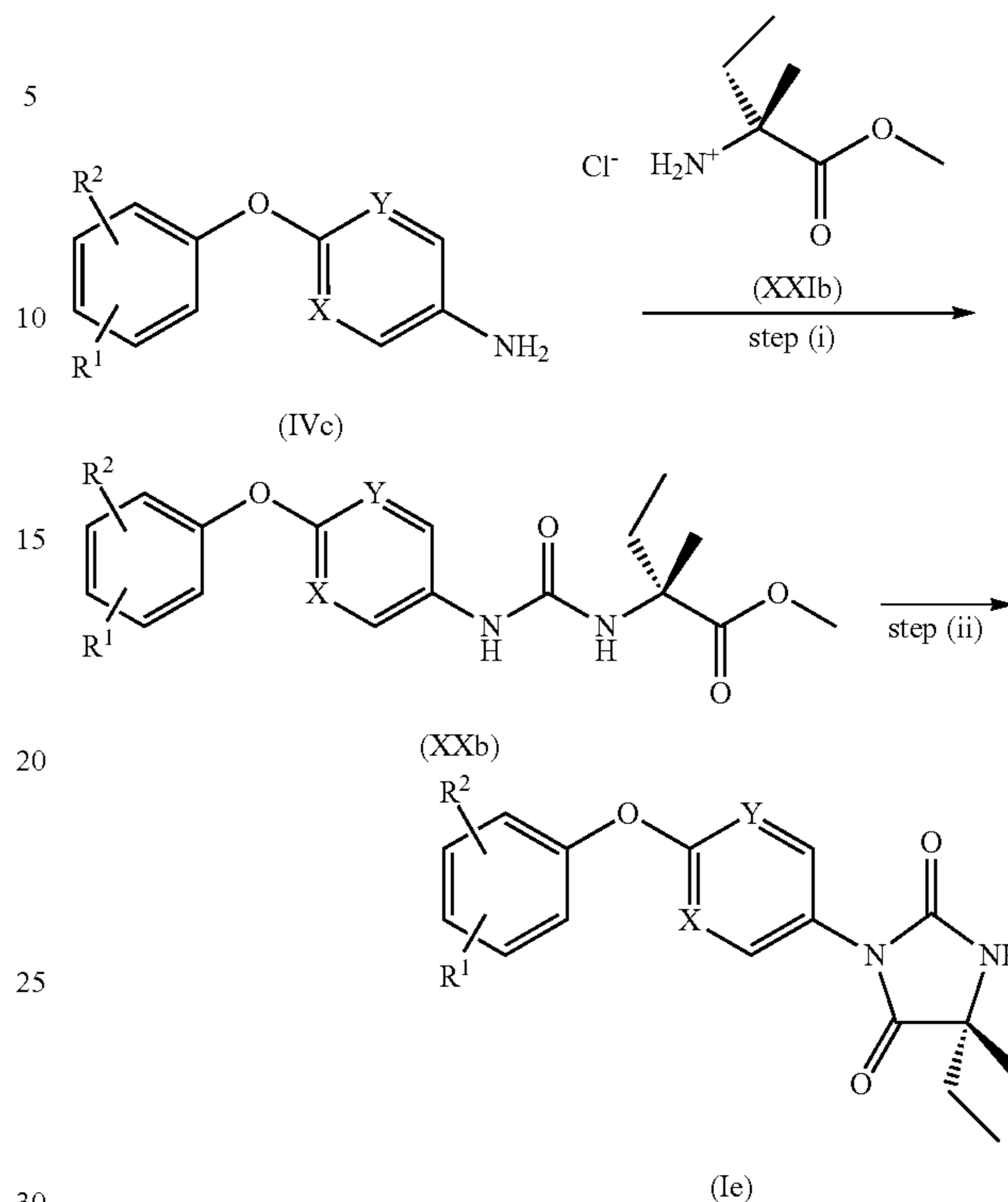
Scheme 14
