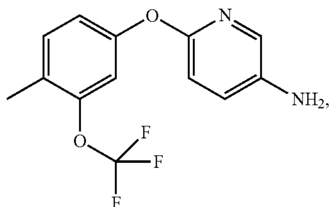
6-[[4-methyl-3-[(trifluoromethyl)oxy]phenyl]oxy]-3-pyridinamine
