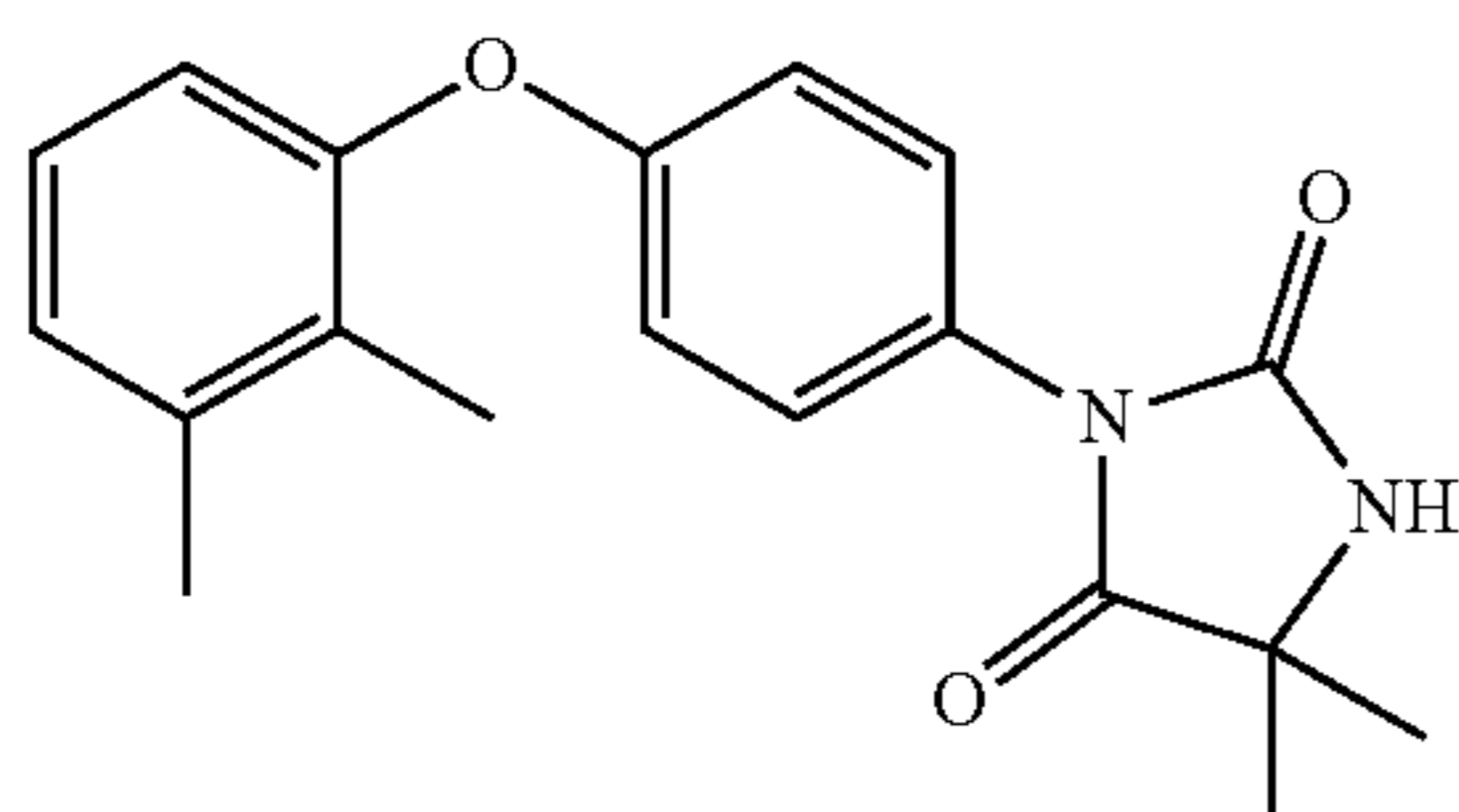
3-{4-[(2,3-dimethylphenyl)oxy]phenyl}-5,5-dimethyl-2,4-imidazolidinedione
