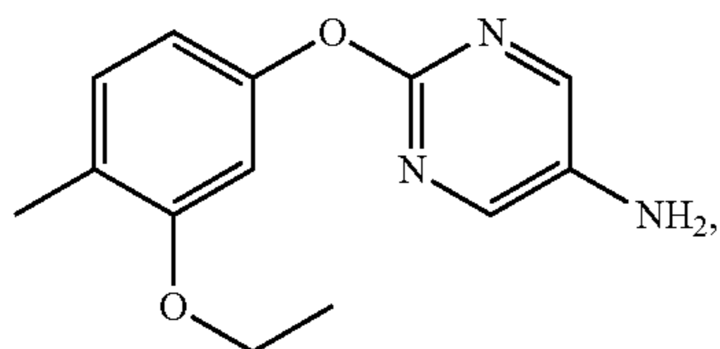
2-[[3-(ethoxy)-4-methylphenyl]oxy]-5-pyrimidinamine
