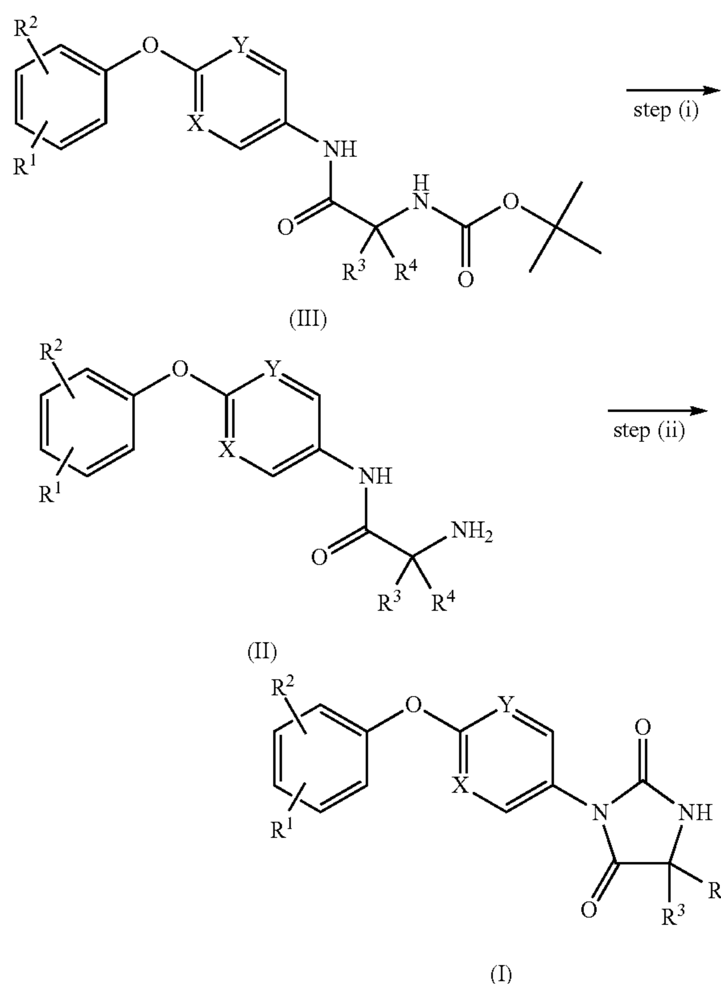
Scheme 1
