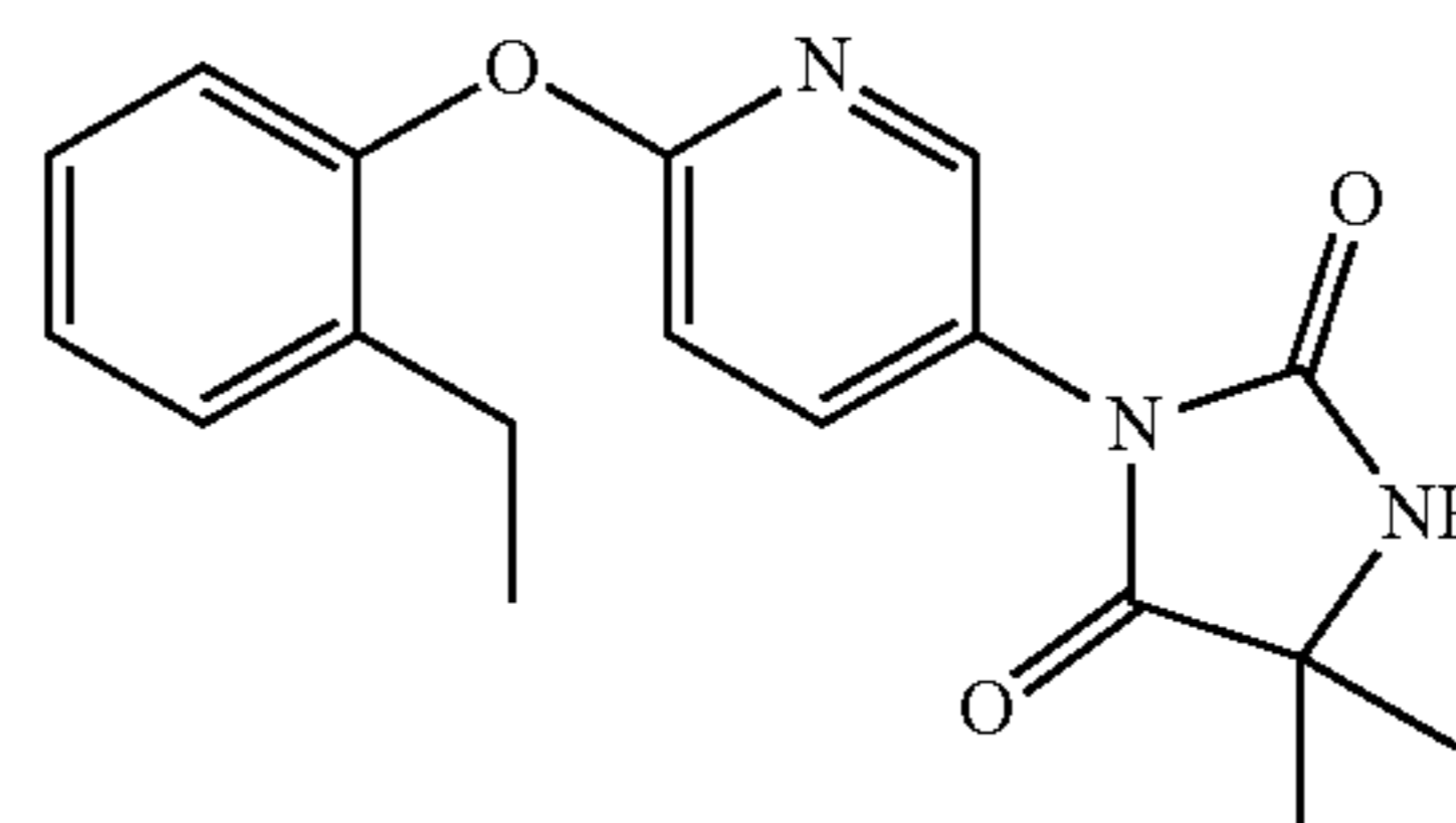
3-{6-[(2-ethylphenyl)oxy]-3-pyridinyl}-5,5-dimethyl-2,4-imidazolidinedione
