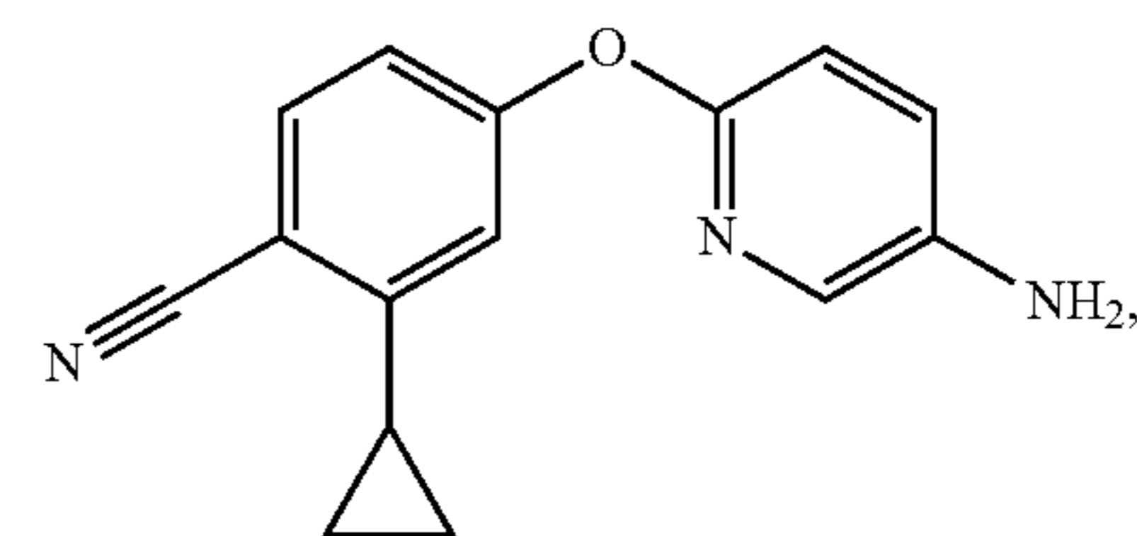
4-[[5-amino-2-pyridinyl]oxy]-2-cyclopropylbenzonitrile
