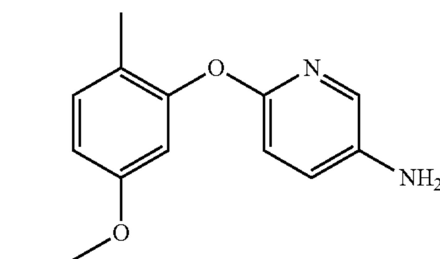
6-([2-methyl-5-(methoxy)phenyl]oxy)-3-pyridinamine
