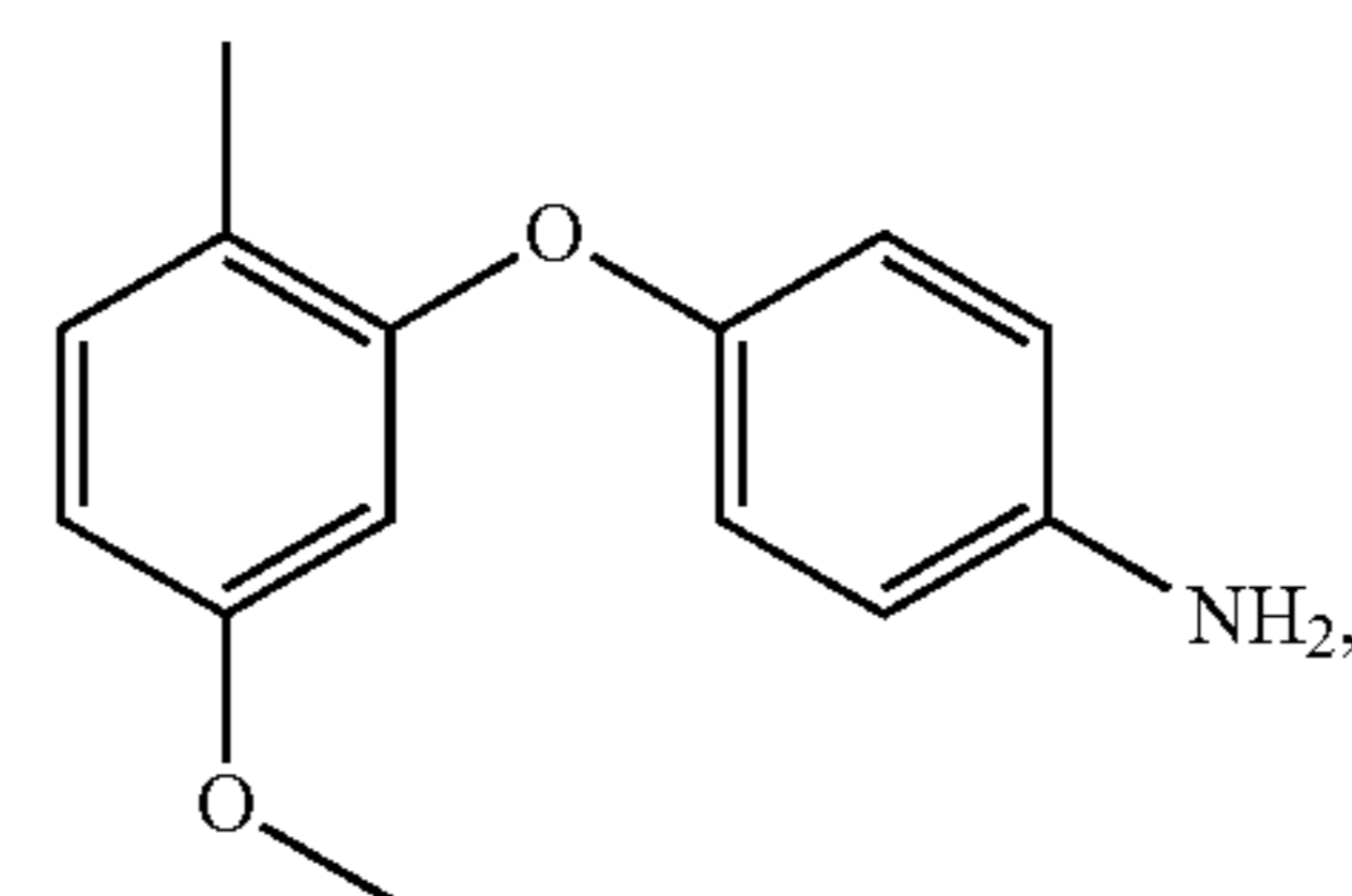
4-([2-methyl-5-(methoxy)phenyl]oxy)aniline
