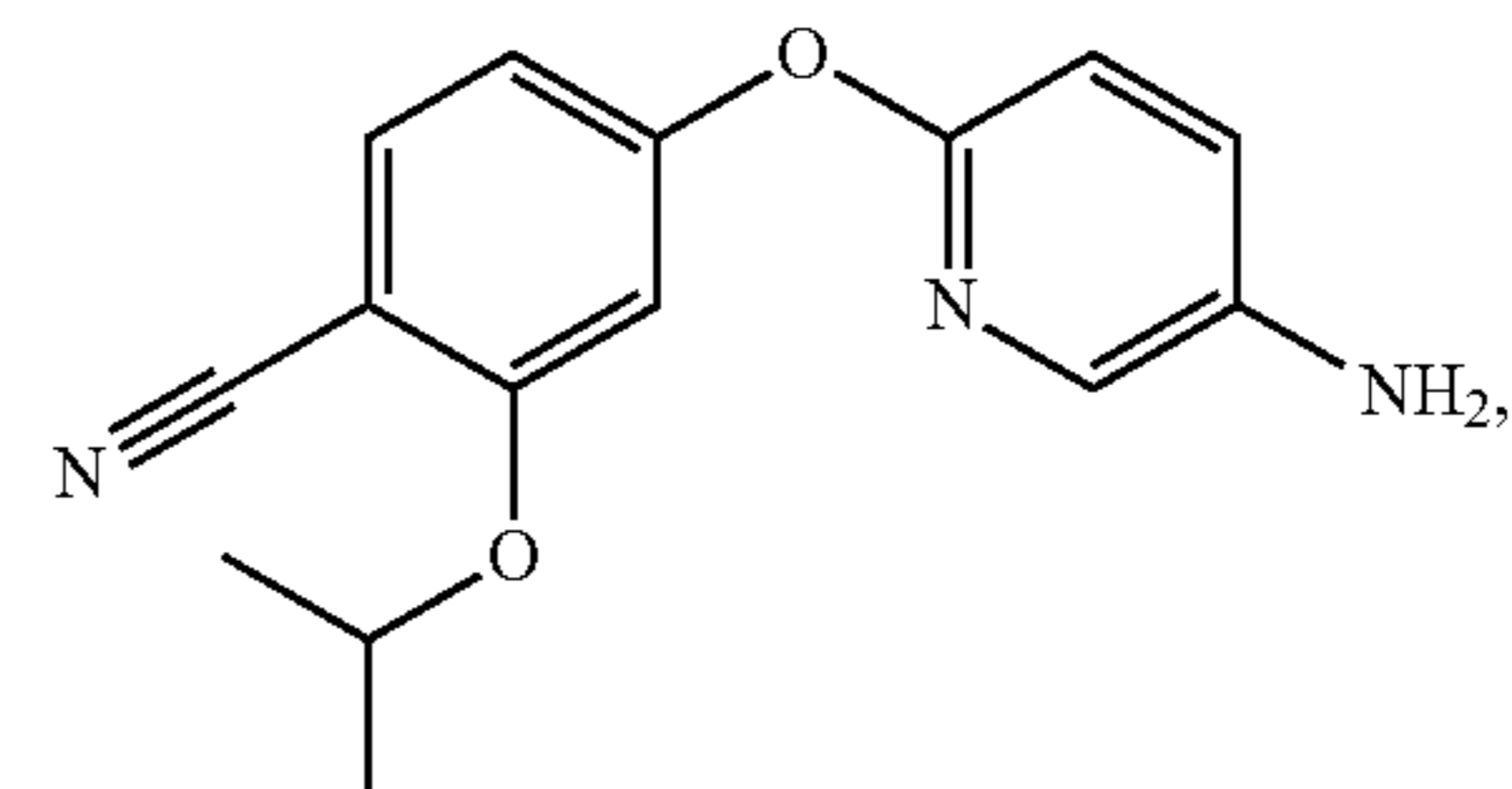
4-[[5-amino-2-pyridinyl]oxy]-2-[(1-methylethyl)oxy]benzonitrile
