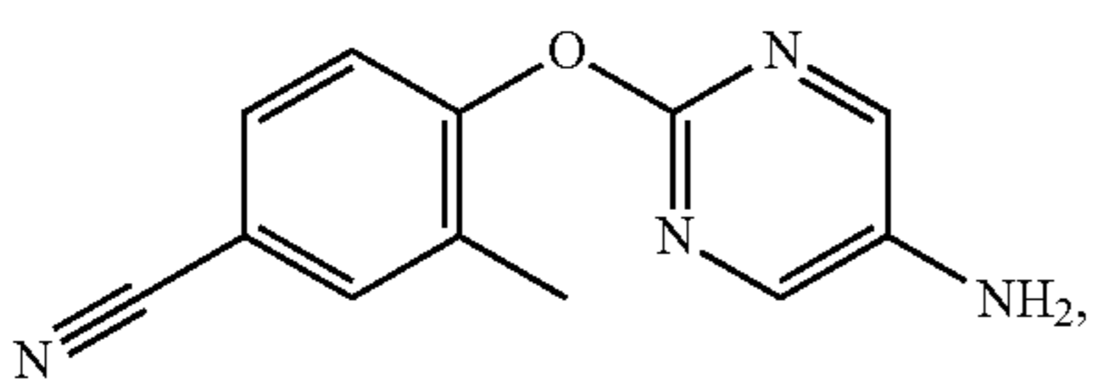
4-[(5-amino-2-pyrimidinyl)oxy]-3-methylbenzonitrile
