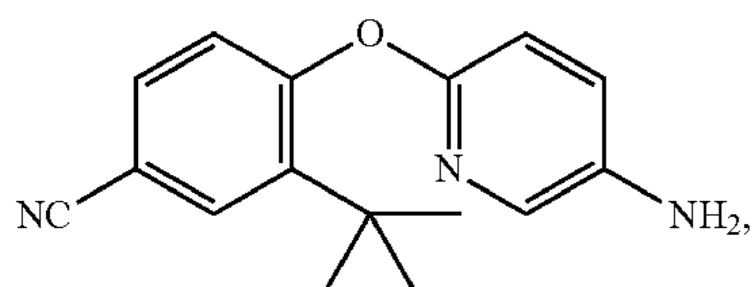
4-[[5-amino-2-pyridinyl]oxy]-3-(1,1-dimethylethyl)benzonitrile
