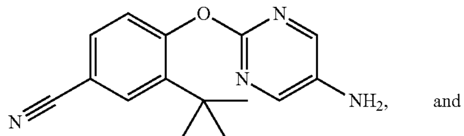
4-[(5-amino-2-pyrimidinyl)oxy]-3-(1,1-dimethylethyl)benzonitrile
