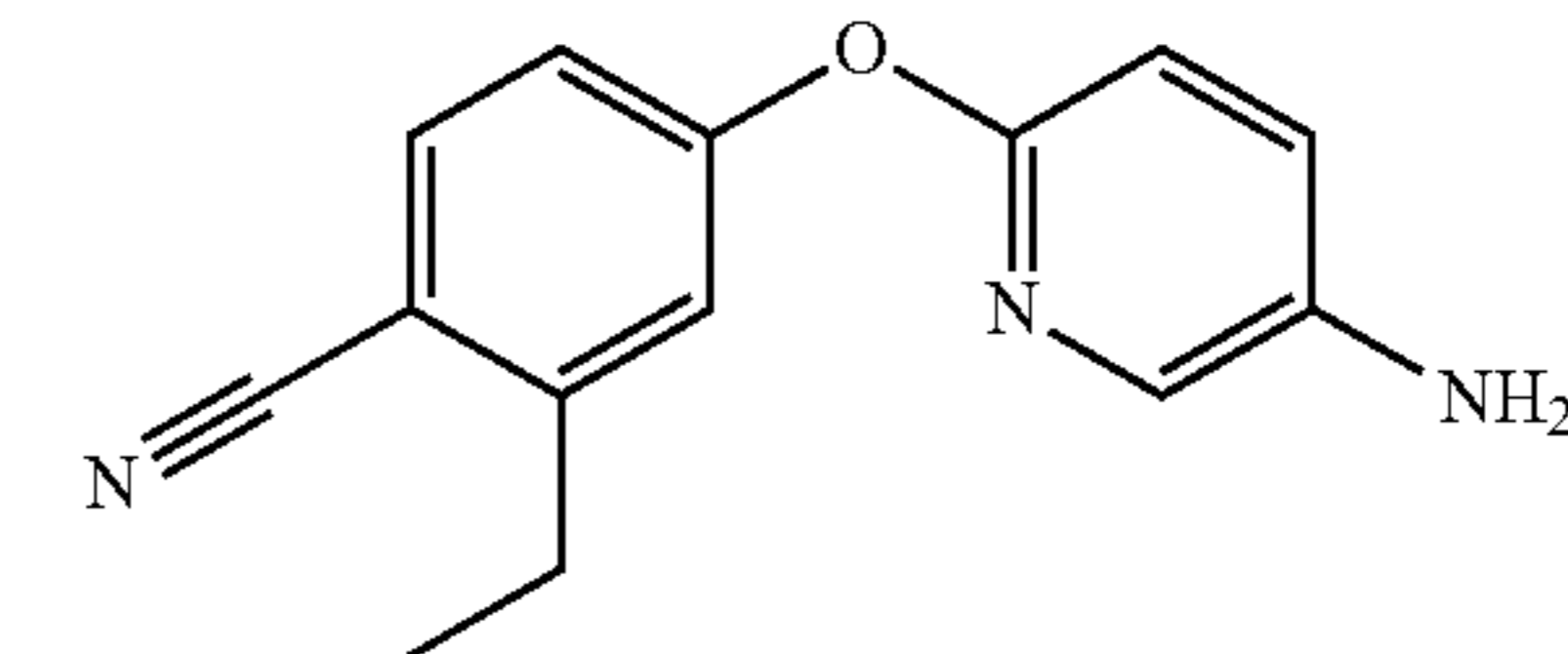
4-[[5-amino-2-pyridinyl]oxy]-2-ethylbenzonitrile
