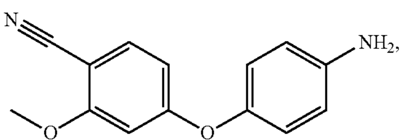
4-[[4-aminophenyl]oxy]-2-(methoxy)benzonitrile
