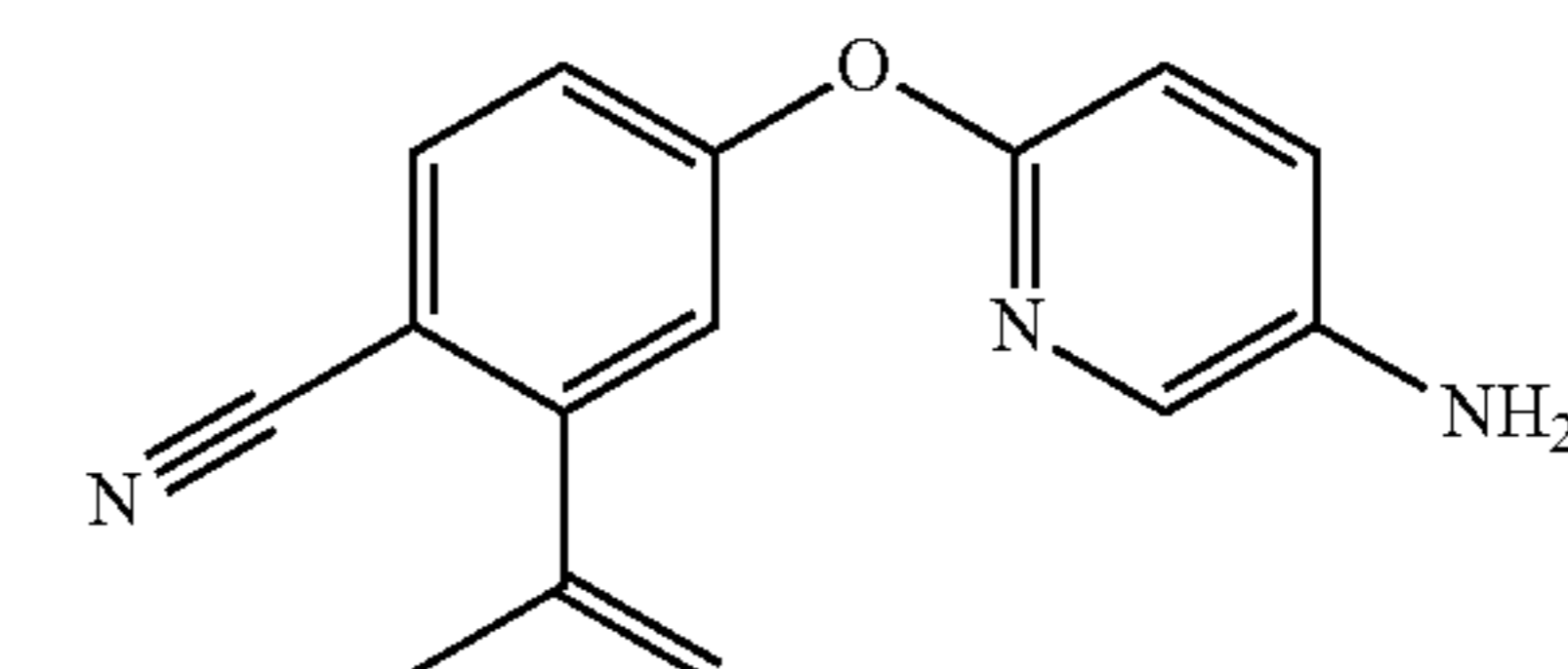
4-[[5-amino-2-pyridinyl]oxy]-2-(1-methylethenyl)benzonitrile
