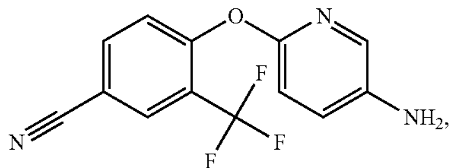
4-[[5-amino-2-pyridinyl]oxy]-3-(trifluoromethyl)benzonitrile
