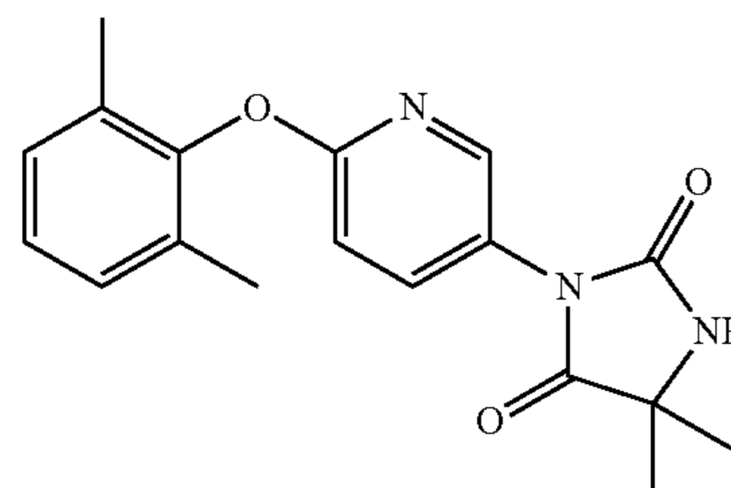
3-{6-[(2,6-dimethylphenyl)oxy]-3-pyridinyl}-5,5-dimethyl-2,4-imidazolidinedione
