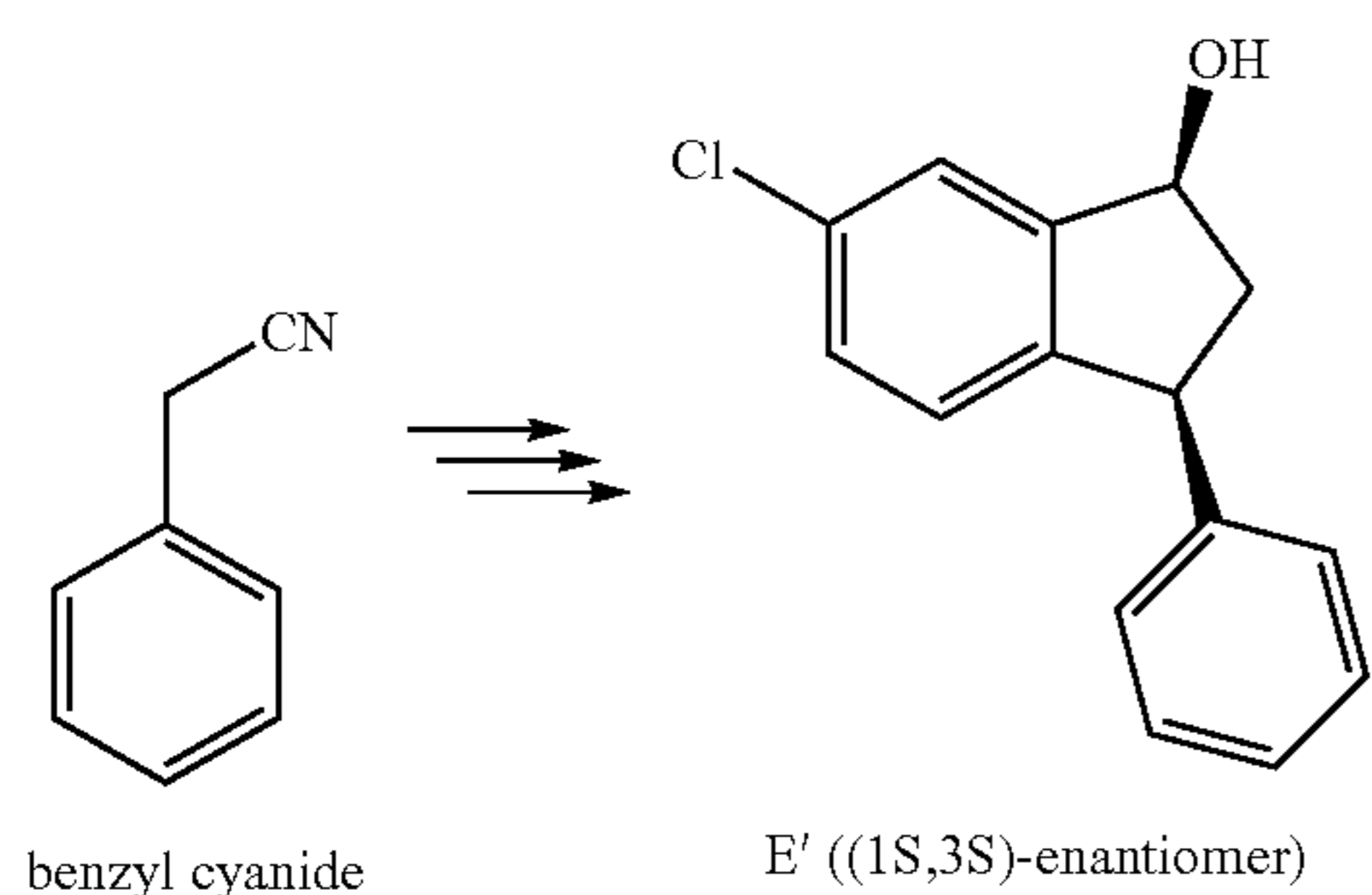
Scheme 4. Exemplary synthesis of intermediates E and E'.
