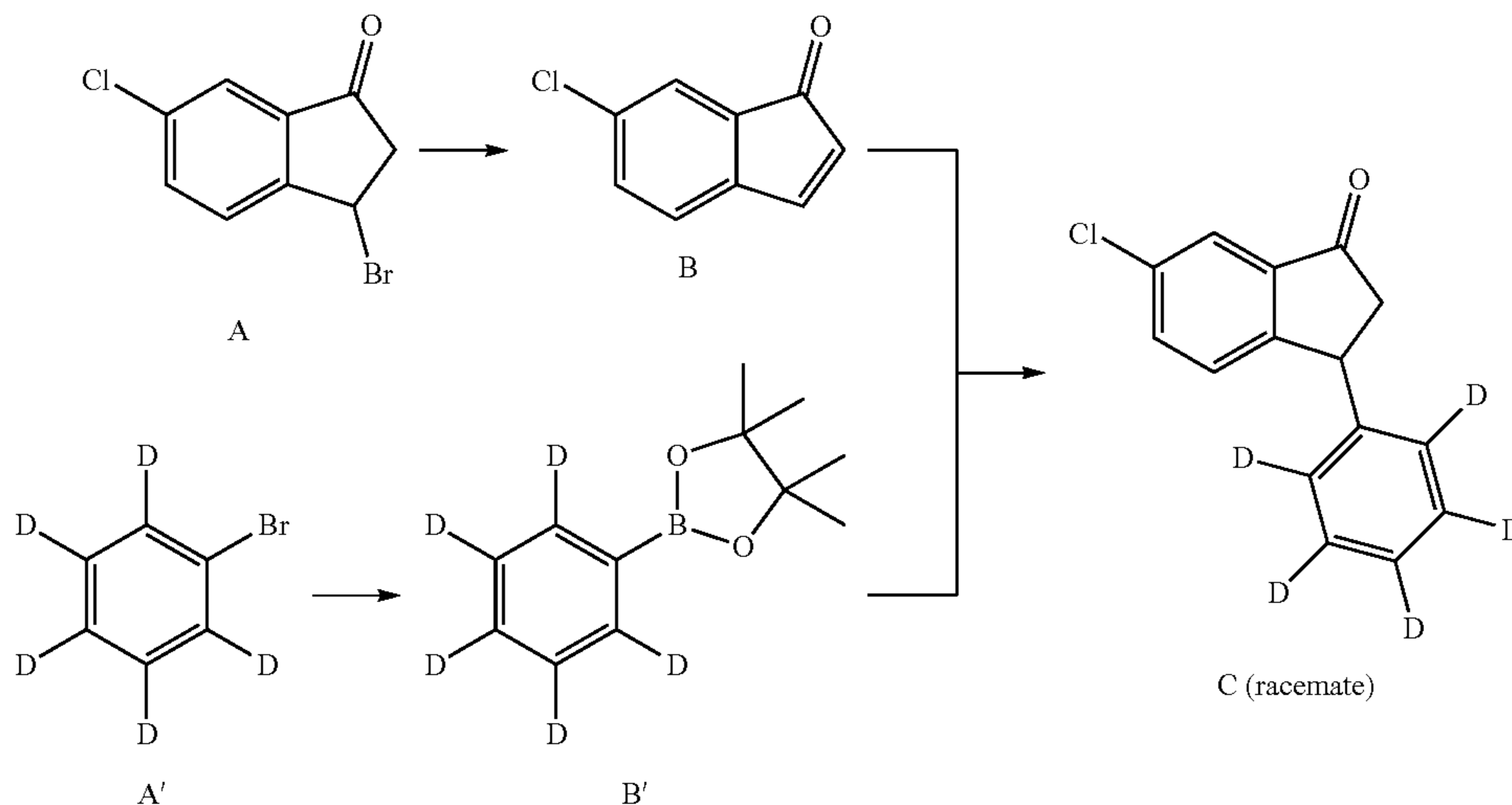
Scheme 9. Synthesis of Compound C.
