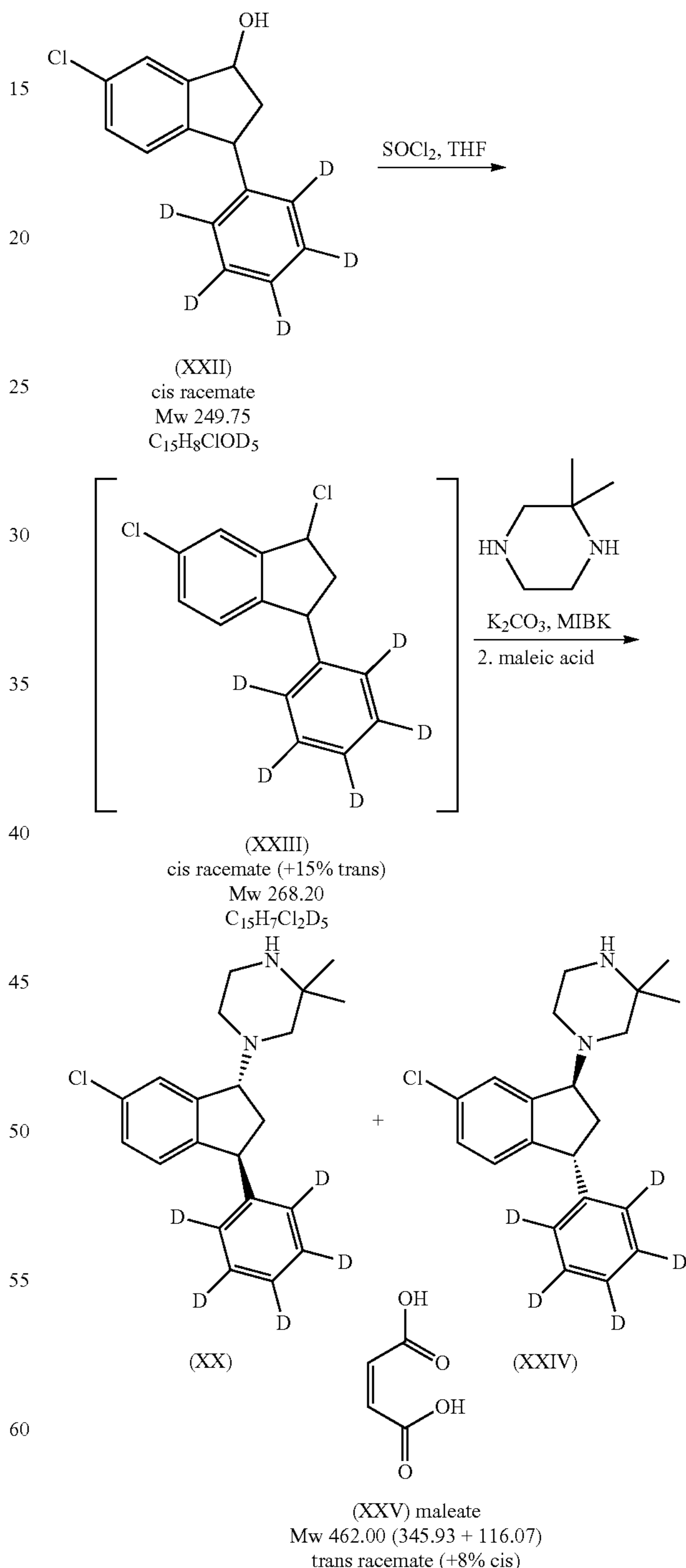
Scheme 16: Synthesis of rac-trans-1-(6-Chloro-3-phenyl(d 5 )-indan-1-yl)-3,3-dimethyl-piperazine maleate
