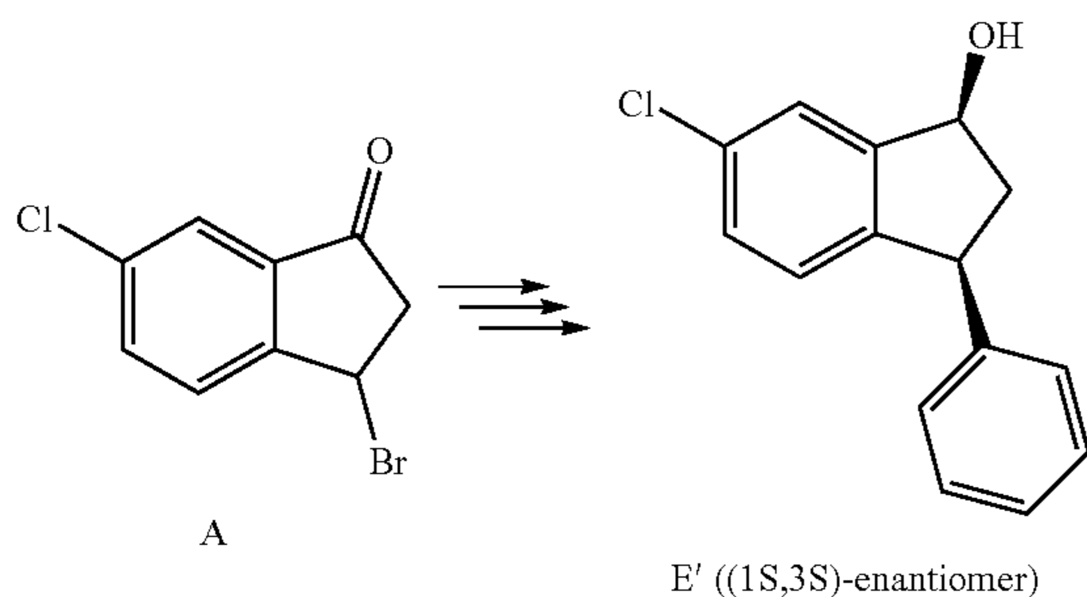
Scheme 3. Exemplary synthesis of intermediate E'.
