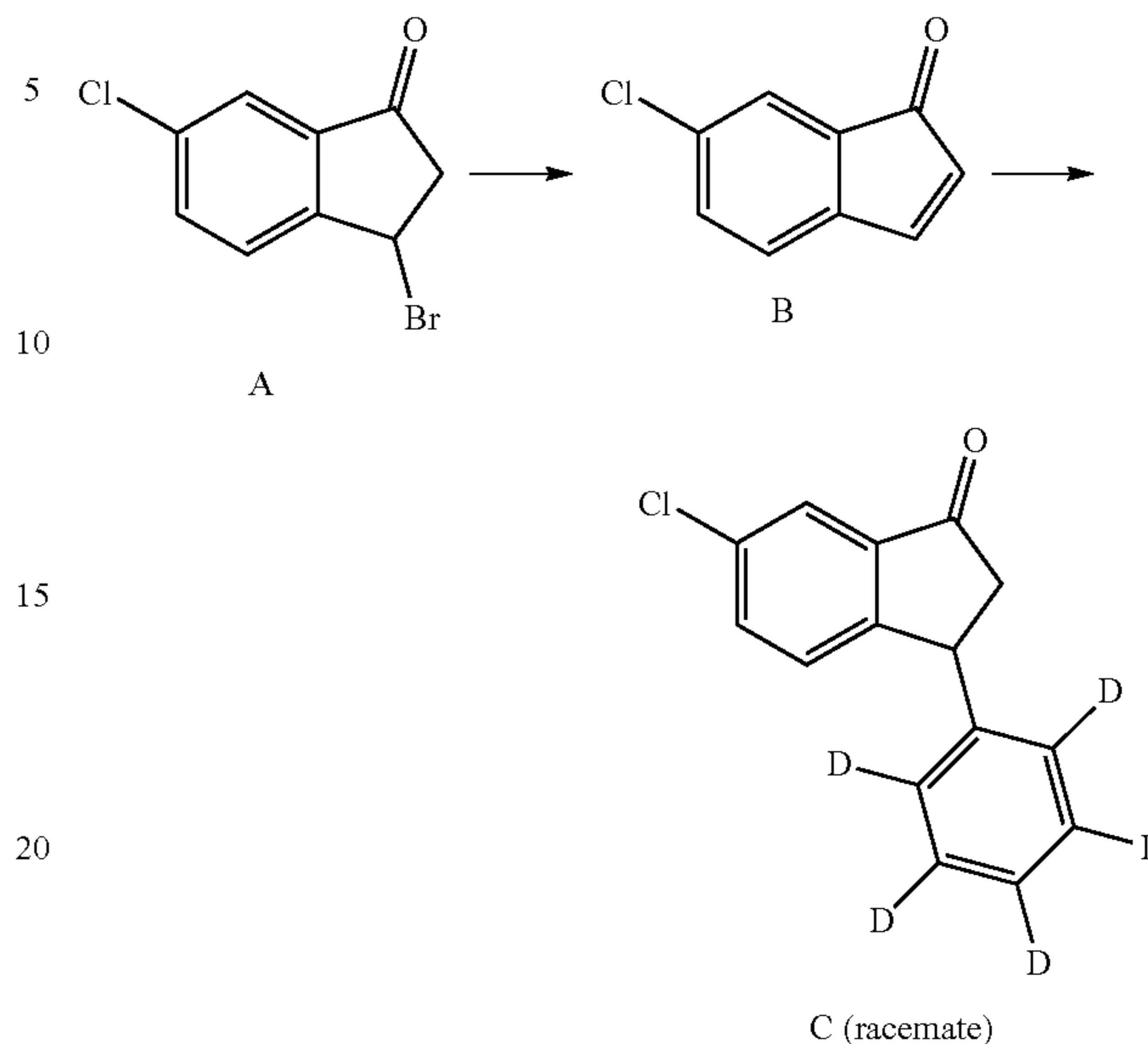
Scheme 1. Exemplary synthesis of intermediate C.
