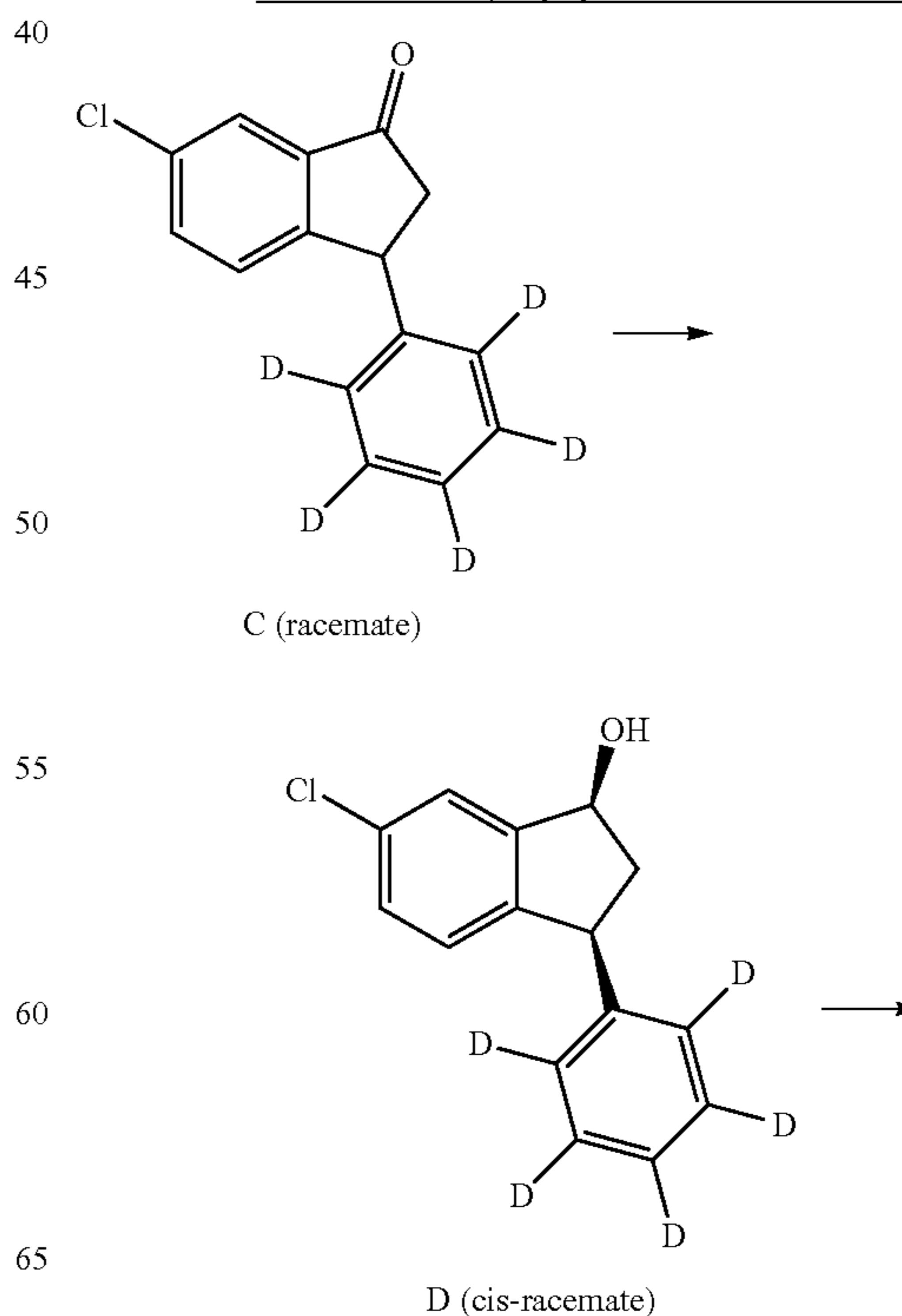
Scheme 2. Exemplary synthesis of intermediate E.
