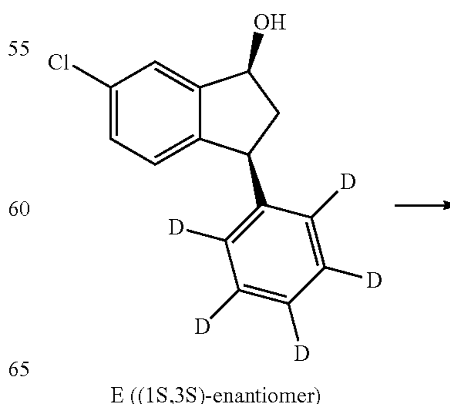
Scheme 5. Exemplary synthesis of intermediates F and Compounds (II) and (IV).
