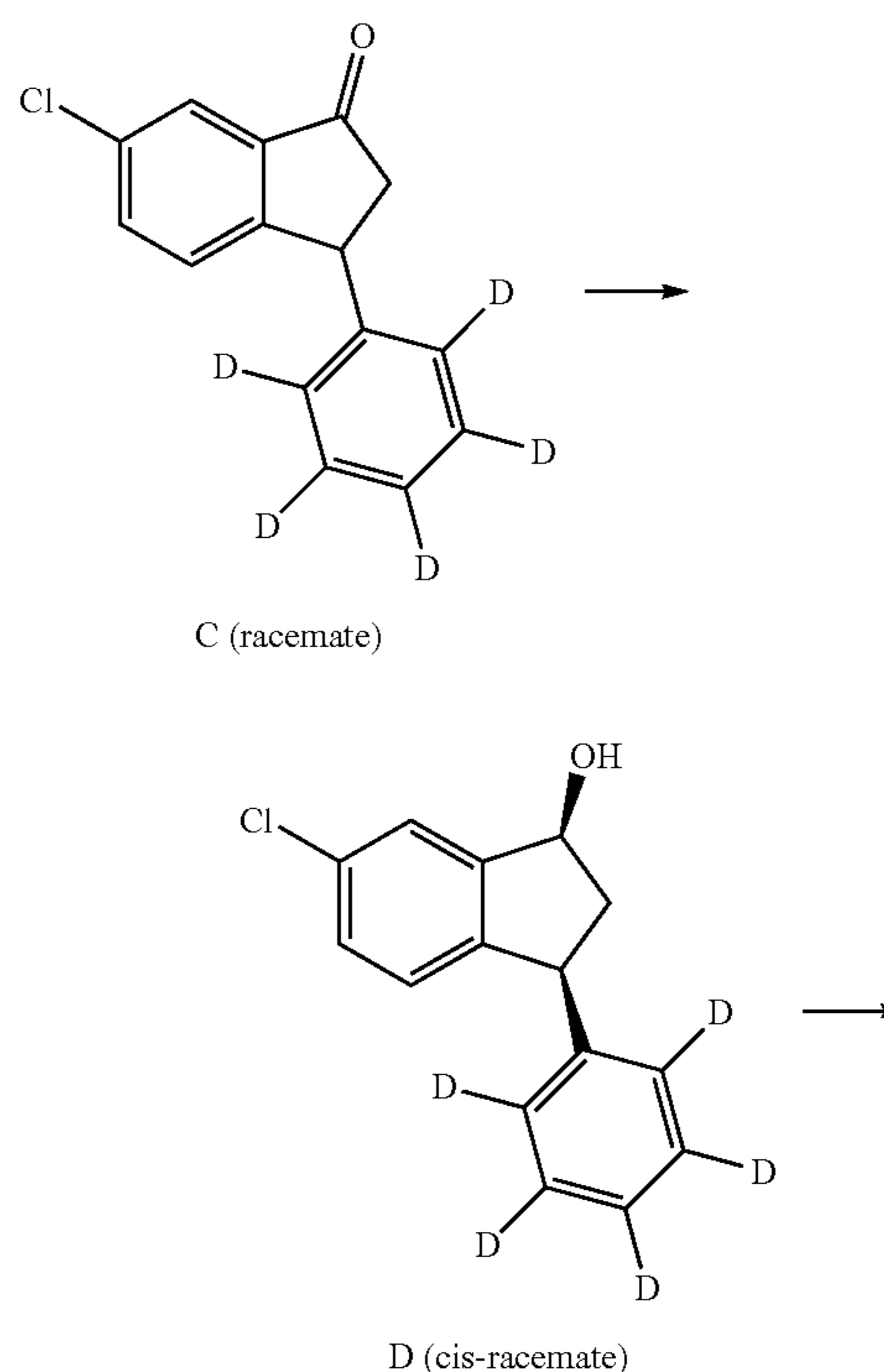
Scheme 10. Synthesis and resolution of Compound E.
