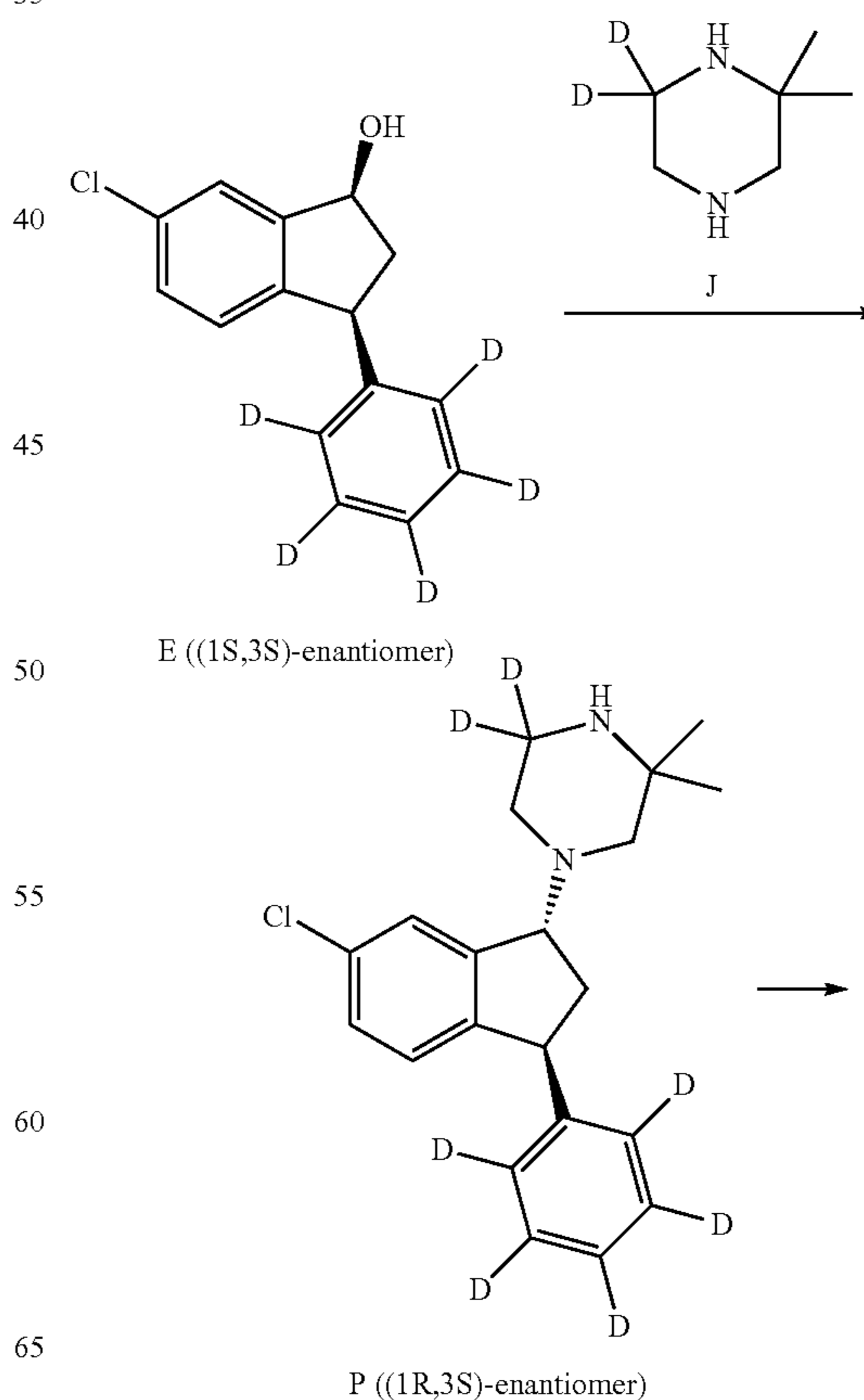
Scheme 13. Synthesis of Compound (VI) and Compound (VII).
