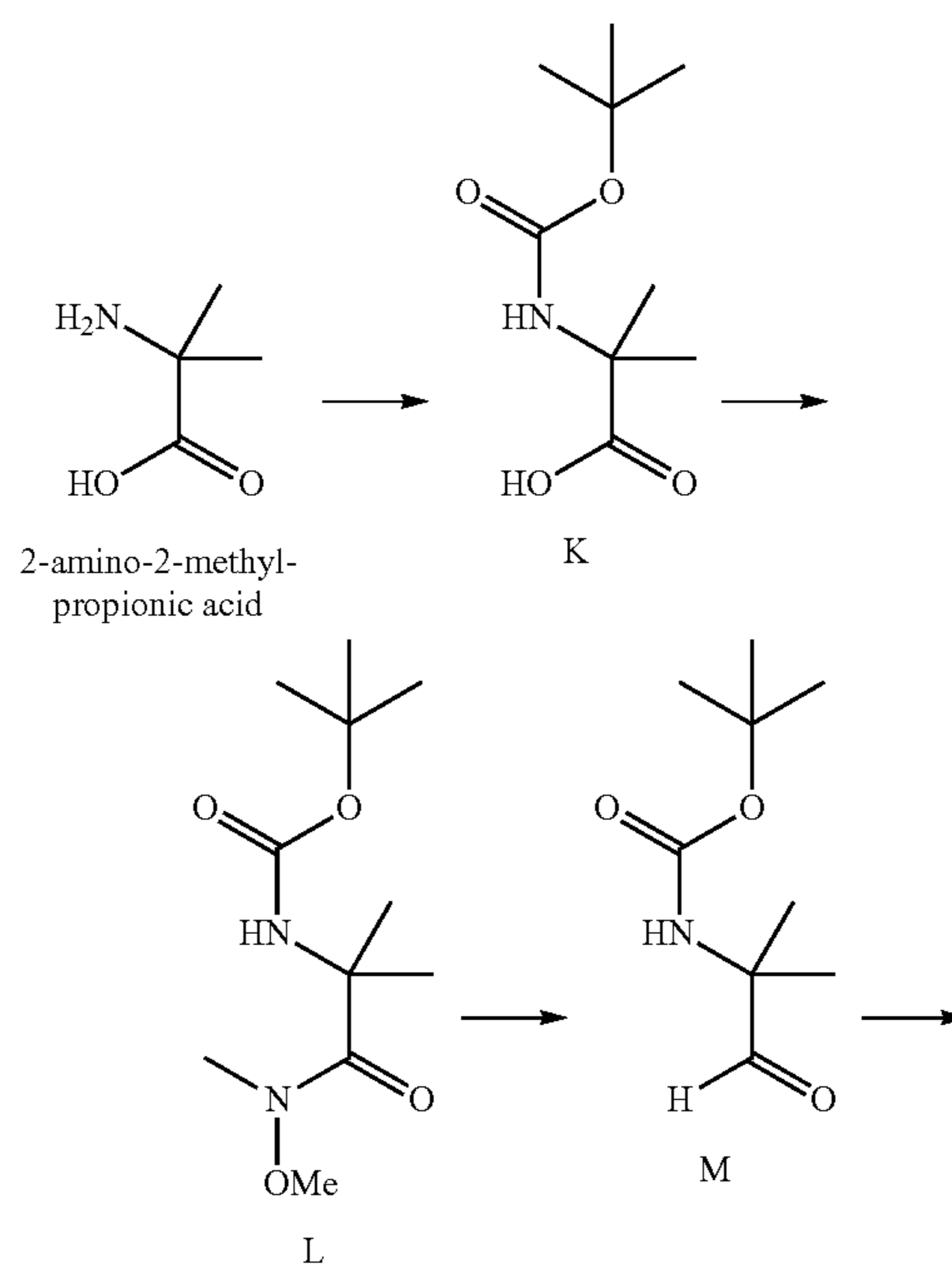
Scheme 11. Synthesis of intermediate J.
