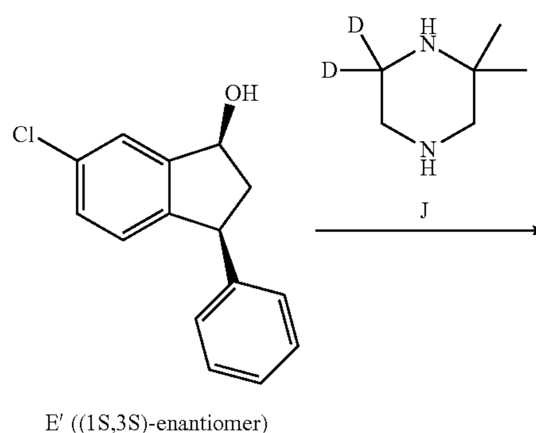
Scheme 12. Synthesis of Compound (III) and Compound (V).
