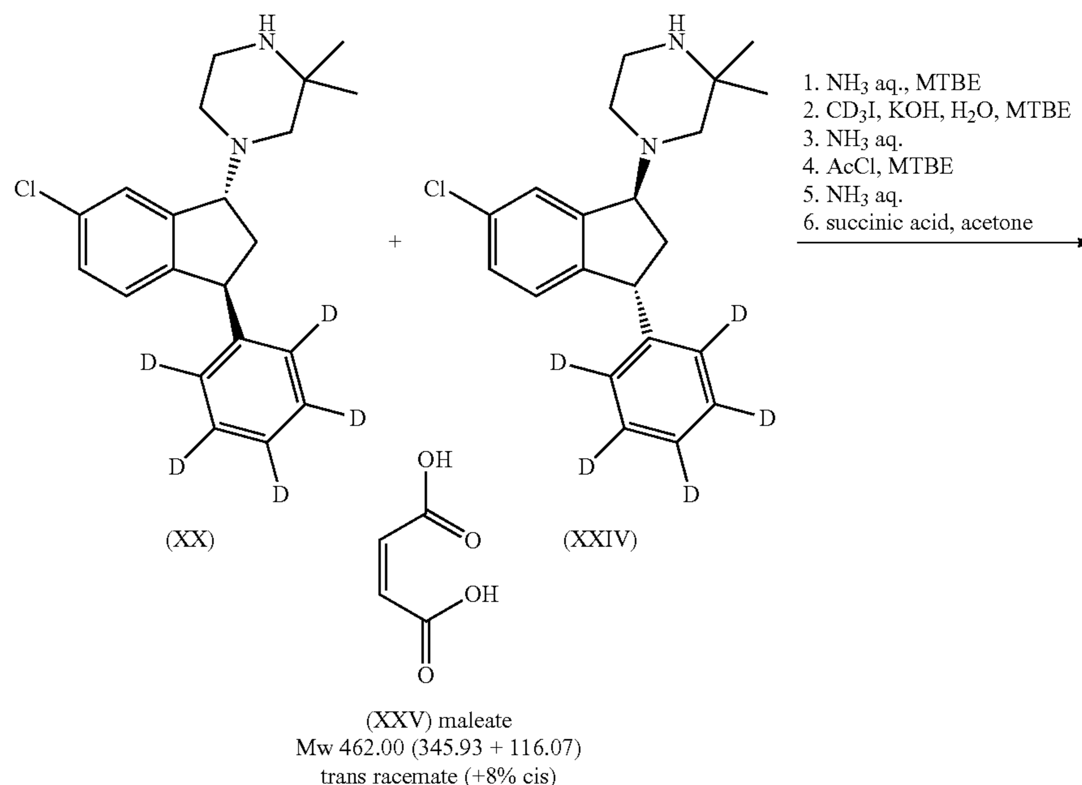
Scheme 17: Synthesis of rac-trans-1-(6-chloro-3-phenyl(d 5 )-indan-1-yl)-1-(d 3 ), 2,2-trimethyl-piperazine succinate
