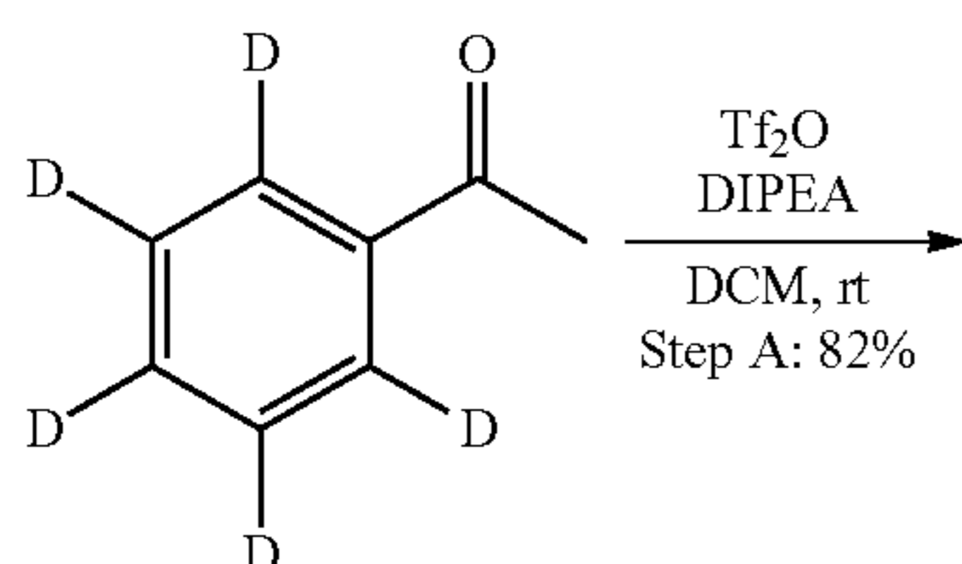
Scheme 14. Synthesis of Compound (XV)
