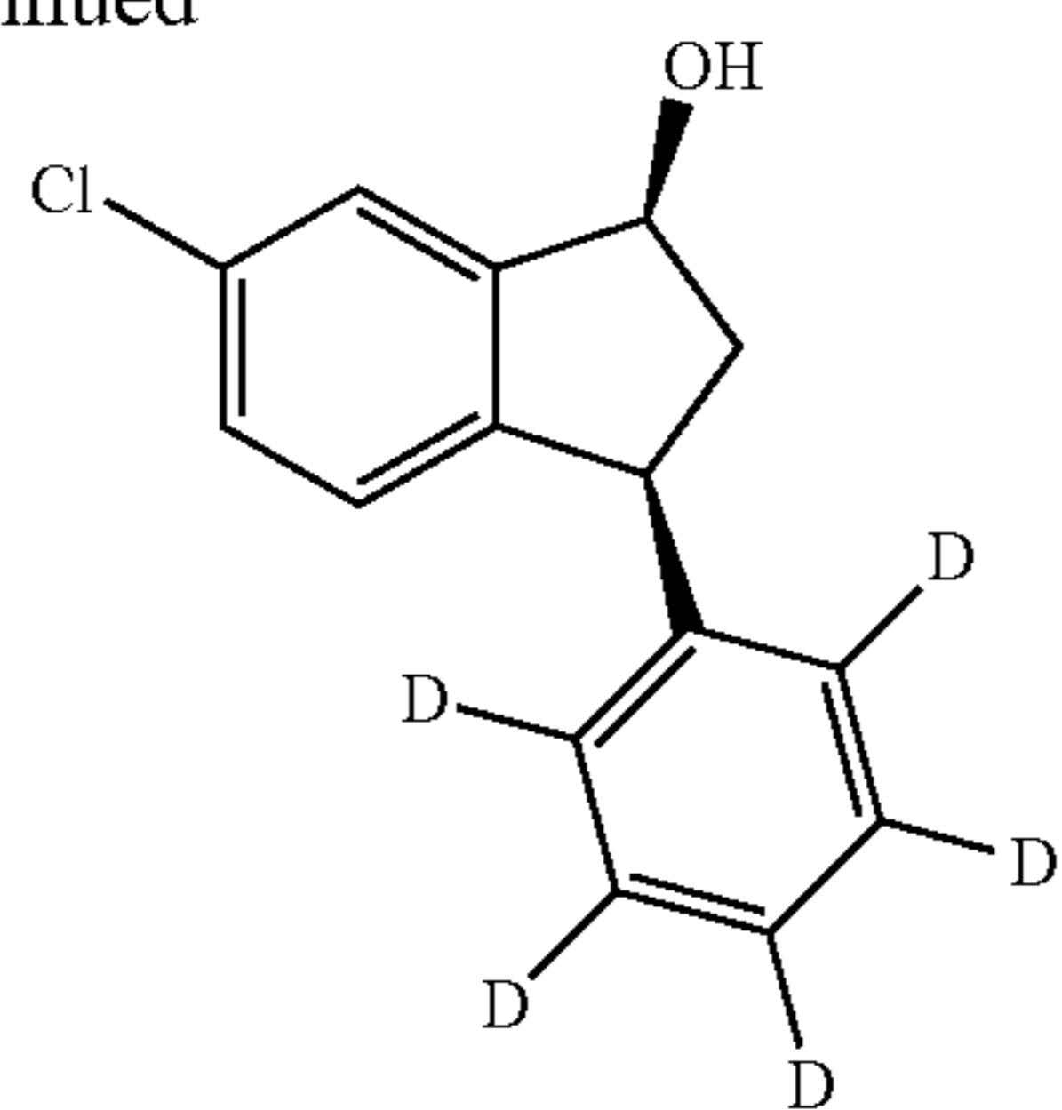
E ((1S,3S)-enantiomer)
