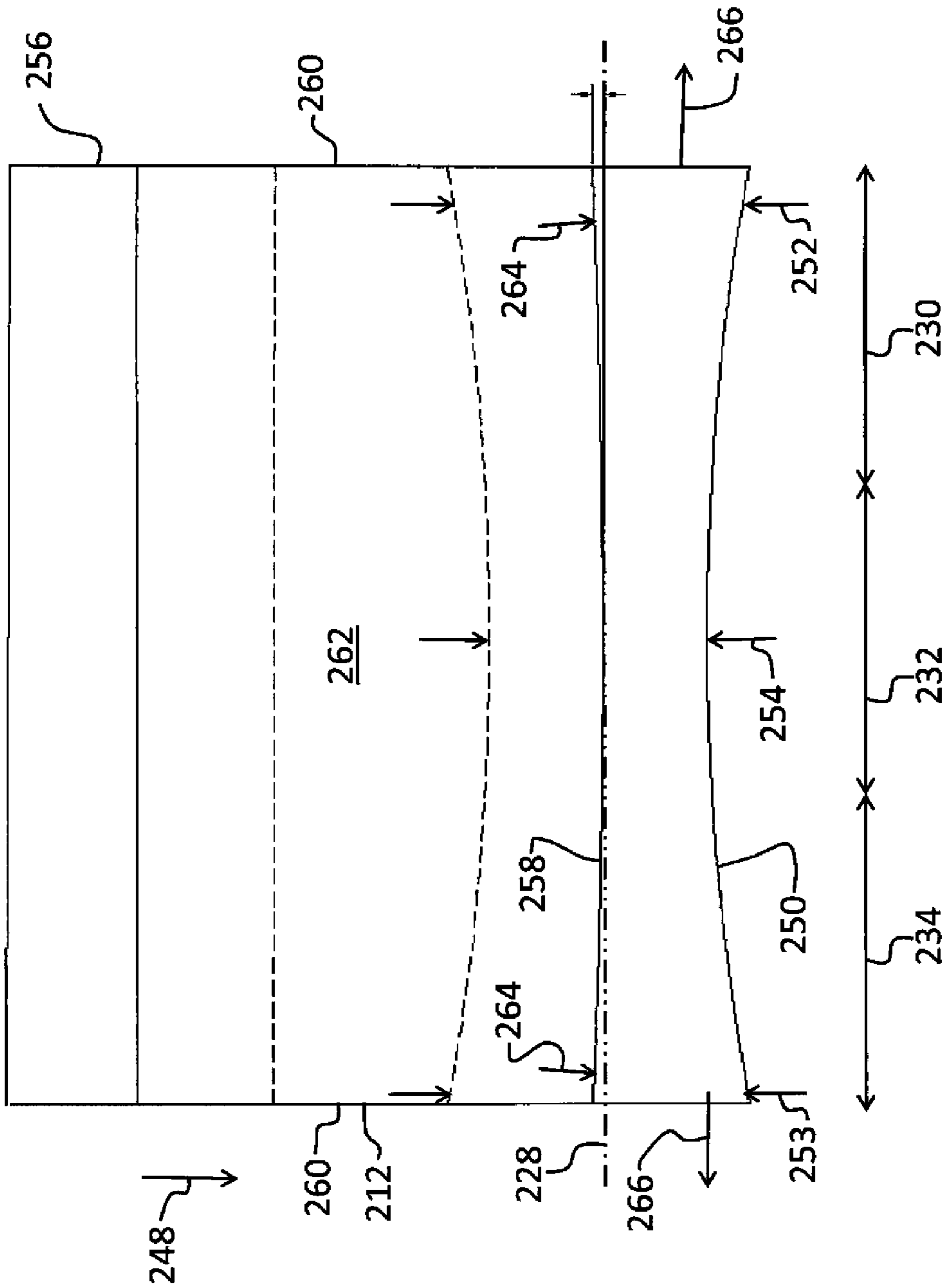
FIG. 4 (Prior Art)
