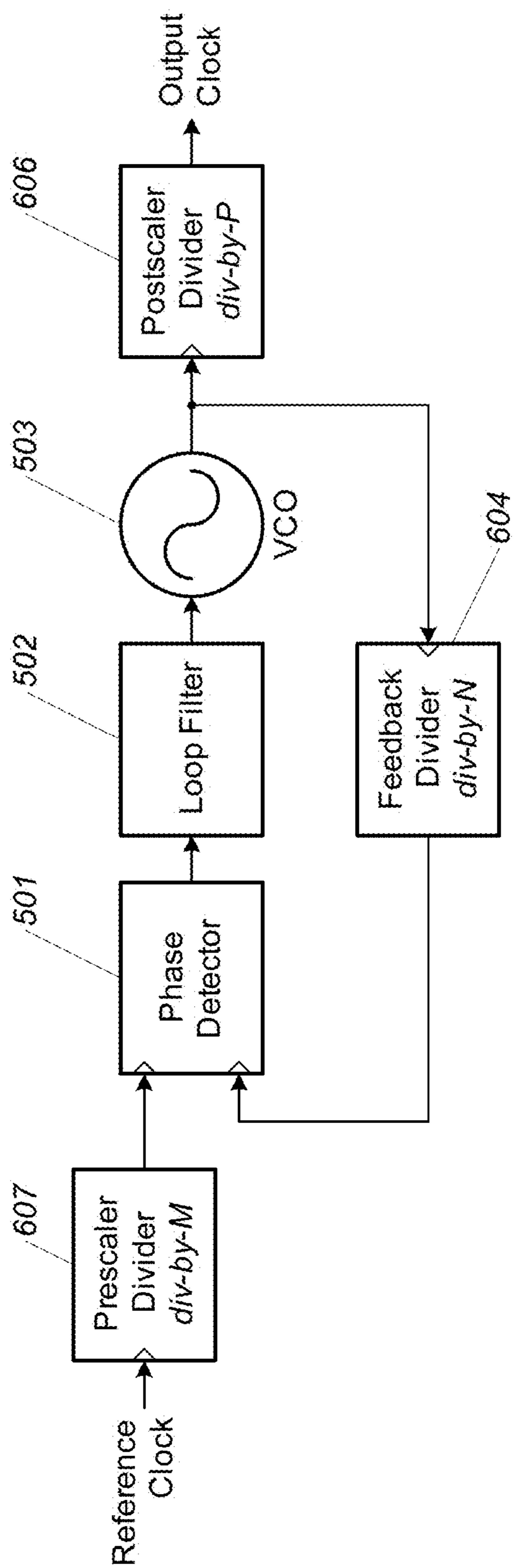
Figure 6 (PRIOR ART)
