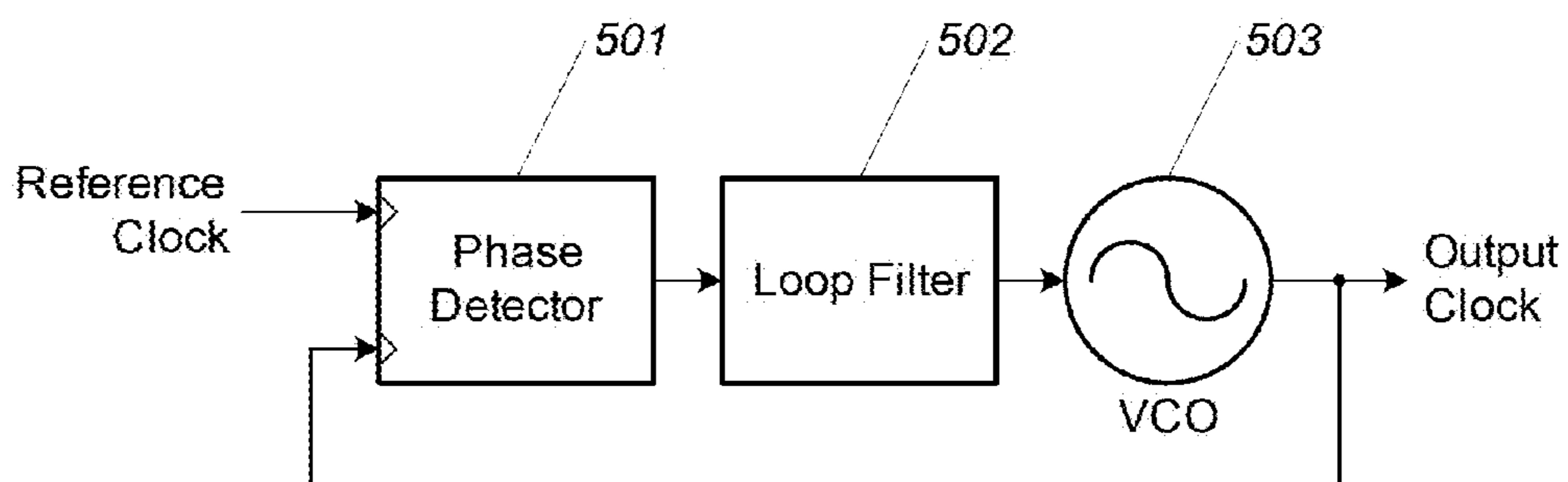
Figure 5 (PRIOR ART)
