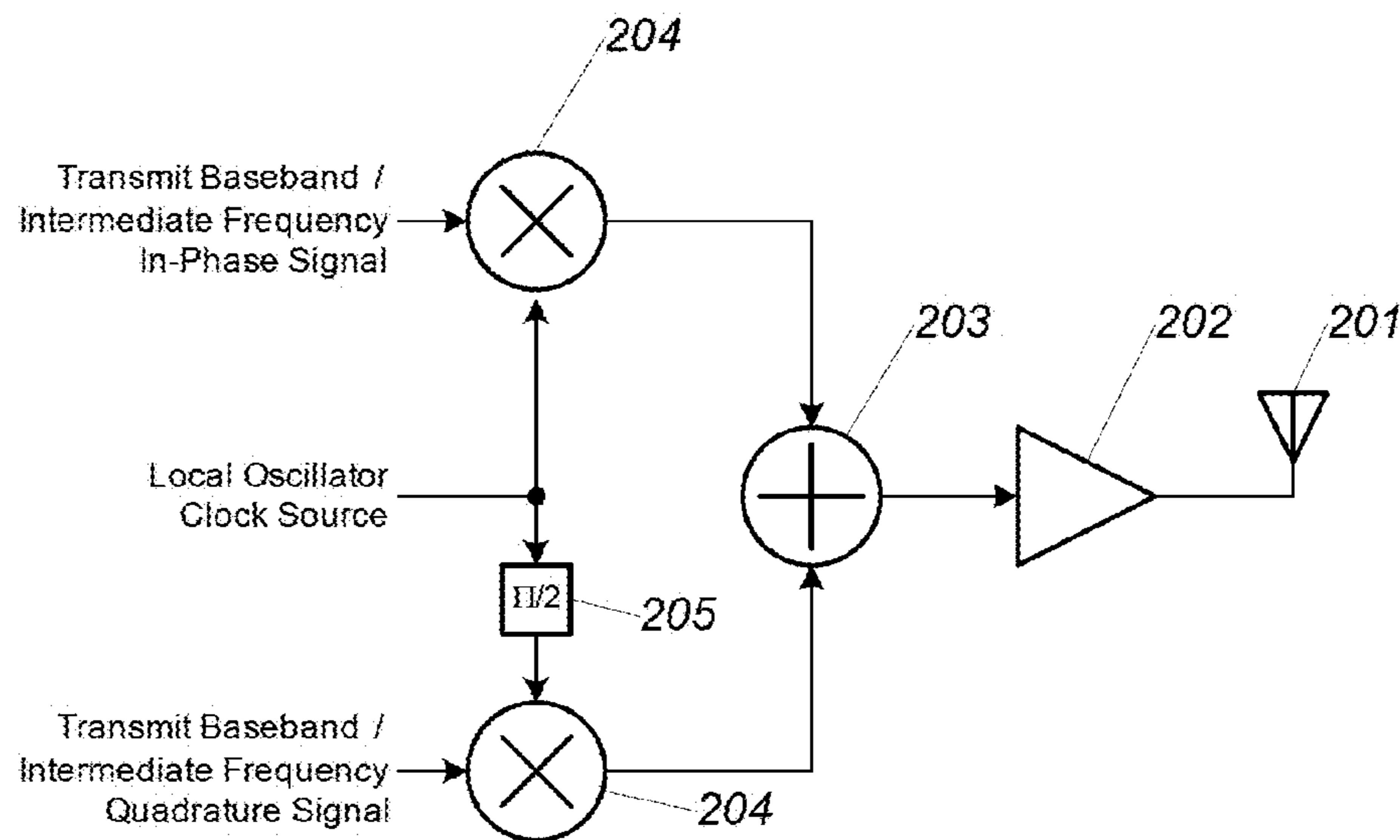
Figure 2 (PRIOR ART)
