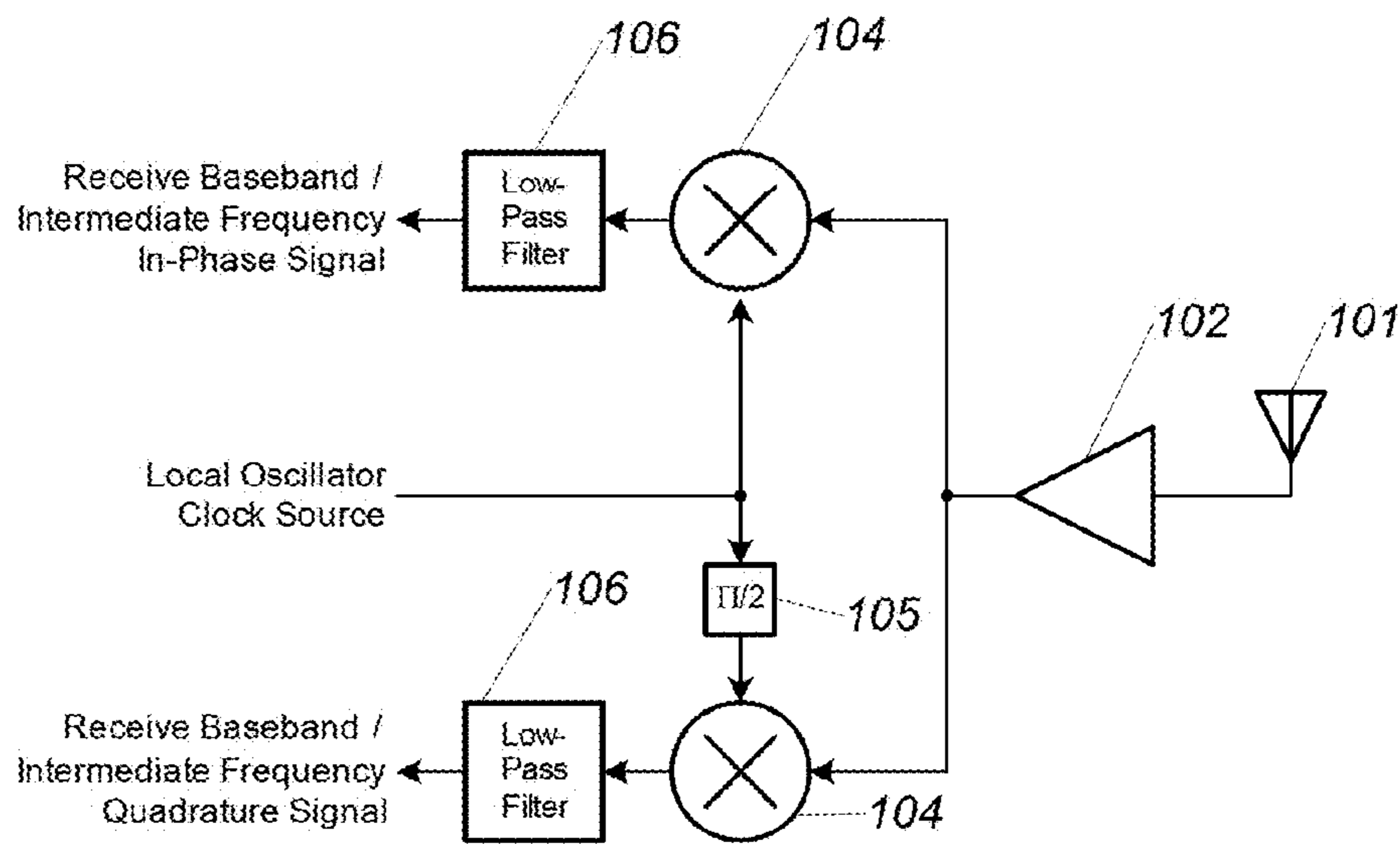
Figure 1 (PRIOR ART)
