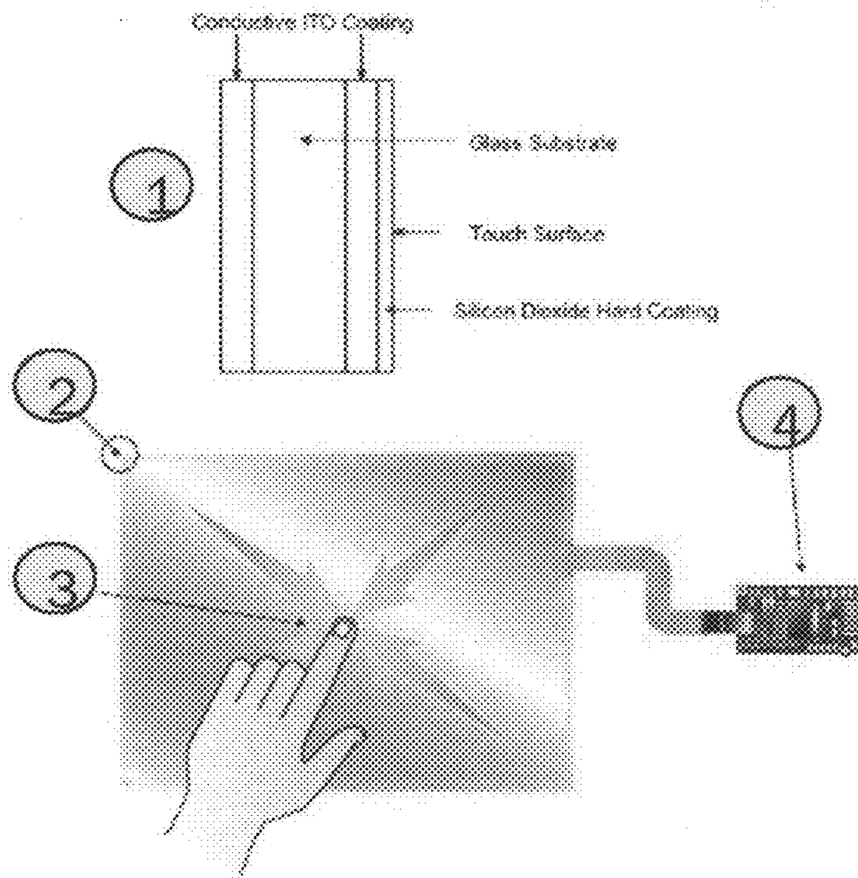
FIG. 3 (PRIOR ART)
