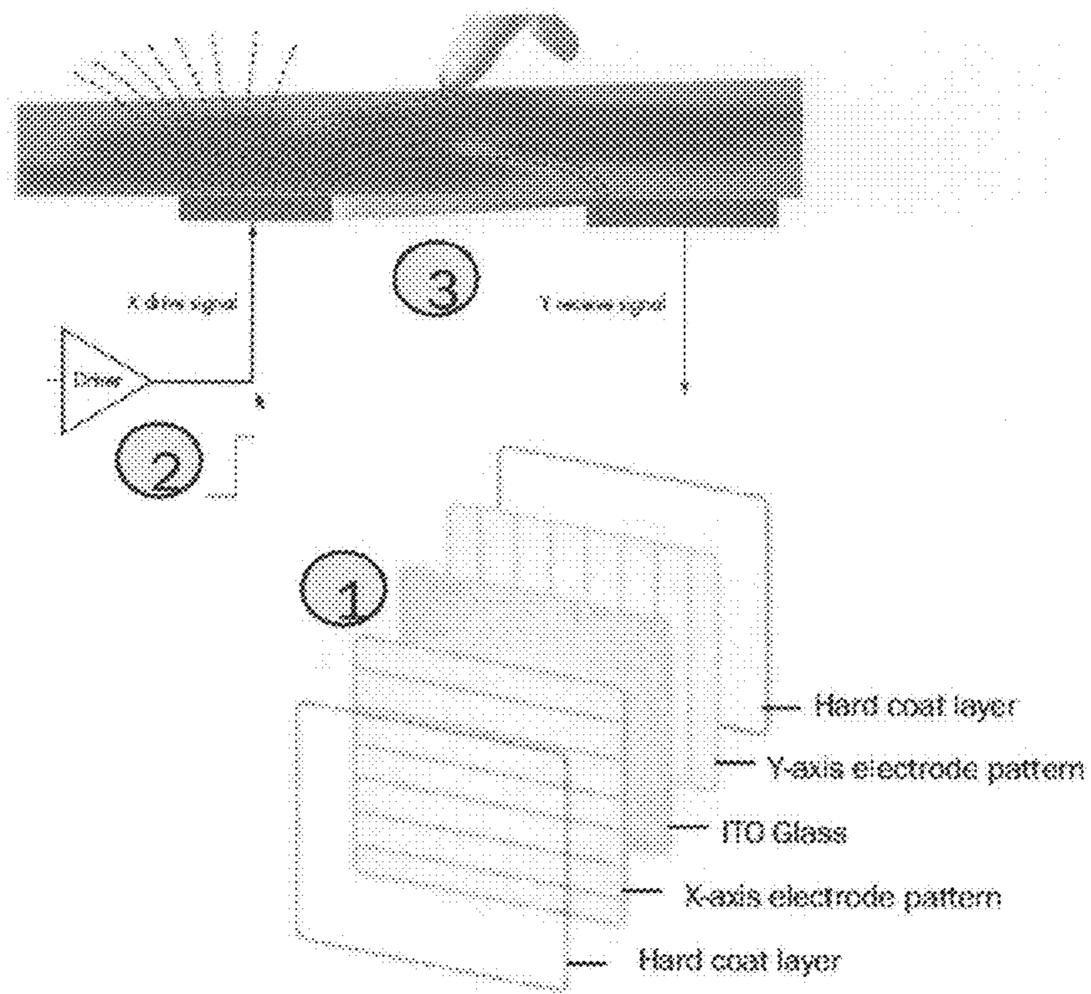
FIG. 4 (PRIOR ART)
