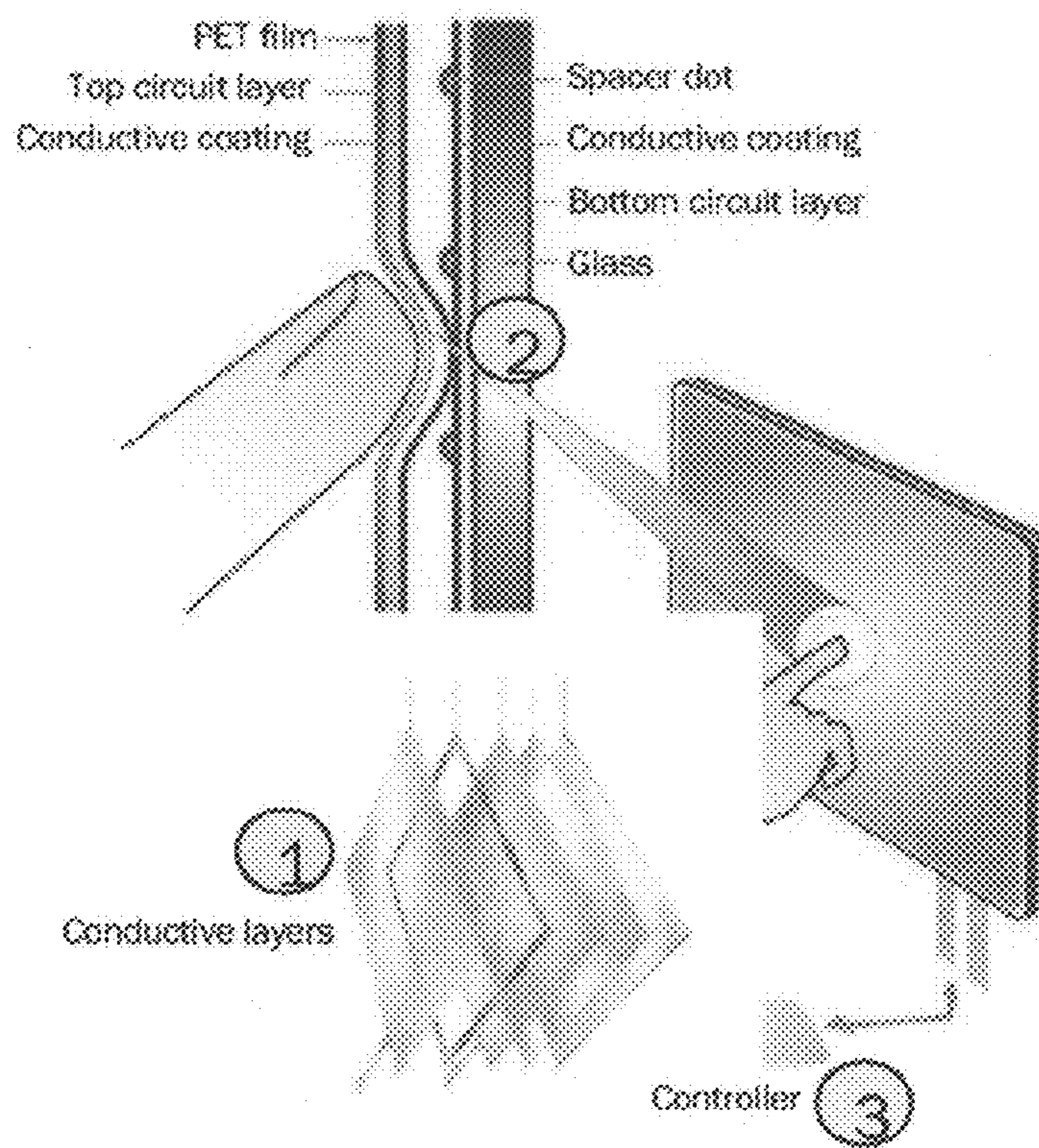
FIG. 2 (PRIOR ART)
