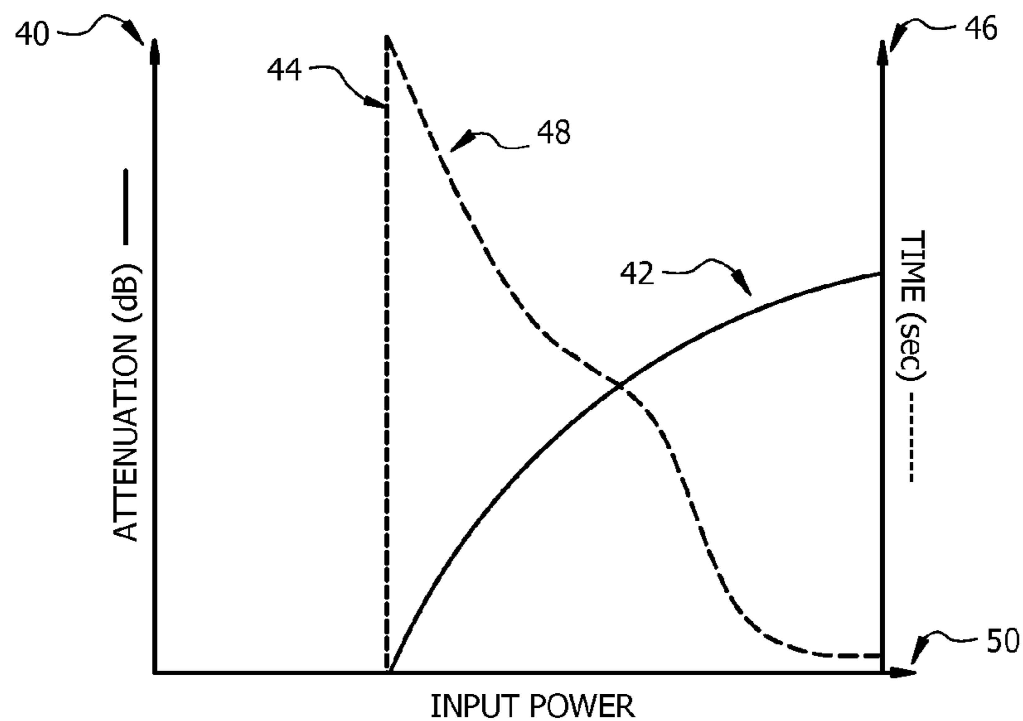
TYPICAL LOUDSPEAKER POWER HANDLING PERFORMANCE
