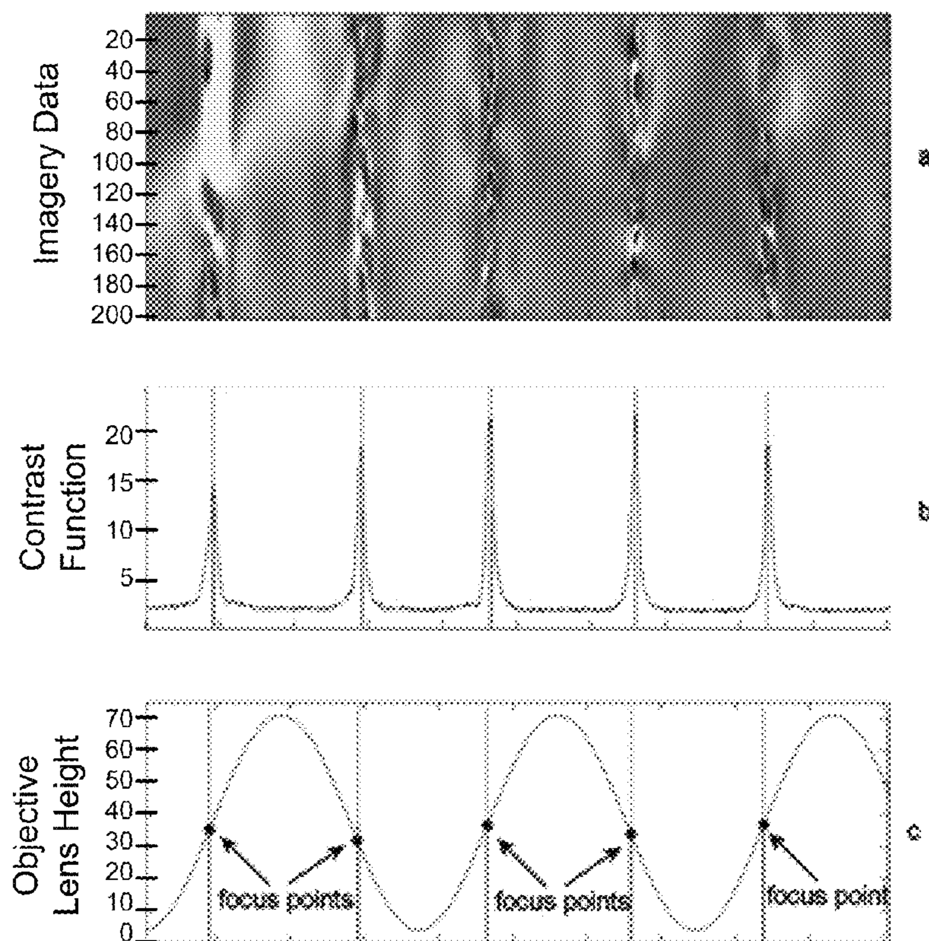
FIG. 5 Time / Position
