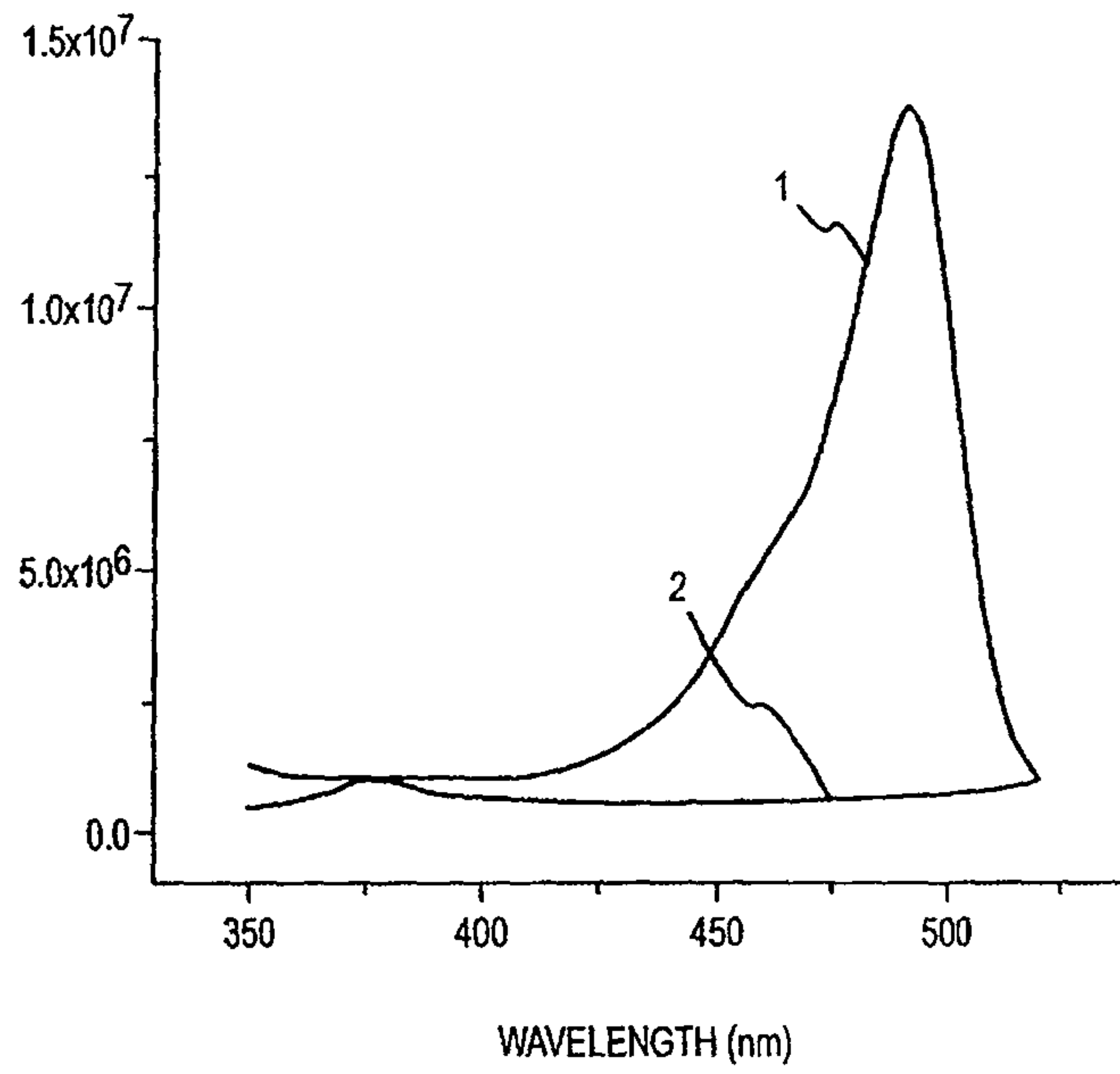
UV ABSORPTION SPECTRA: (1) FLUORESCHEIN (2) FLUORESCHEIN + DPI AFTER SINGLE FLASH FROM CAMERA STROBE
