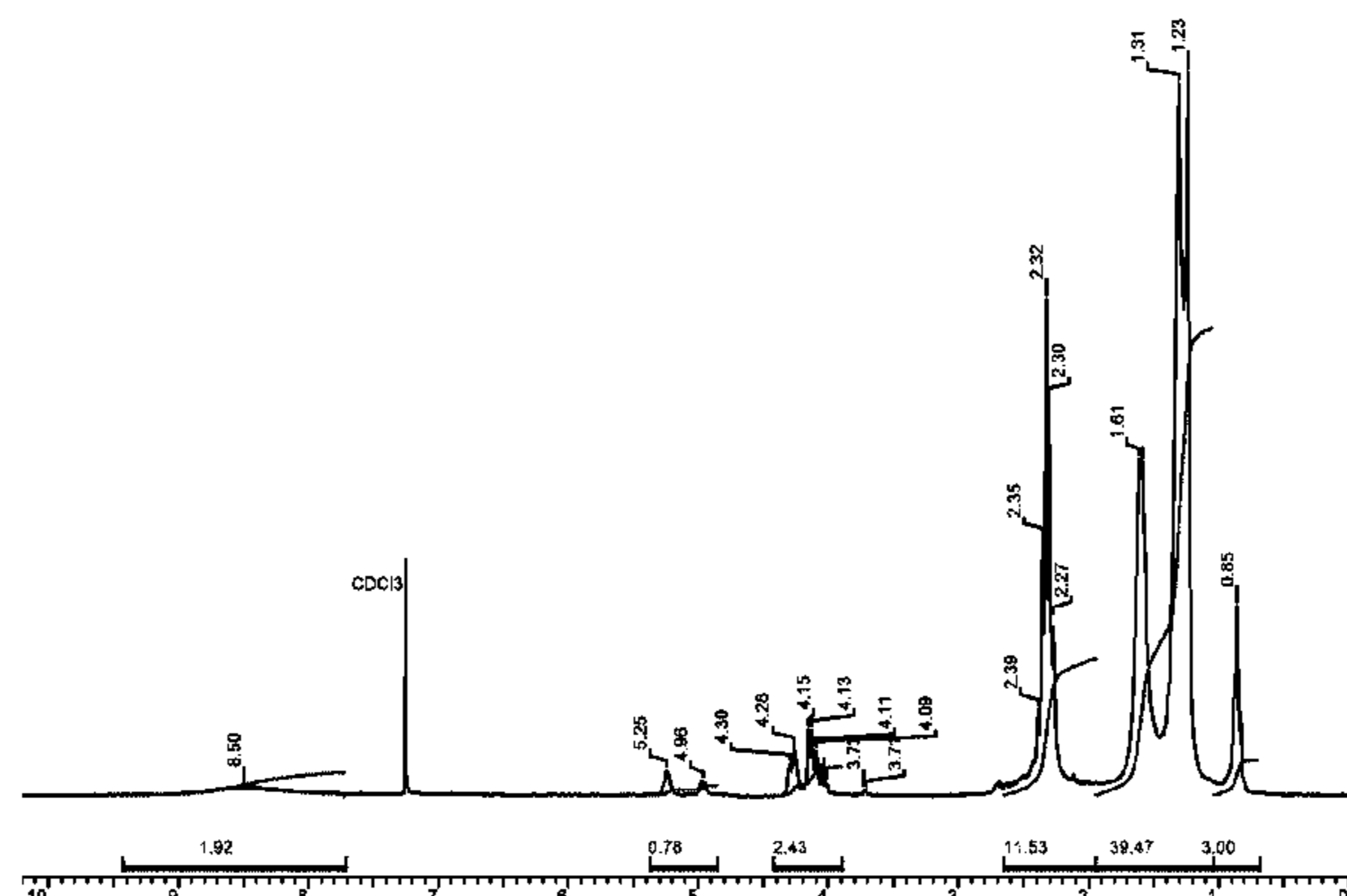
H-NMR spectrum of the mixture of triglycerides containing saturated carboxylic acids having more than one acid function of Example 1
