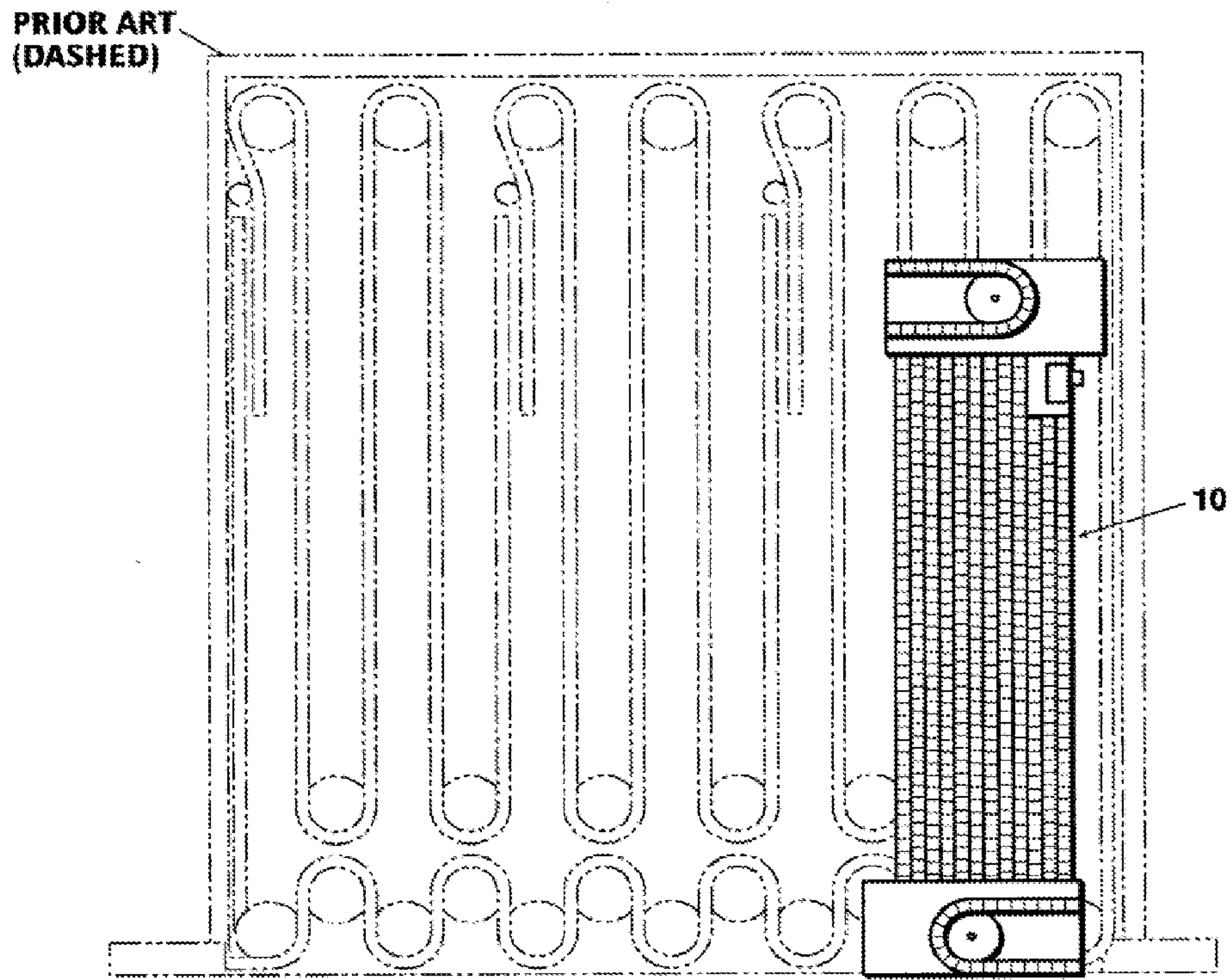
Fig. 20 FOOTPRINT COMPARISON
