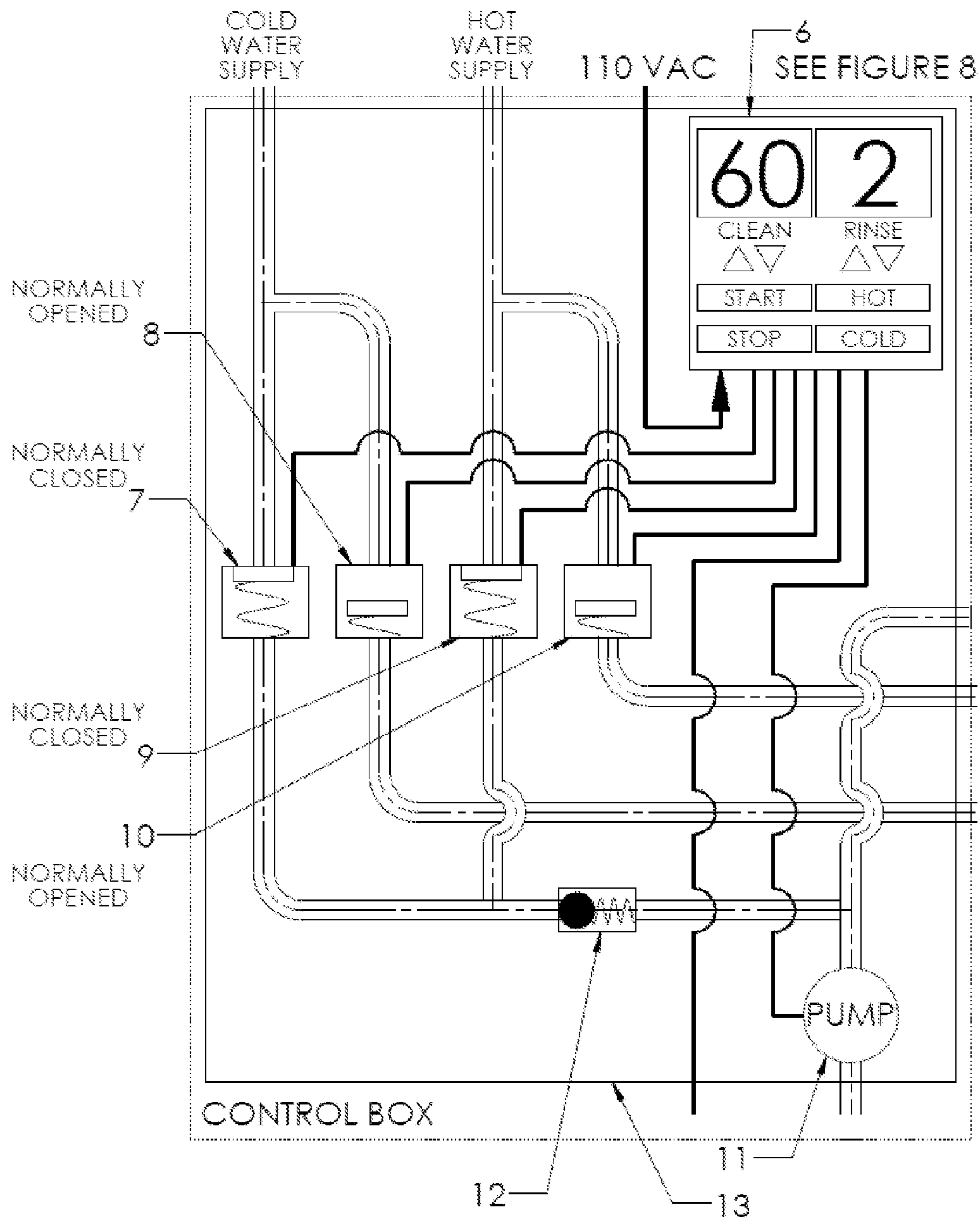
FIGURE 5: CONTROL BOX COMPONENTS
