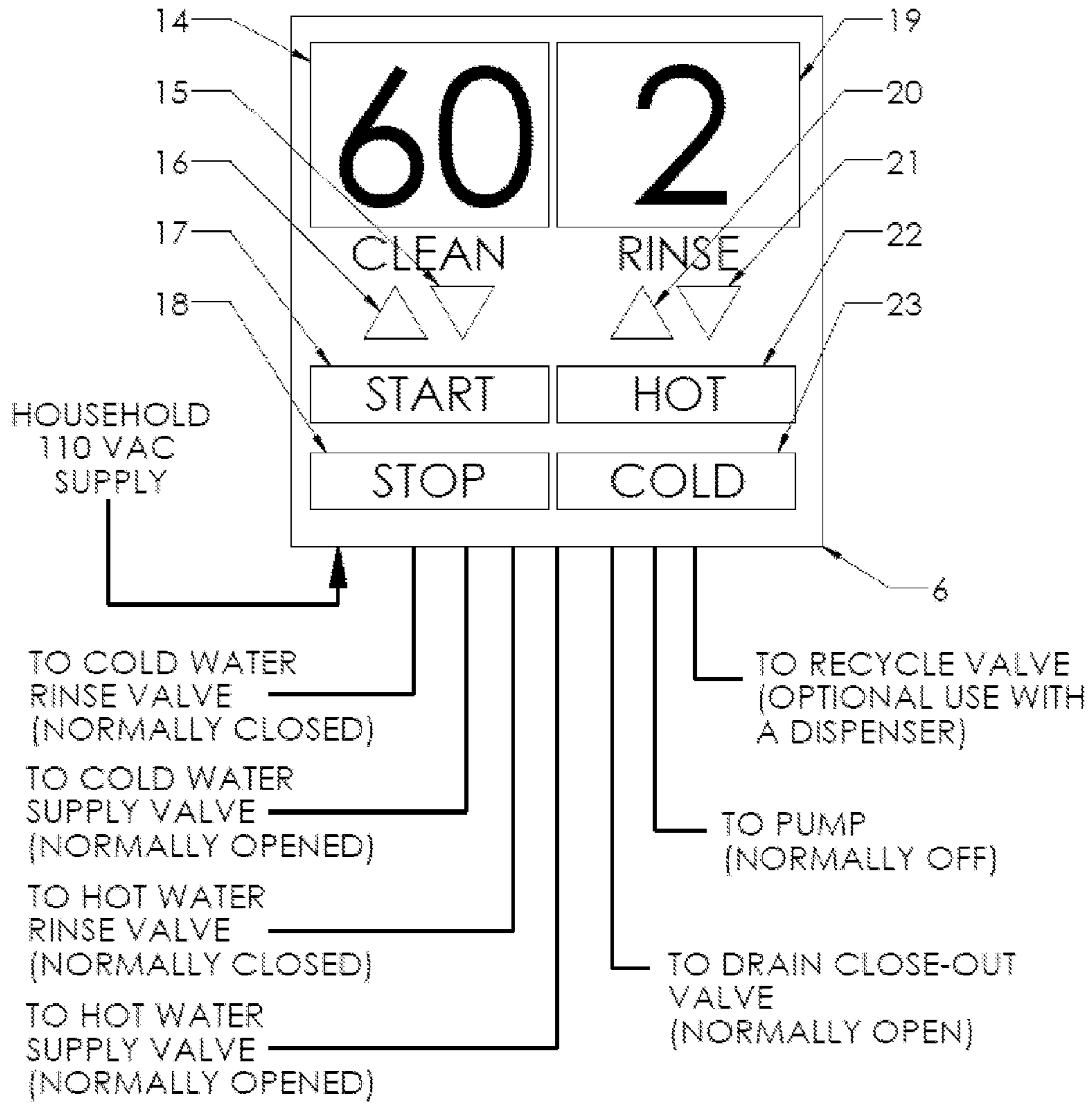
FIGURE 8: CONTROL PANEL/CIRCUIT BOARD
