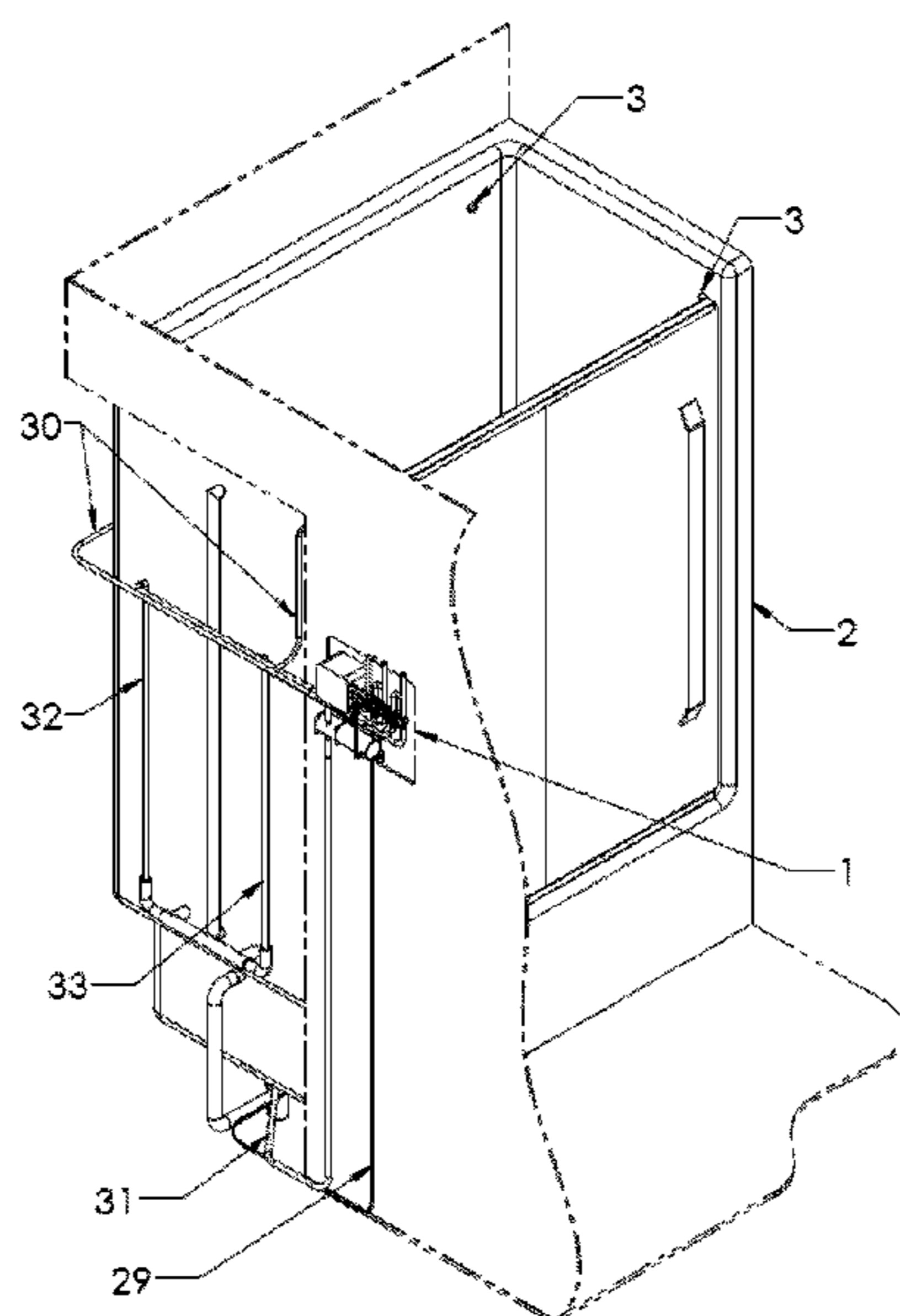
SELF-CLEANING SHOWER/BATHTUB (VIEW FROM BEHIND WALL)
