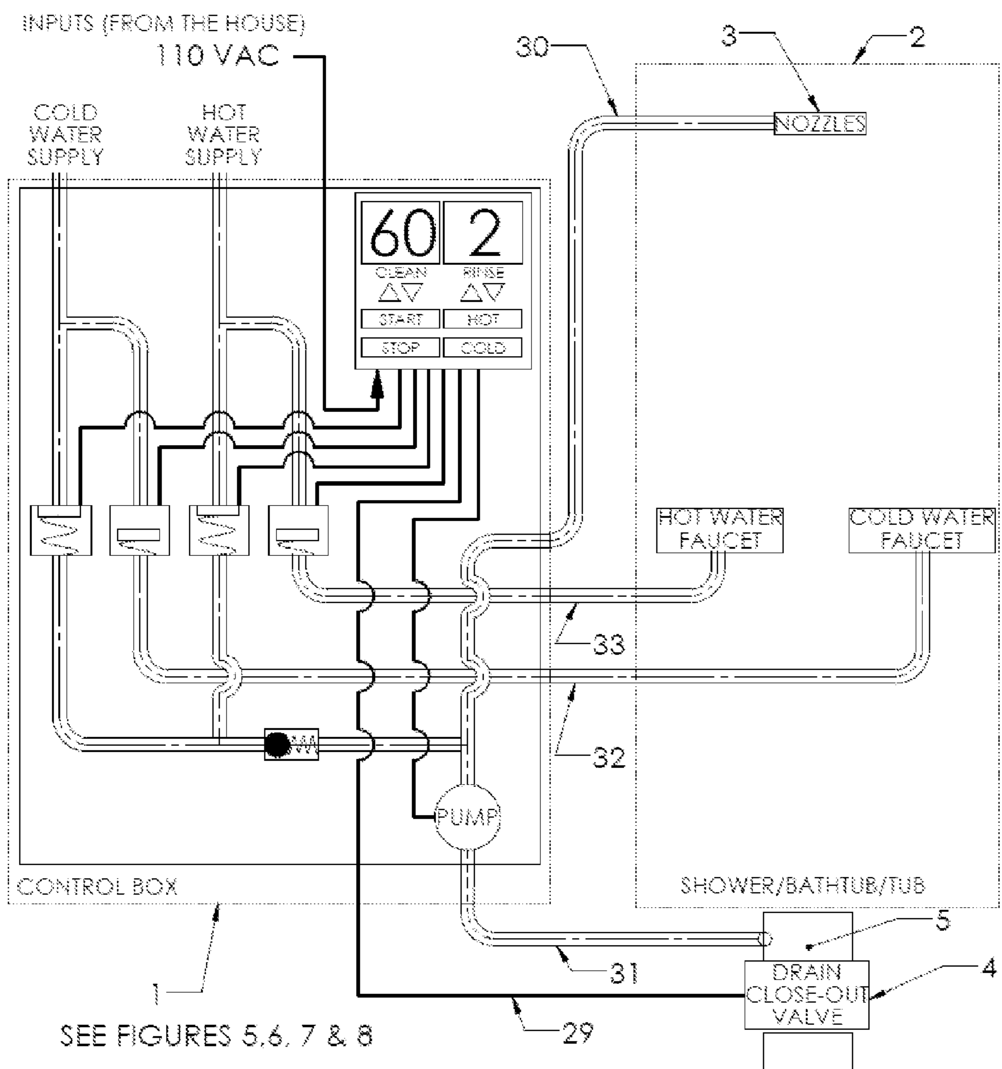
FIGURE 4: SELF-CLEANING SHOWER/BATHTUB/TUB
