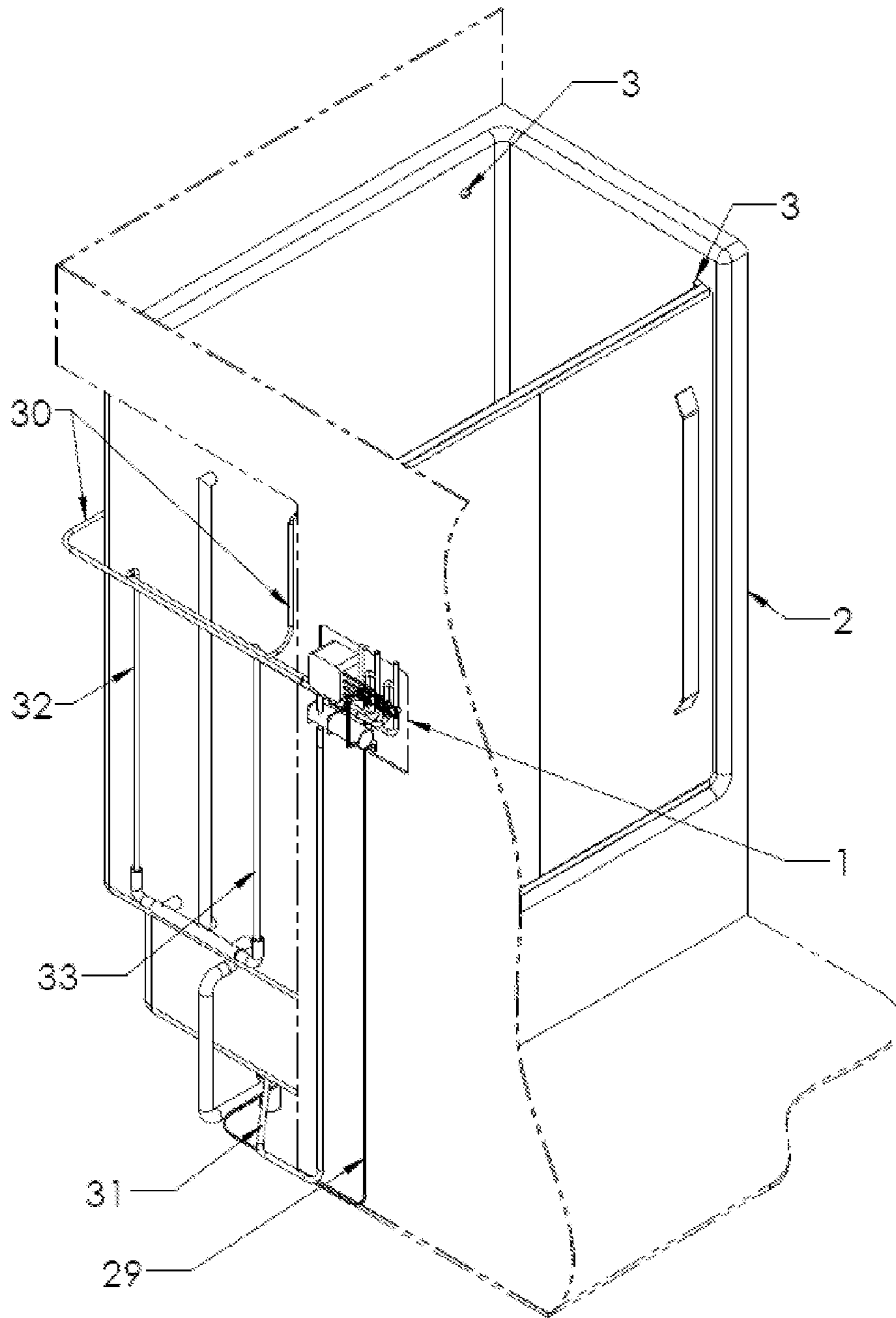
FIGURE 1: SELF-CLEANING SHOWER/BATHTUB (VIEW FROM BEHIND WALL)
