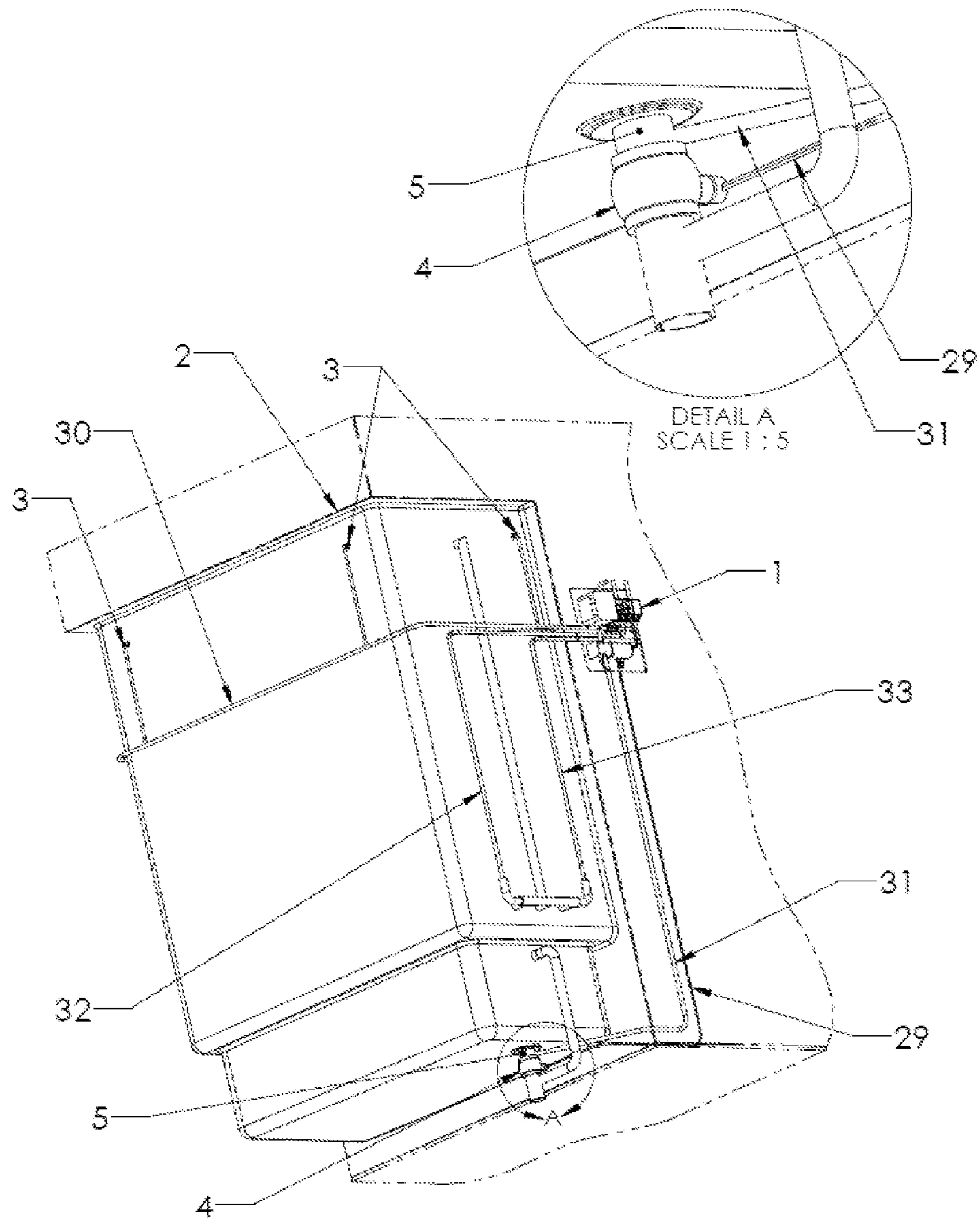
FIGURE 3: DRAIN CLOSE-OUT VALVE AND RESERVOIR
