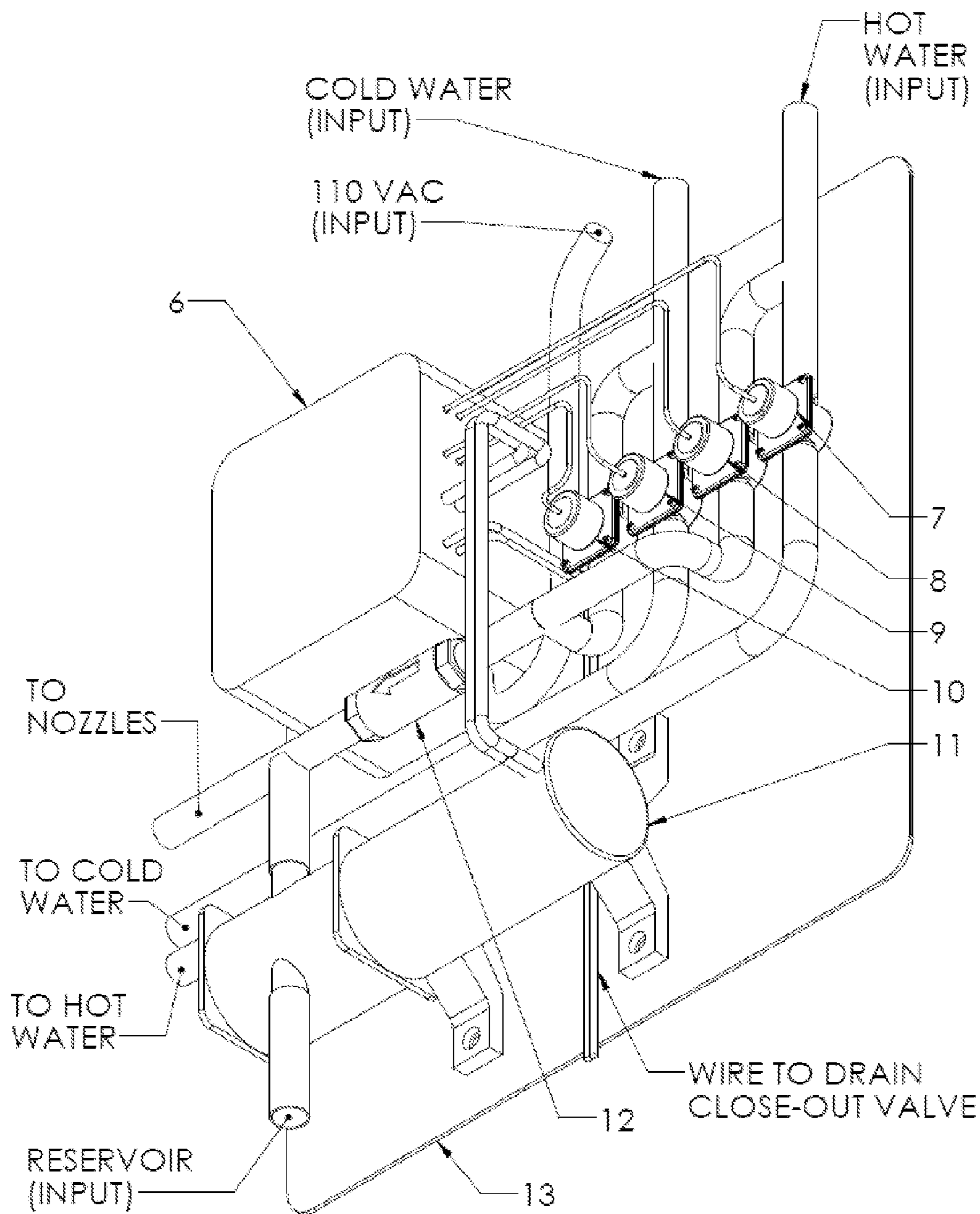
FIGURE 6: CONTROL BOX INPUTS & OUTPUTS
