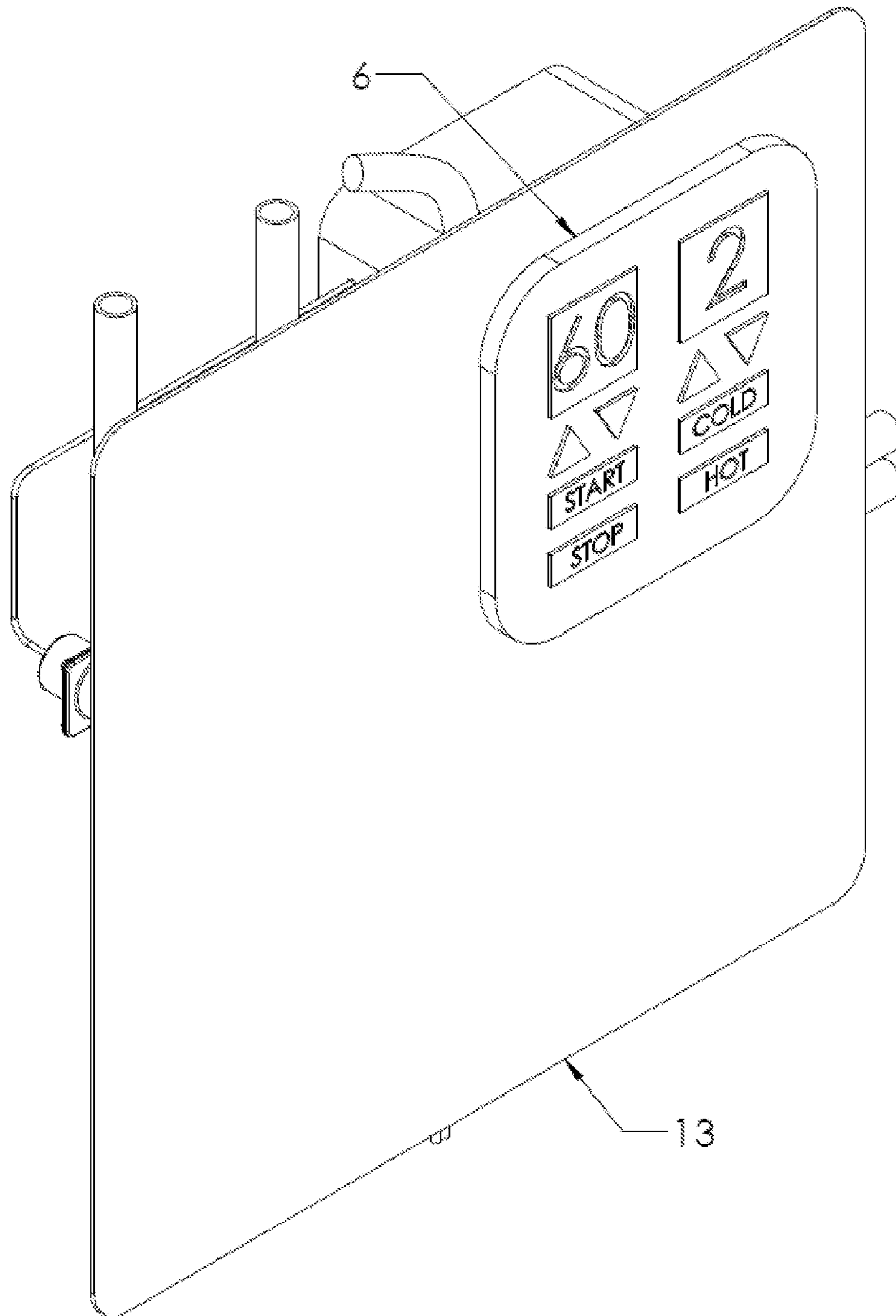
FIGURE 7: CONTROL PANEL (USER INTERFACE)
