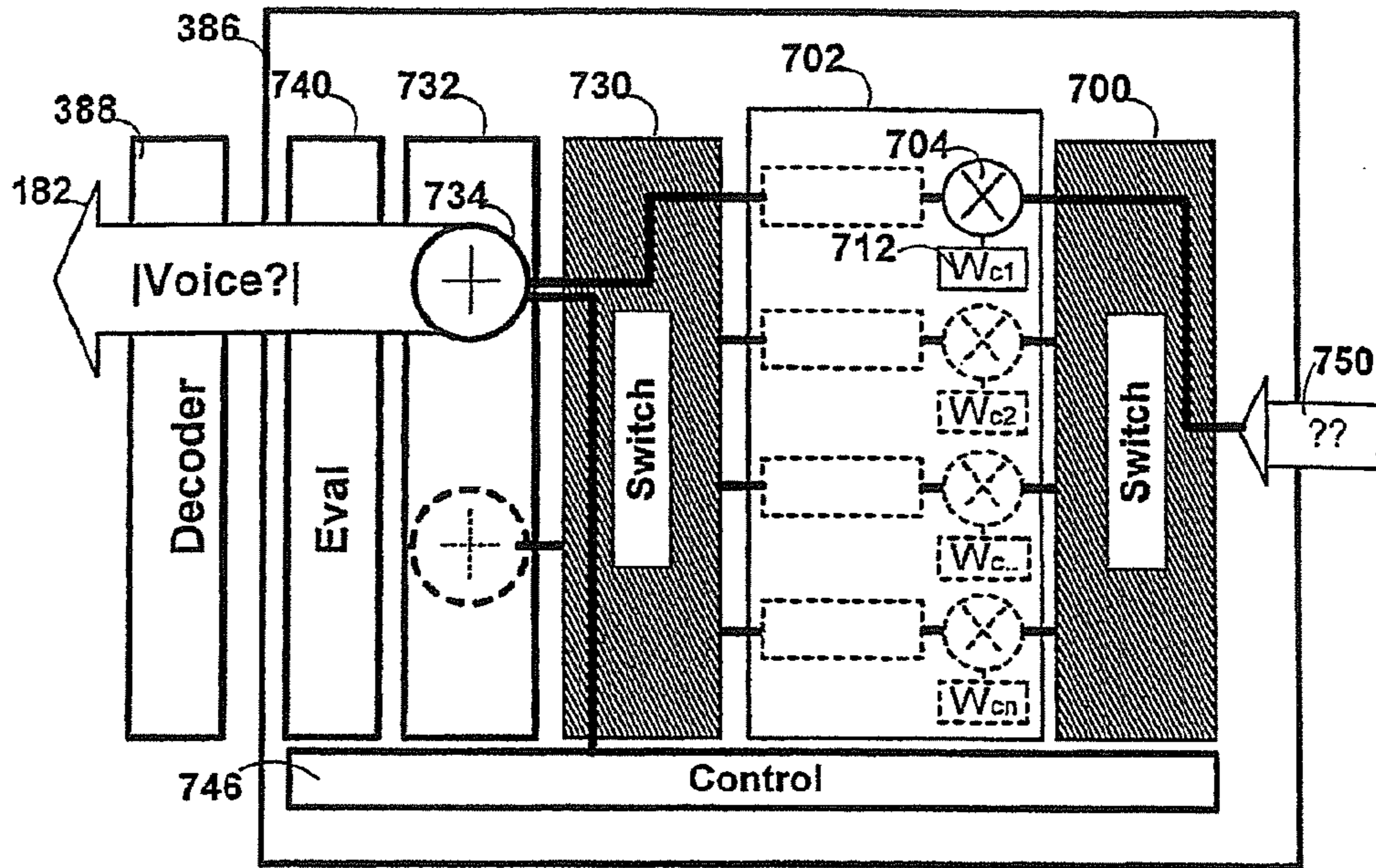
Spatial Processor
