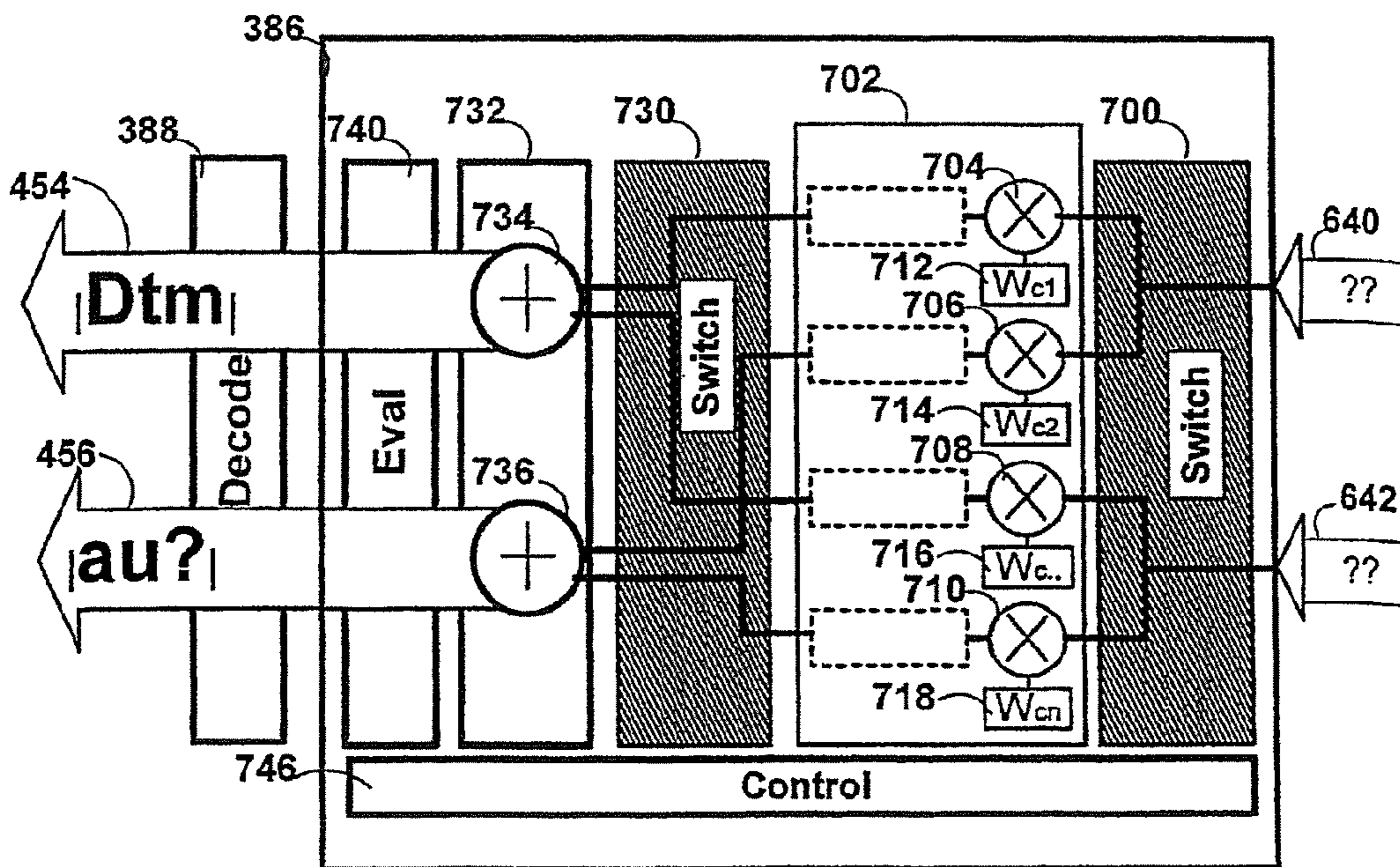
Spatial Processor
