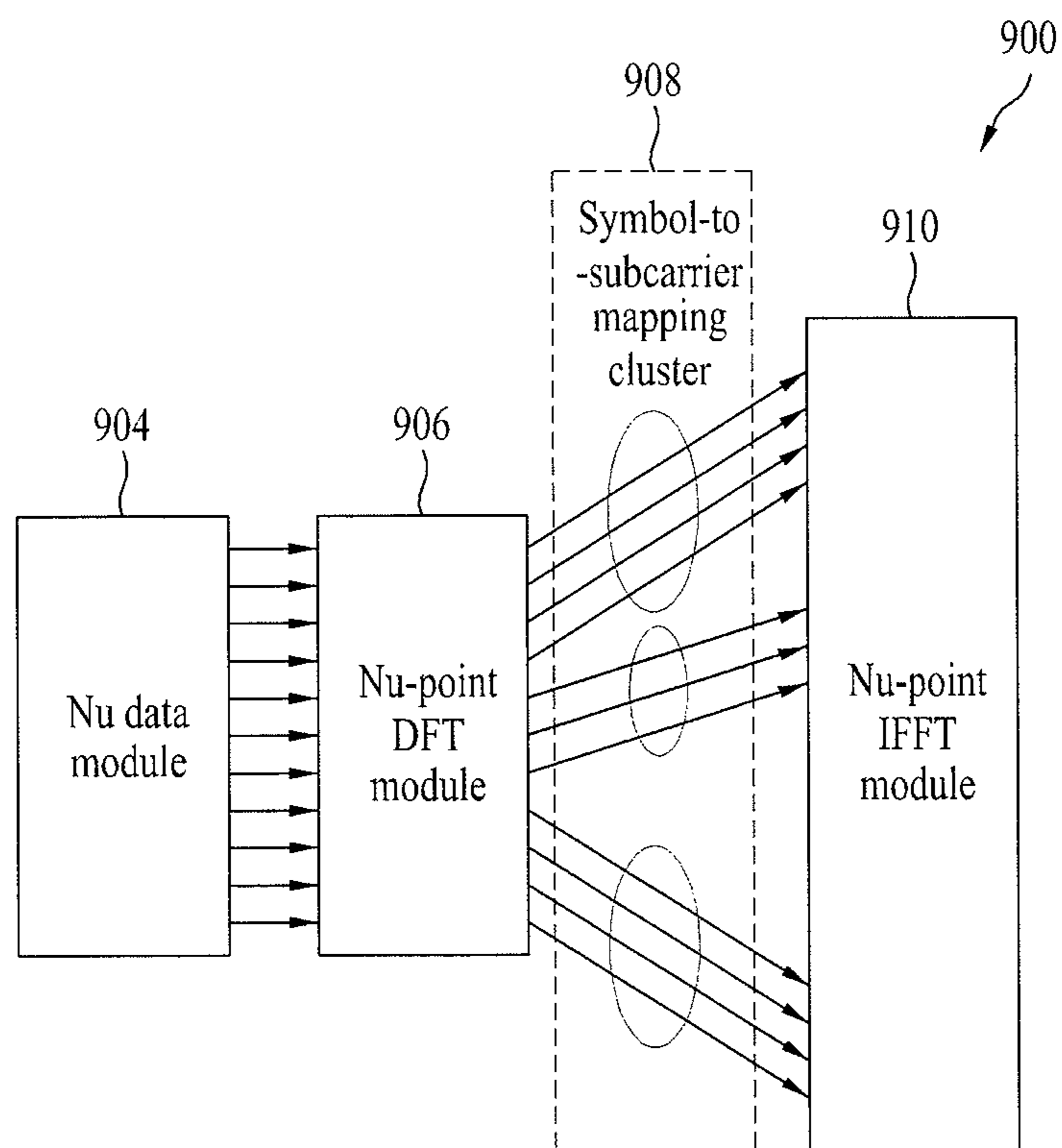
Clusters DFT-s-OFDMA
