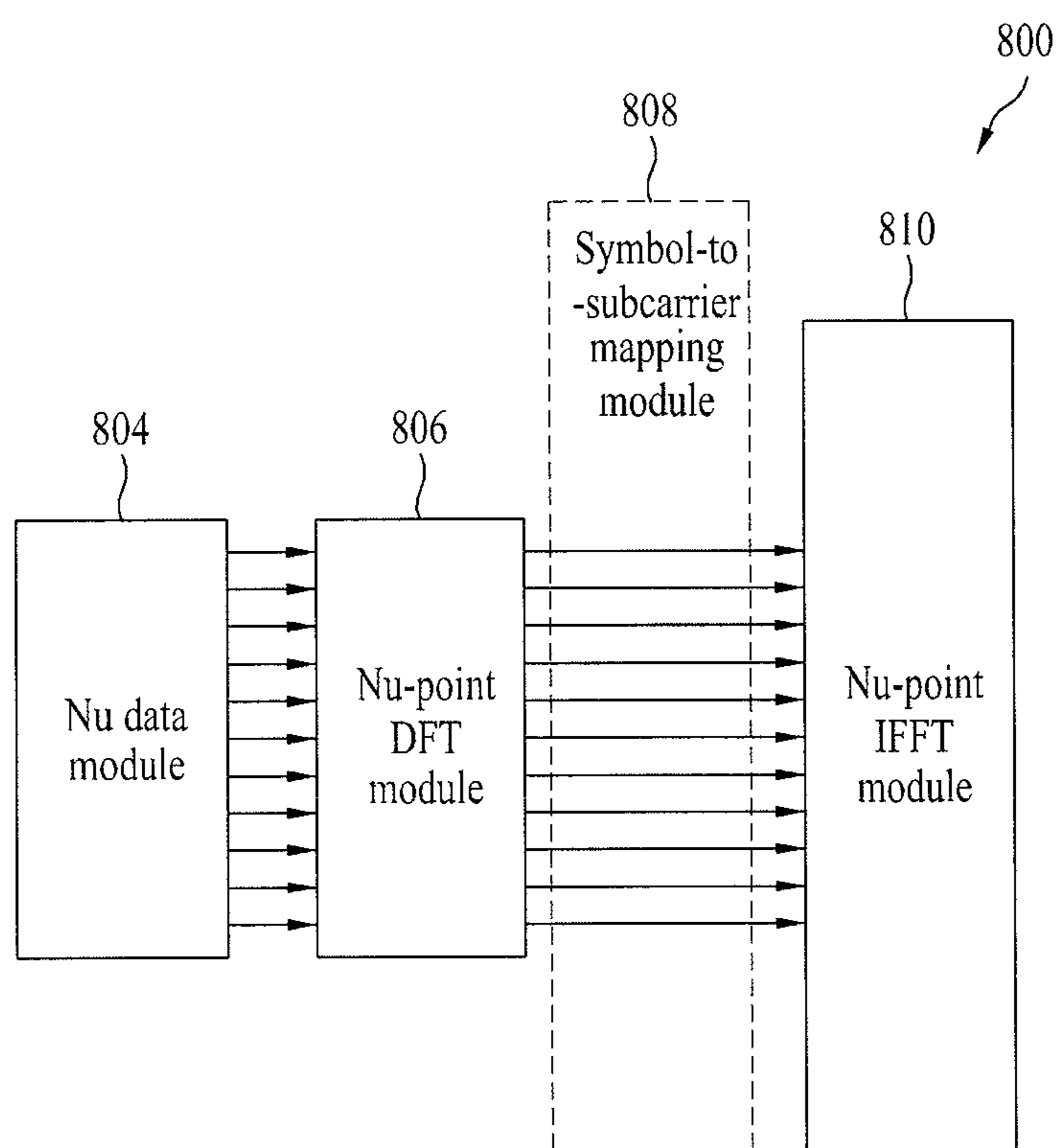
Localized DFT-s-OFDMA
