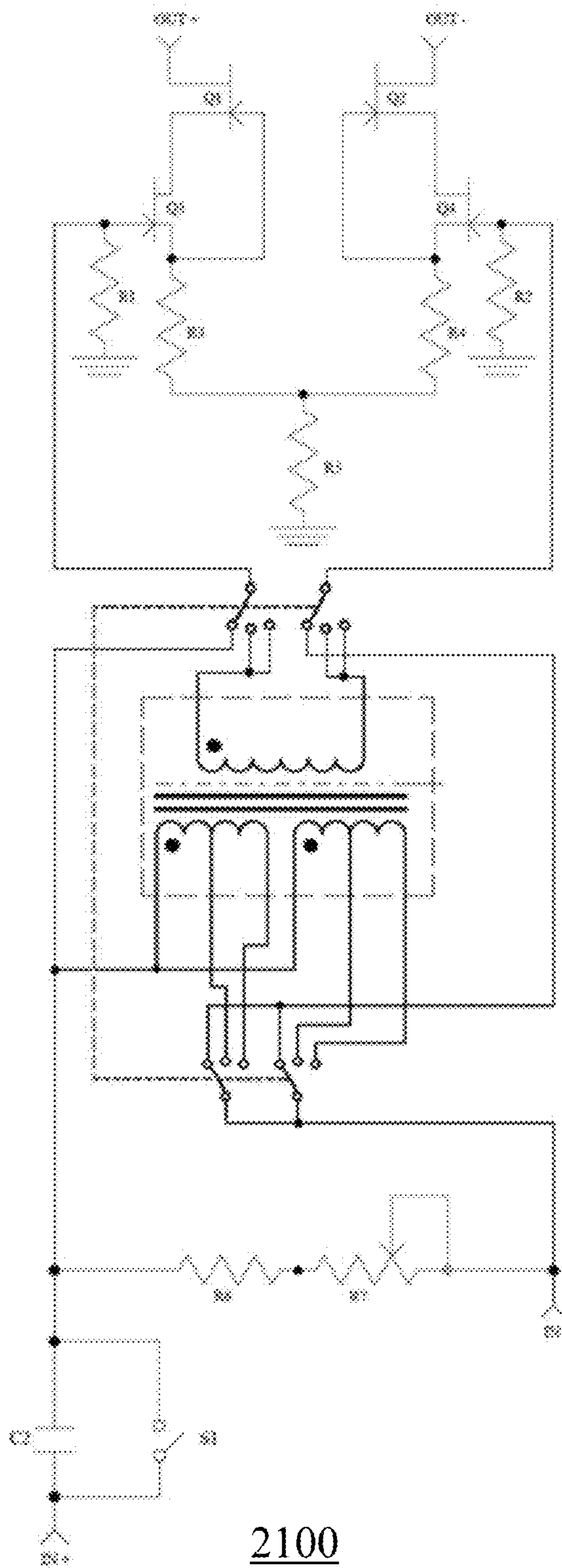
Preamp Circuit with XFMR and high-pass filter
