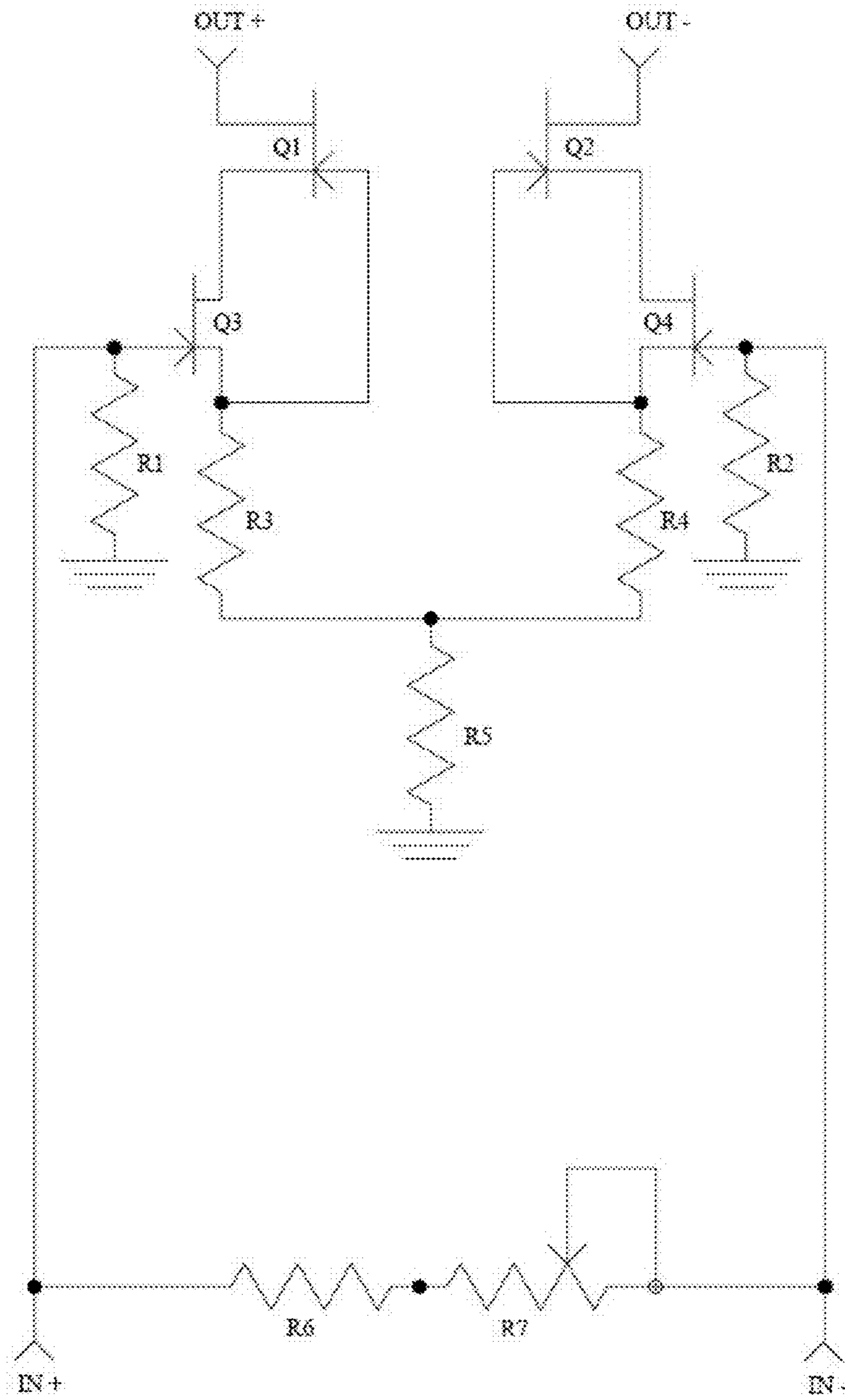
Preamp Circuit without high-pass filter
