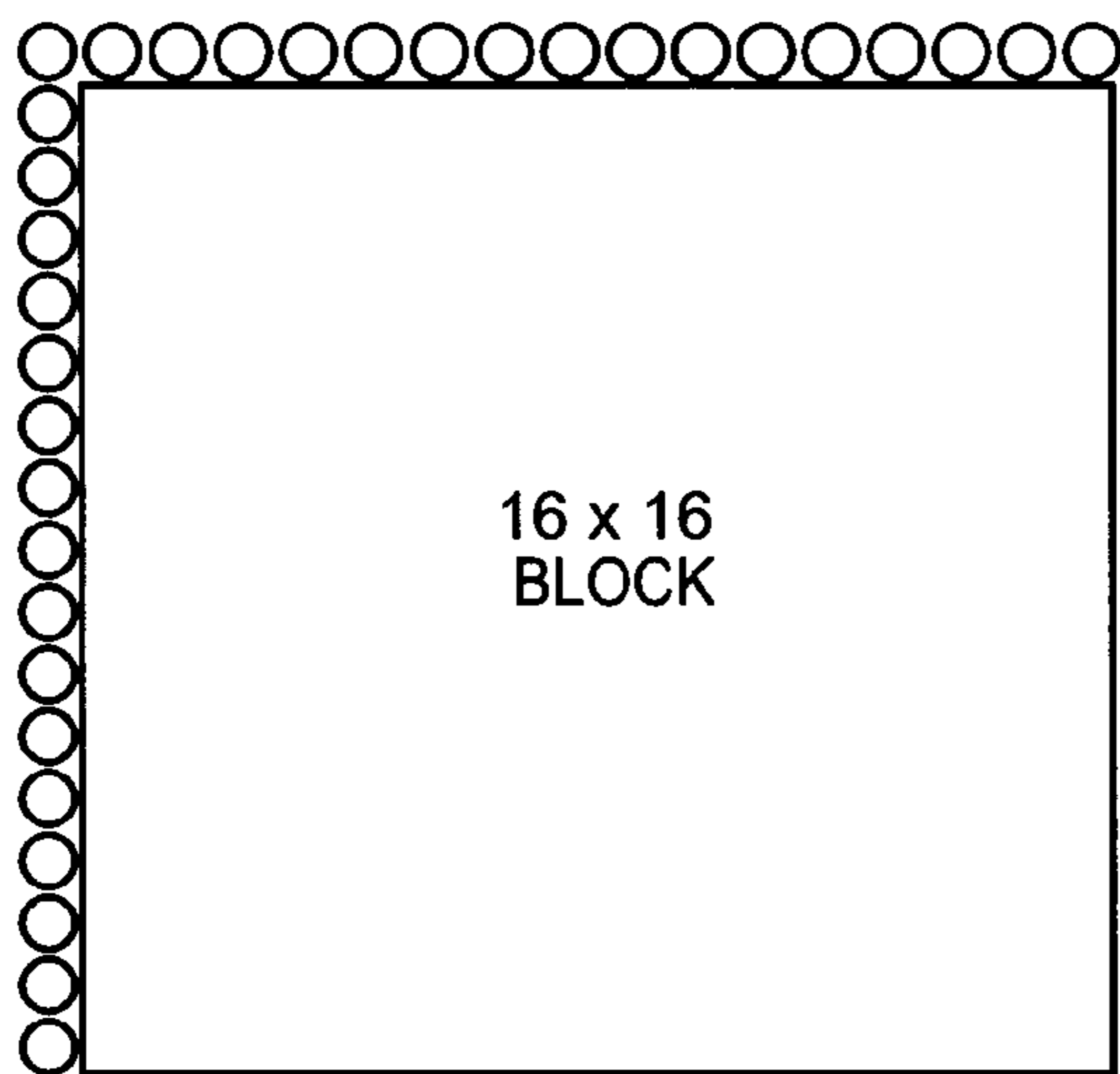
Intra_16 x 16
