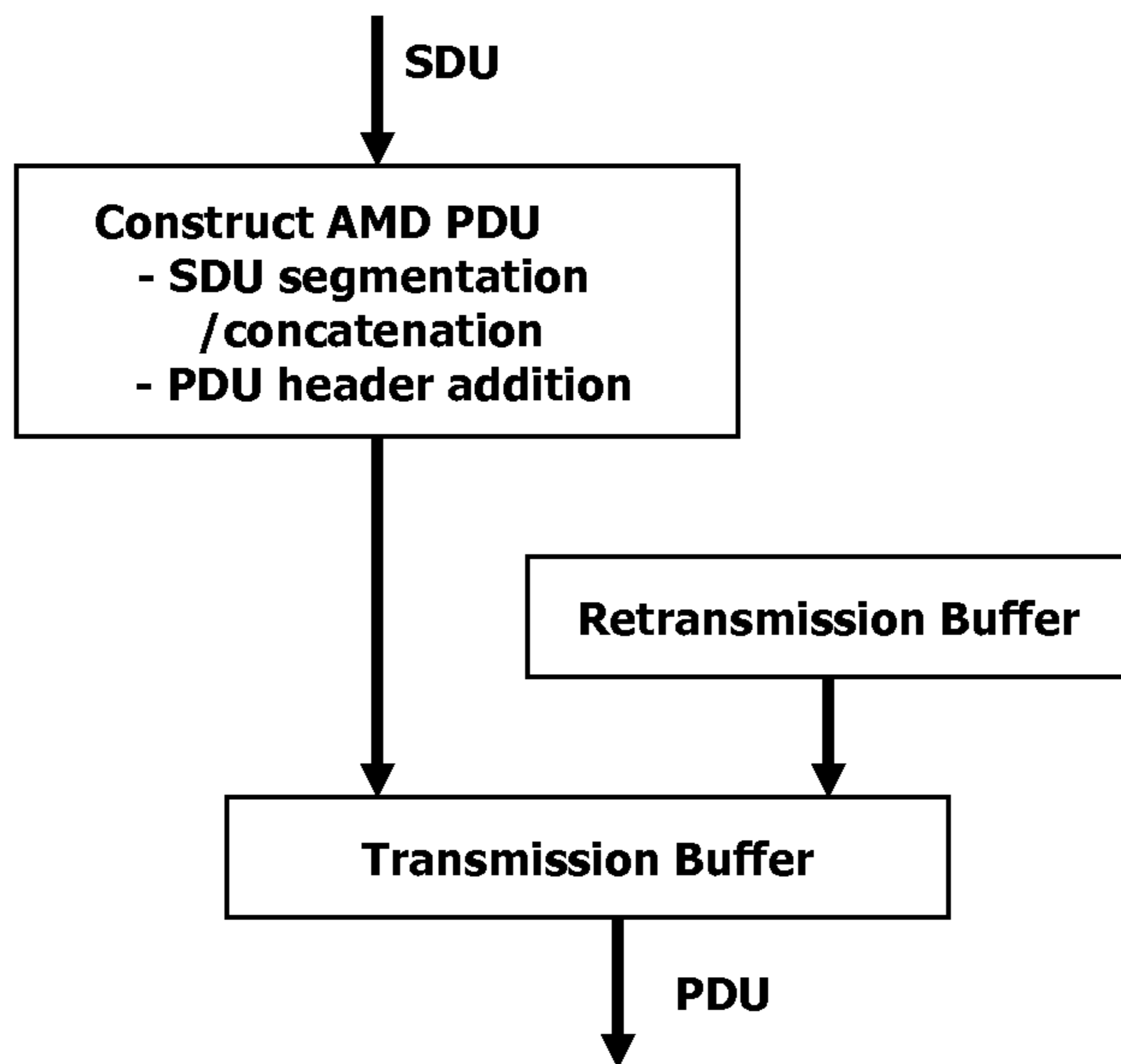
FIG.5 BACKGROUND ART
