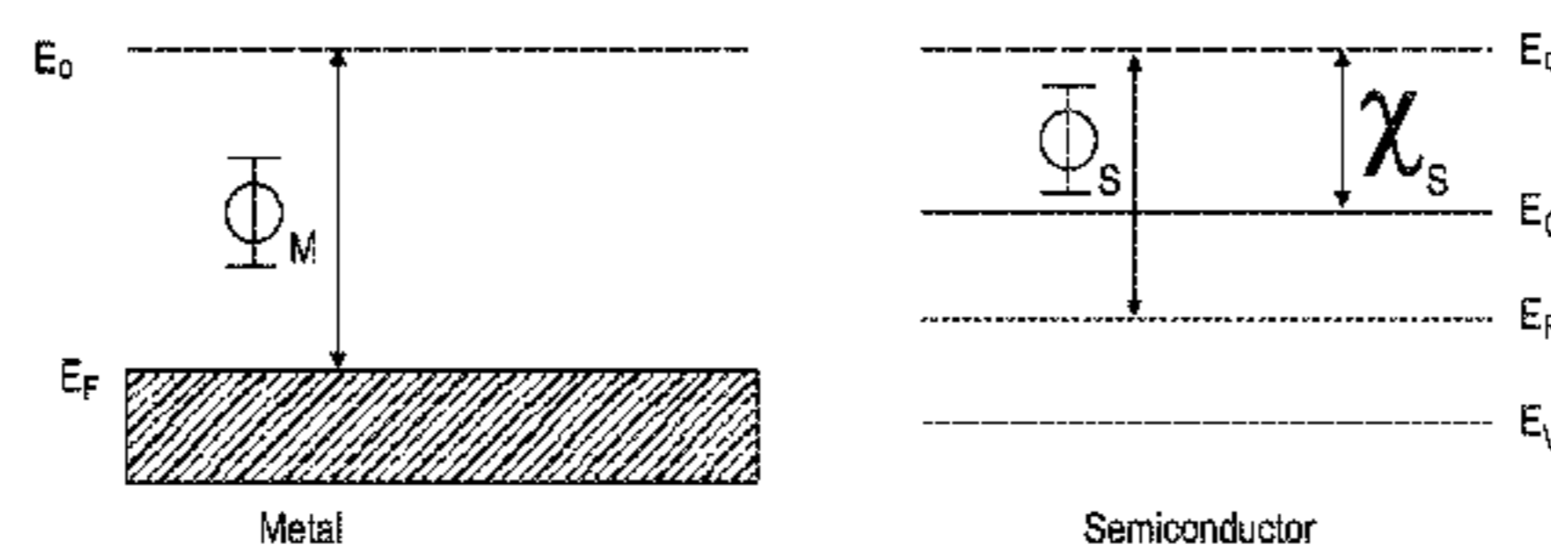
Energy Scales for Metal - Semiconductor Junctions
