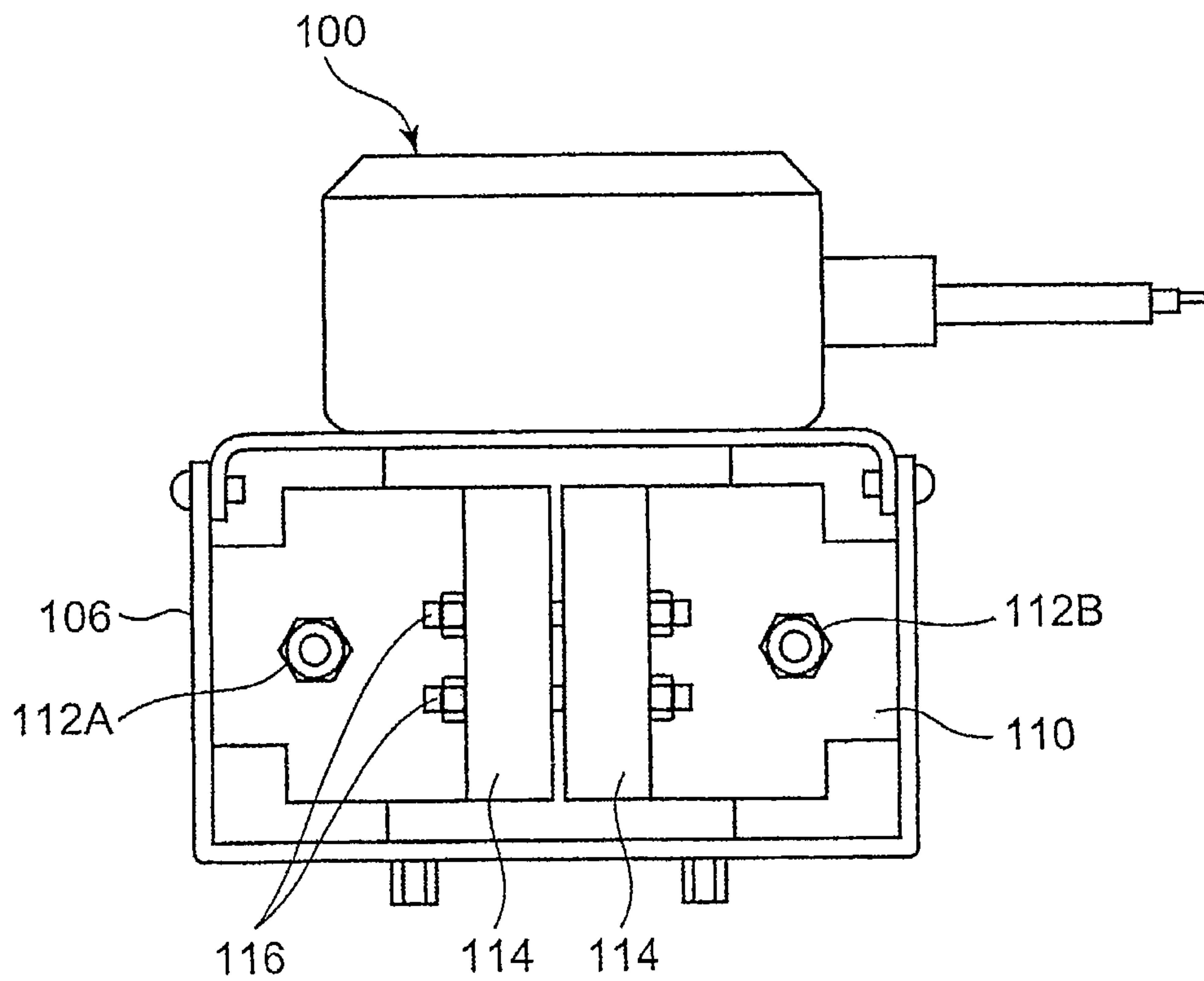
Fig. 9 PRIOR ART
