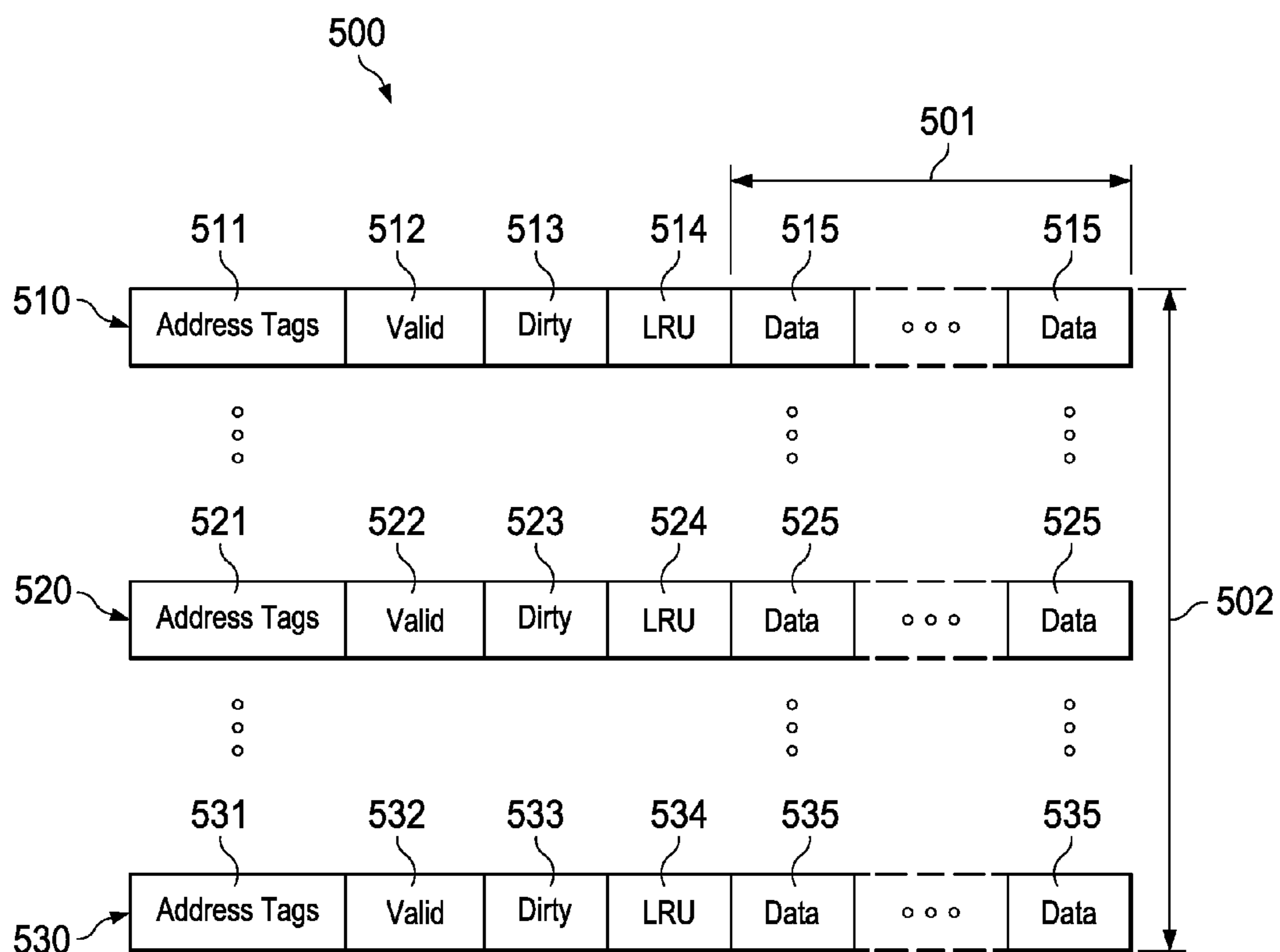
FIG. 5 (PRIOR ART)
