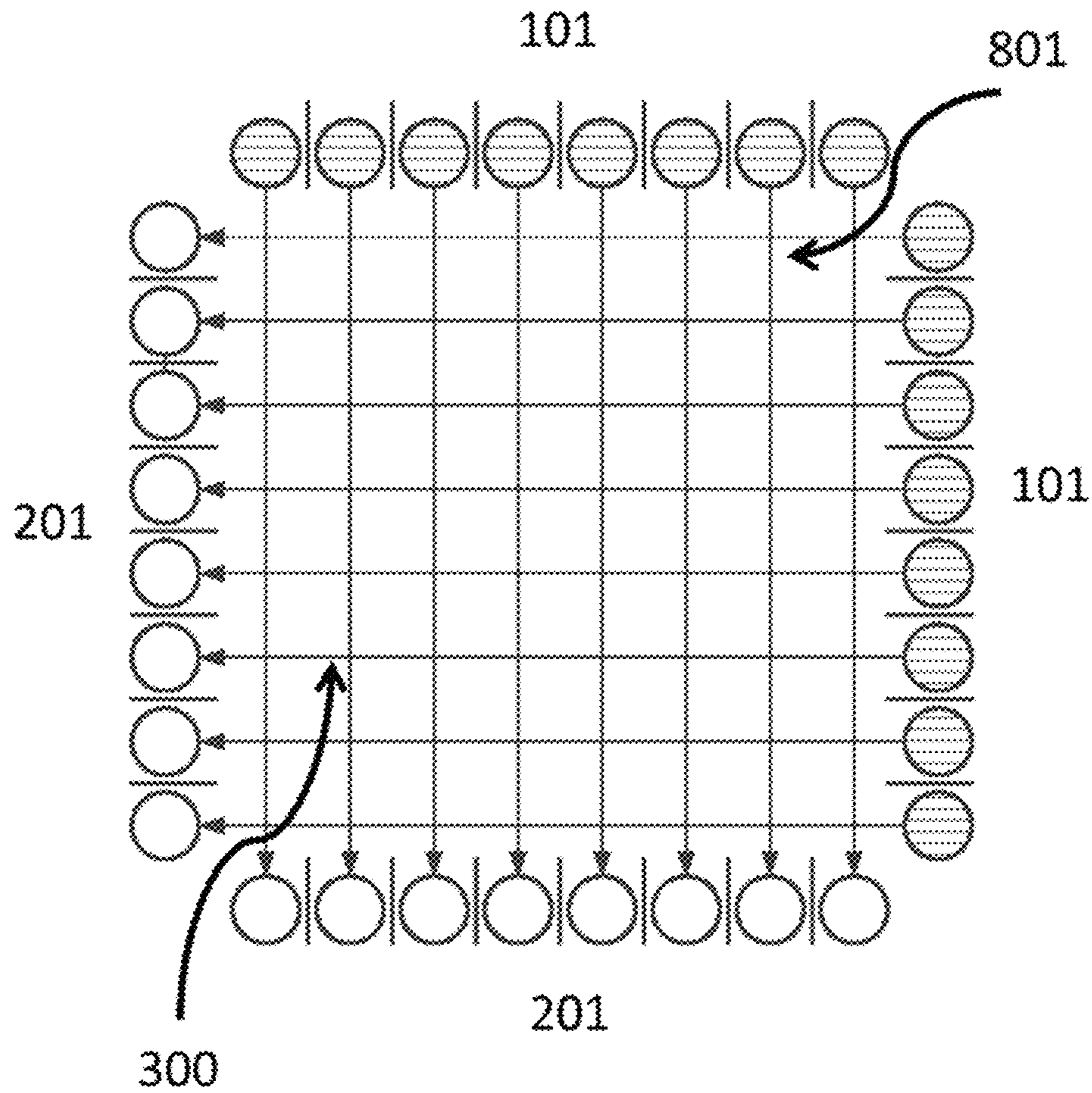
FIG. 1 (PRIOR ART)
