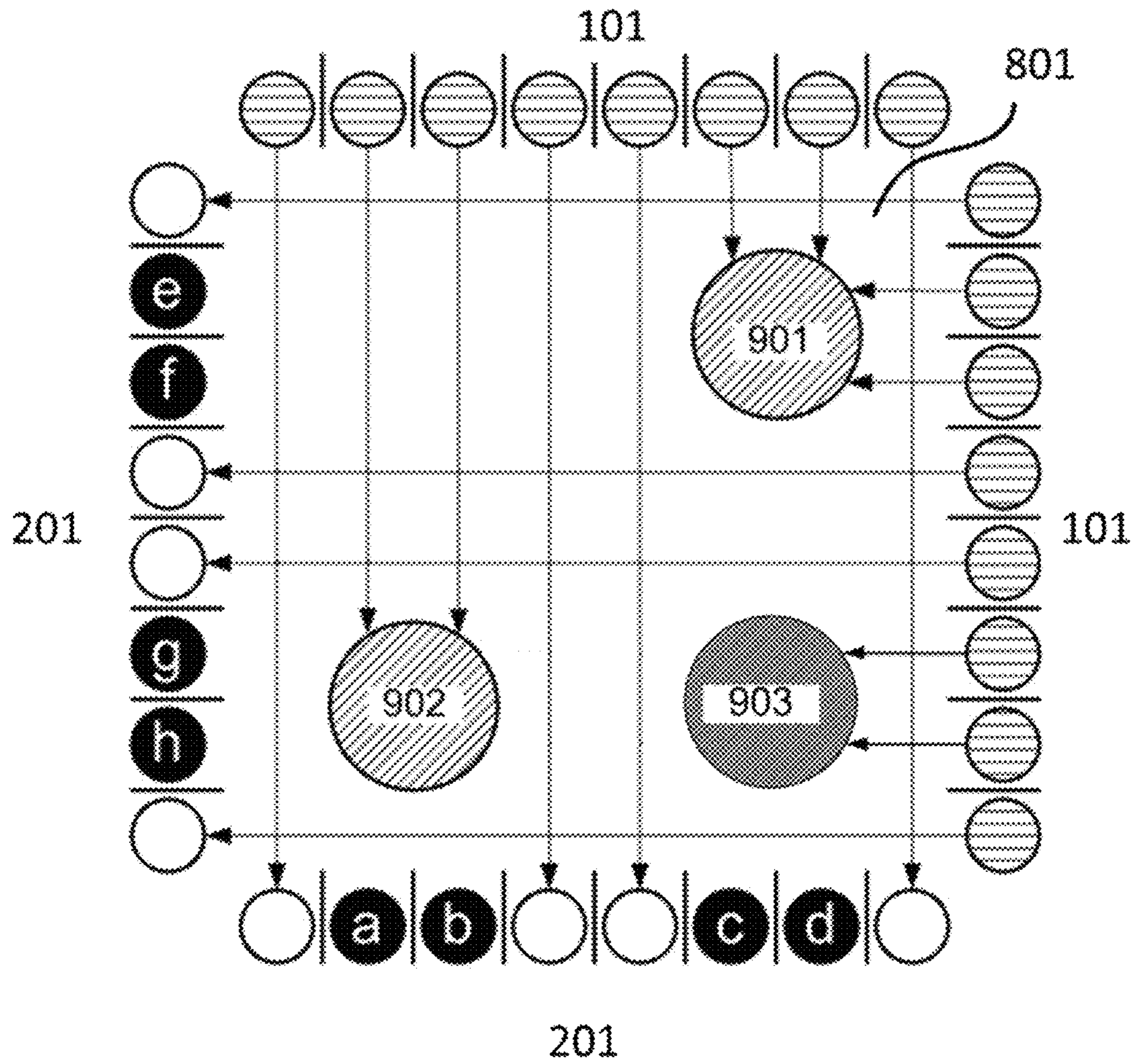
FIG. 4 (PRIOR ART)
