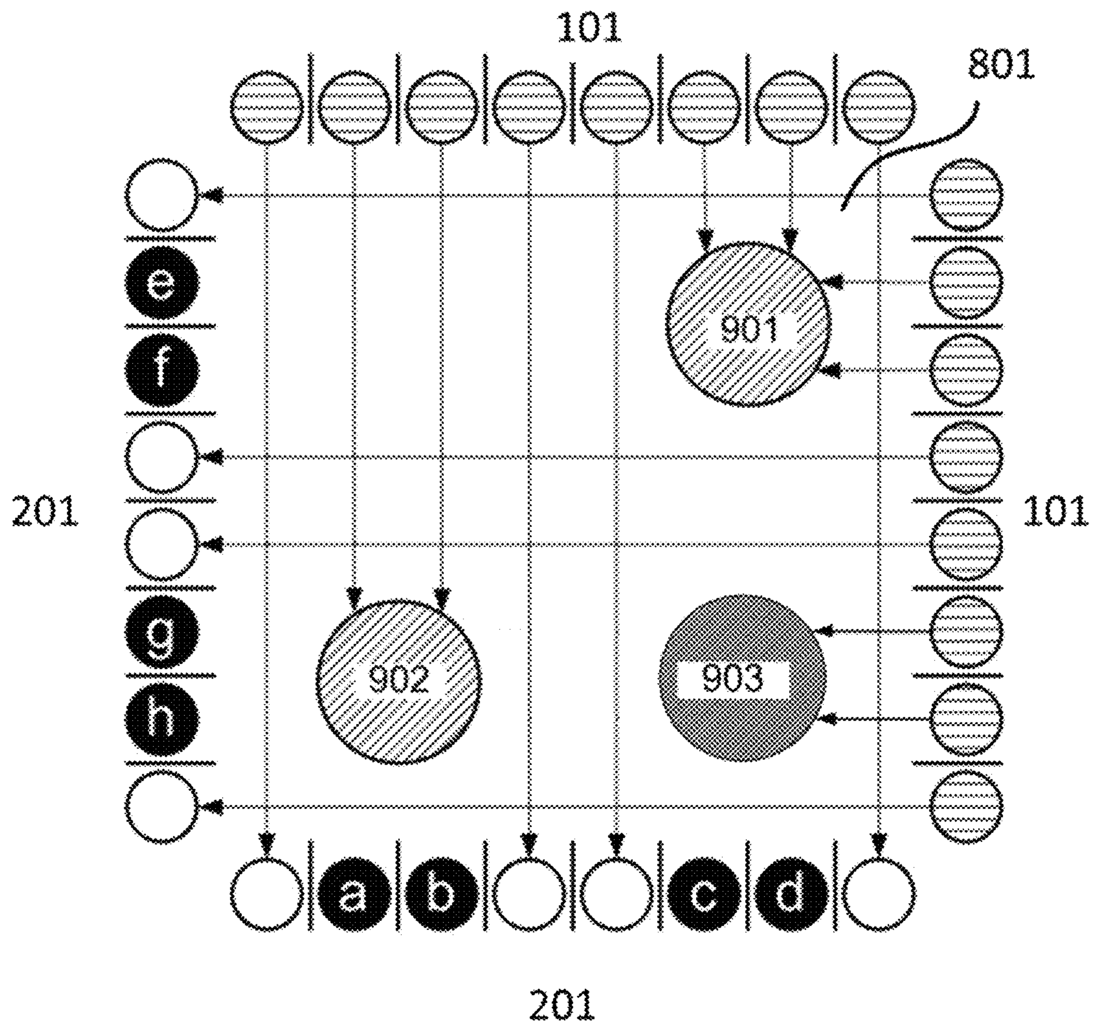
FIG. 4 (PRIOR ART)
