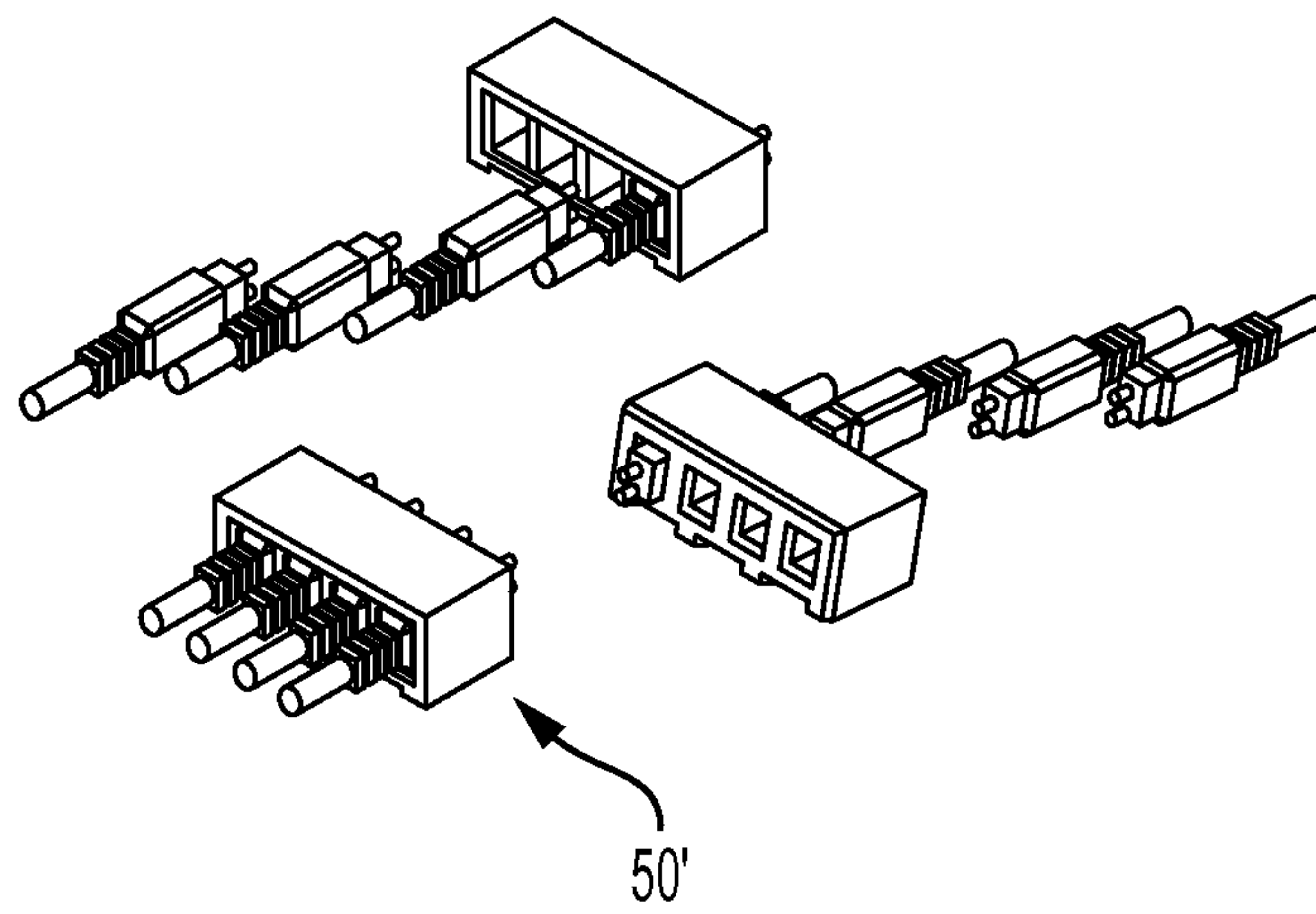
FIG. 4 PRIOR ART
