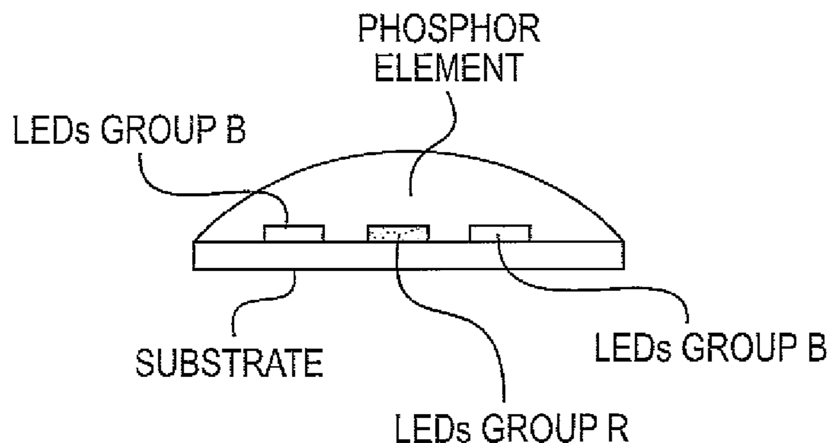
BLUE AND RED LEDs UNDER A COMMON PHOSPHOR ELEMENT
