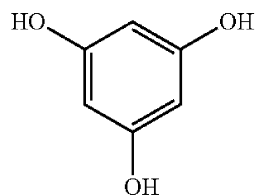
1,3,5-Trihydroxyl-benzene
