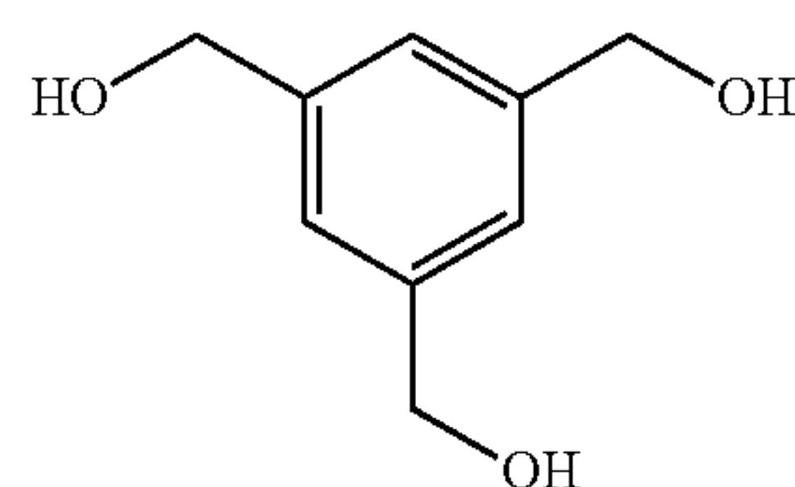
1,3,5-Tri(hydroxymethyl)benzene
