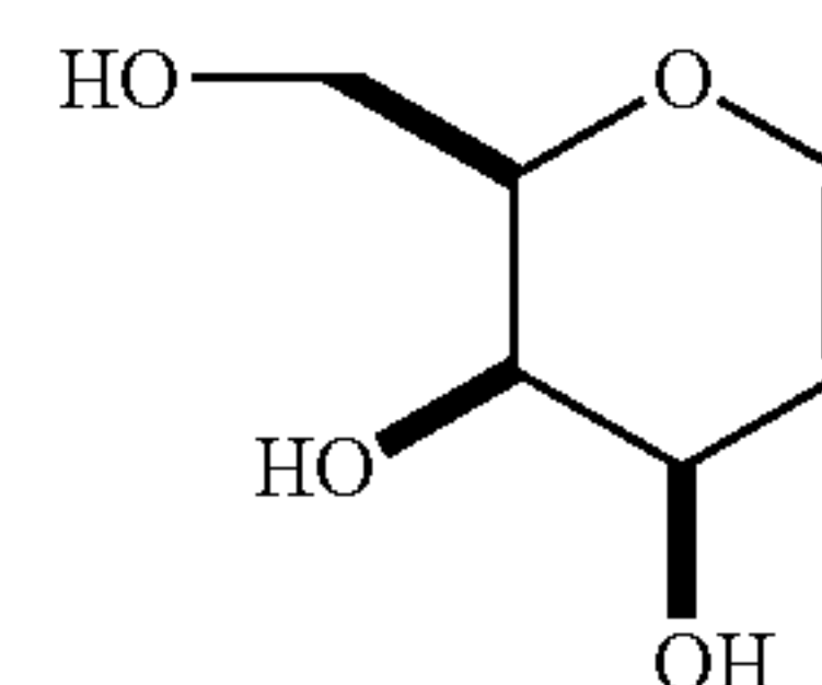
D-Galactool
