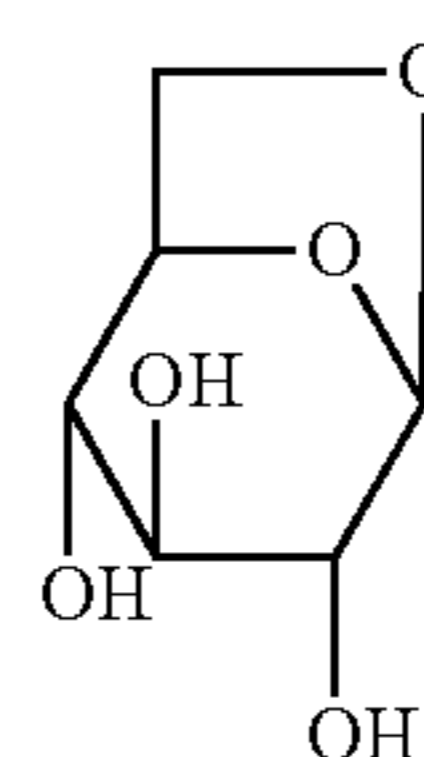
1,6-anhydro- \beta -D-Glucose
