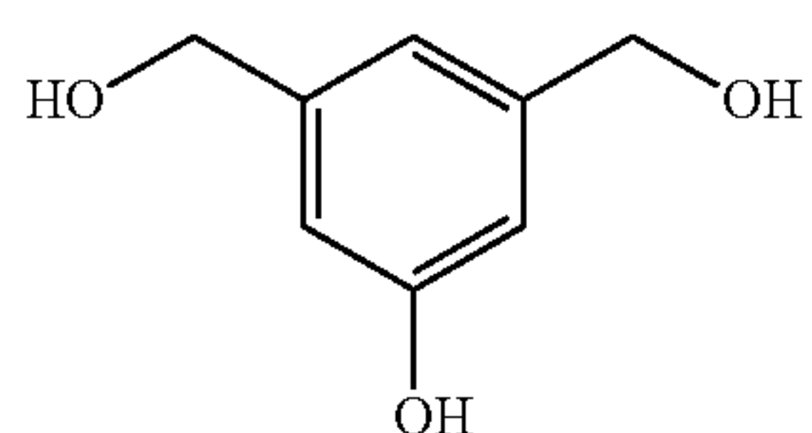
3,5-Di(hydroxymethyl)phenol
