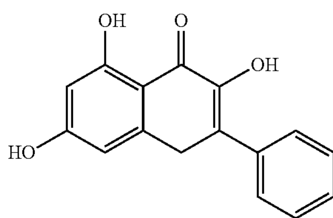
3,5,7-Trihydroxyflavone
