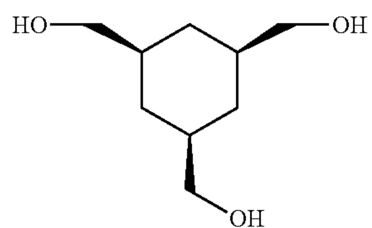
cis-1,3,5-Tri(hydroxymethyl)cyclohexane
