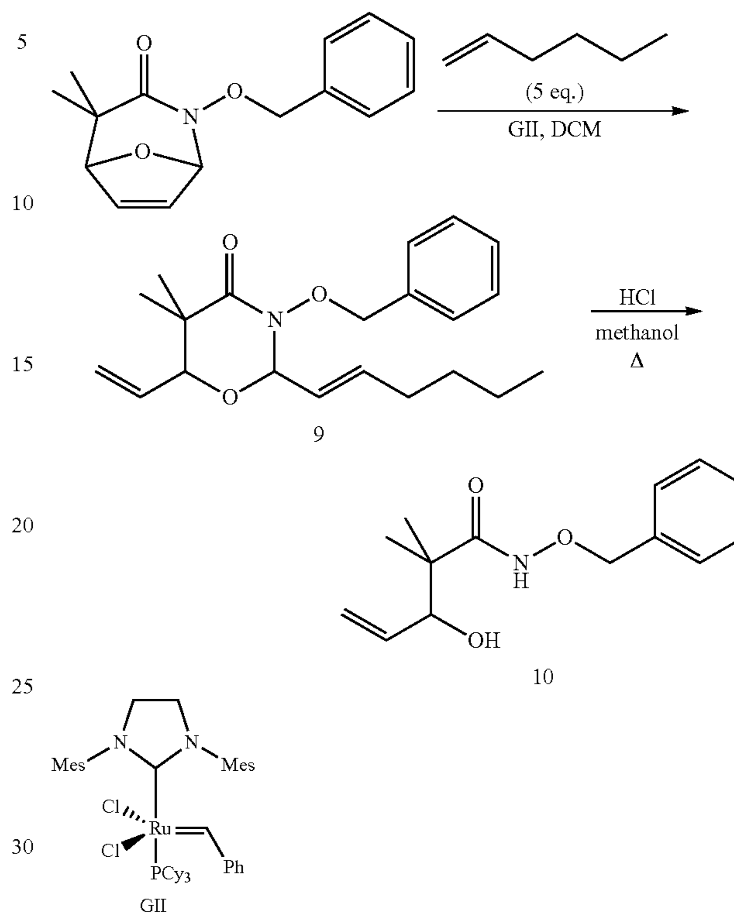
Scheme 5: 3-benzyloxy-5,5-dimethyl-2-(1'-pentenyl)-6-vinyl-1,3-oxazin-4-one, 9.
