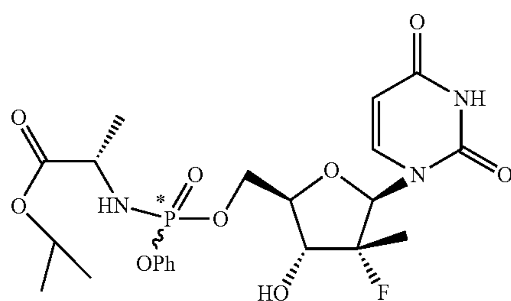
5'-O-phosphoramidate (2 diastereomers)
