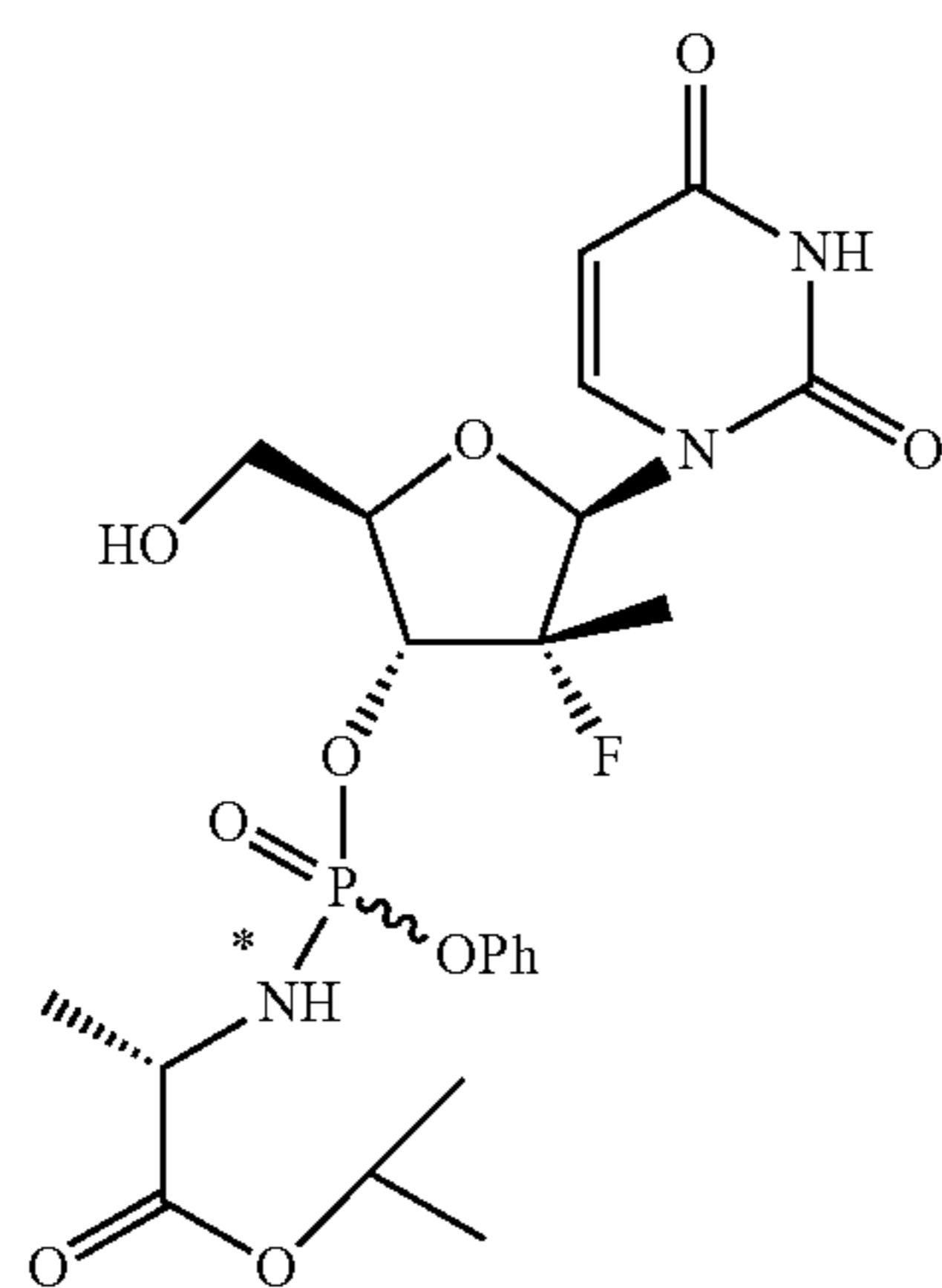
3'-O-phosphoramidate (2 diastereomers)
