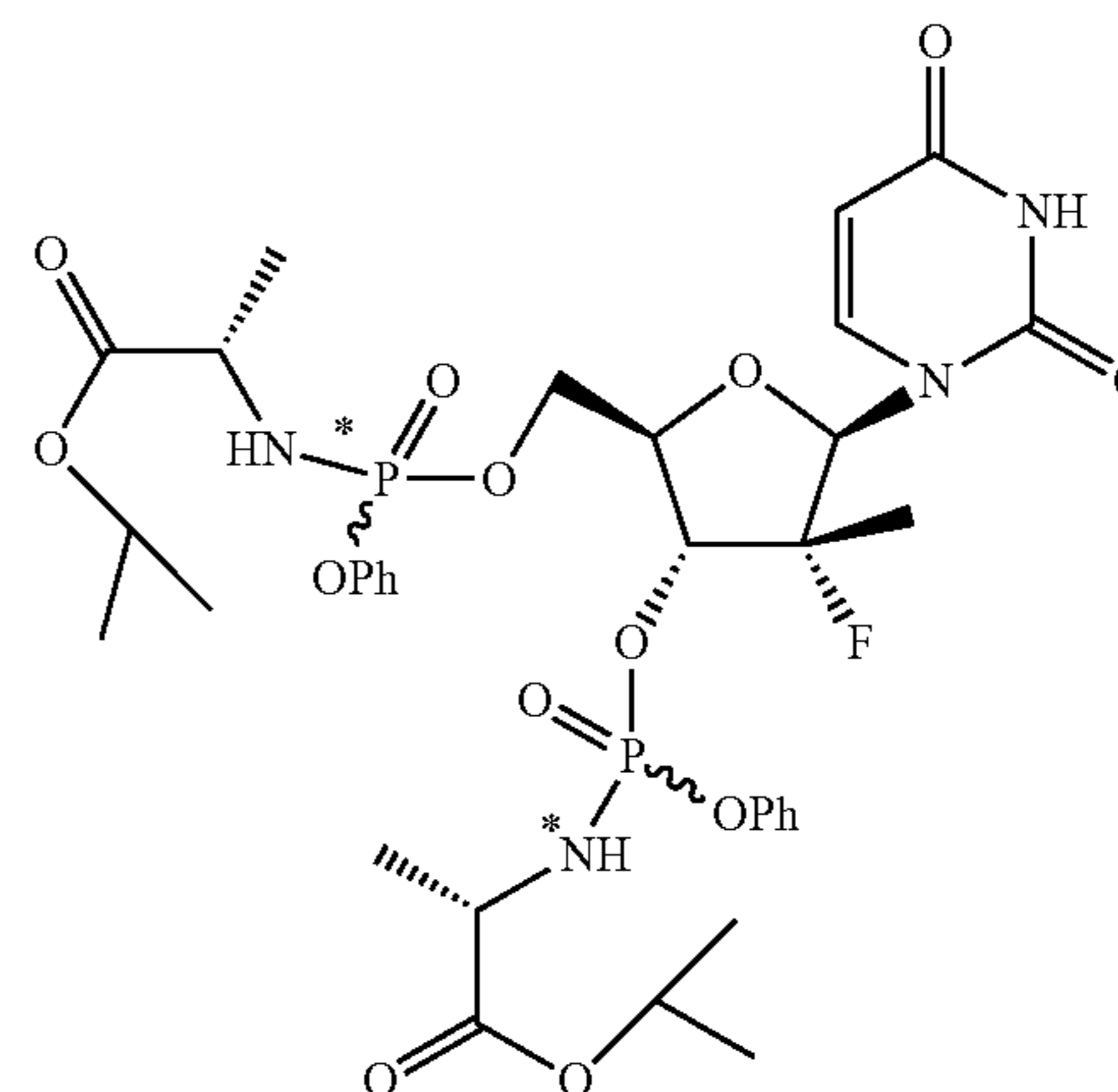
3', 5'-bis-O-phosphoramidate (4 diastereomers)
