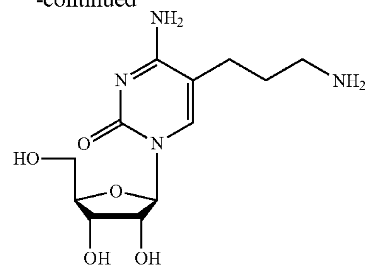
4 MW = 300.31 5-(3-aminopropyl)cytidine
