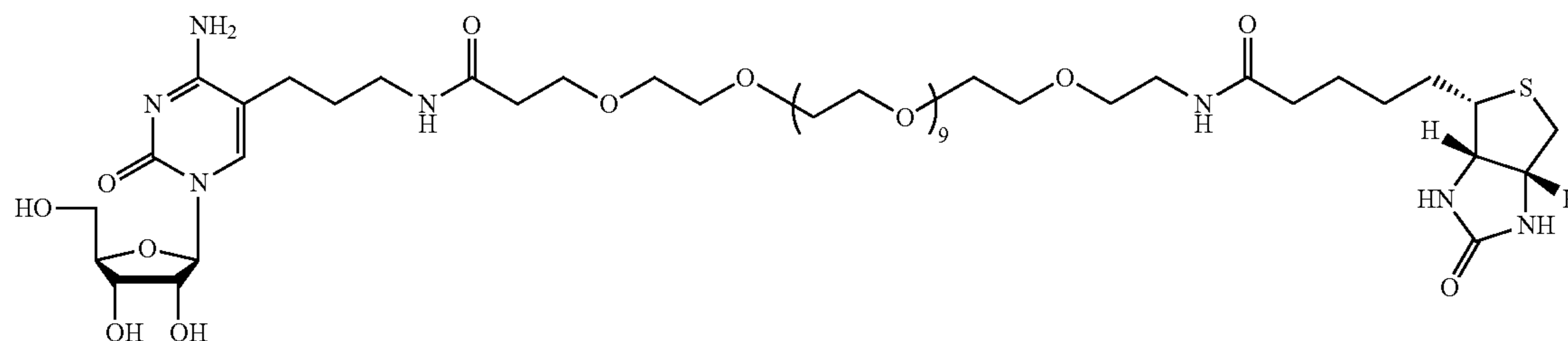
7 MW = 1126.31 Biotin-PEG 12 -Alkane-Cytidine (BP 12 AC)
