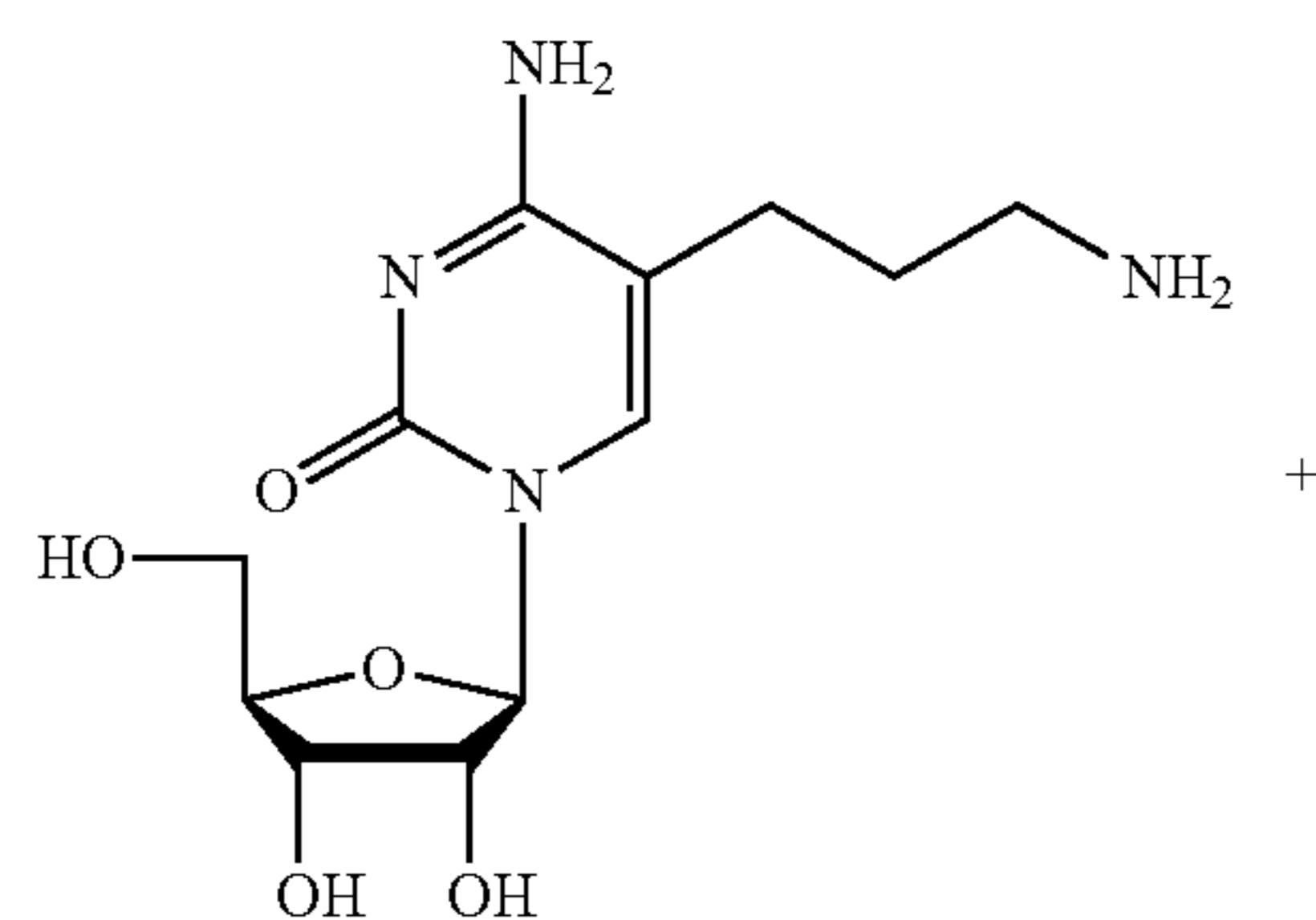
4 MW = 300.31 5-(3-aminopropyl)cytidine
