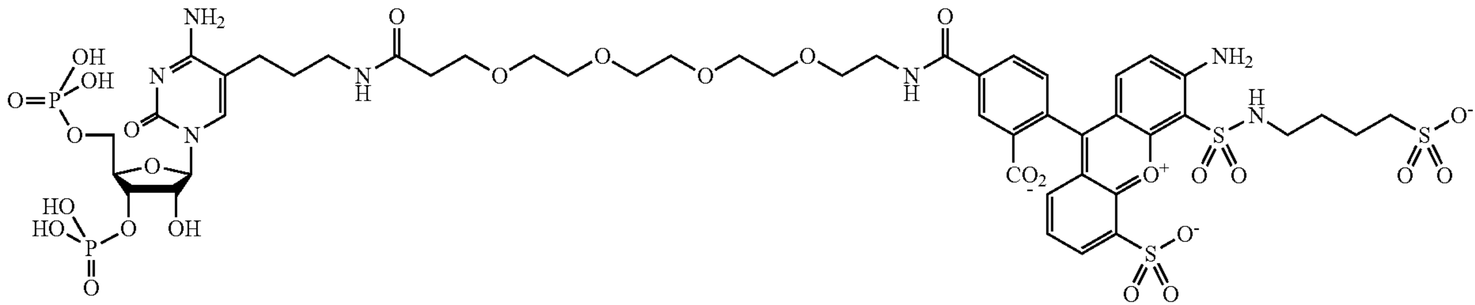
DyLight488-PEG 4 -Alkane-3',5'-Bisphosphate-Cytidine (Dy488P 4 A-3',5'-pCp)
