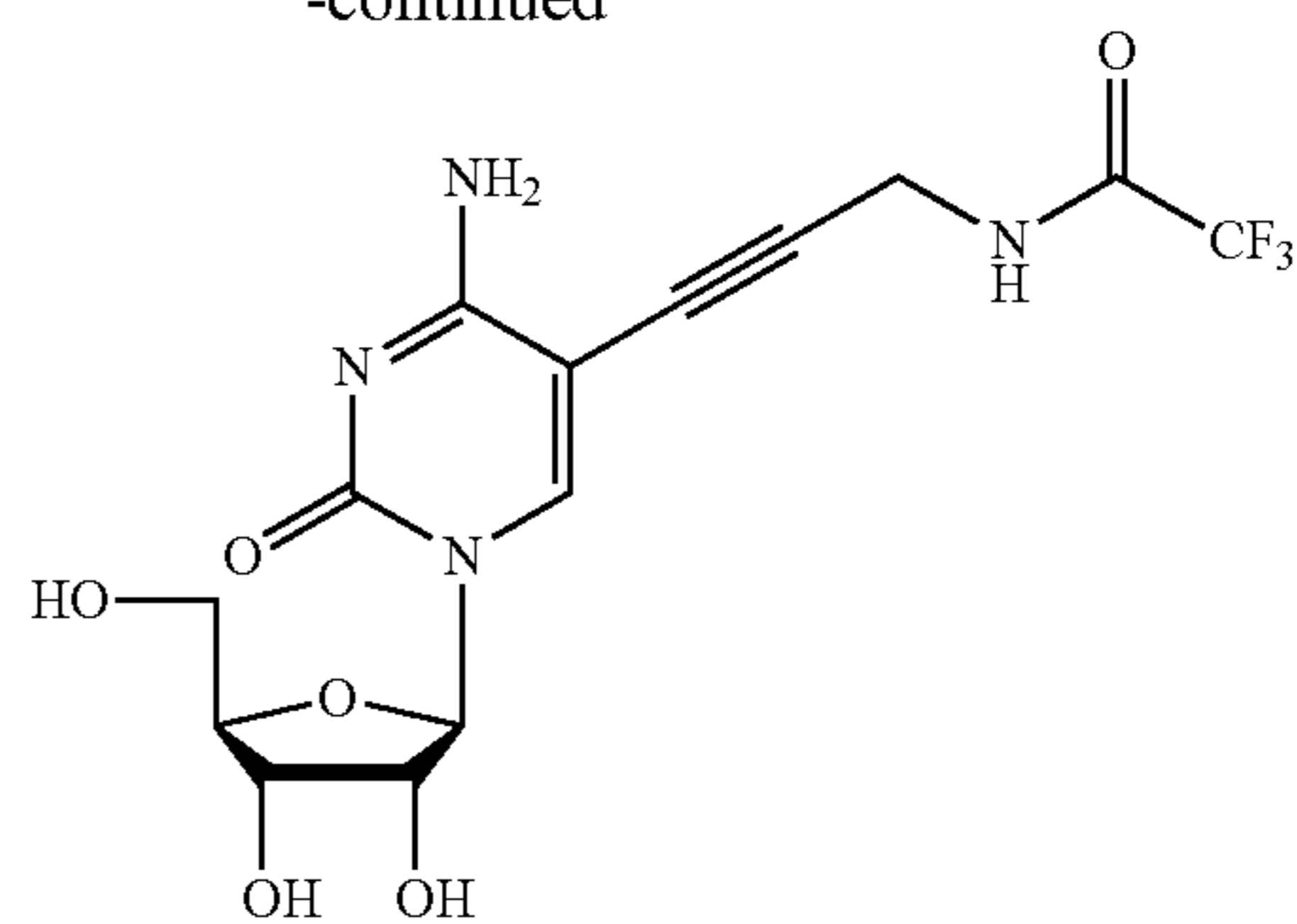
2 MW = 392.29 5-[3-(trifluoroacetamido)propynyl]cytidine
