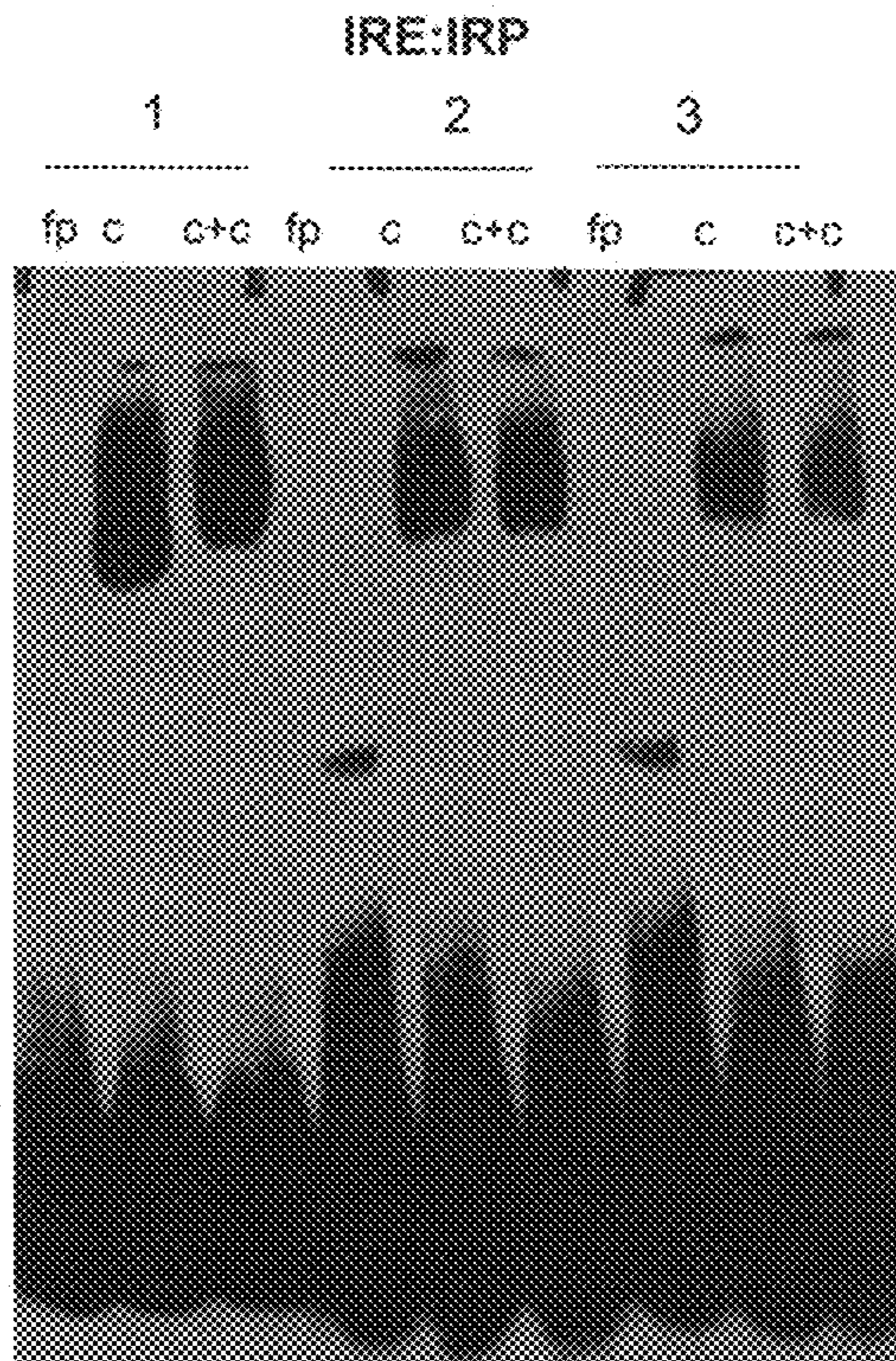
3',5'-Bisphosphorylated Cytidine-Alkene-LC-Biotin
