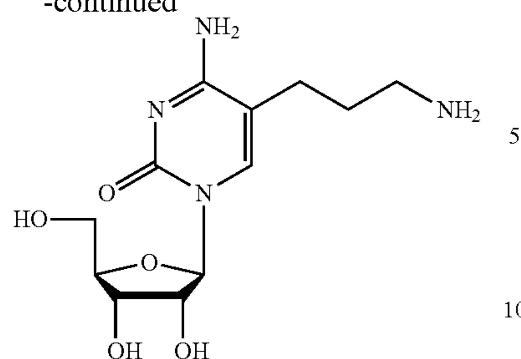
4 MW = 300.31 5-(3-aminopropyl)cytidine
