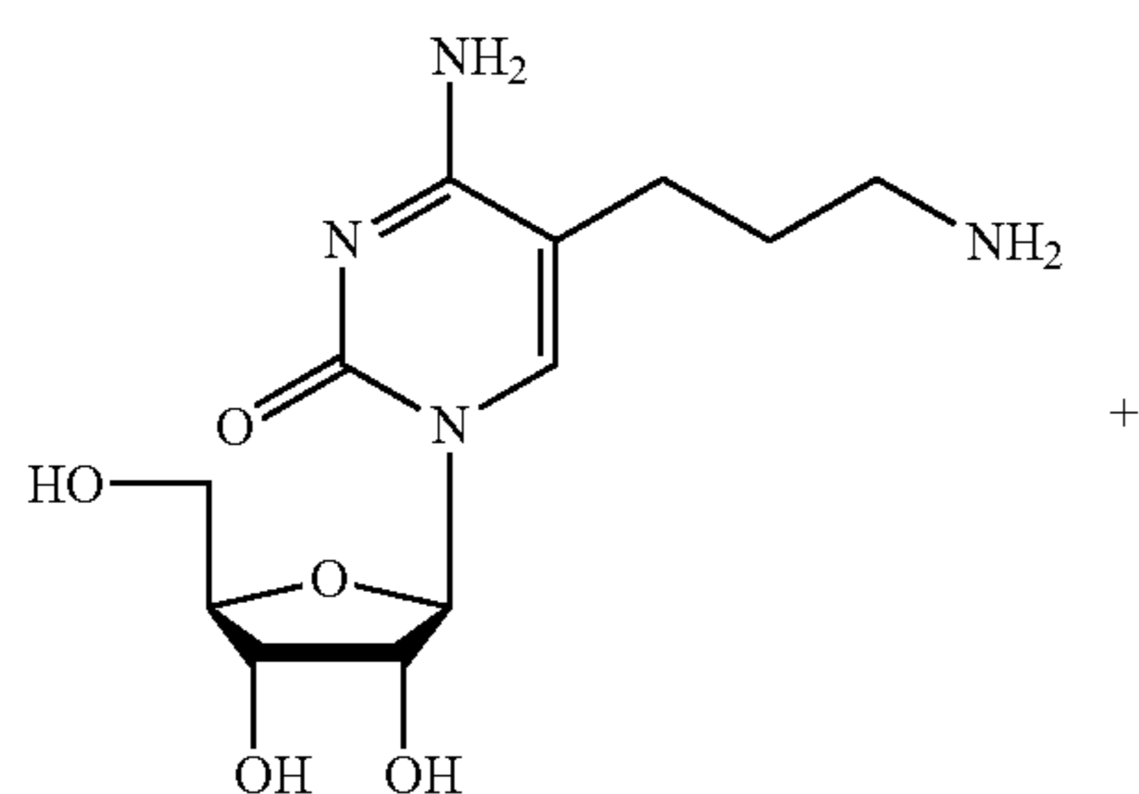
4 MW = 300.31 5-(3-aminopropyl)cytidine
