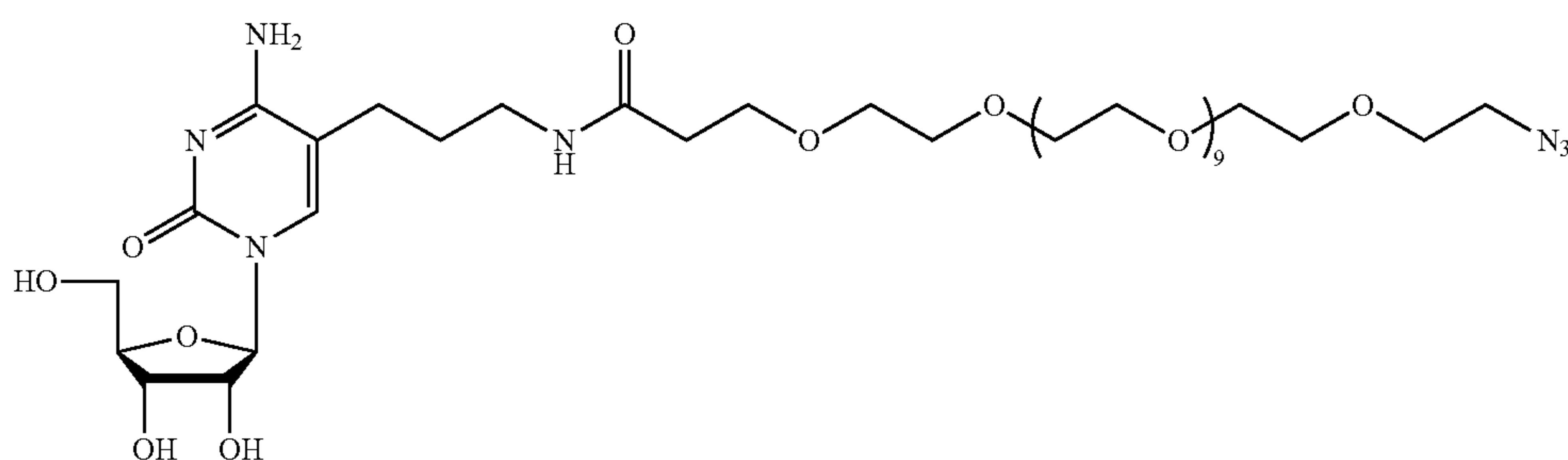
18 MW = 926.02 Azido-PEG 12 -Alkane-Cytidine (AzP 12 AC)
