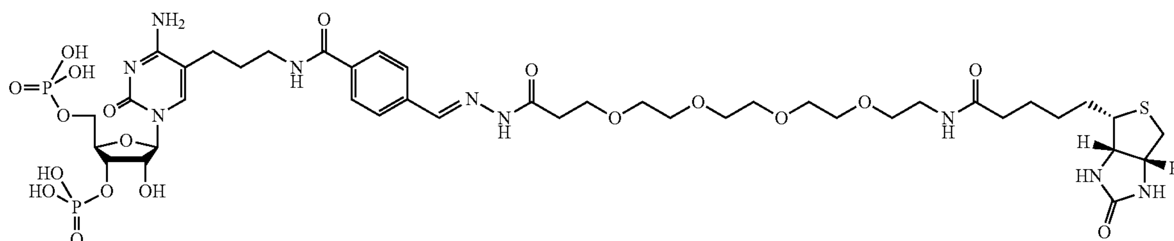
Hydrazone Exchange Cleavable Biotin-PEG 4 -Hydrazone-Alkane-3',5'-Bisphosphate-Cytidine (BP 4 HA-3',5'-pCp)
