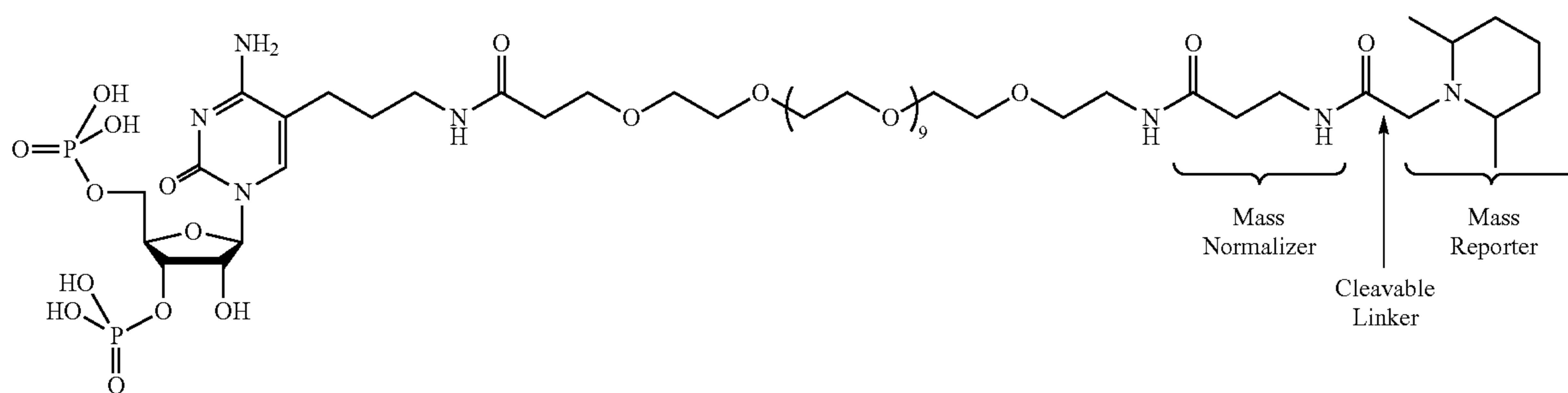
TMT-PEG 12 -Alkane-3',5'-Bisphosphate-Cytidine (TMTP 12 A-3',5'-pCp)
