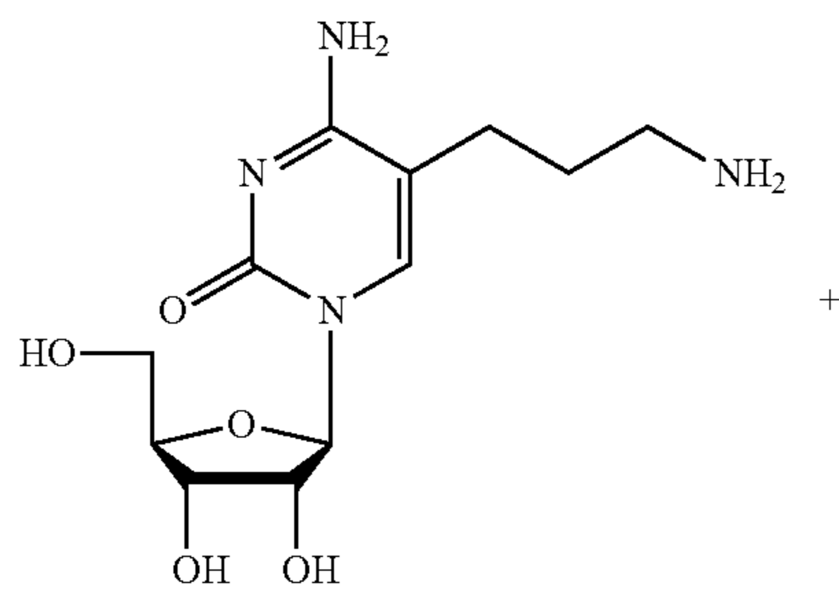
4 MW = 300.31 5-(3-aminopropyl)cytidine
