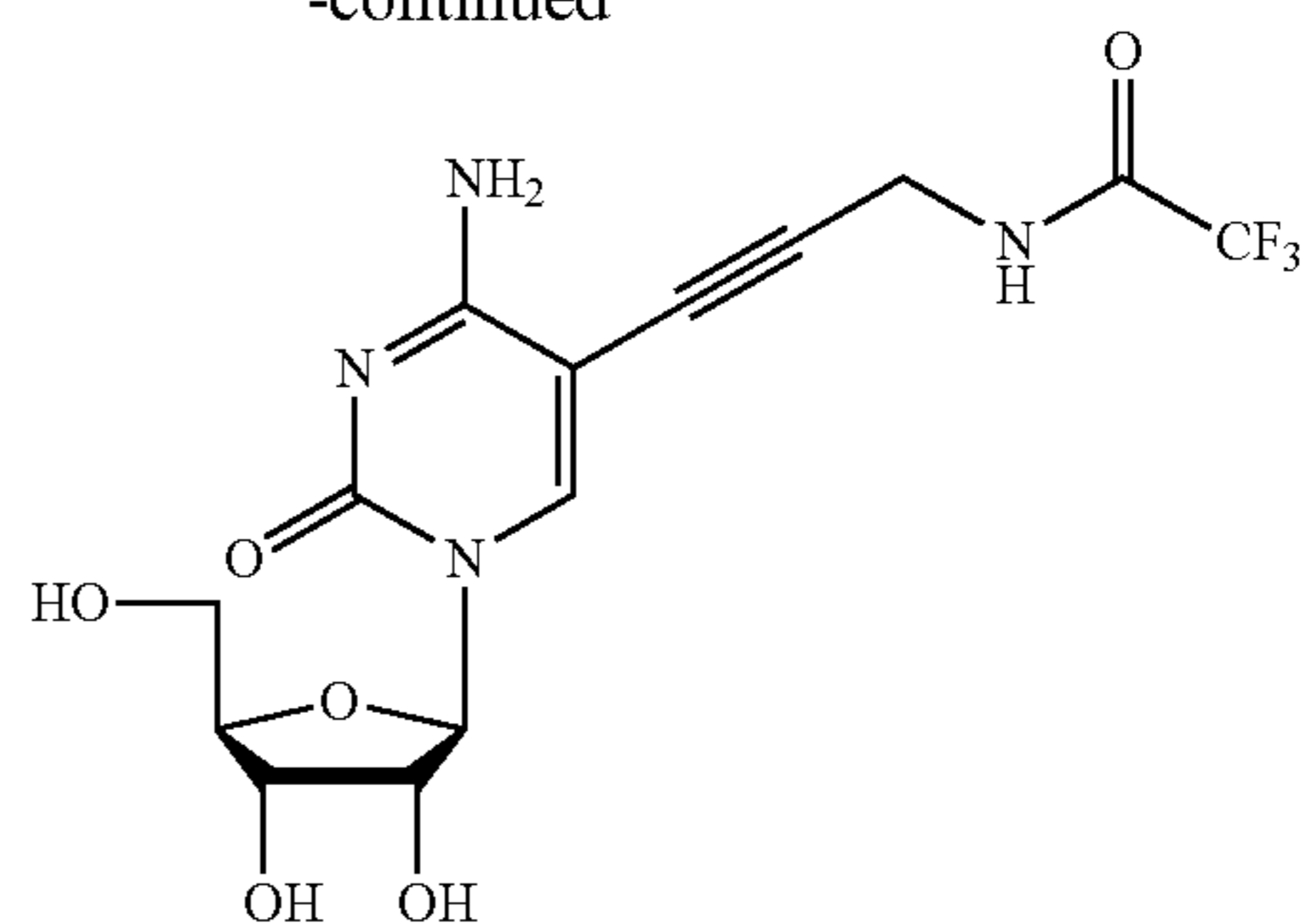
2 MW = 392.29 5-[3-(trifluoroacetamido)propynyl]cytidine
