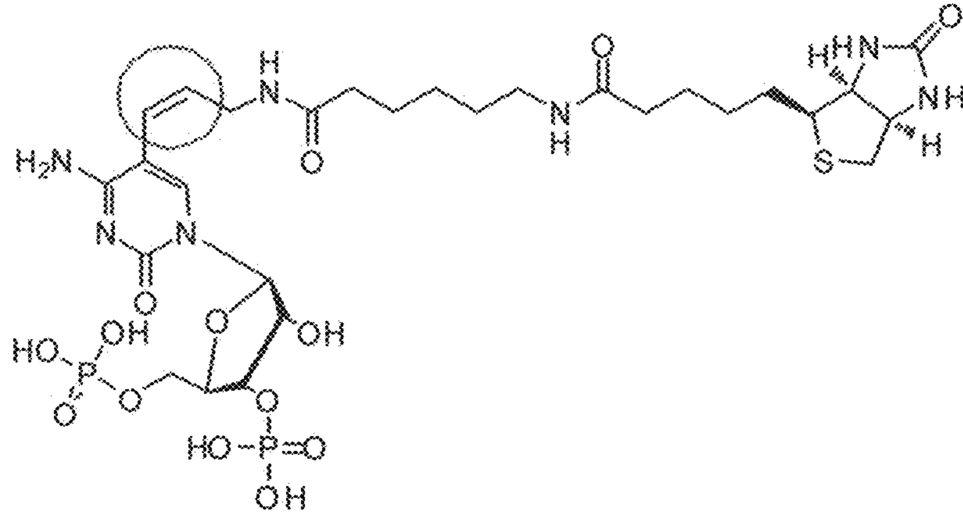
3',5'-Bisphosphorylated Cytidine-Alkene-LC-Biotin
