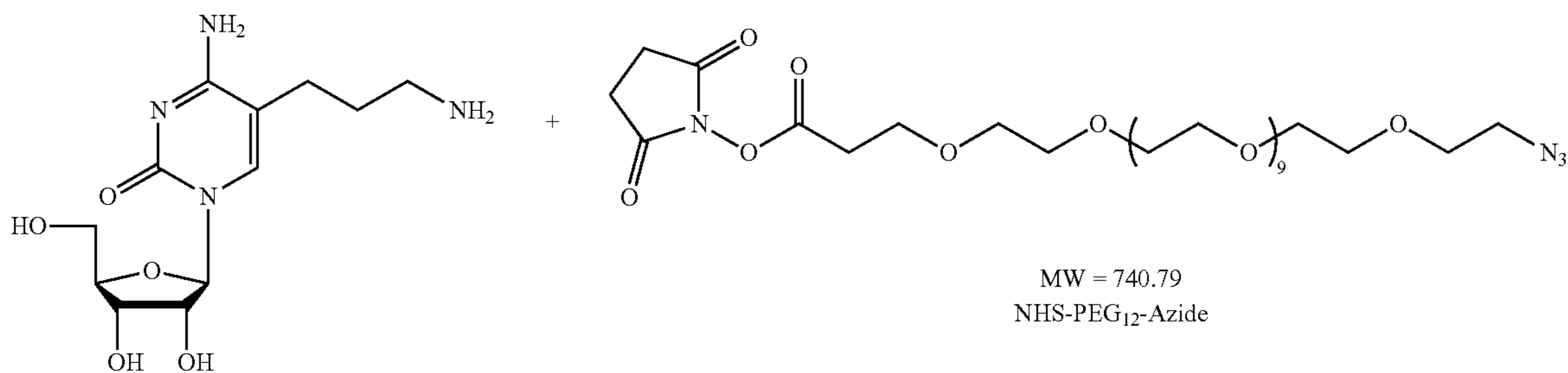
4 MW = 300.31 5-(3-aminopropyl)cytidine
