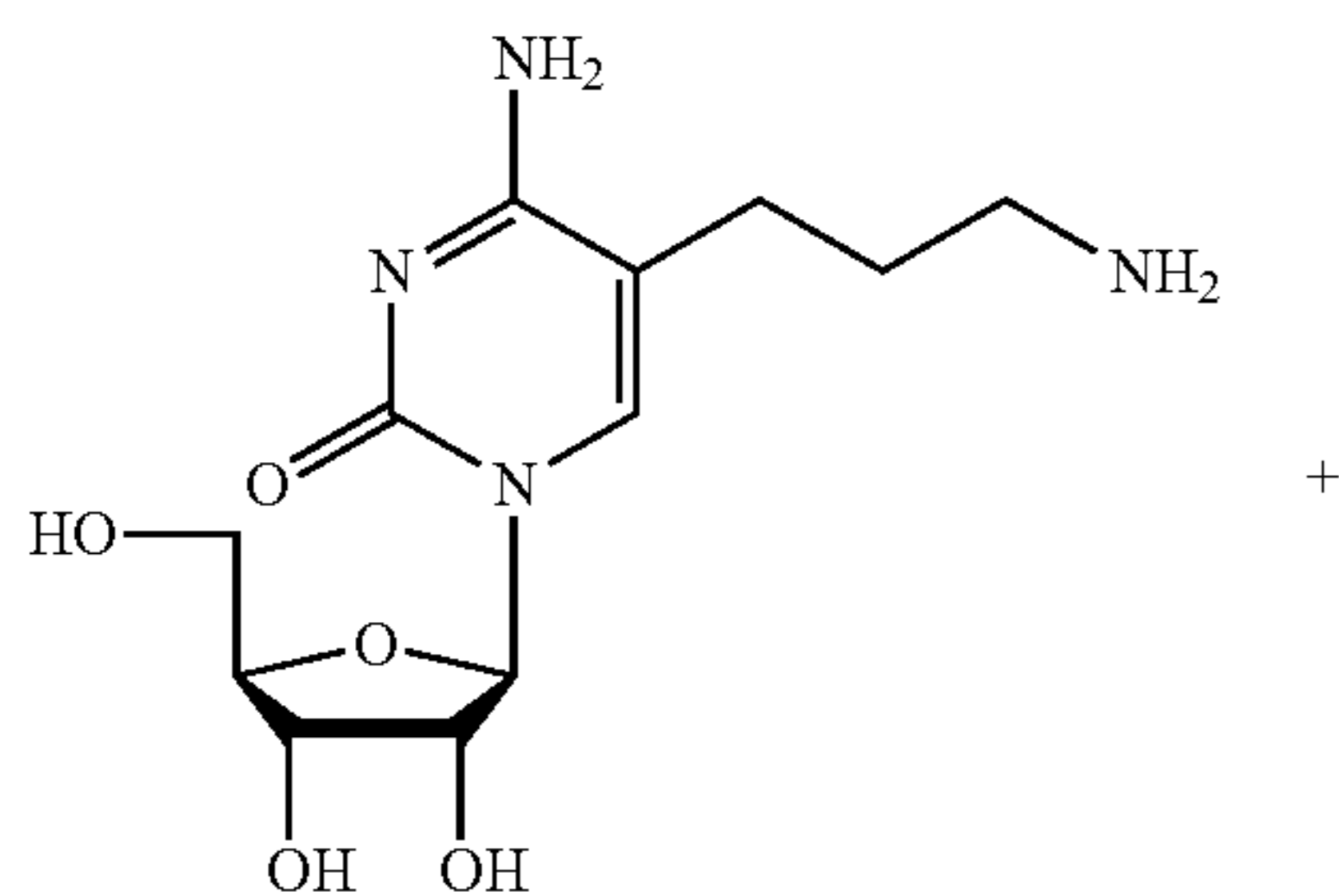
4 MW = 300.31 5-(3-aminopropyl)cytidine
