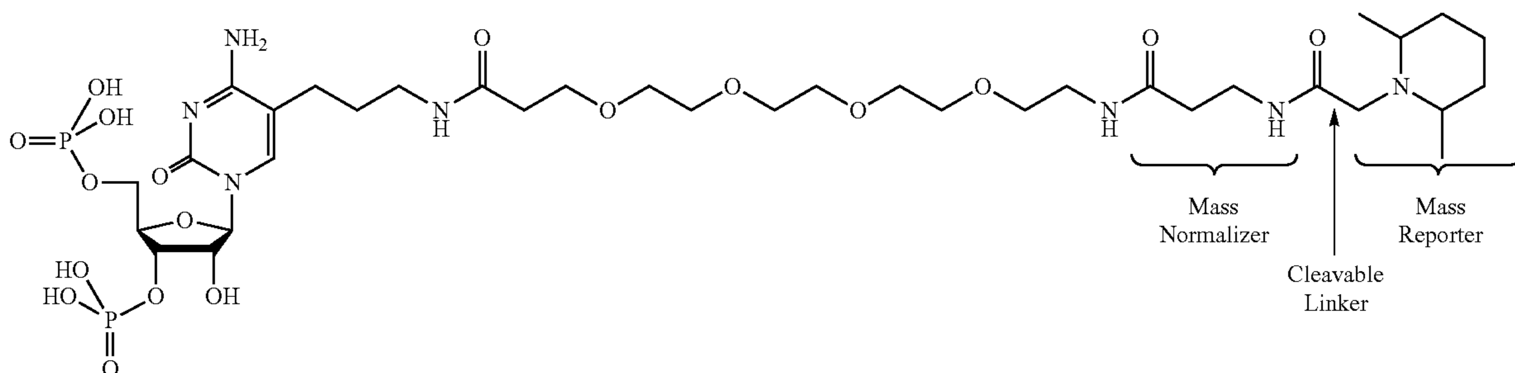
TMT-PEG 4 -Alkane-3',5'-Bisphosphate-Cytidine (TMTP 4 A-3',5'-pCp)
