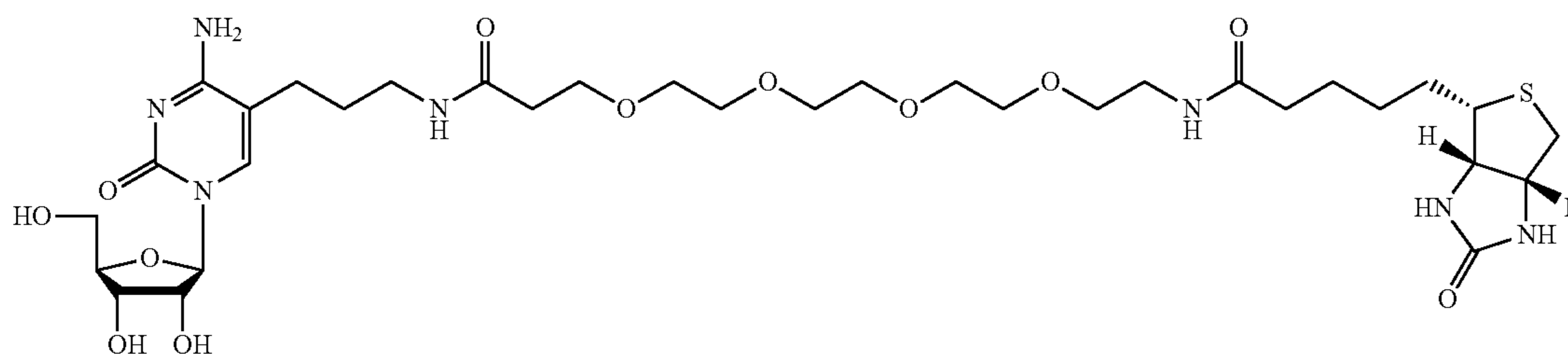
5 MW = 773.89 BPAC
