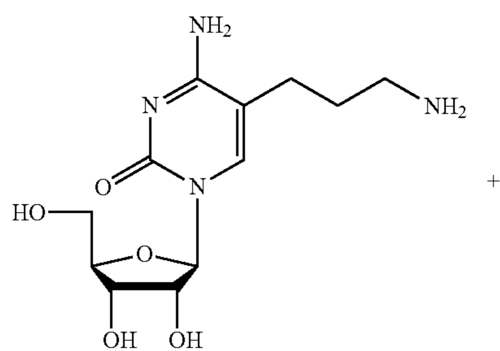
4 MW = 300.31 5-(3-aminopropyl)cytidine
