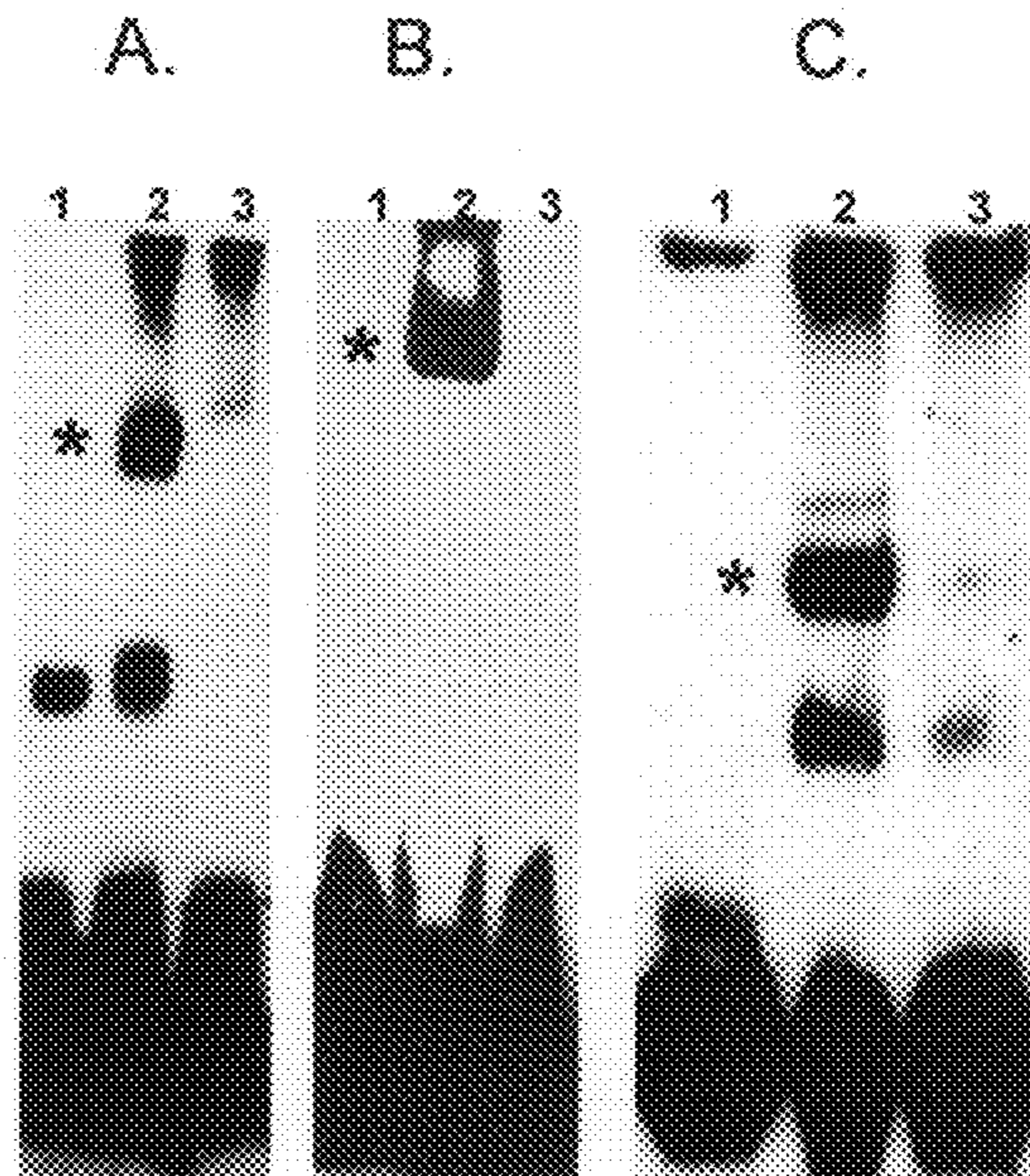
Functionality of Biotin-PEG n -Alkane-3', 5'-Cytidine Bisphosphate
