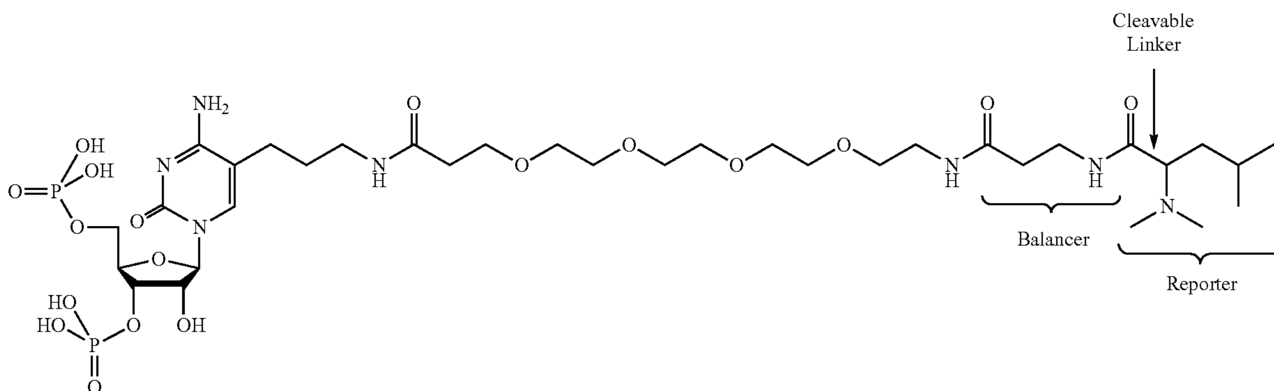
DiART-PEG 4 -Alkane-3',5'-Bisphosphate-Cytidine (DiARTP 4 A-3',5'-pCp)
