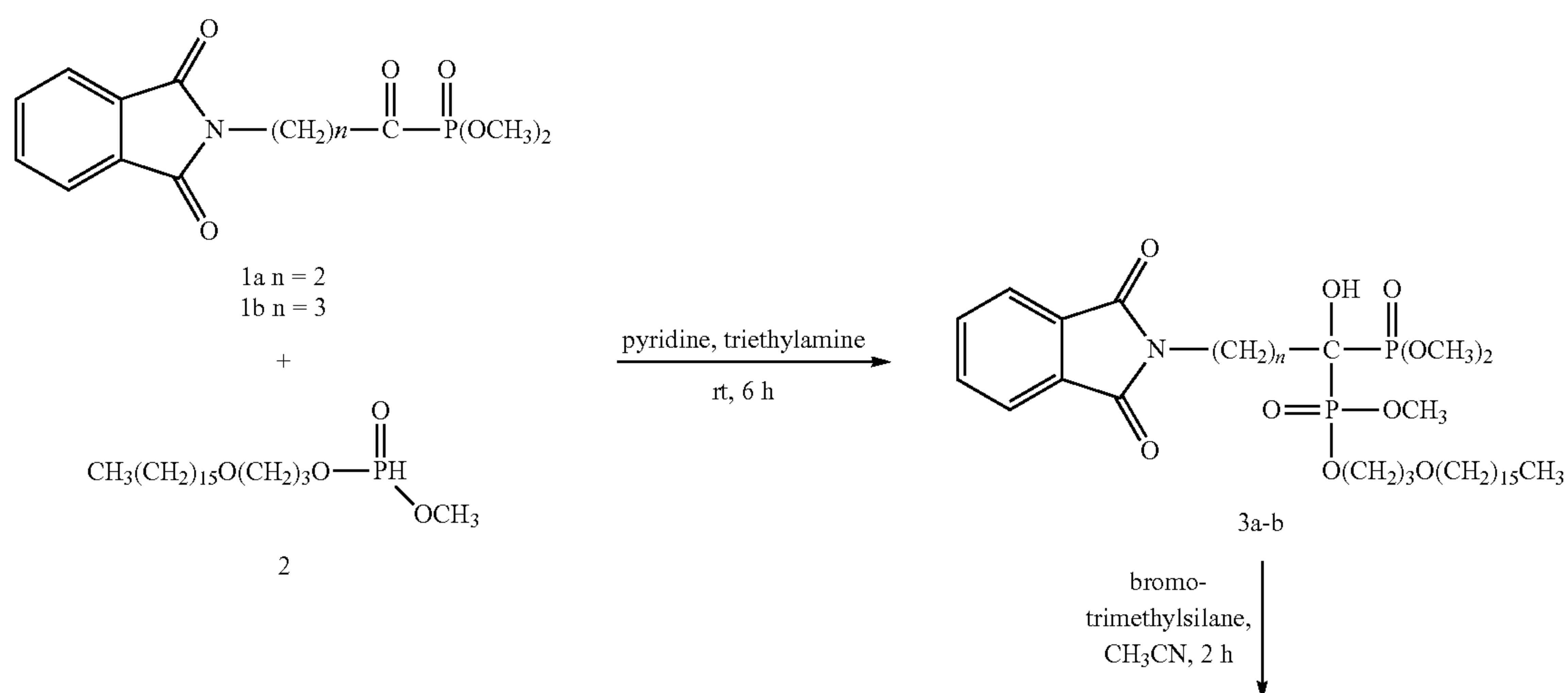
Scheme I
