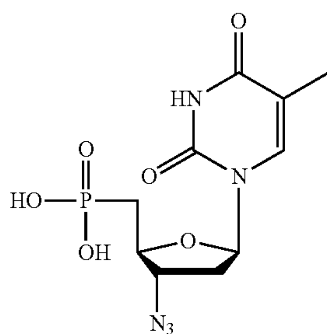
AZT 5'-phosphonate
