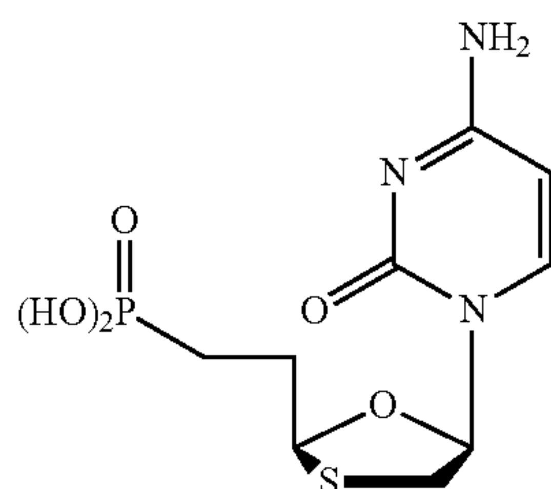
3'-thia-2',3'-dideoxycytidine-5'-phosphonic acid
