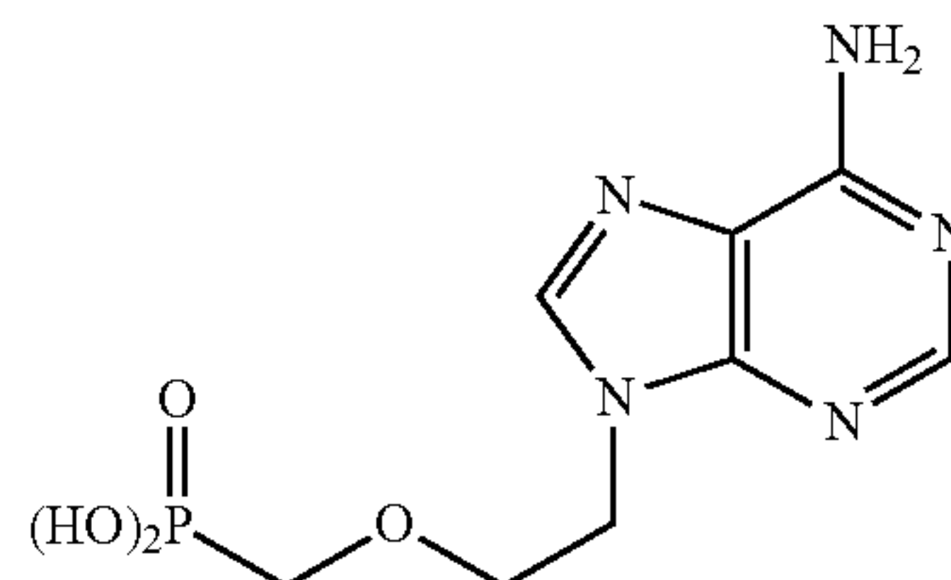
9-[3-(phosphonomethoxy)propyl]adenine (Adefovir)
