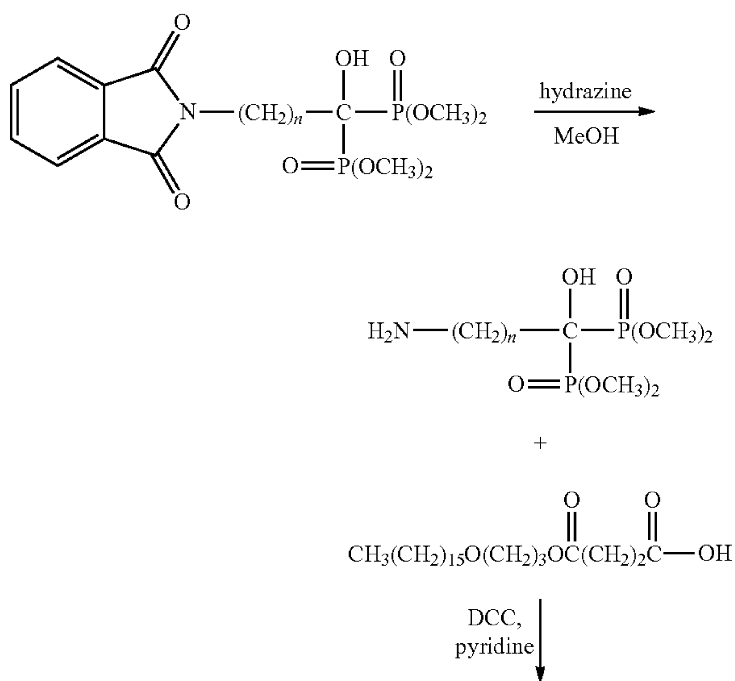
Scheme IV
