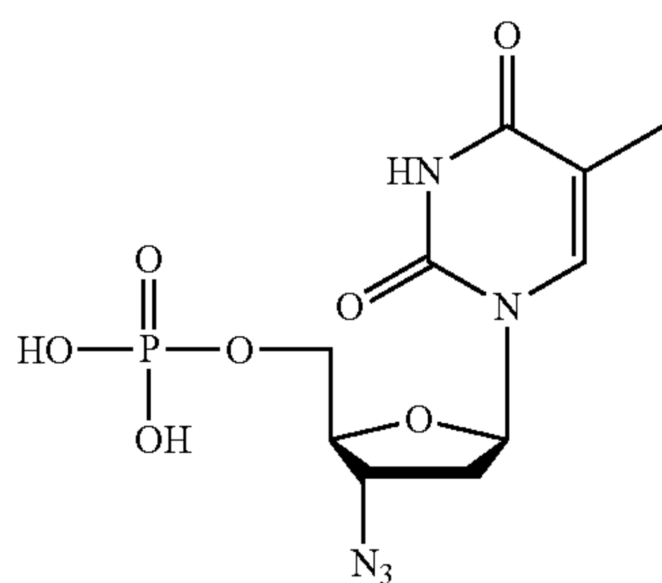
AZT 5'-phosphate
