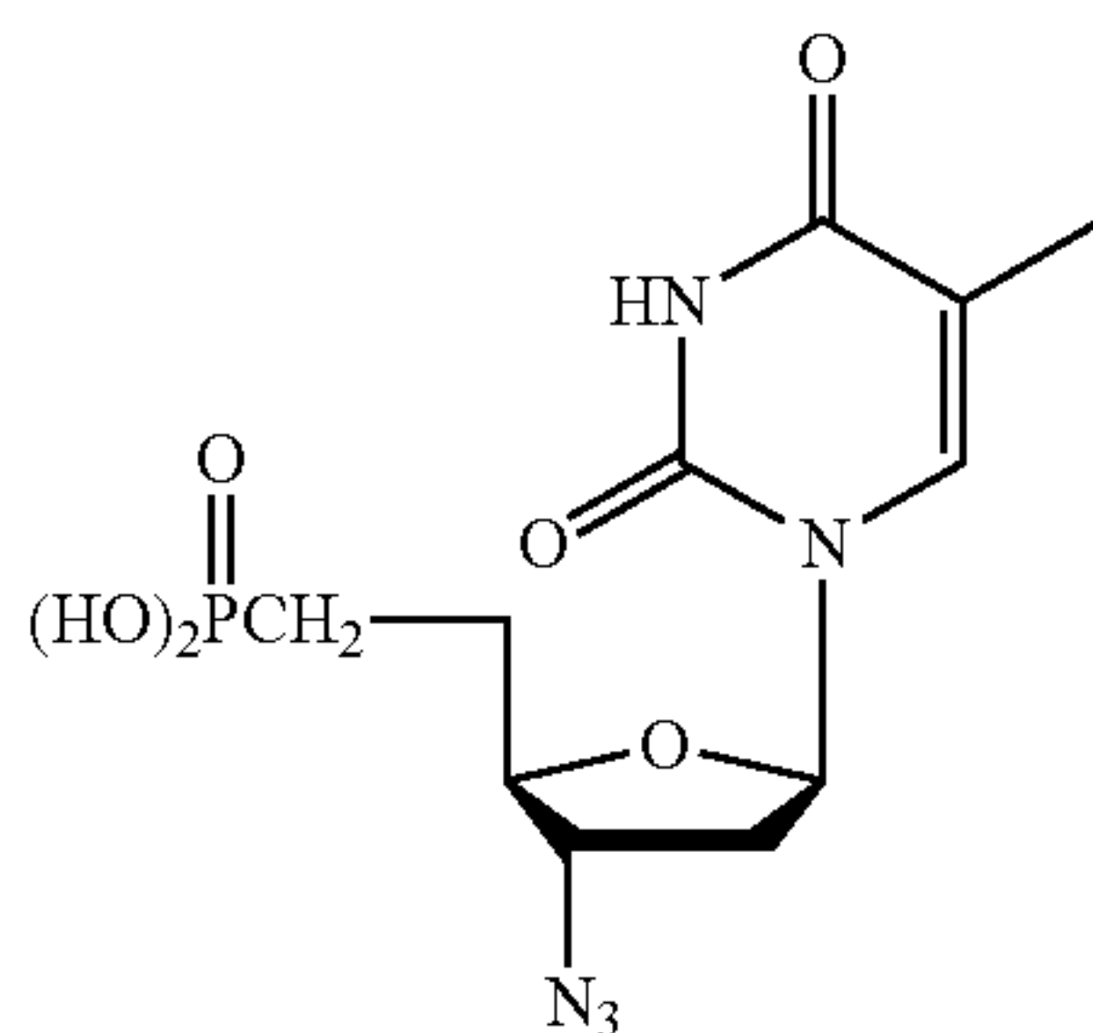
AZT 5'-methylene-phosphonate
