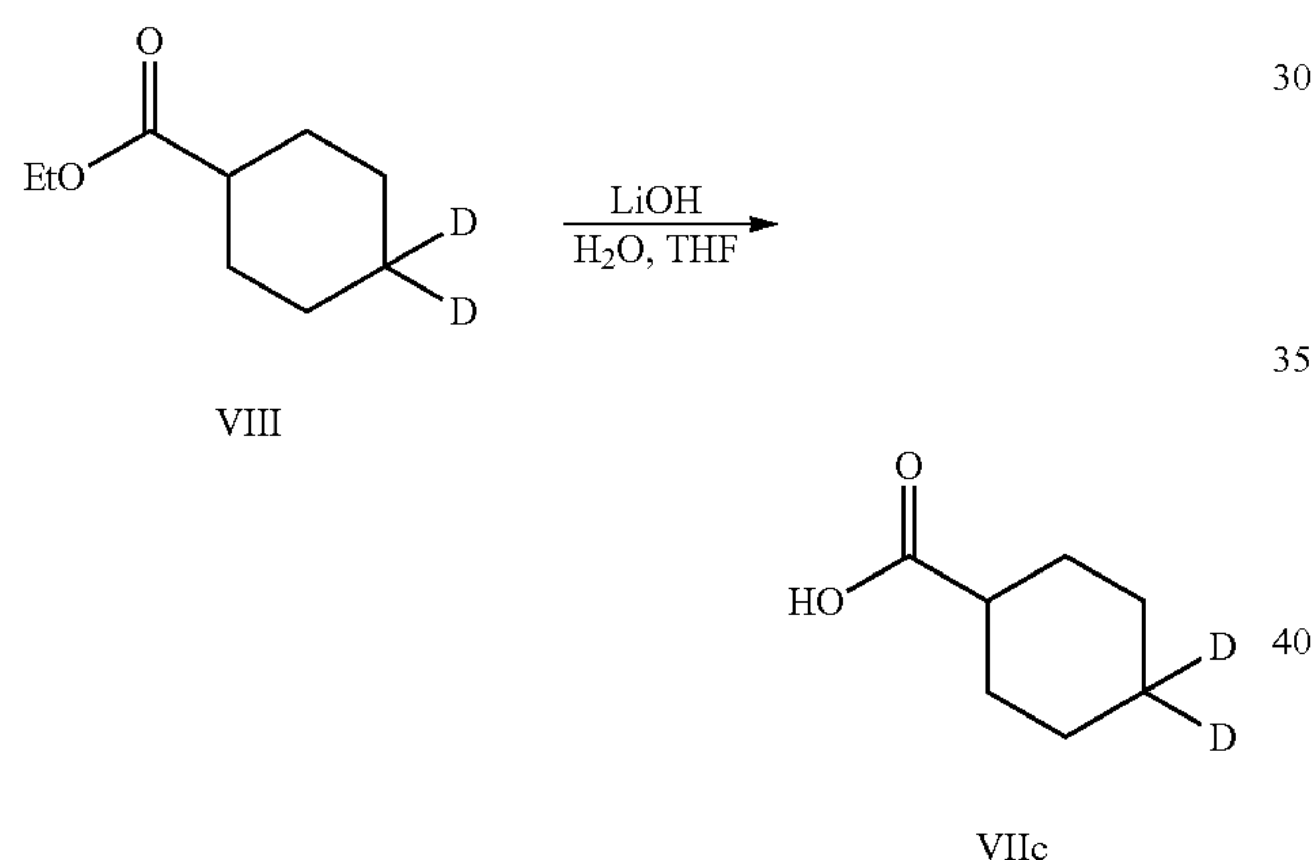
Scheme 3: Method for Preparation of Intermediate VIIc
