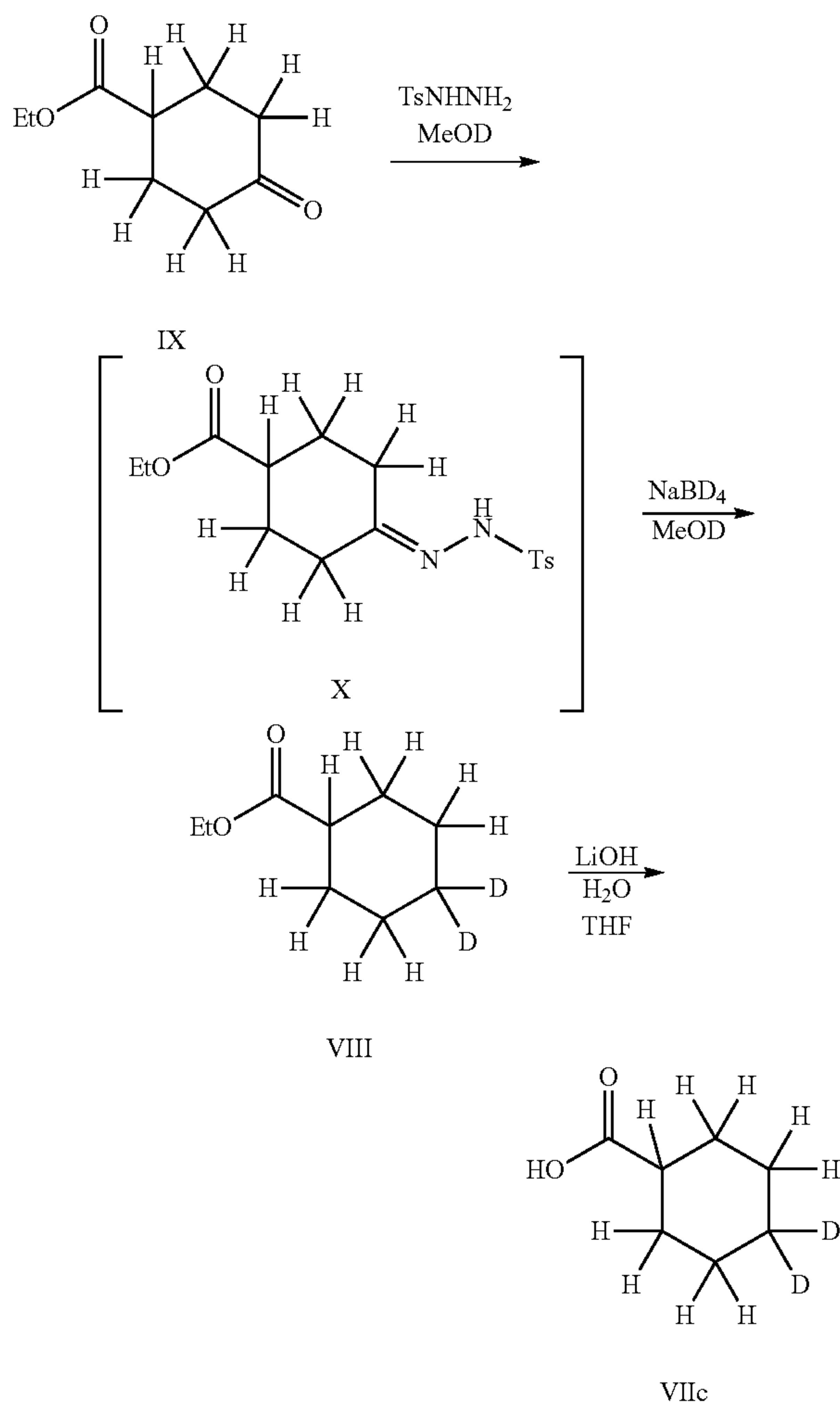
Scheme 7. Preparation of Intermediate VIIc
