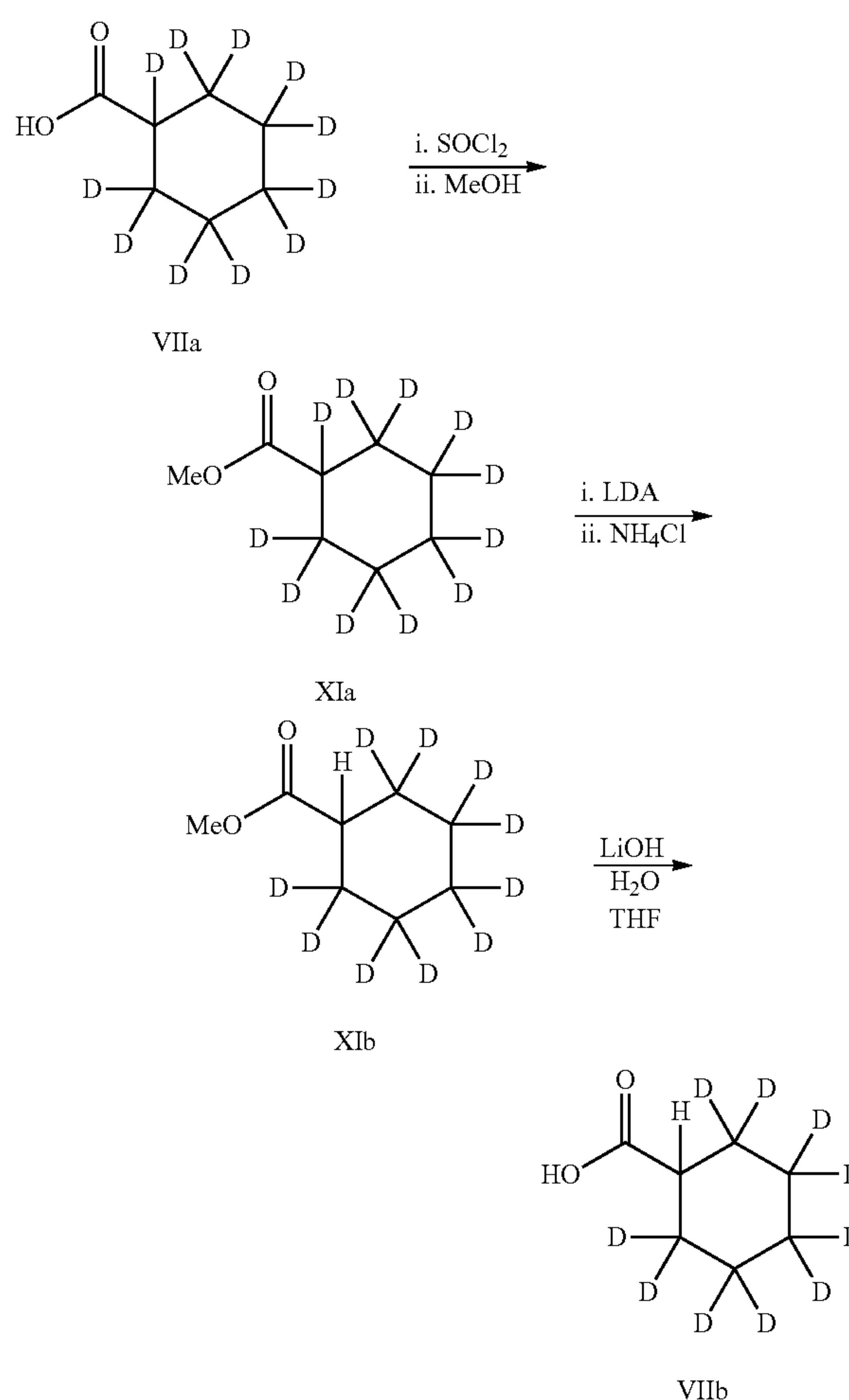
Scheme 6. Preparation of Intermediate VIIb
