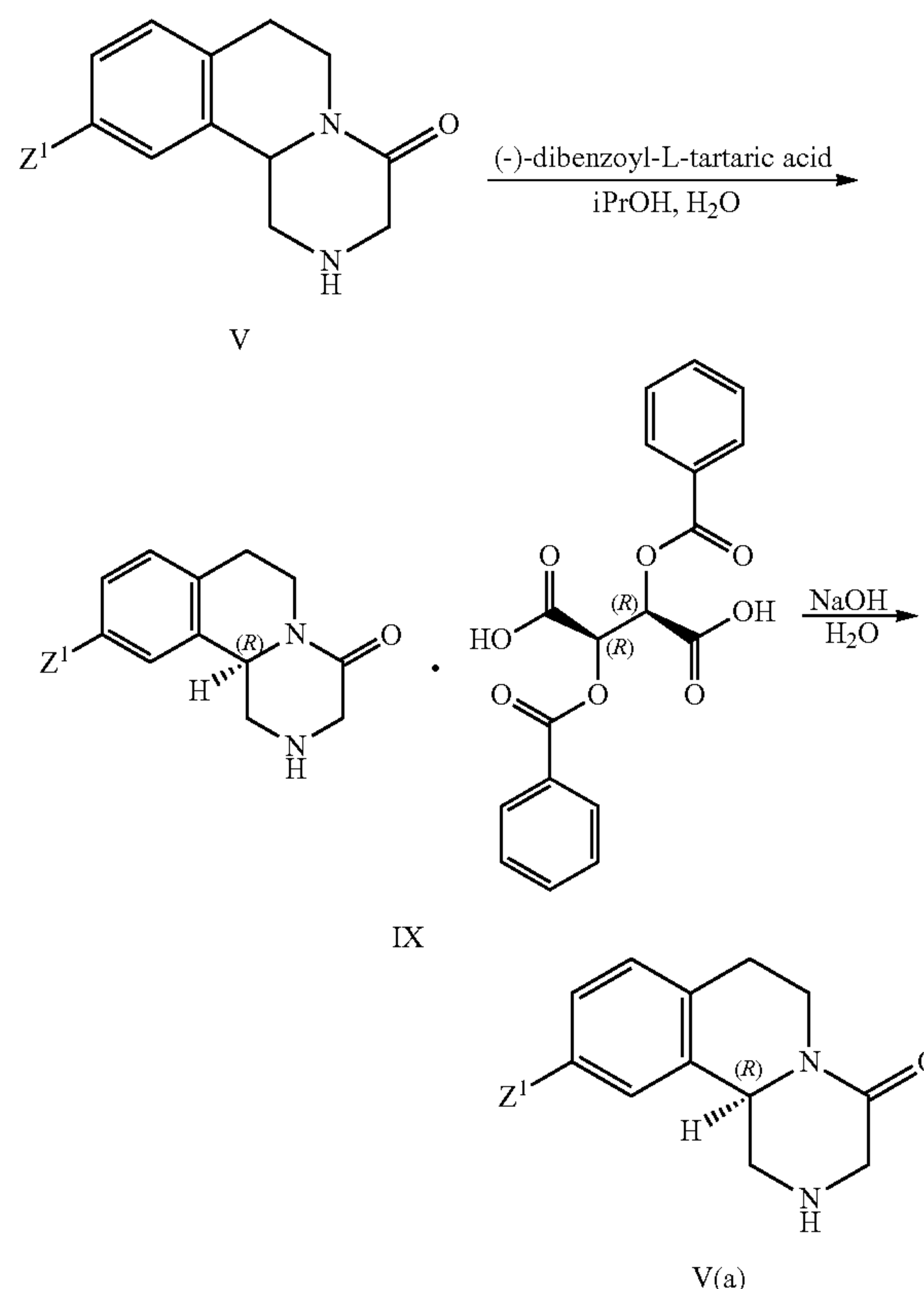
Scheme 5: Method for the Preparation of Intermediates V(a)
