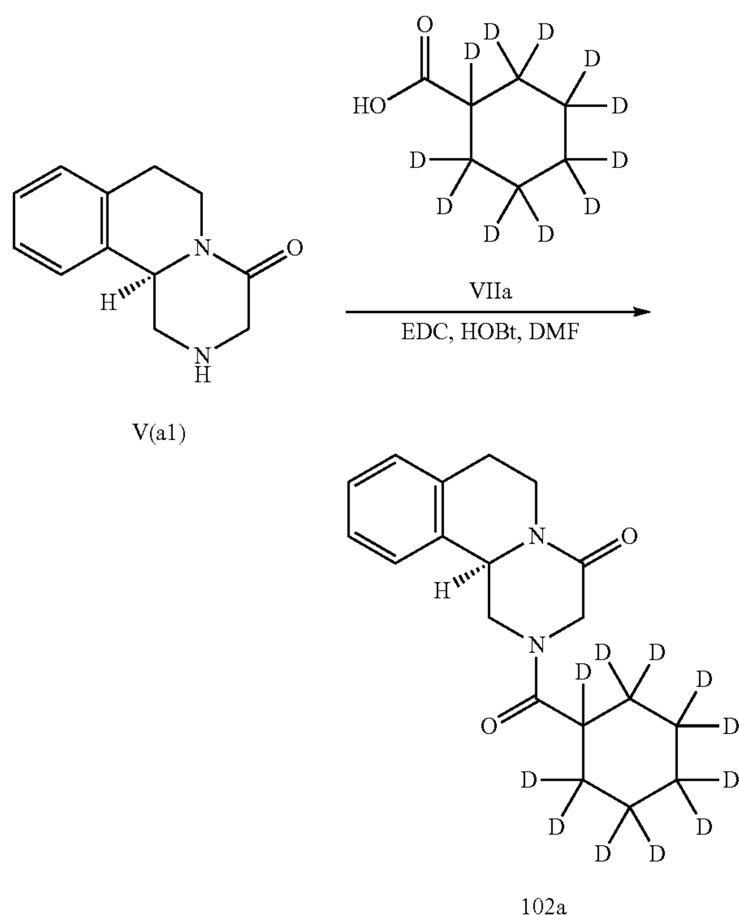
Scheme 10. Preparation of Compound 102a
