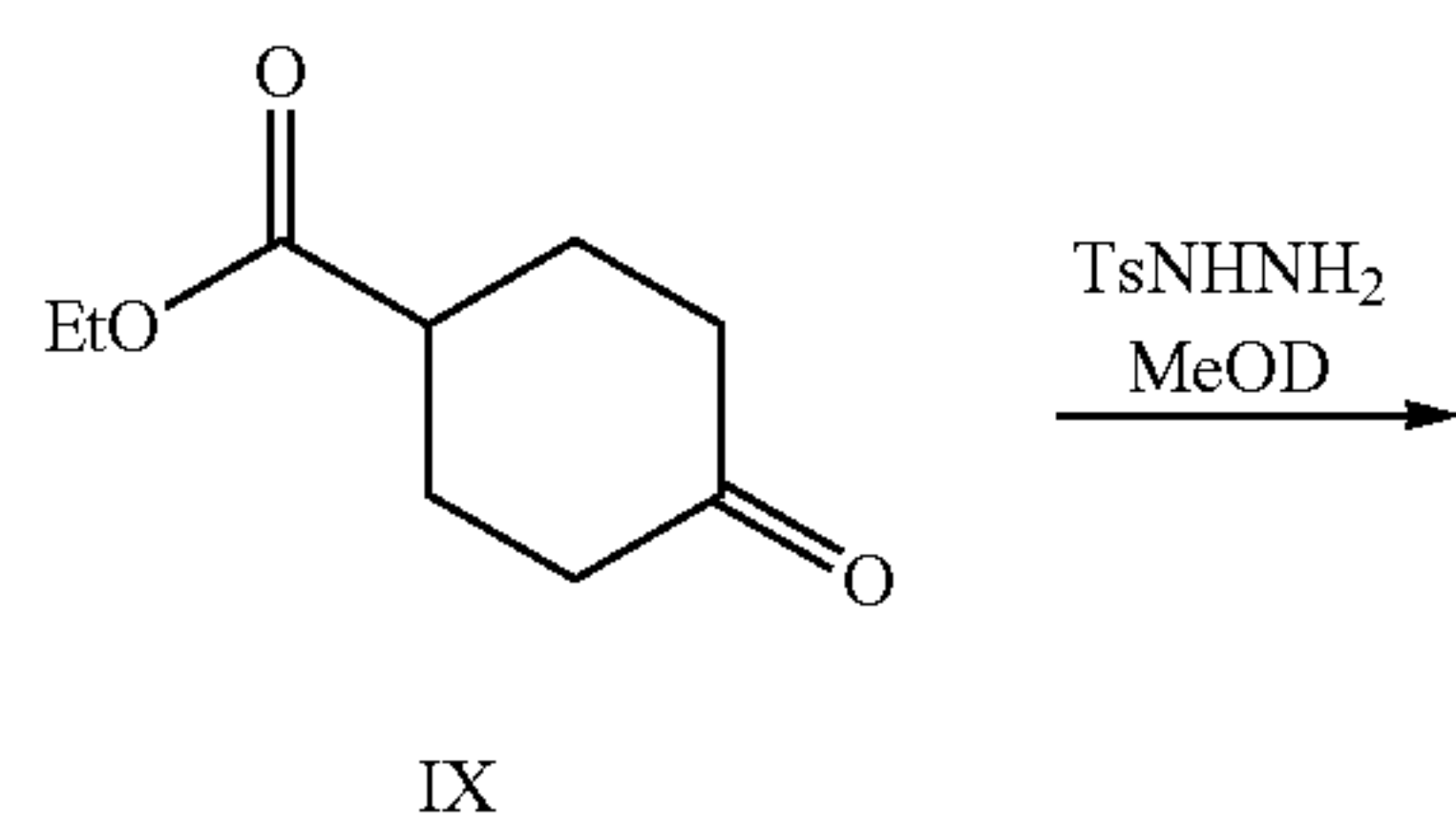
Scheme 3a: Method for Preparation of Intermediate VIII
