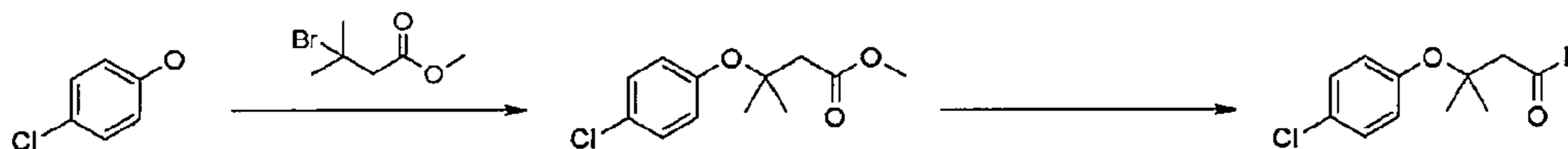
Scheme 5:
