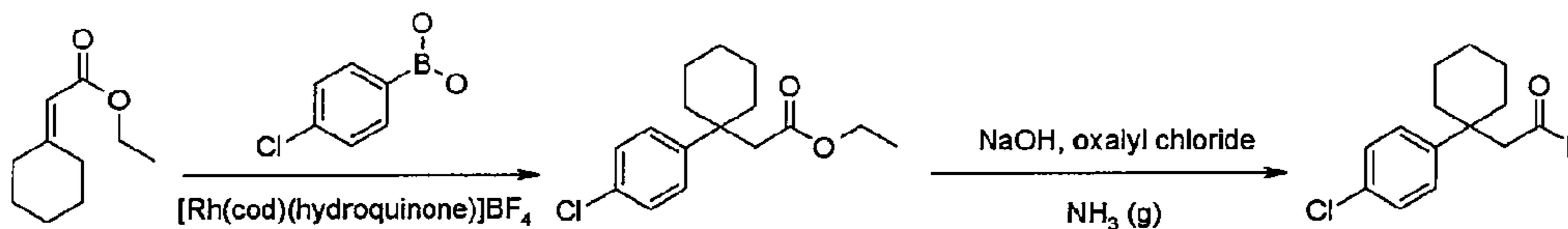
Scheme 4:
