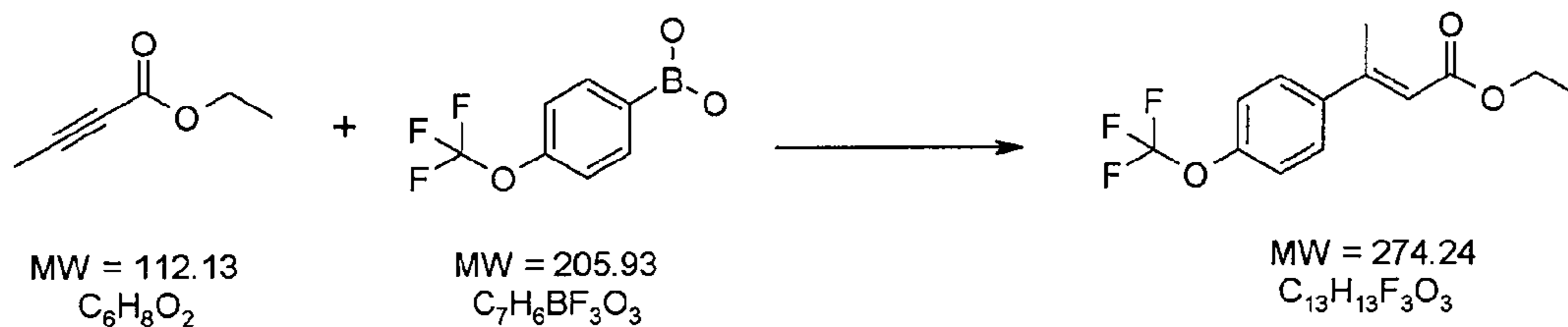
Scheme 10:
