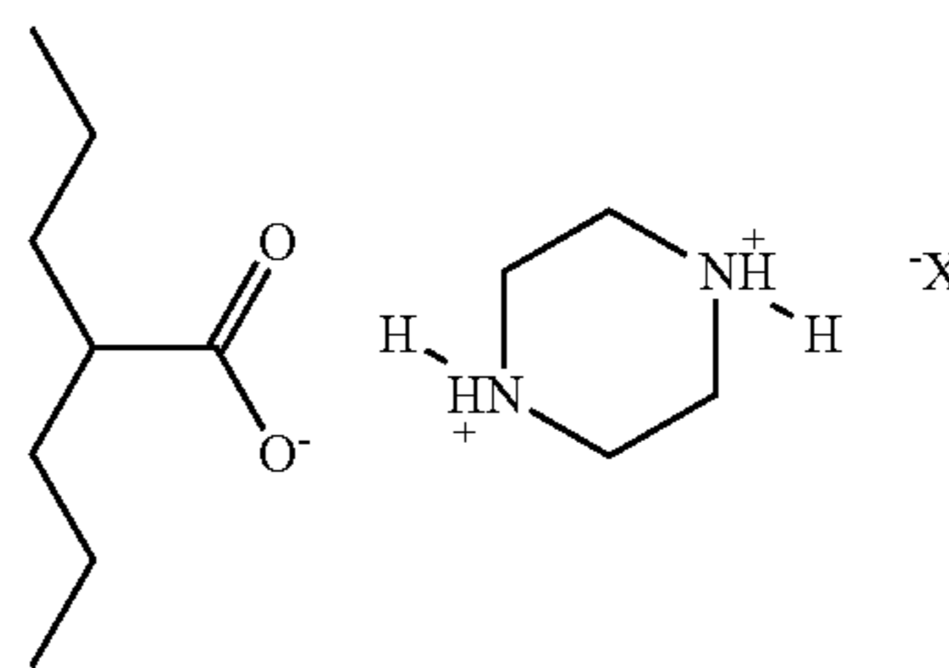
Formula I
