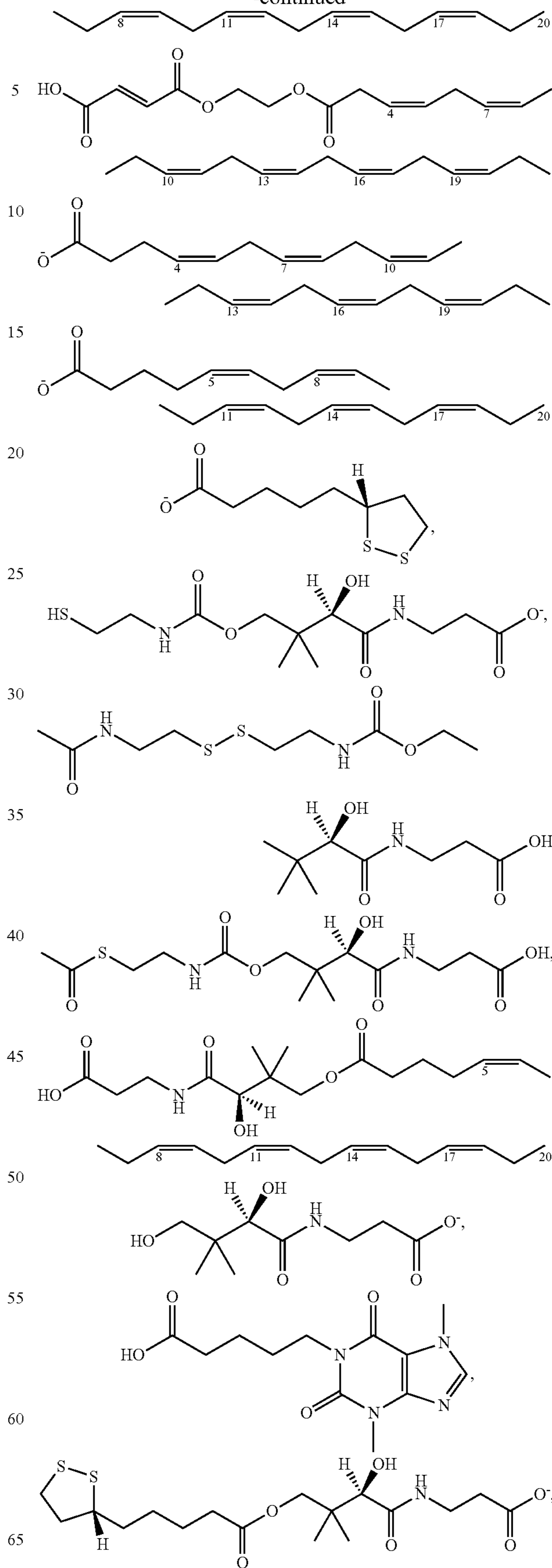
Formula I
