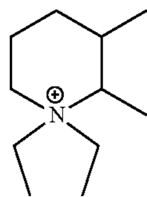
N,N-diethyl- 2,3-dimethyl- piperidinium cation
