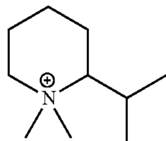
N,N-dimethyl-2- isopropylpiper- idinium cation
