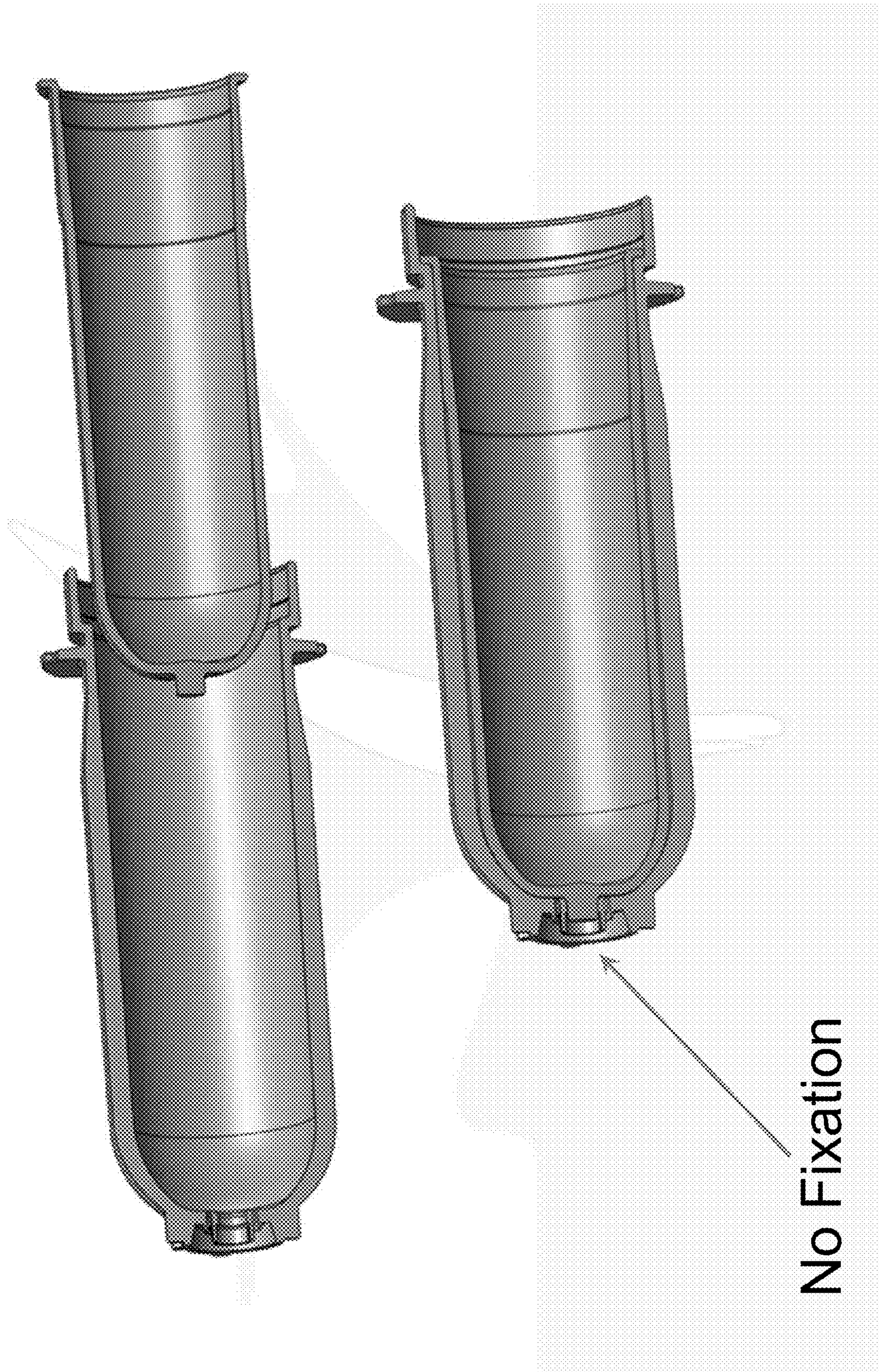
Fig. 23 - Assembly of the Pre-form
