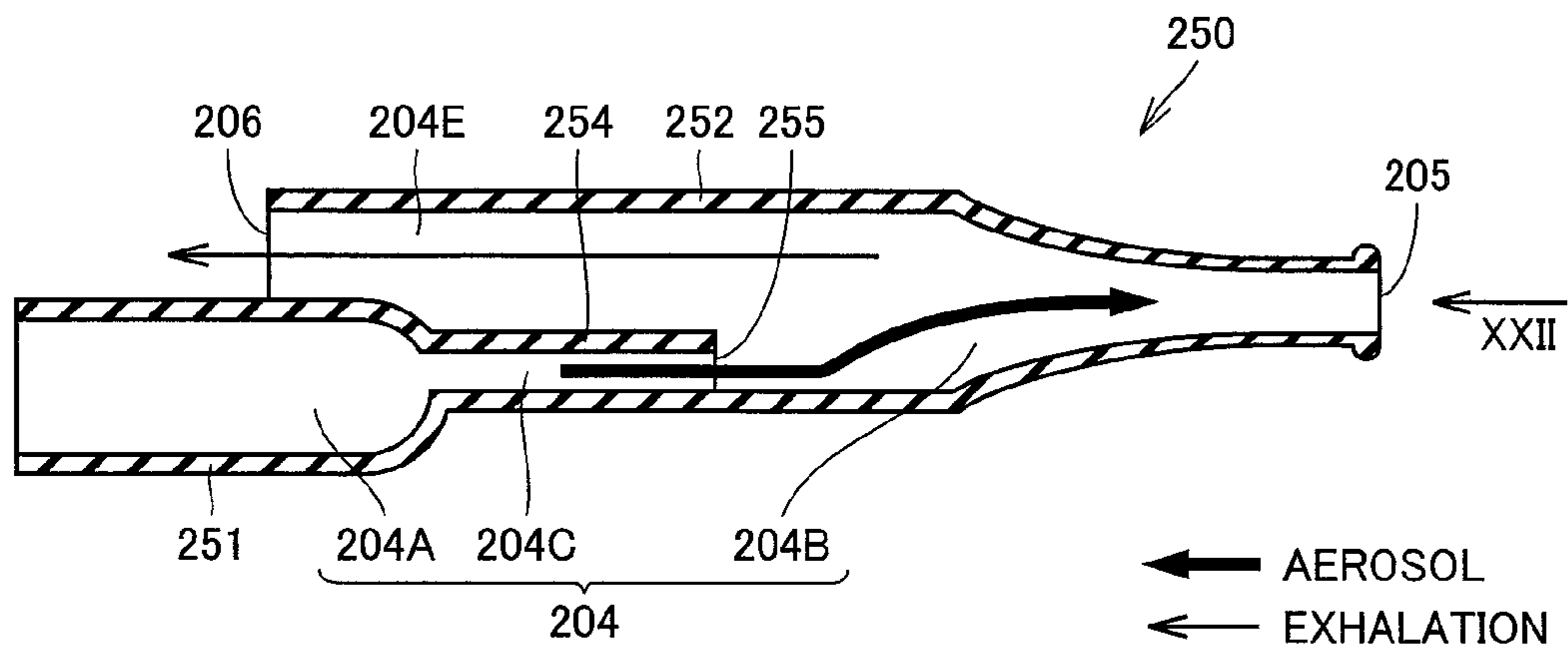
FIG.21 PRIOR ART
