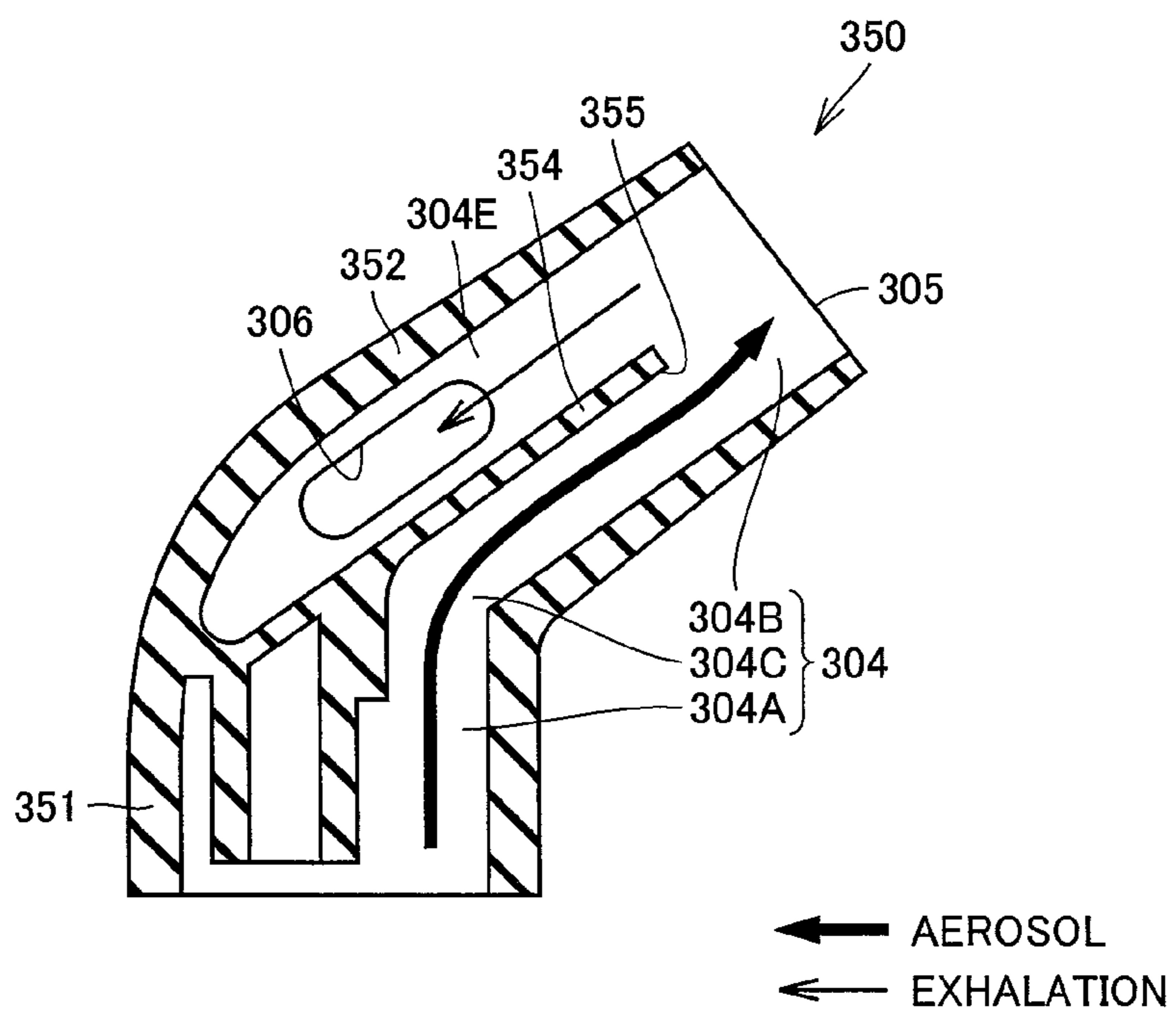
FIG.23 PRIOR ART
