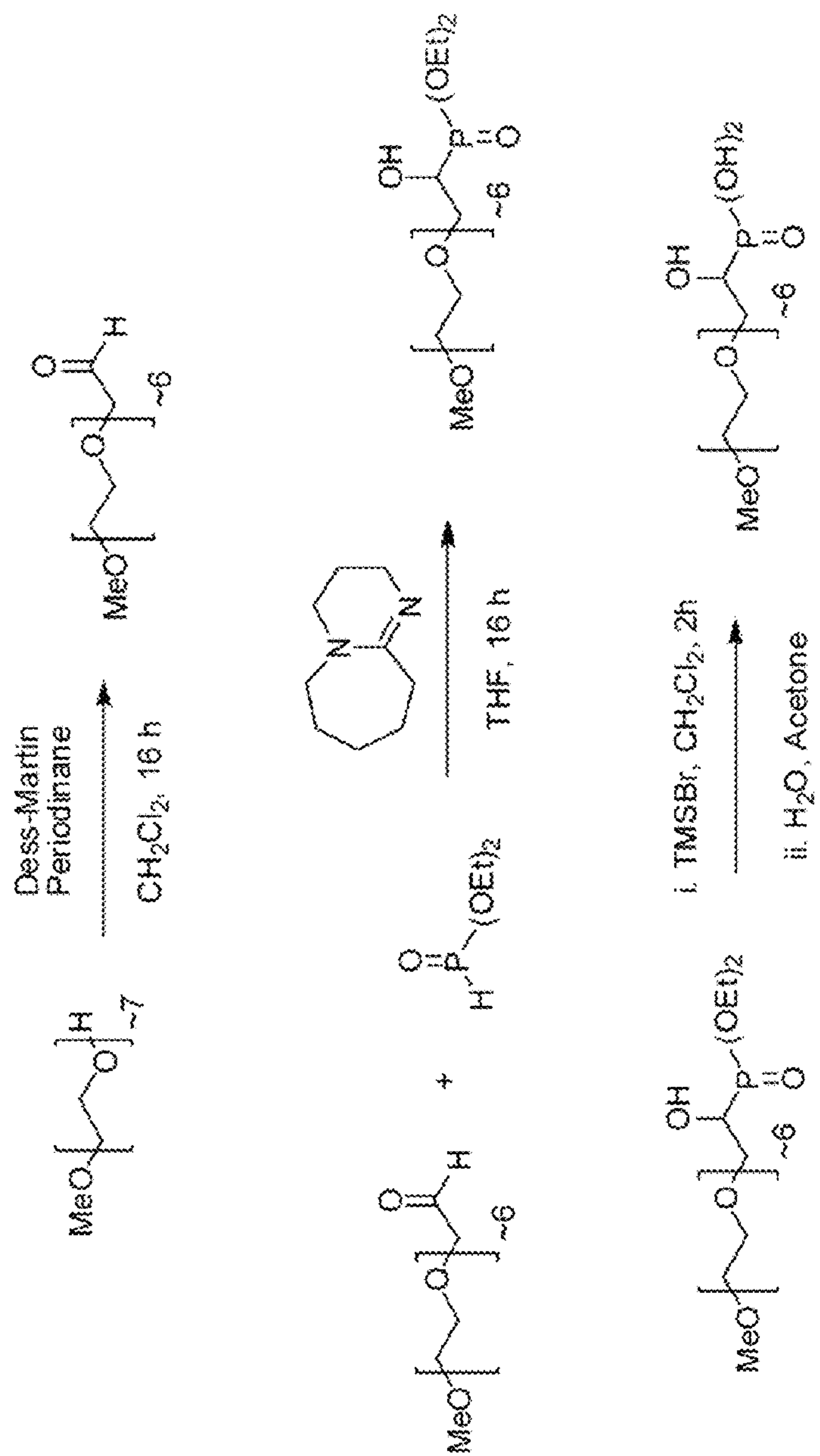
Synthesis of \alpha -Hydroxy PEG-350 Phosphonic Acid
