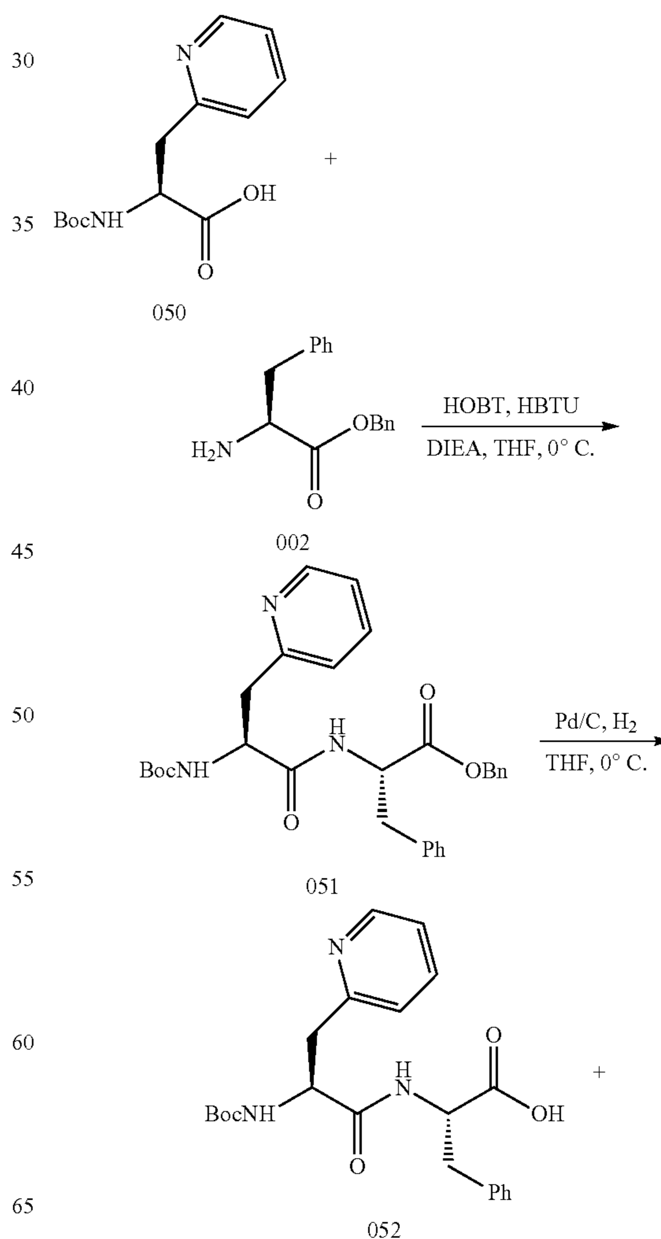
Scheme 8: Synthesis of Example 055
