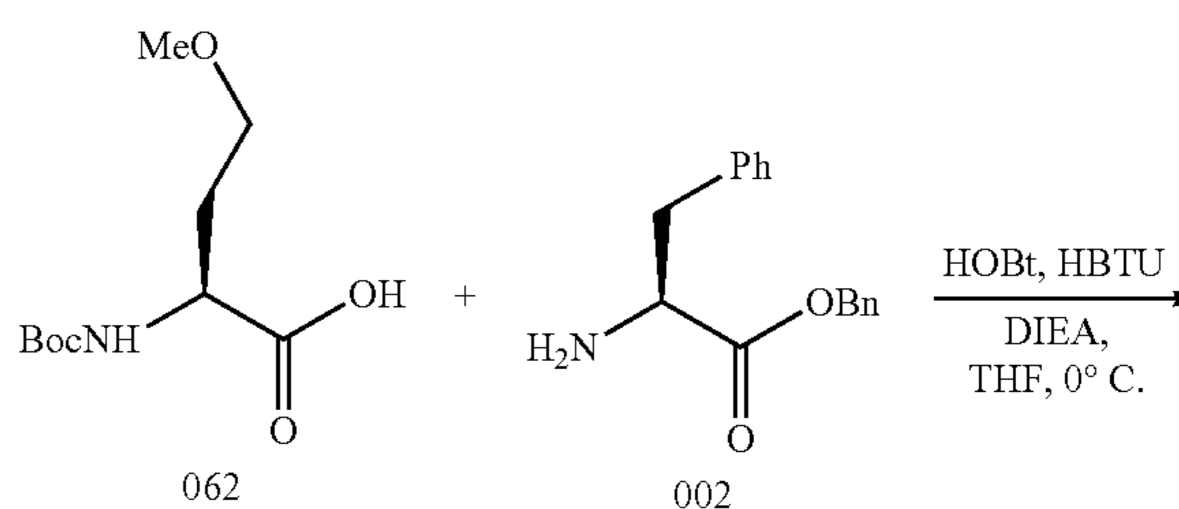
Scheme 10: Synthesis of Example 068
