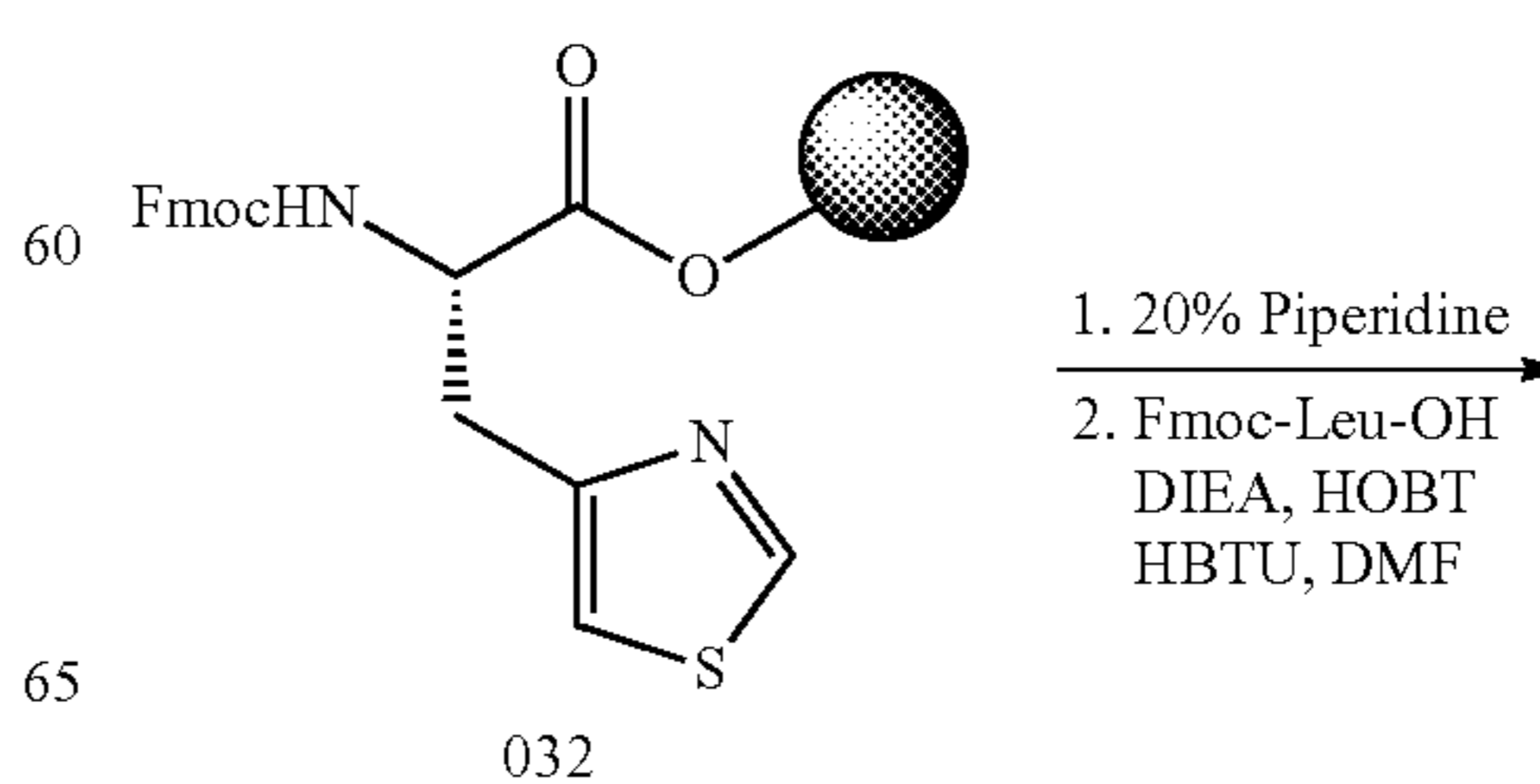
Scheme 5: Synthesis of Example 039
