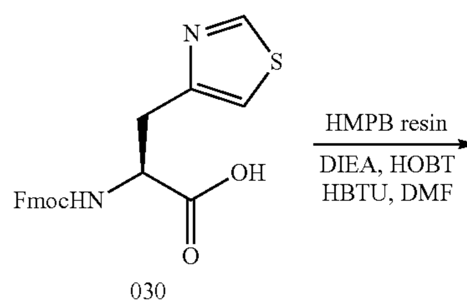
Scheme 4: Synthesis of Example 035
