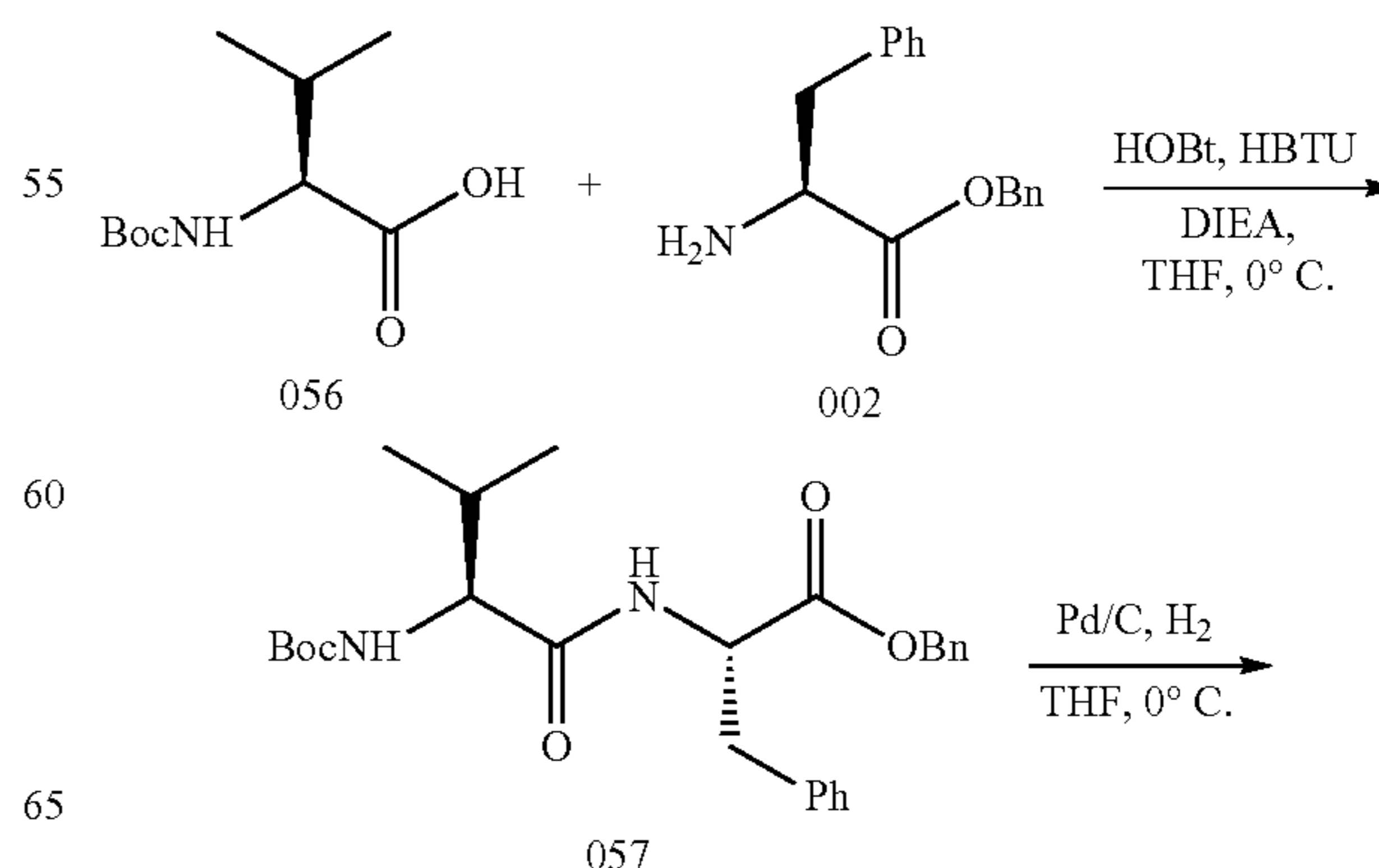
Scheme 9: Synthesis of Example 061
