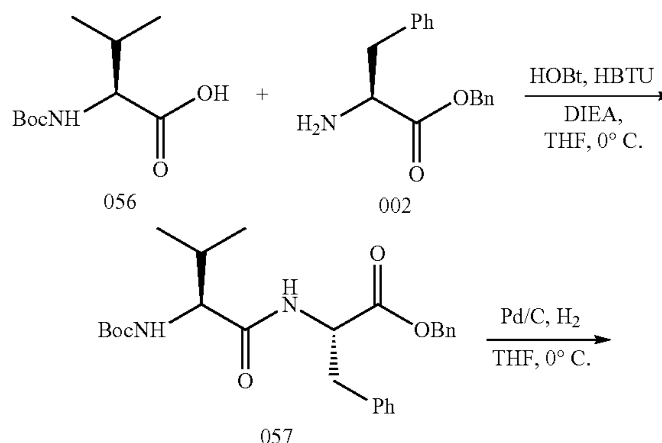
Scheme 9: Synthesis of Example 061
