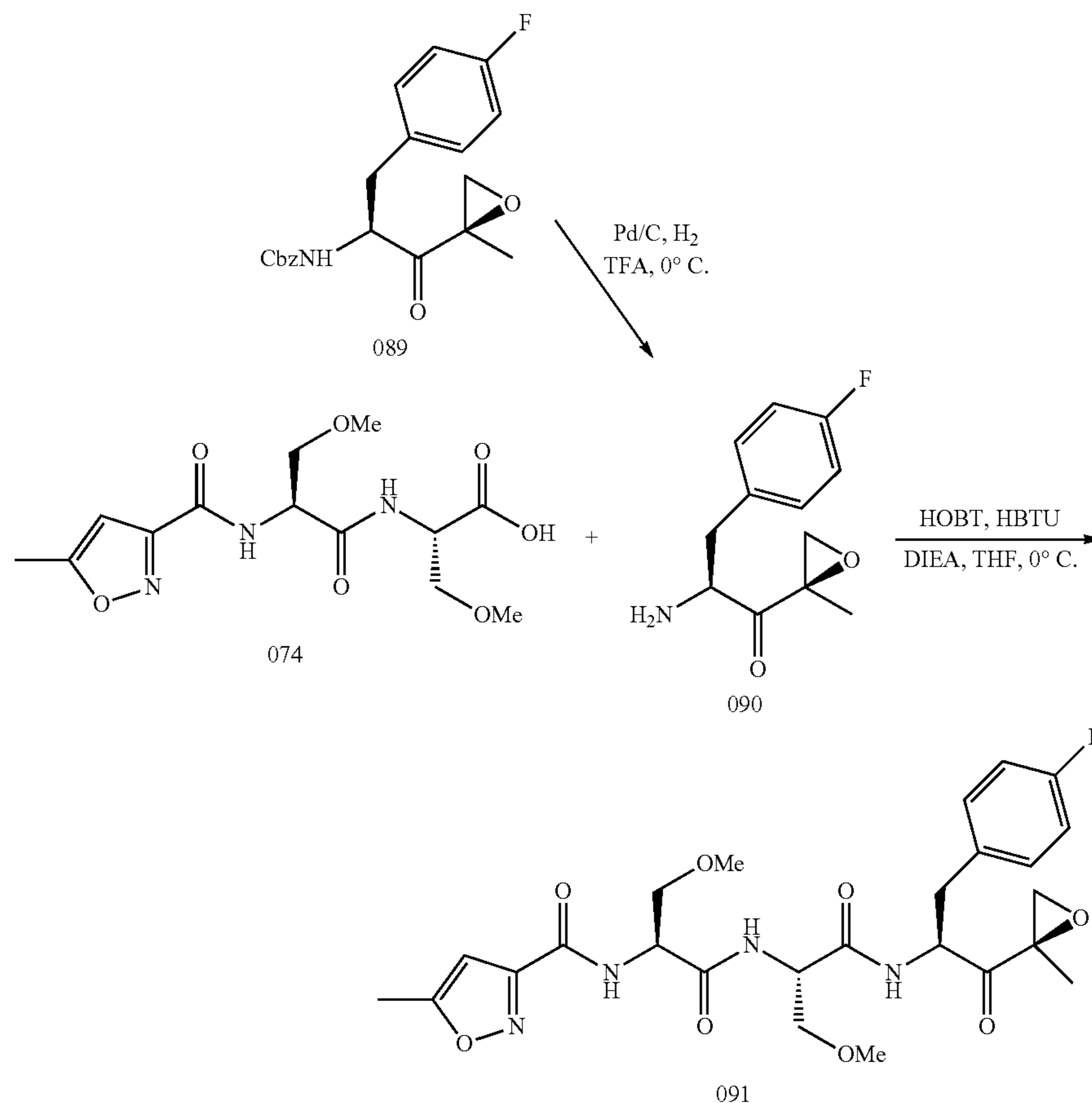
Scheme 16: Synthesis of Example 091
