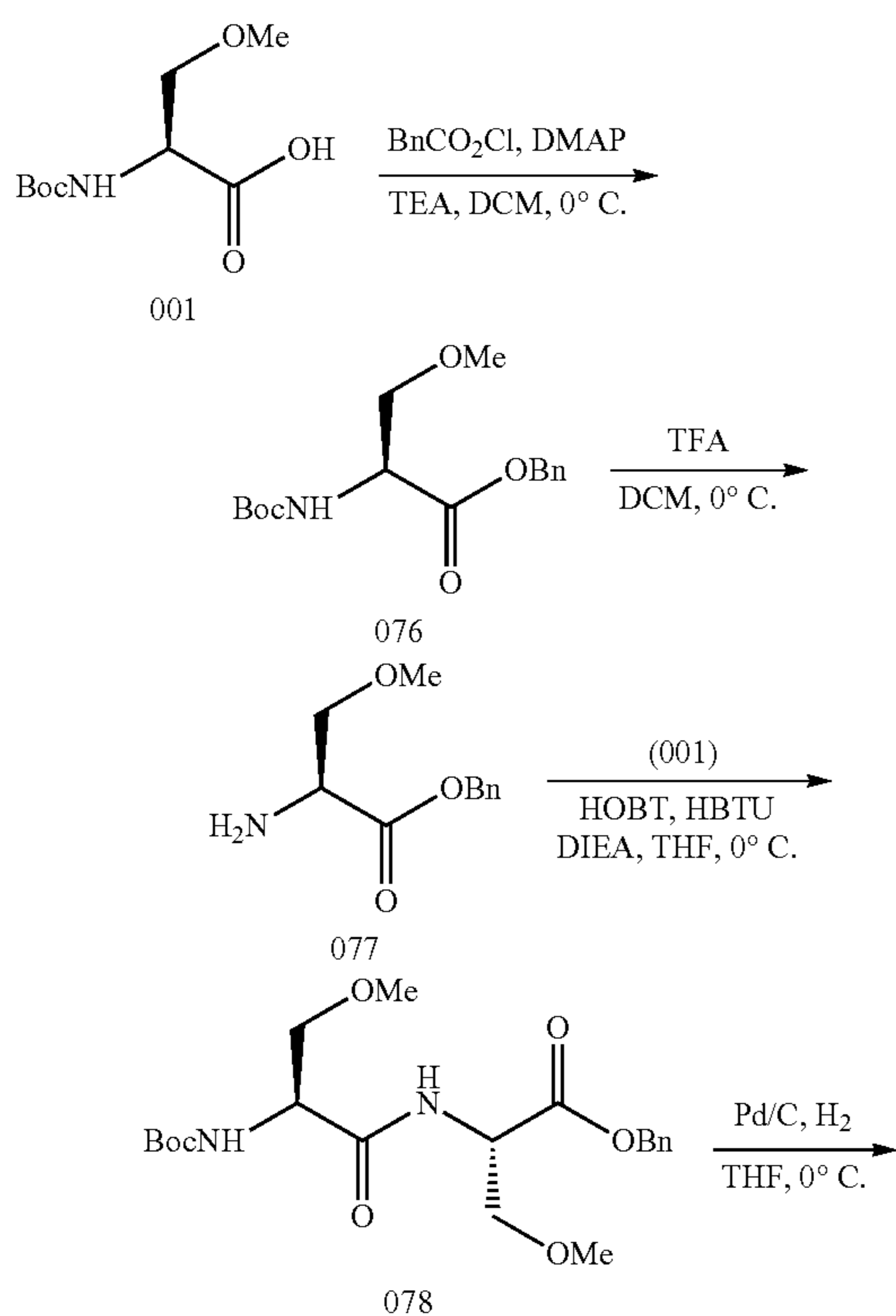
Scheme 12: Synthesis of Example 075 (approach B)
