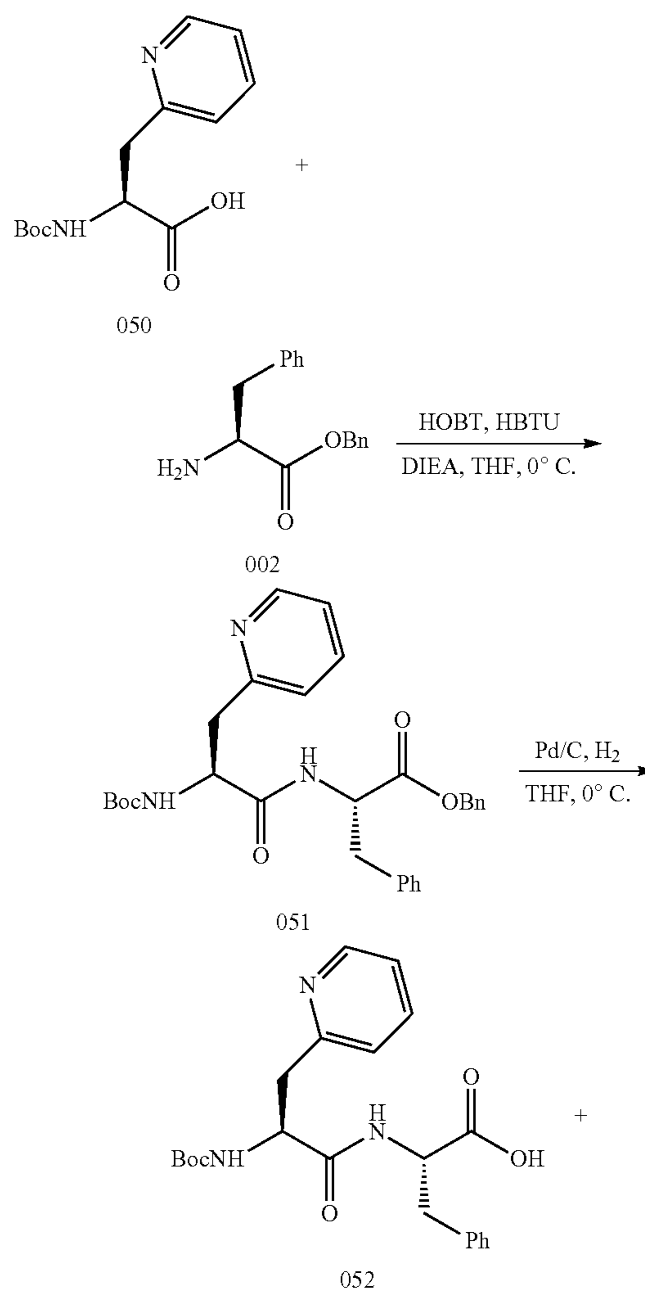
Scheme 8: Synthesis of Example 055
