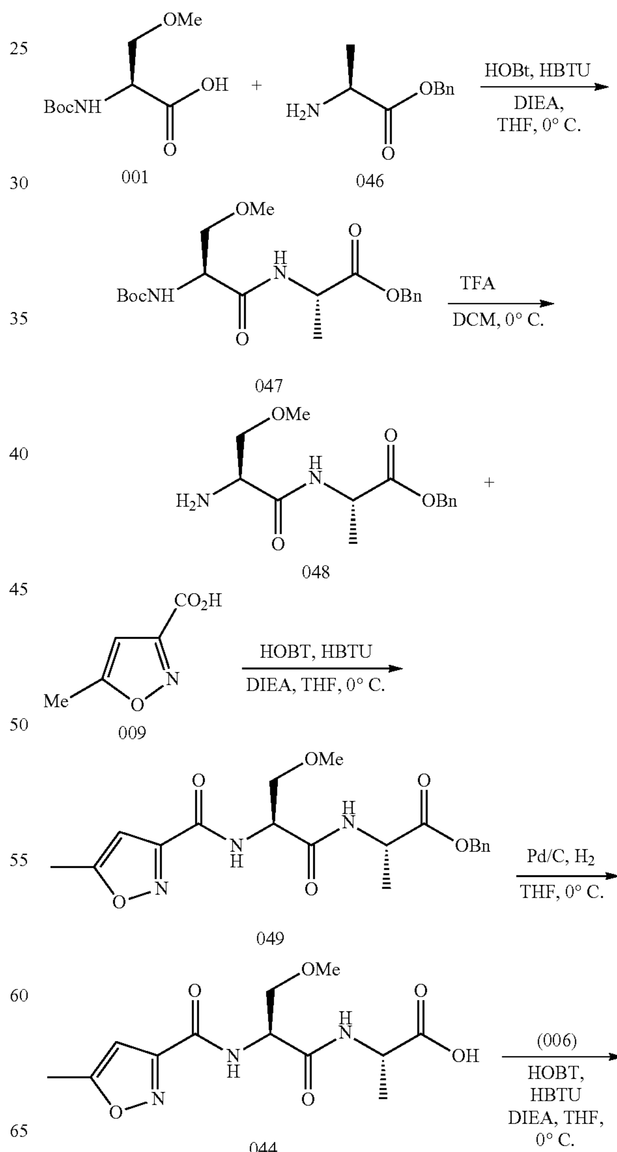
Scheme 7: Synthesis of Example 045 (approach B)
