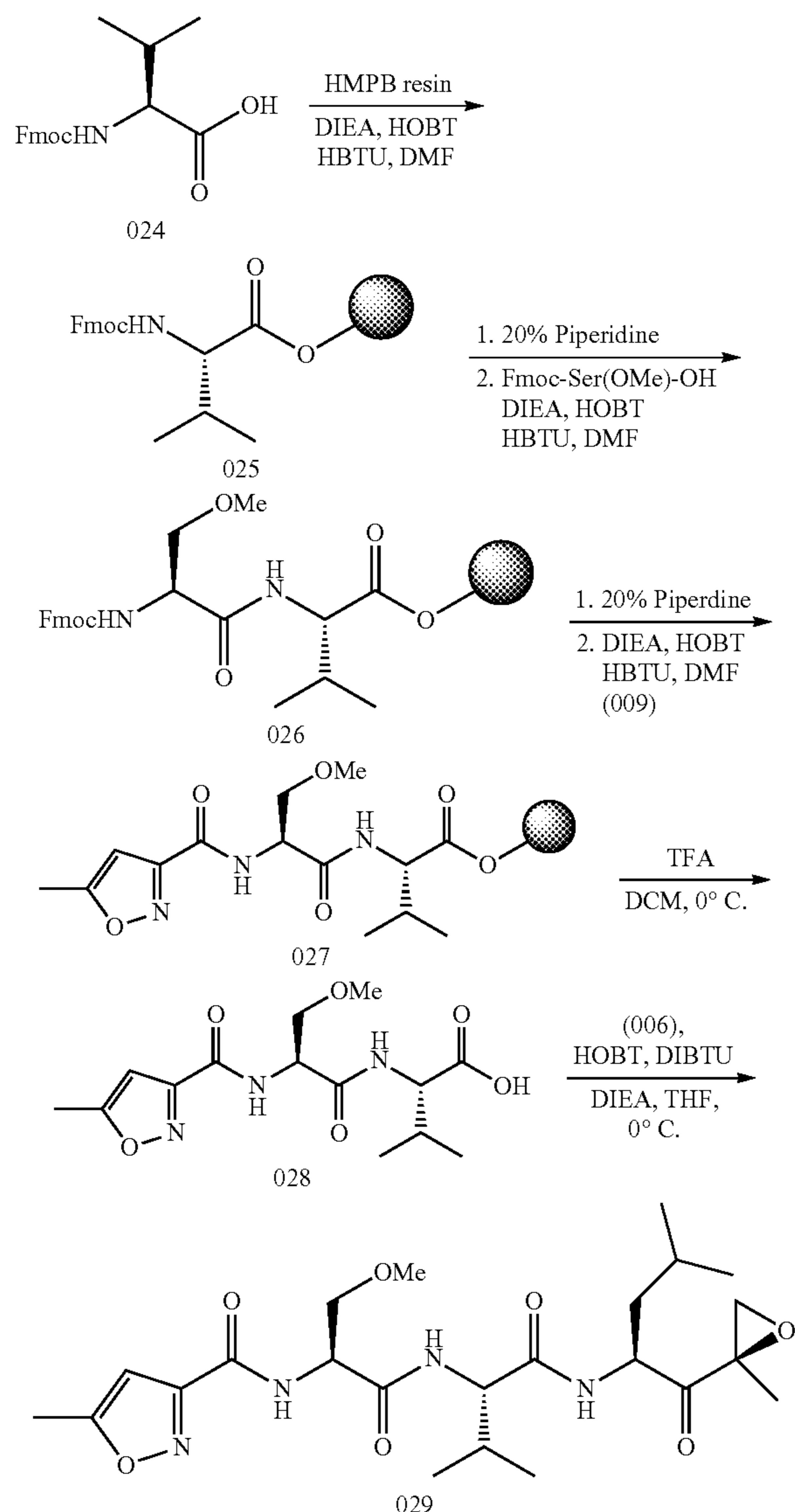
Scheme 3: Synthesis of Example 029
