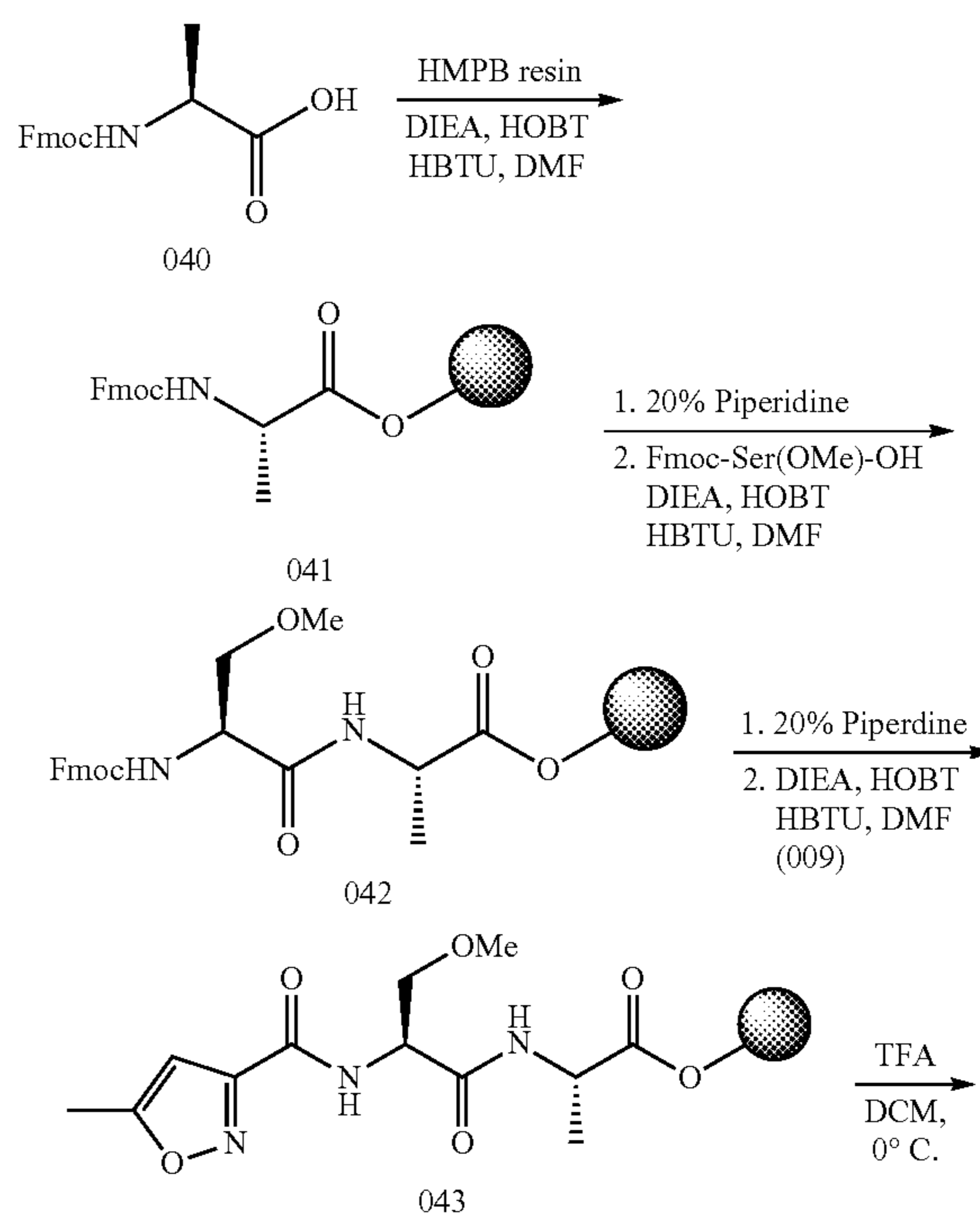
Scheme 6: Synthesis of Example 045 (approach A)
