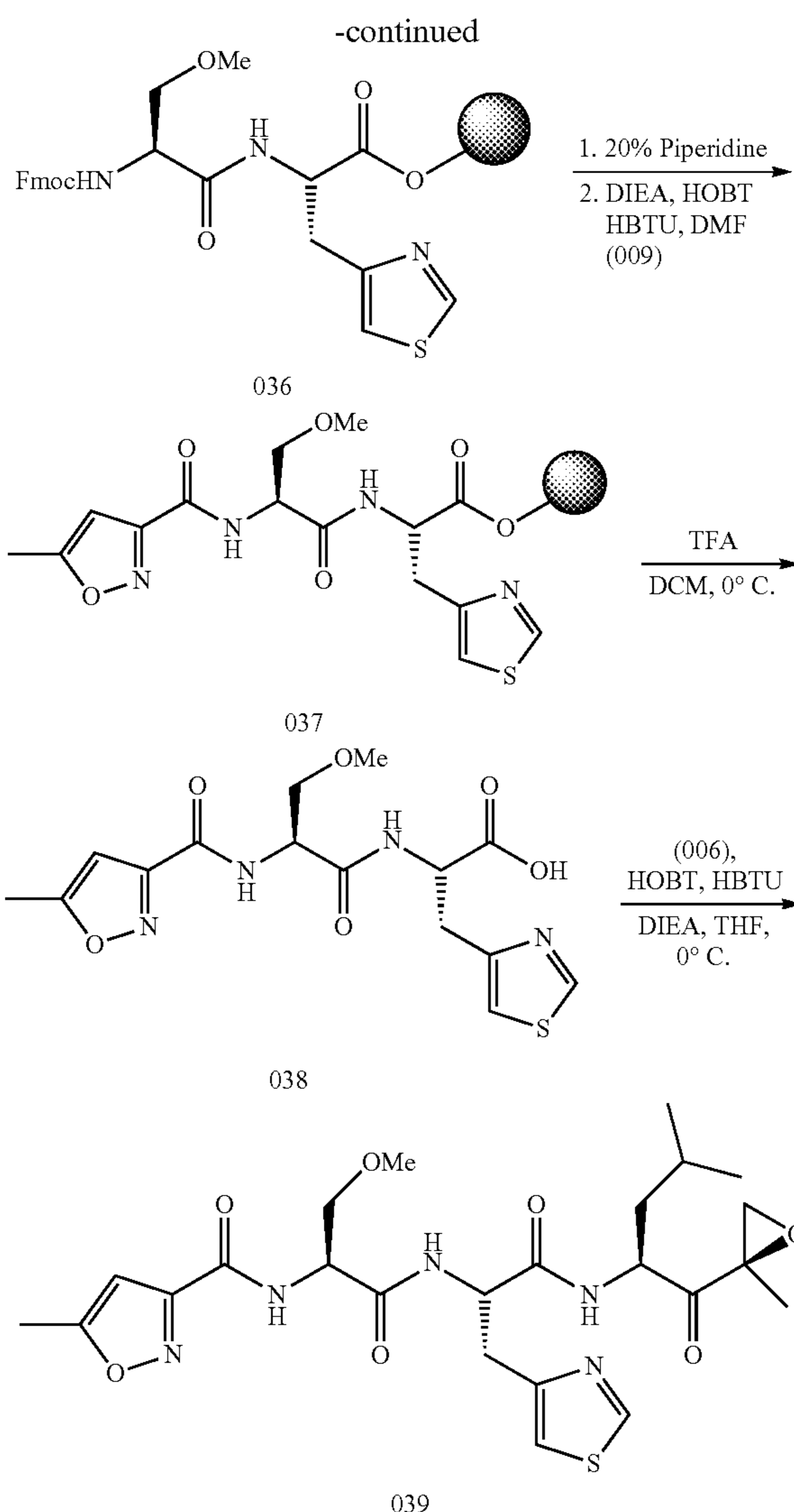
Scheme 6: Synthesis of Example 045 (approach A)
