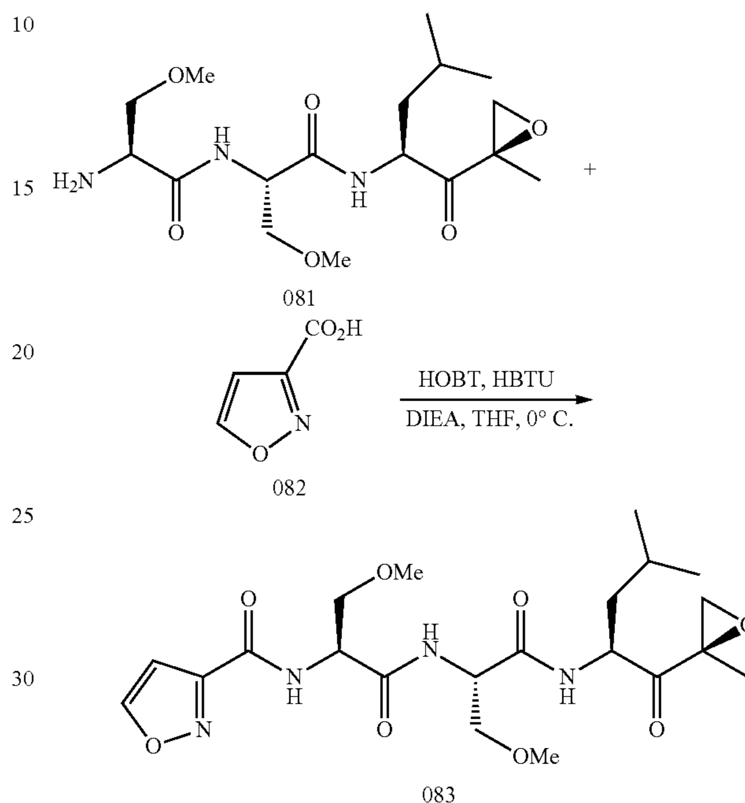
Scheme 13: Synthesis of Example 083
