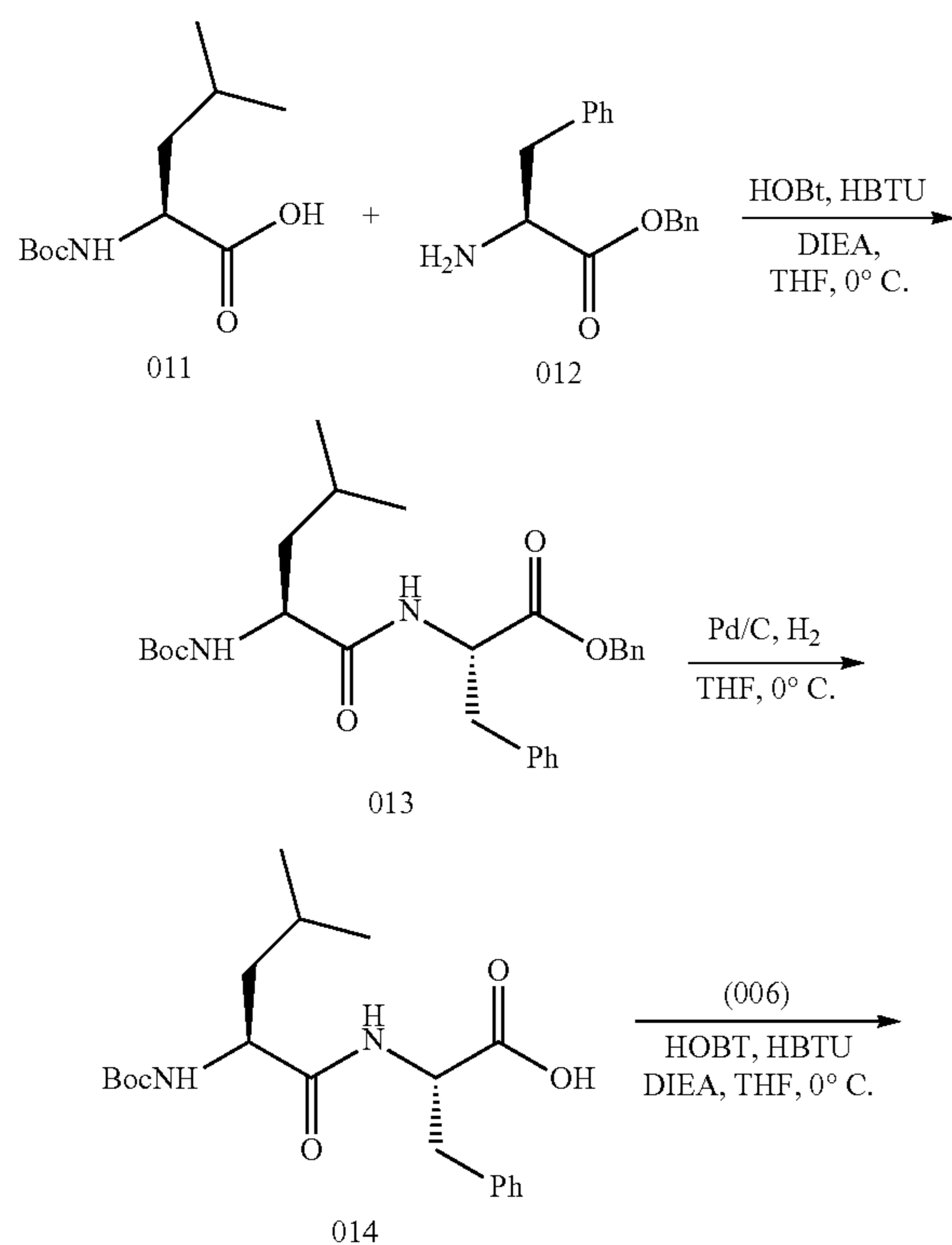
Scheme 2: Synthesis of Example 023
