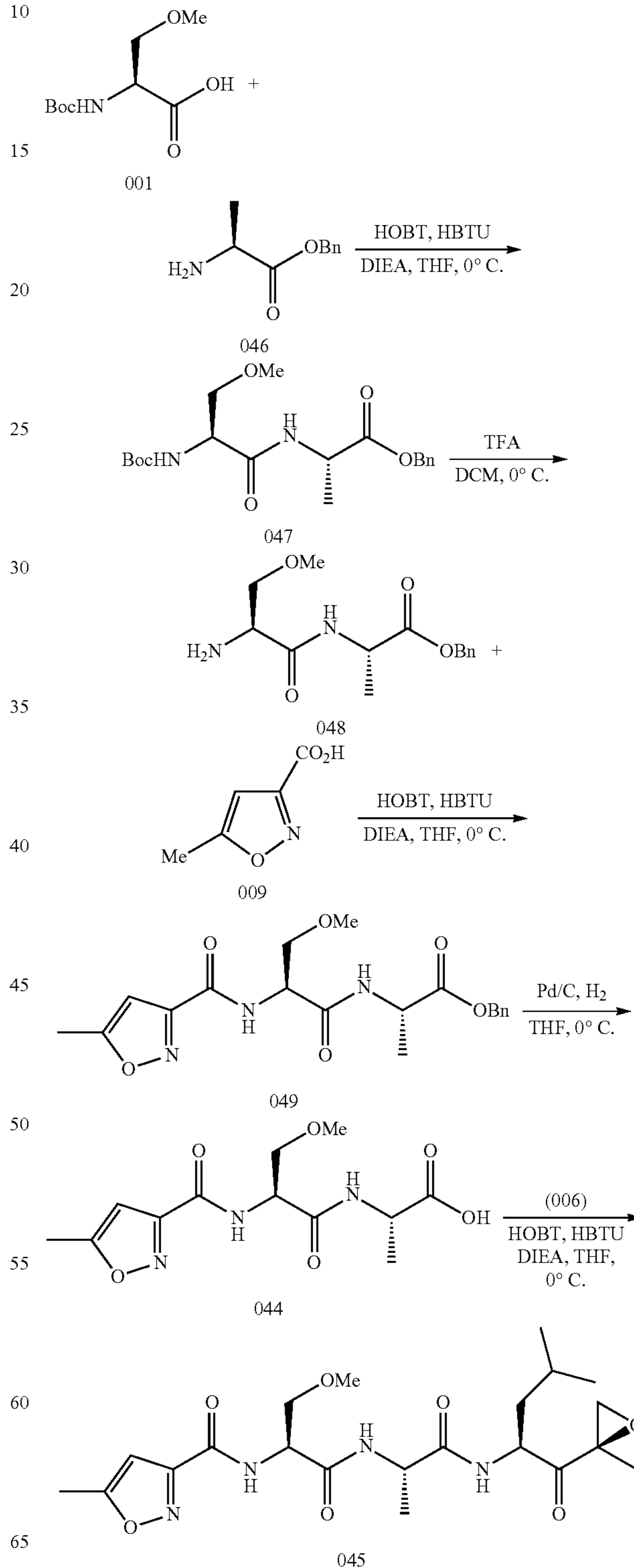
Scheme 7: Synthesis of Example 045 (approach B)
