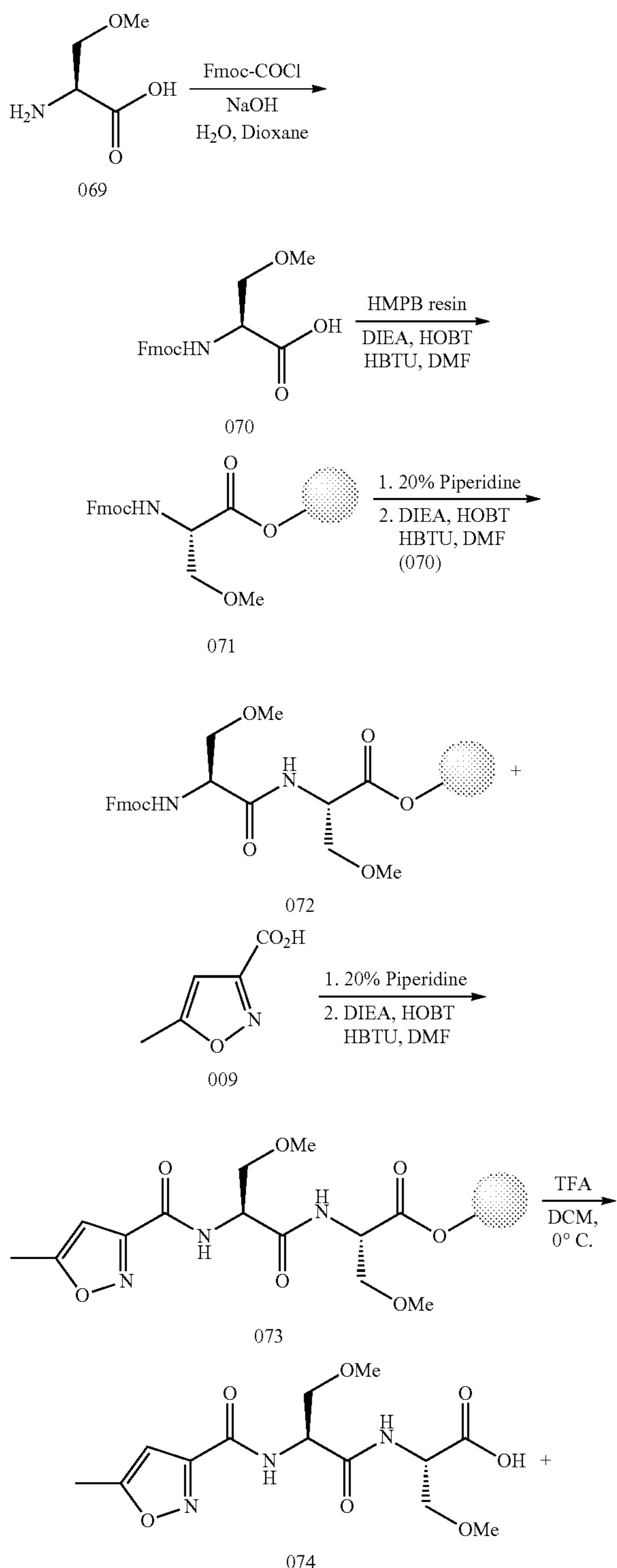
Scheme 11: Synthesis of Example 075 (approach A)
