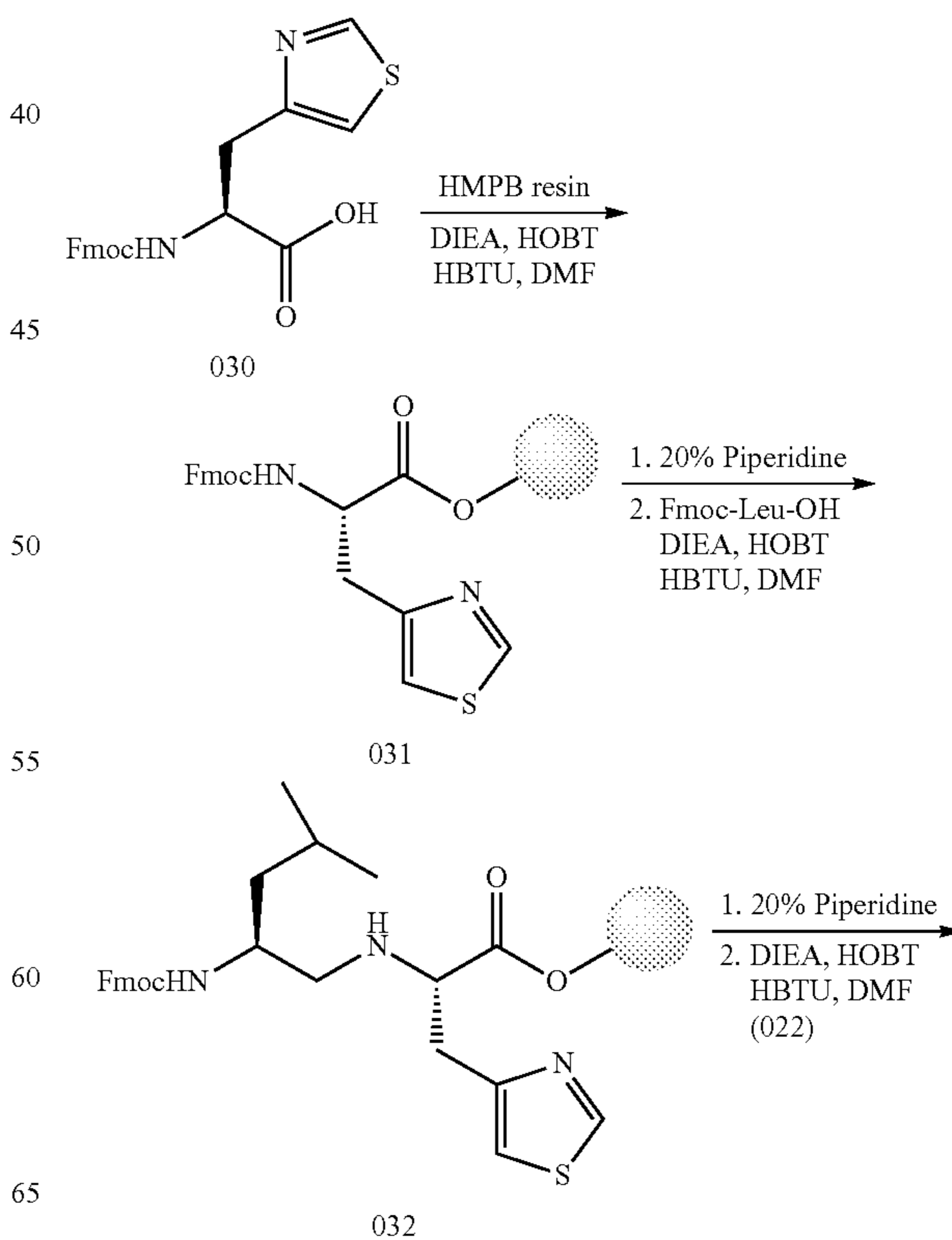
Scheme 4: Synthesis of Example 035
