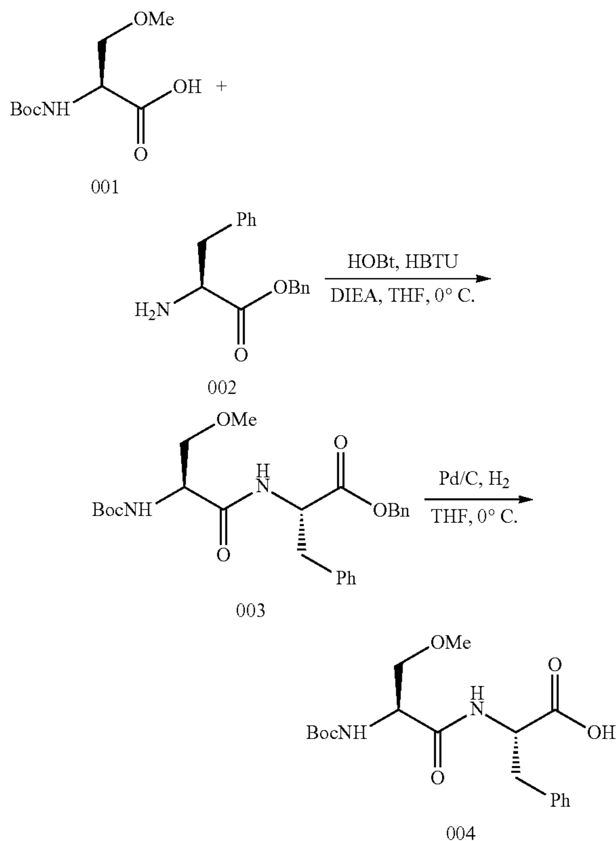
Scheme 1: Synthesis of Compound 010
