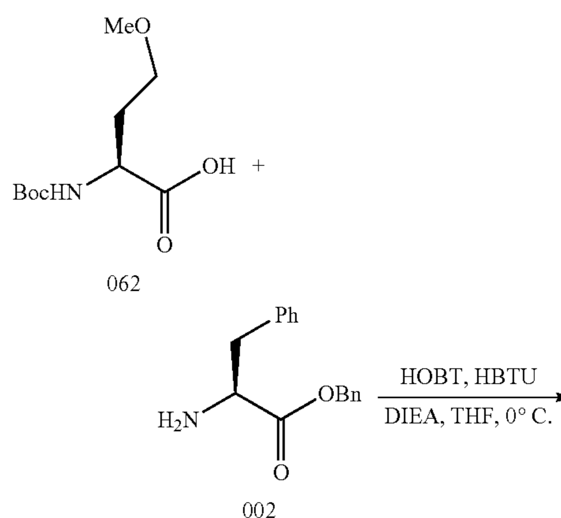
Scheme 10: Synthesis of Example 068
