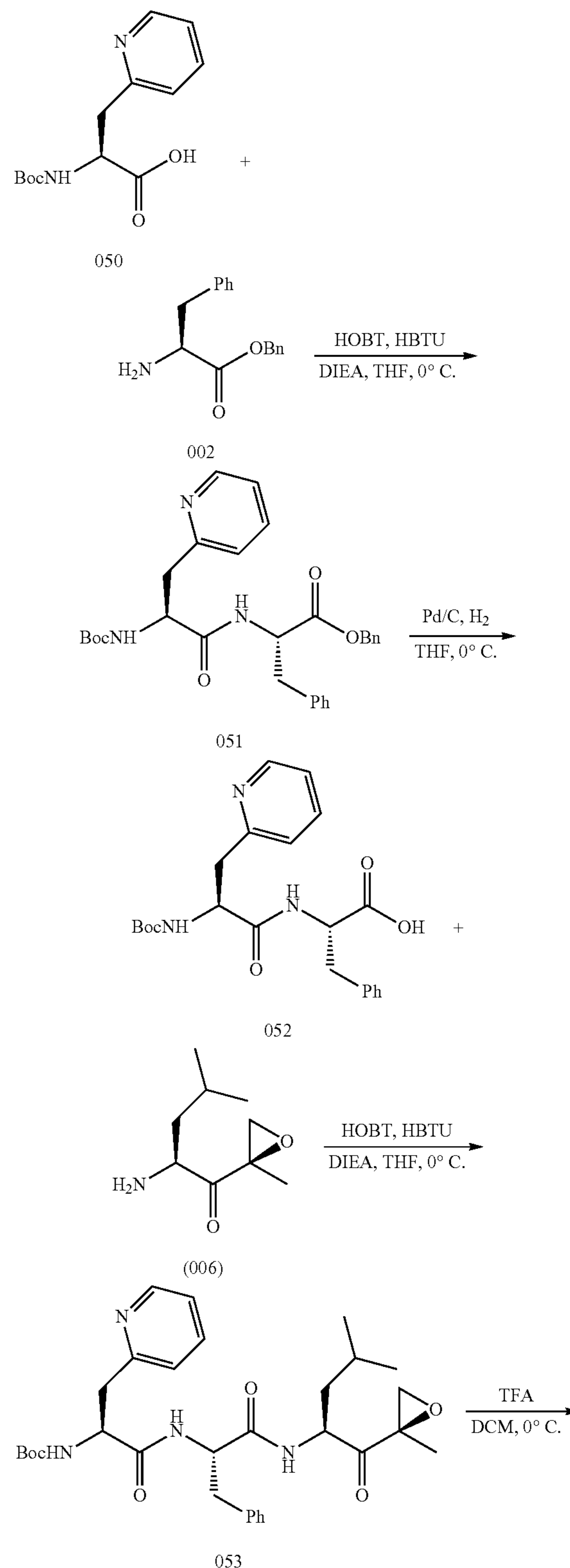
Scheme 8: Synthesis of Example 055
