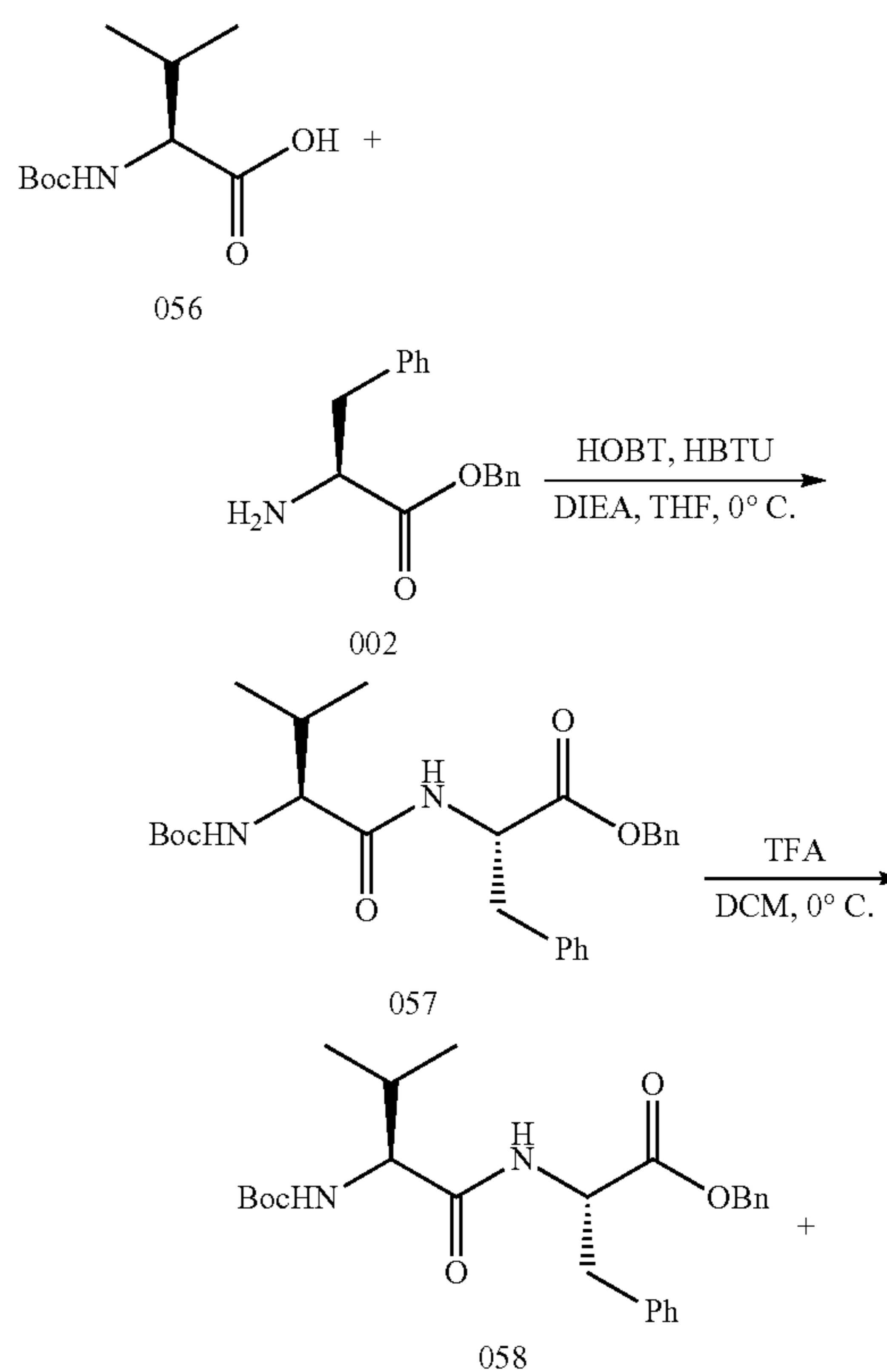
Scheme 9: Synthesis of Example 061
