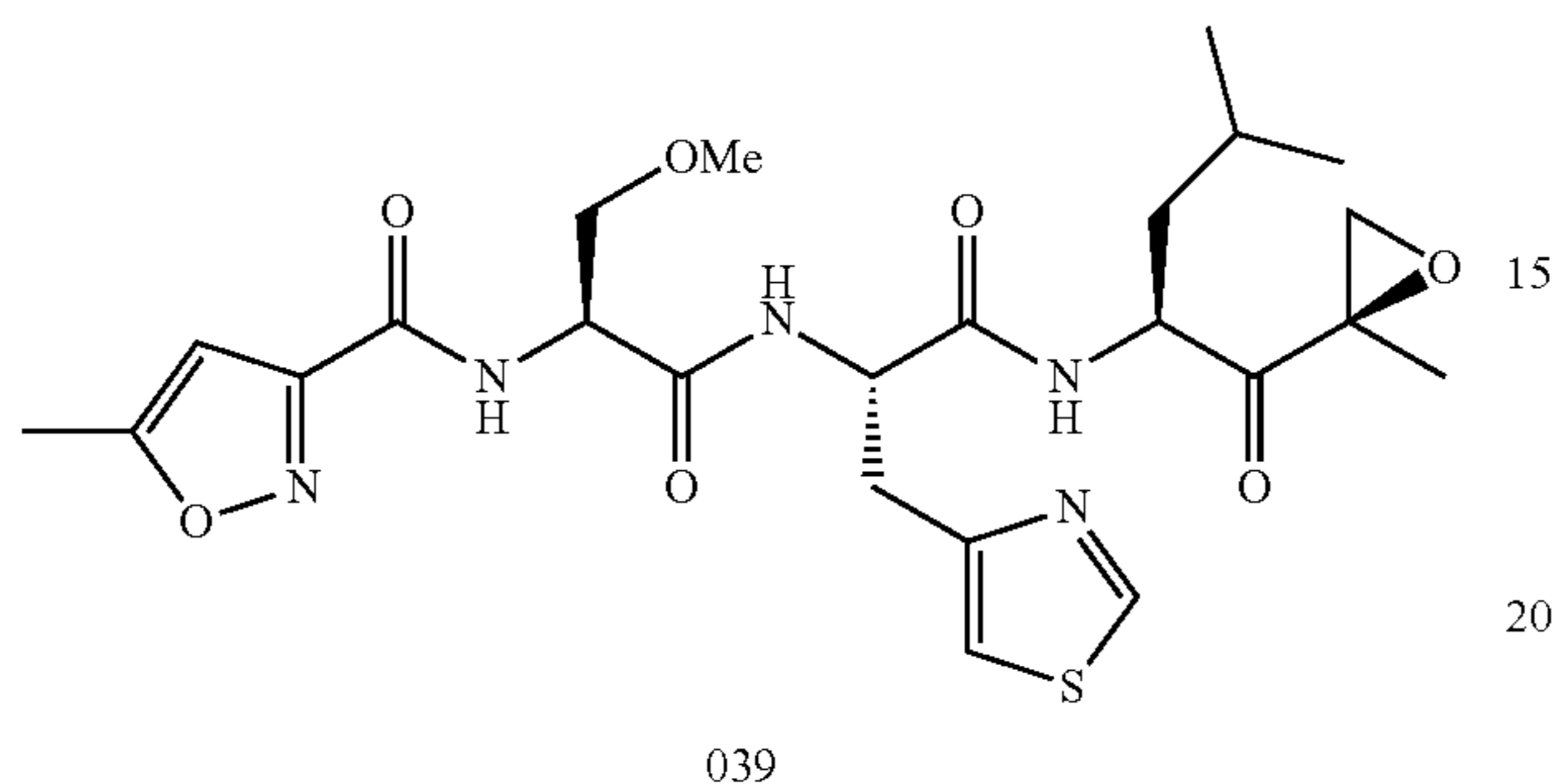
Scheme 6: Synthesis of Example 045 (approach A)
