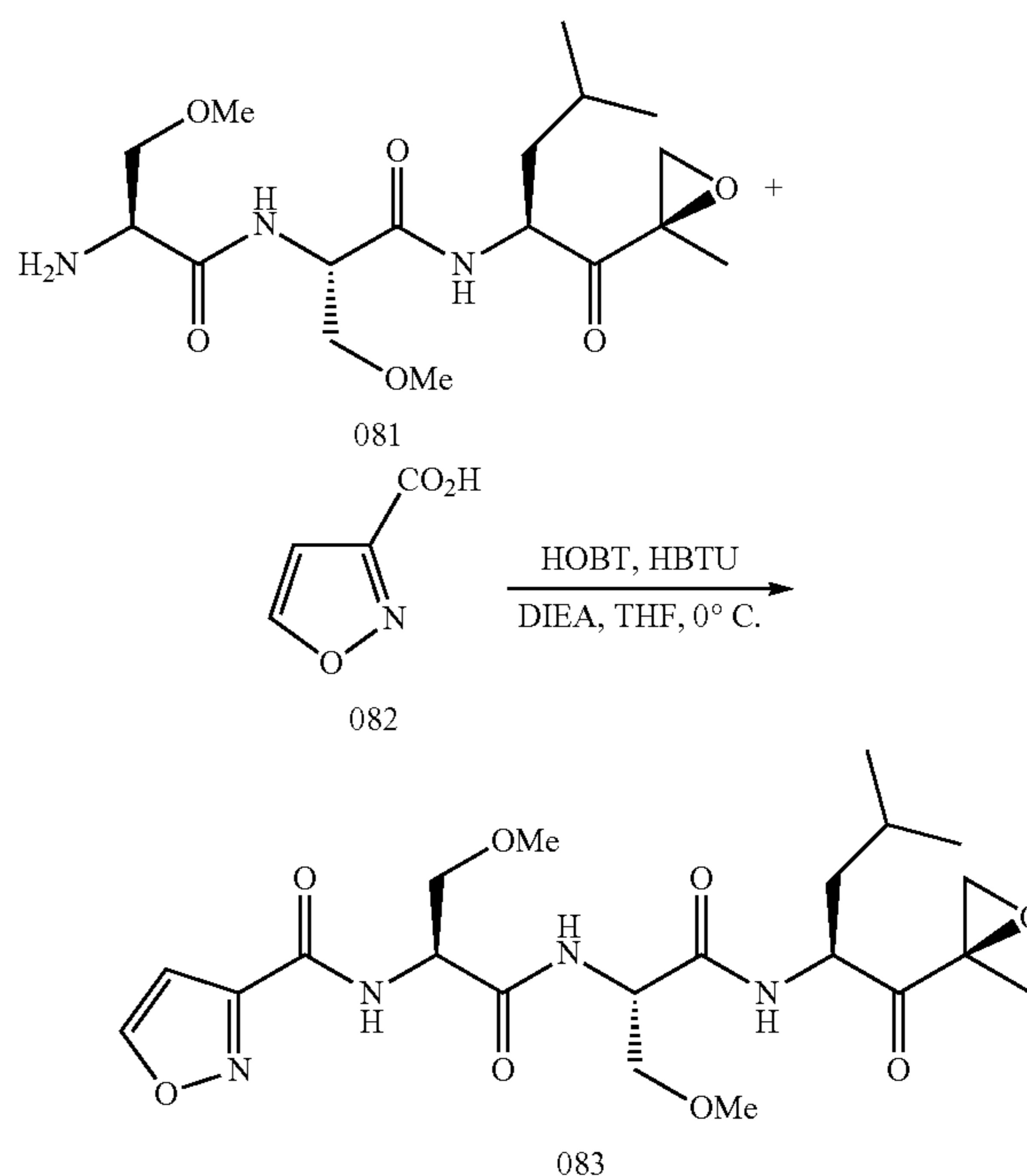
Scheme 13: Synthesis of Example 083
