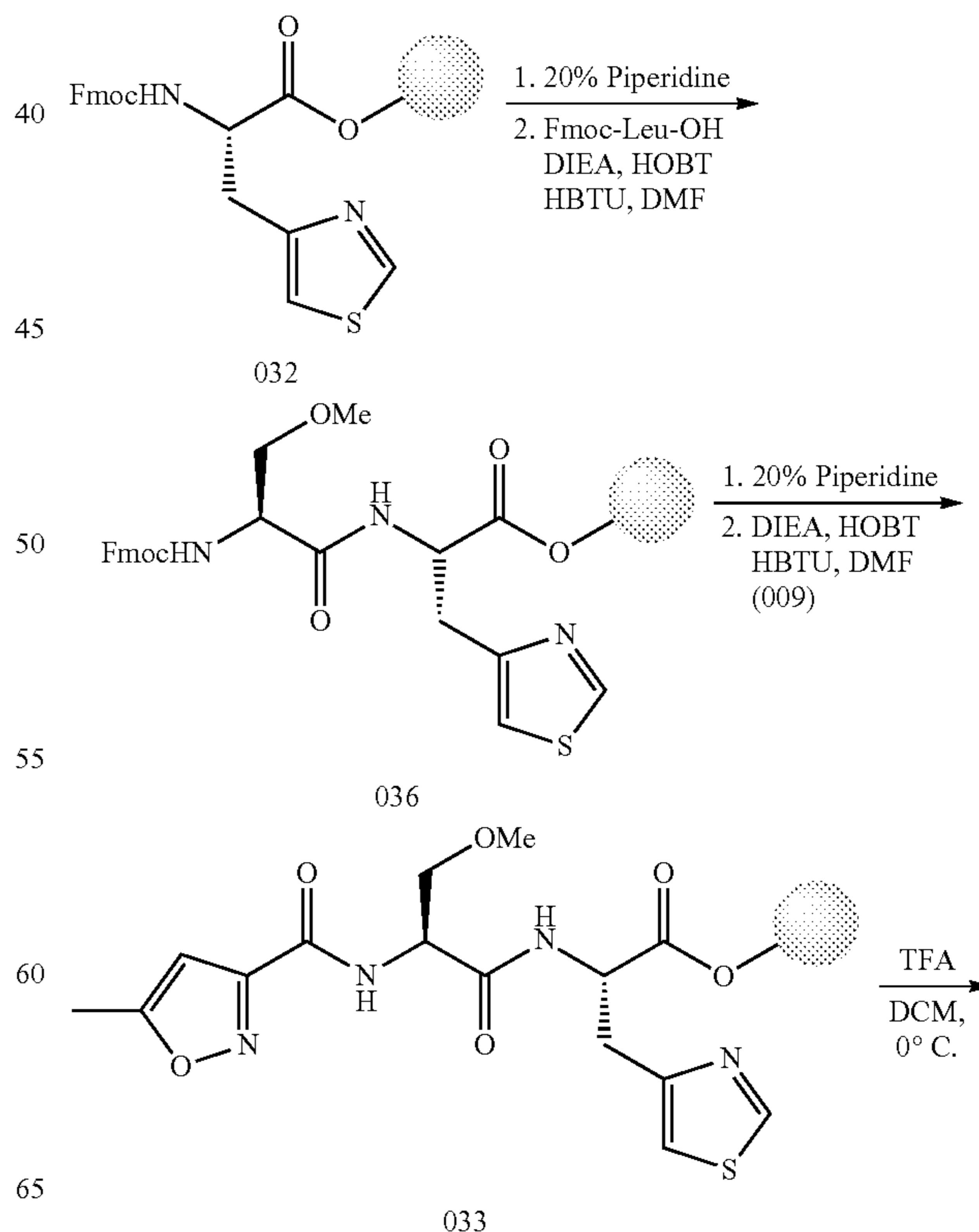
Scheme 5: Synthesis of Example 039
