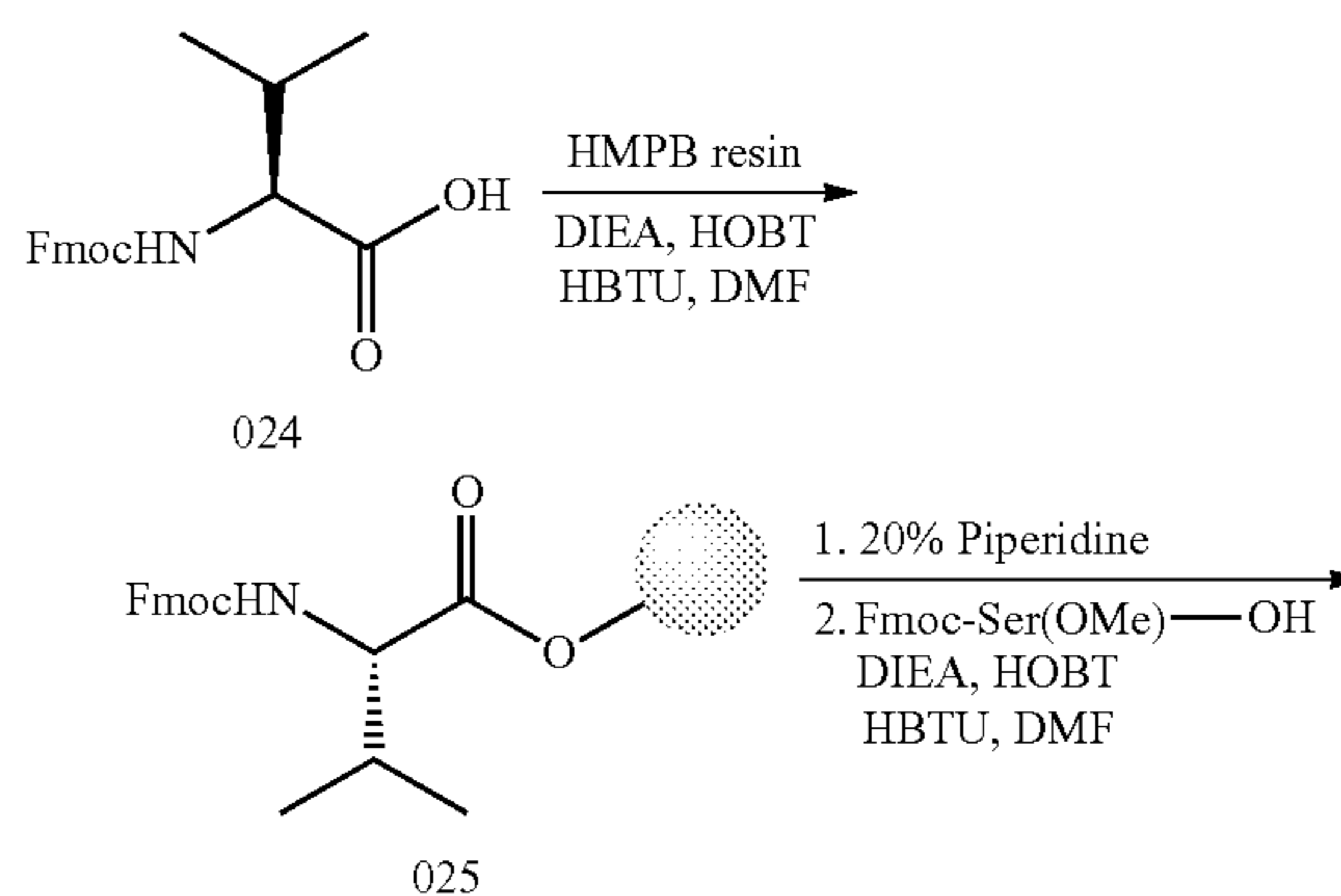
Scheme 3: Synthesis of Example 029
