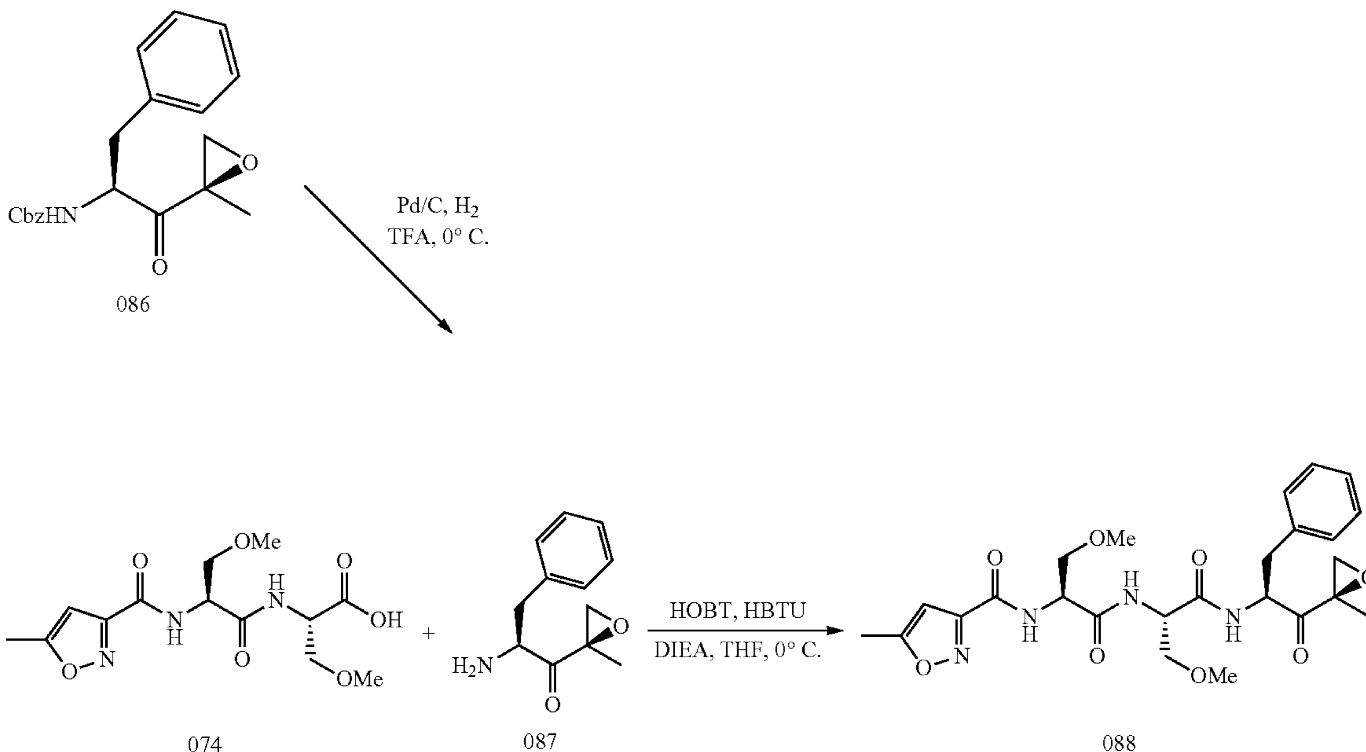
Scheme 15: Synthesis of Example 088
