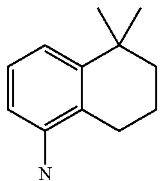
5,5-dimethyl-5,6,7,8-tetrahydronaphthalen-1-amine
