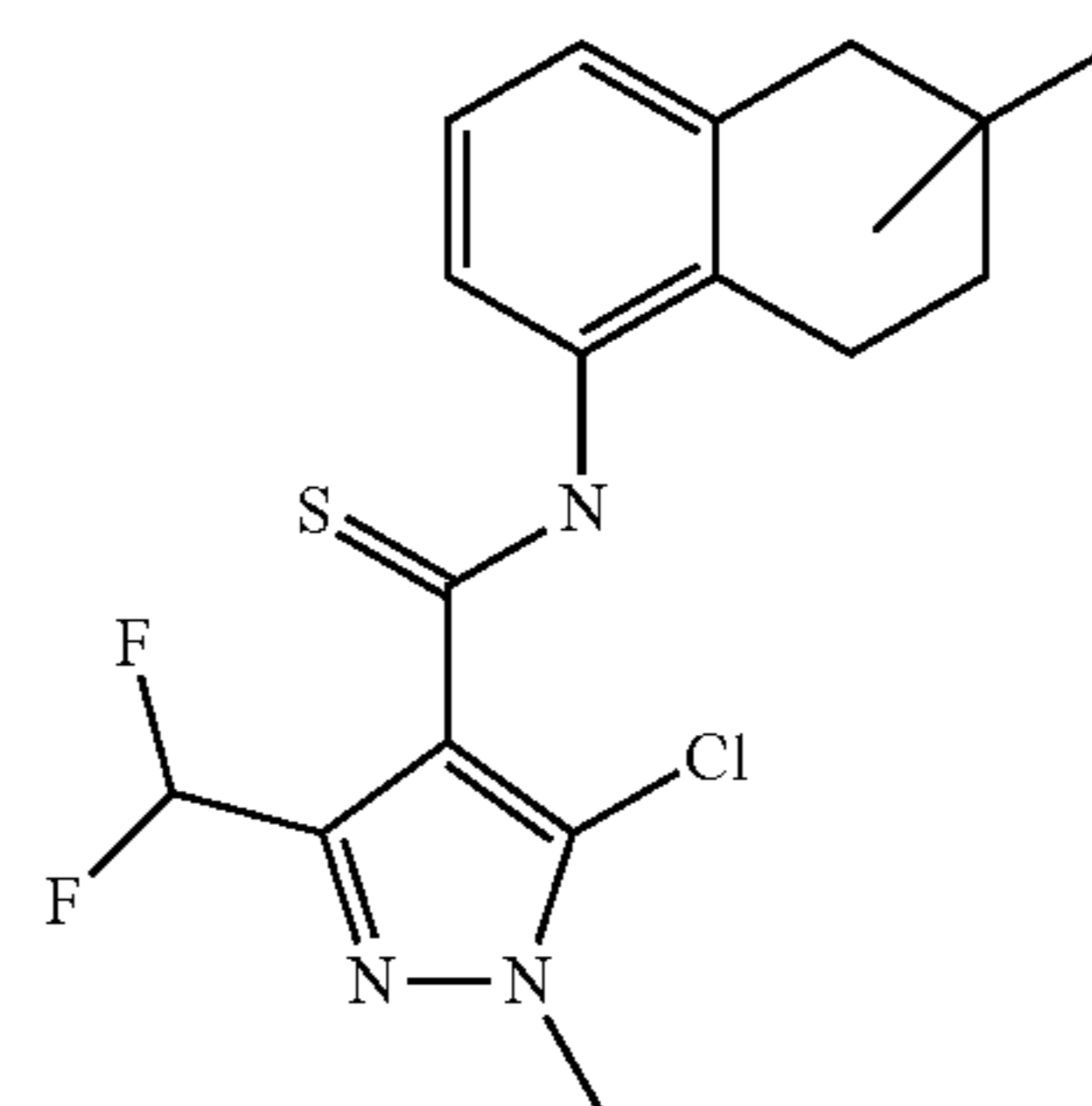
5-chloro-3-(difluoromethyl)-N-(6,6-dimethyl-5,6,7,8-tetrahydronaphthalen-1-yl)-1-methyl-1H-pyrazole-4-carbothioamide
