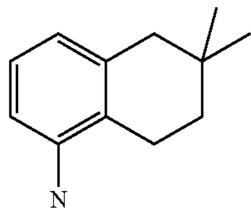
6,6-dimethyl-5,6,7,8-tetrahydronaphthalen-1-amine
