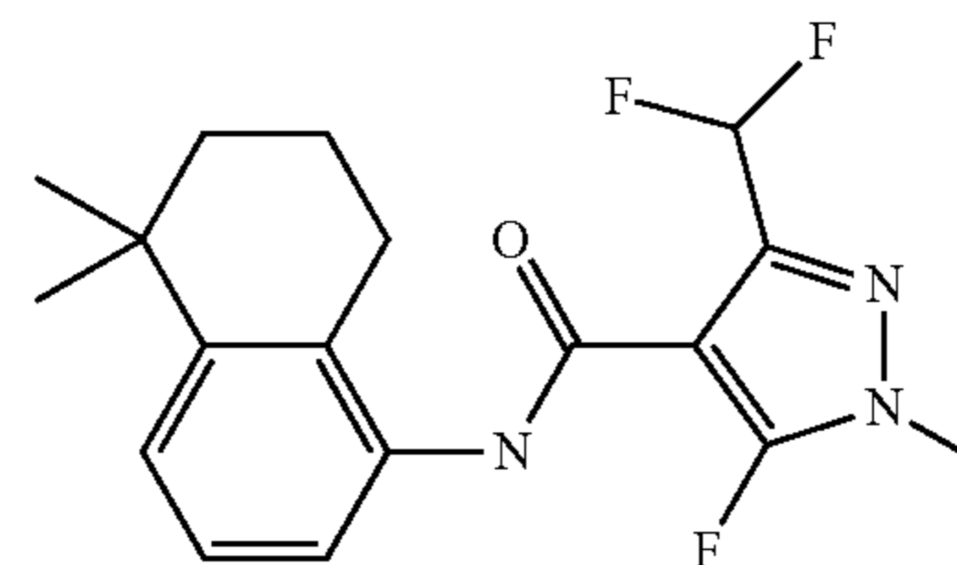
5-fluoro-3-(difluoromethyl)-N-(5,5-dimethyl-5,6,7,8-tetrahydronaphthalen-1-yl)-1-methyl-1H-pyrazole-4-carboxamide
