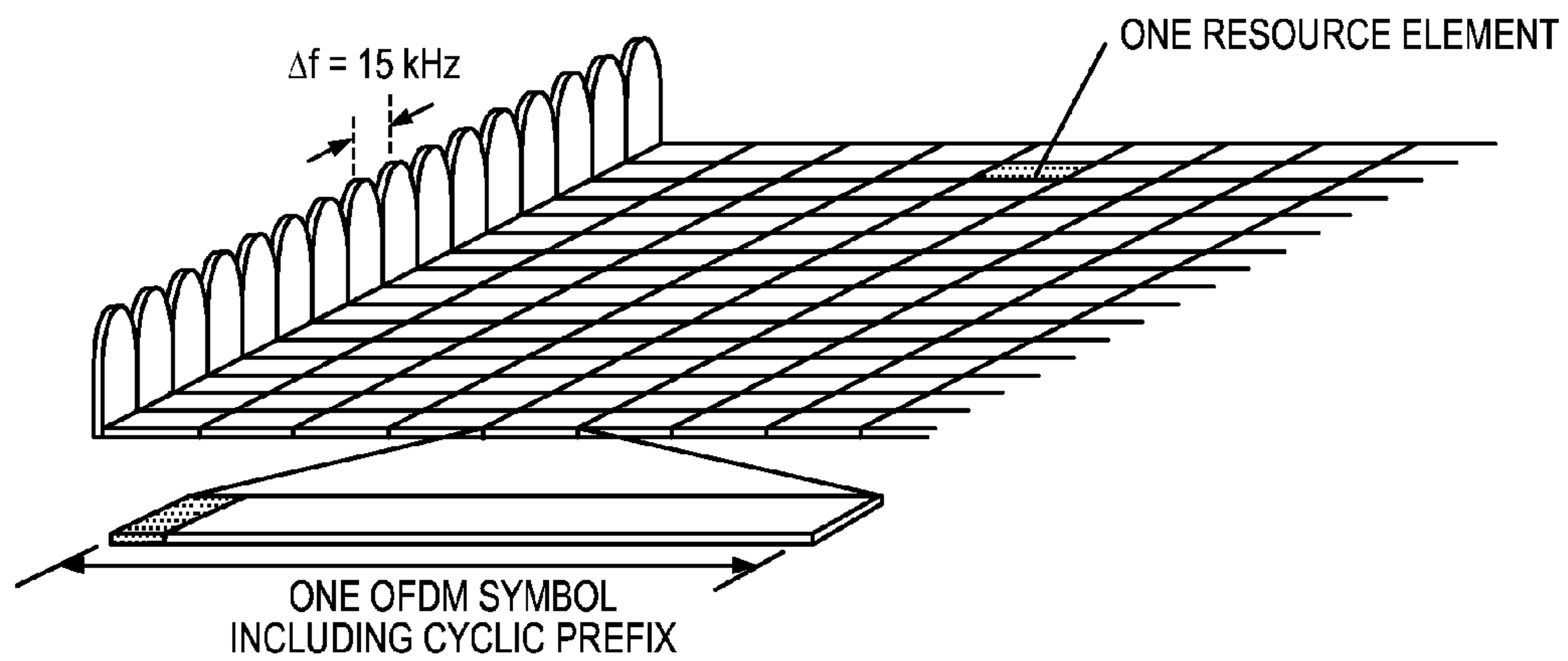
FIG. 1 (PRIOR ART)
