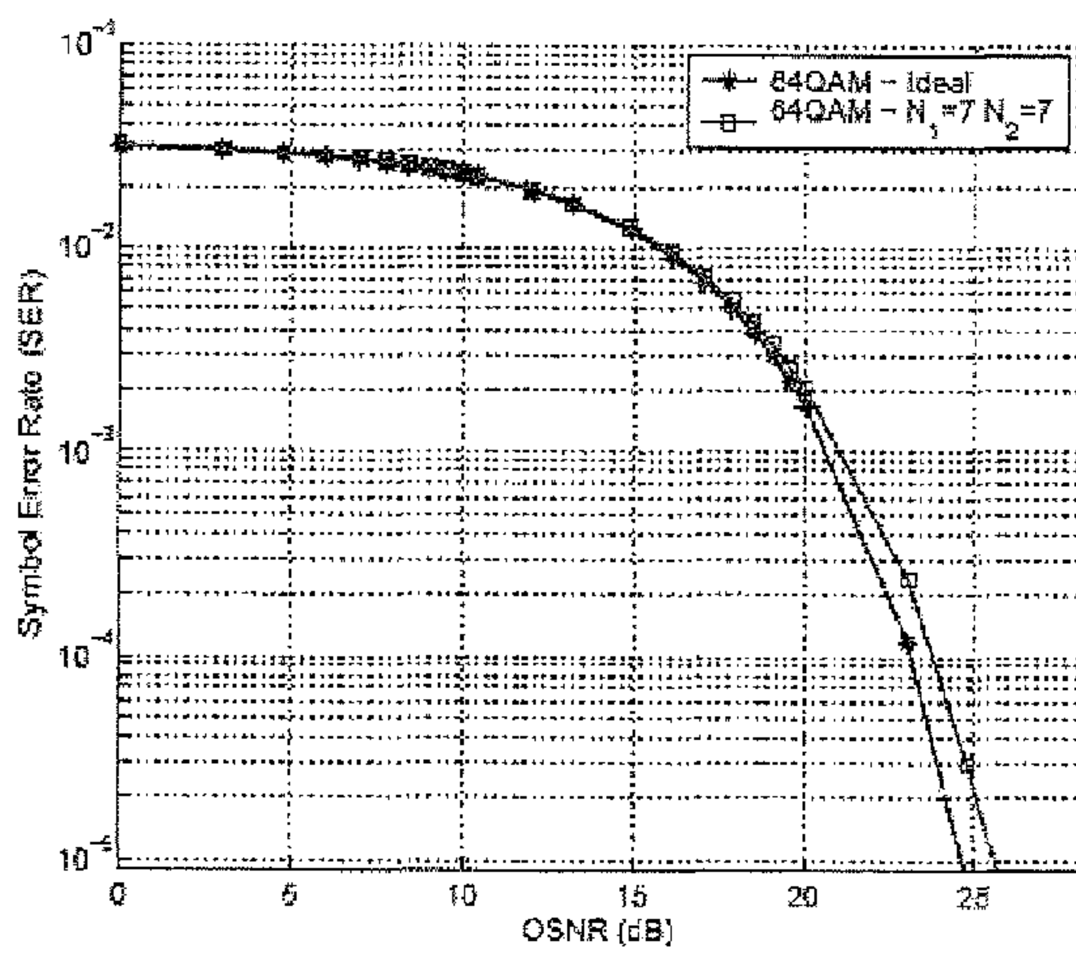
(a) 64-QAM
