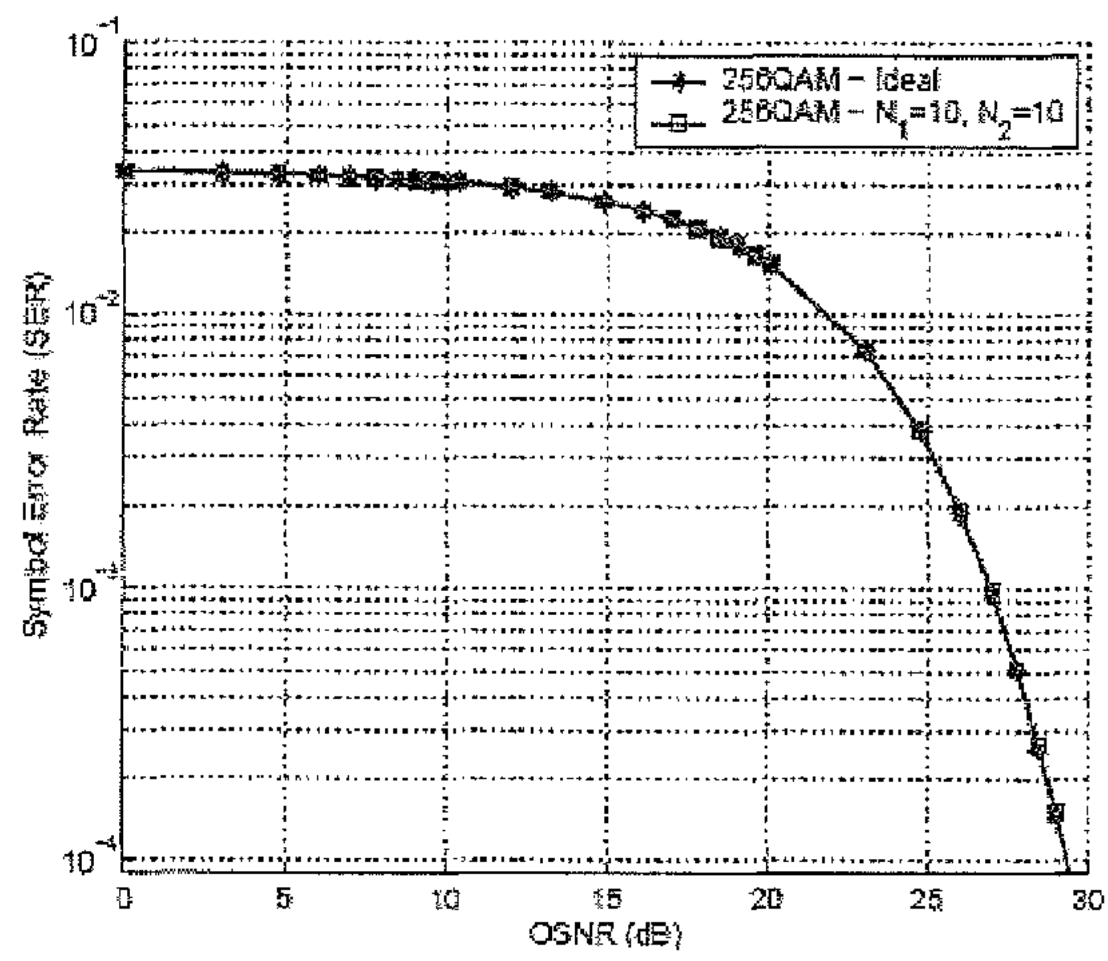
(b) 256-QAM
