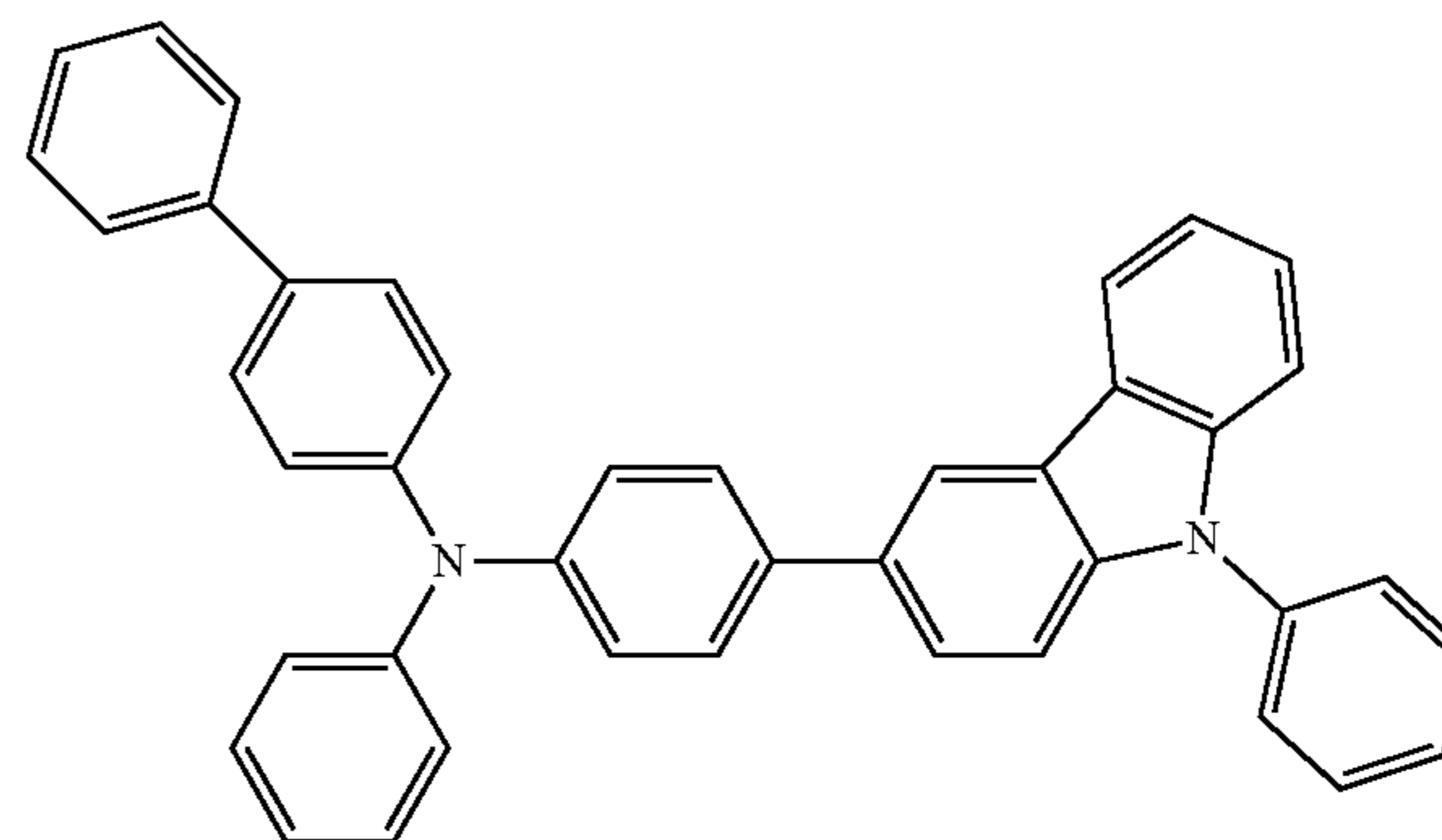
PCBA1BP
