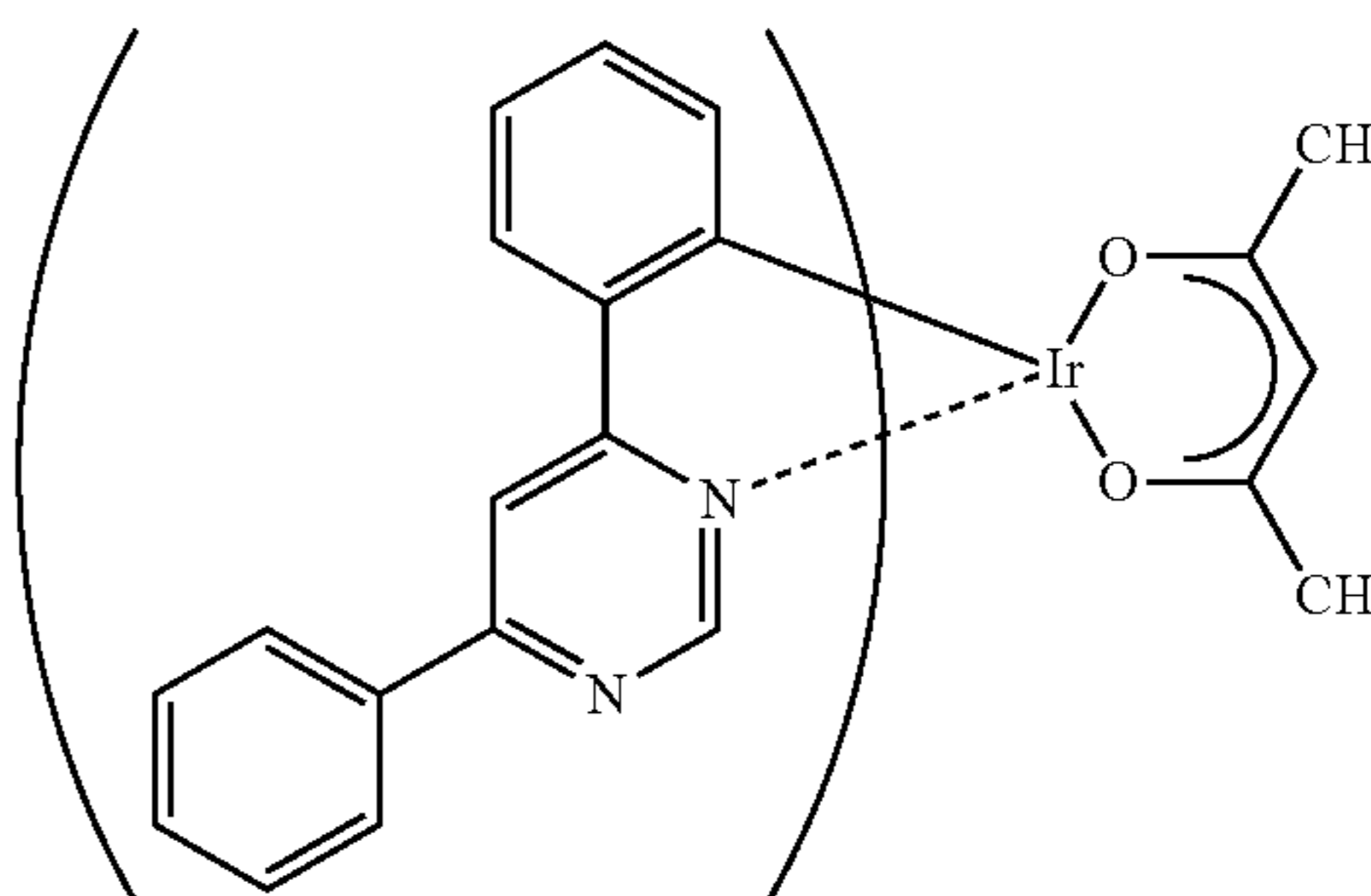
[Ir(dppm) 2 (acac)]
