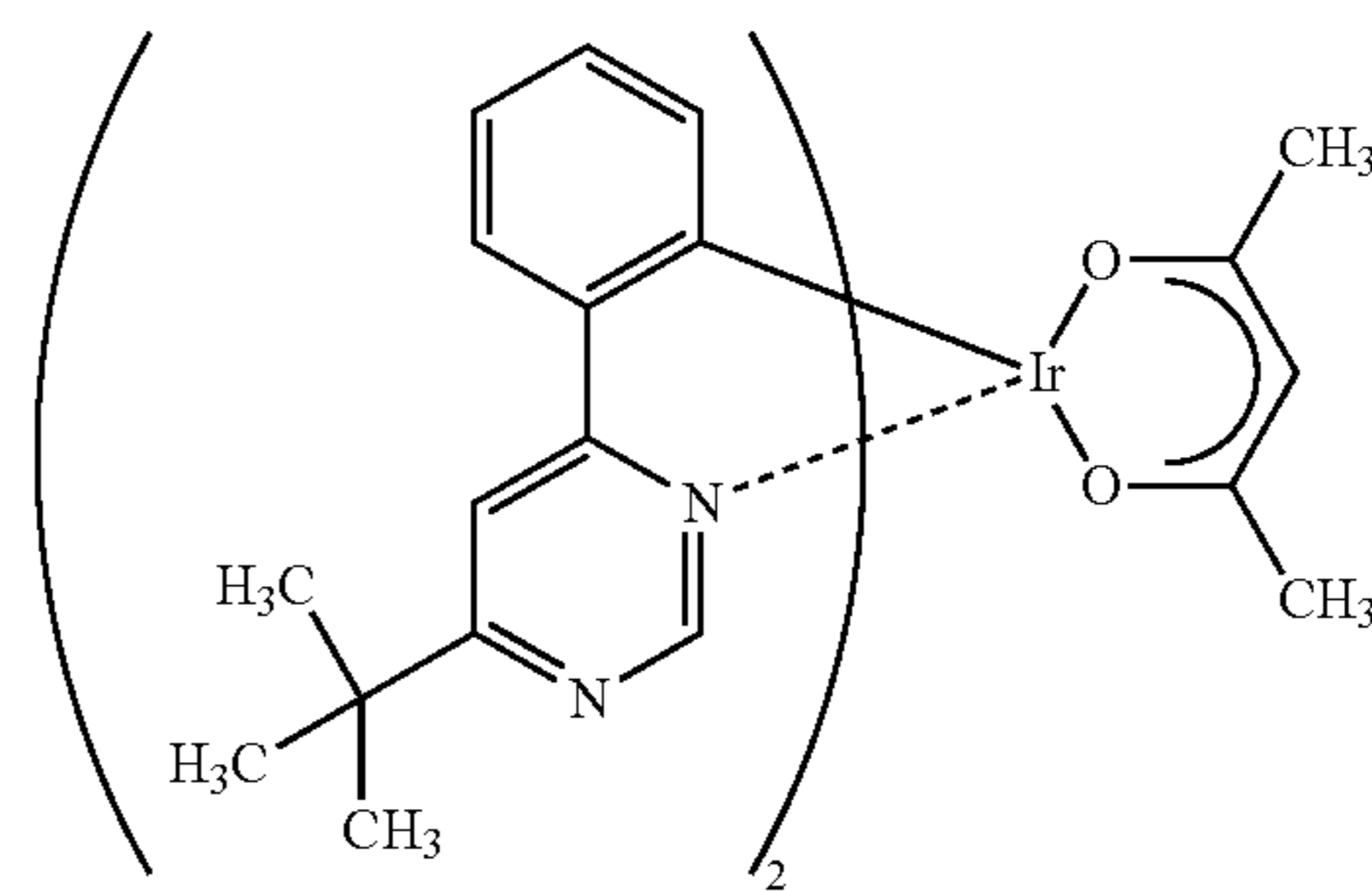
[Ir(tBuppm) 2 (acac)]
