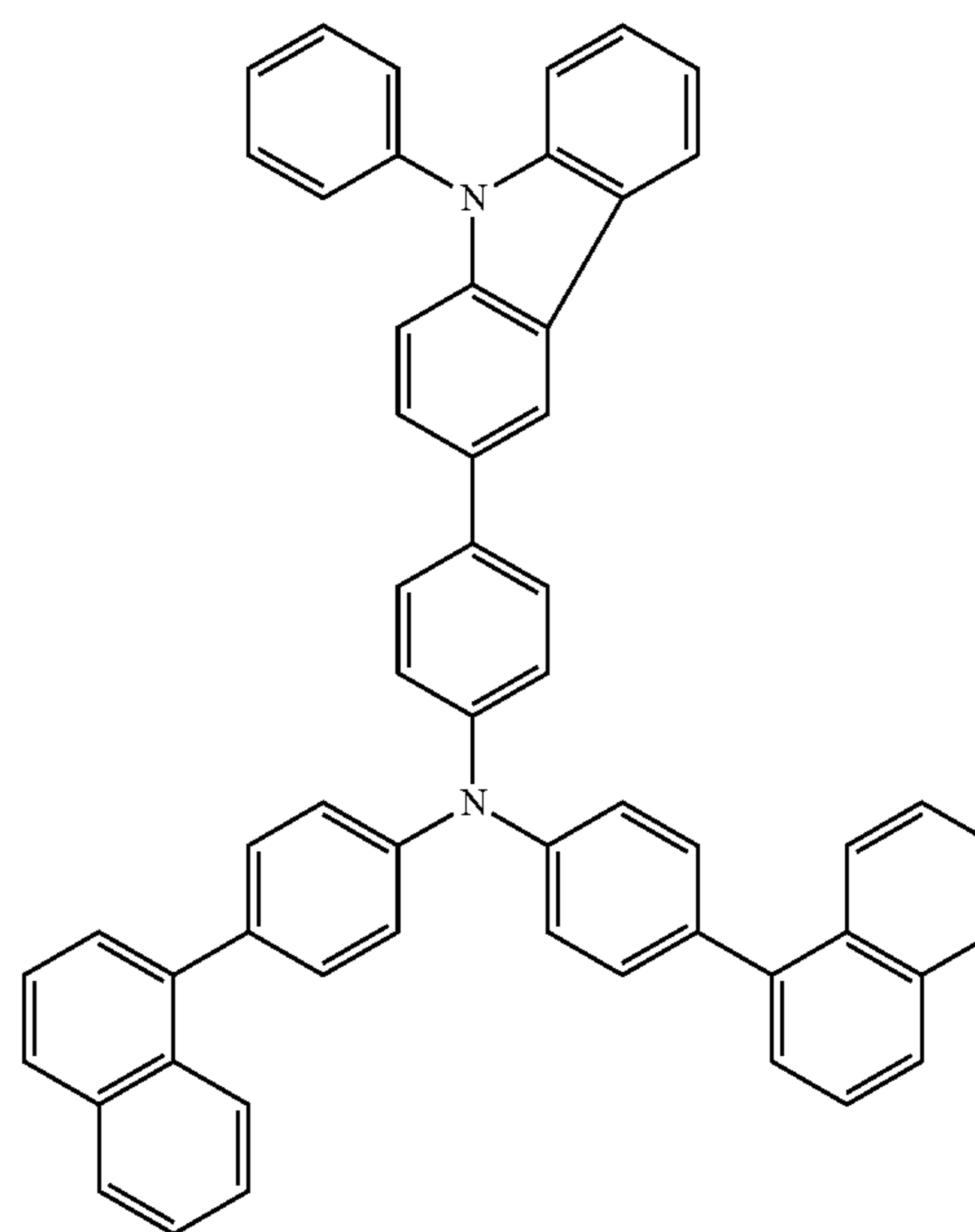
PCBNBB
