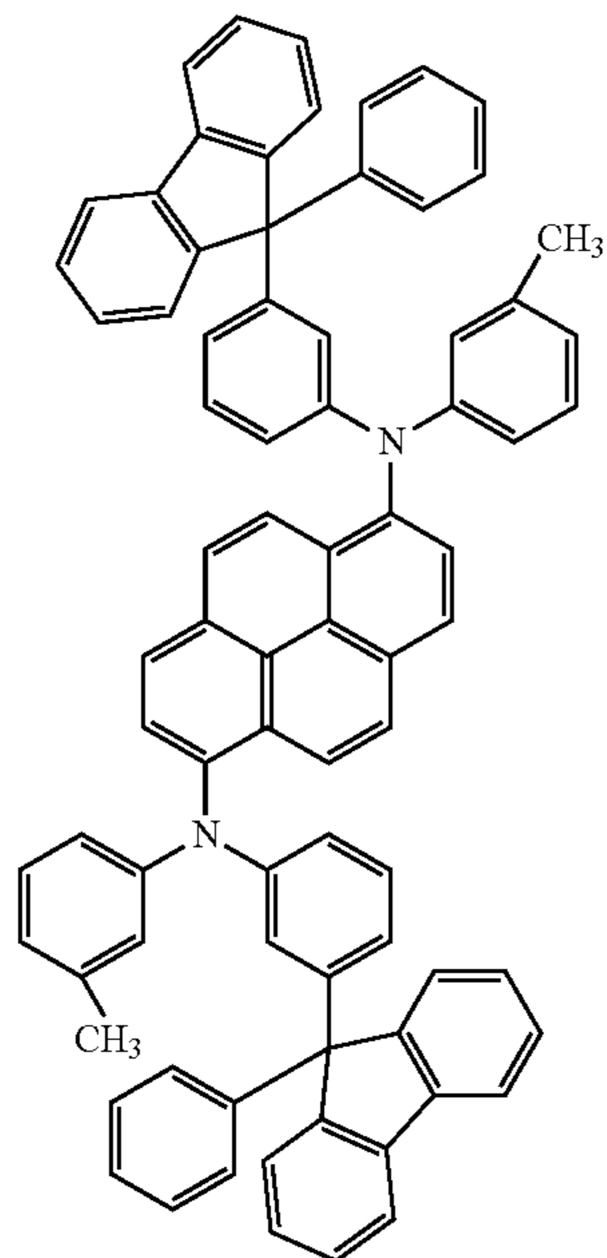
1,6mMemFLPAPrn
