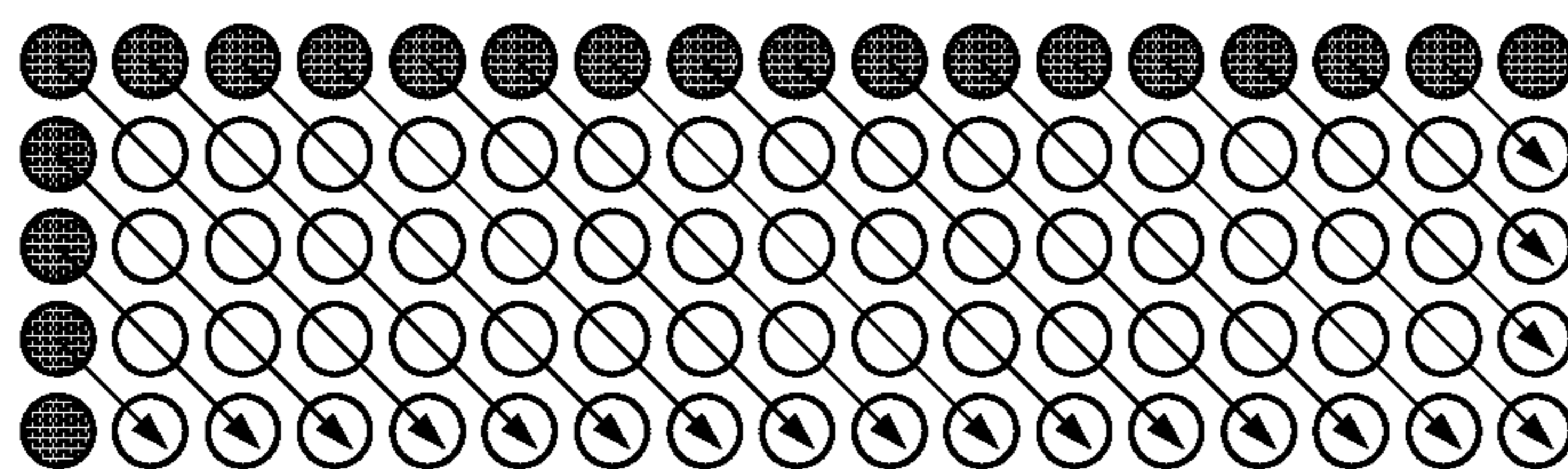
Prediction mode 4
