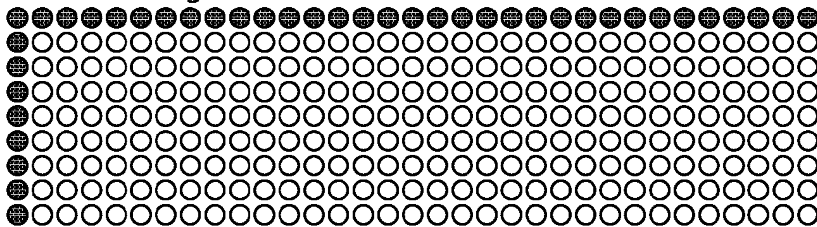
Prediction mode 2
