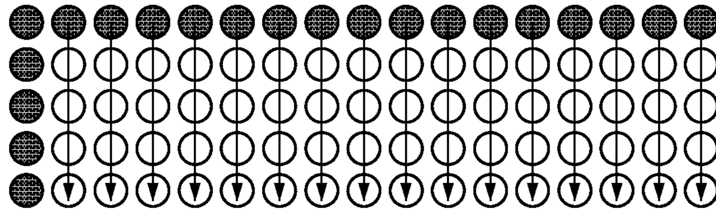
Prediction mode 0
