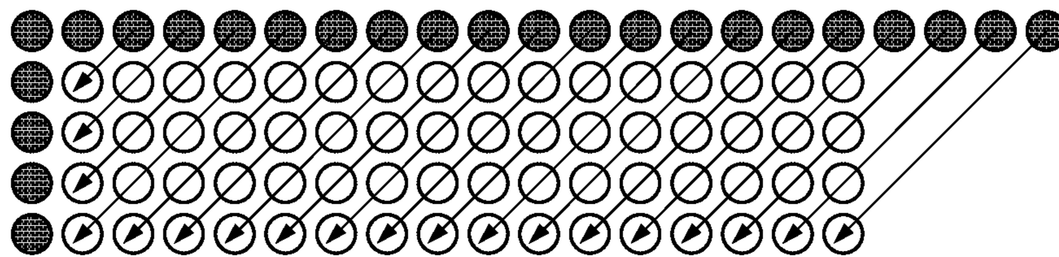
Prediction mode 3
