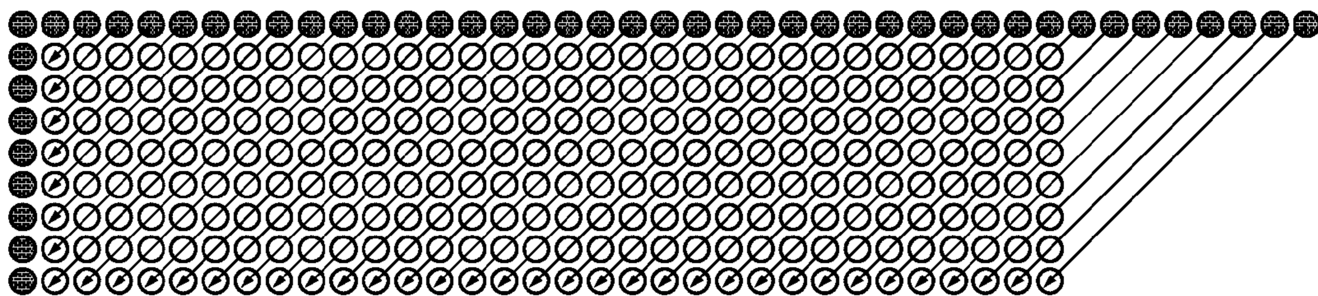
Prediction mode 3
