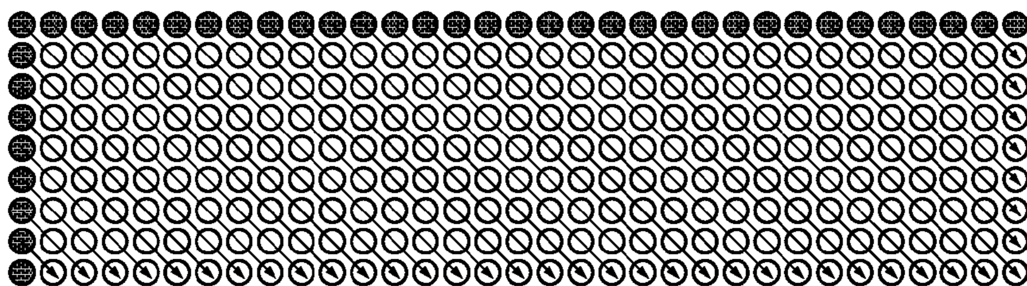
Prediction mode 4
