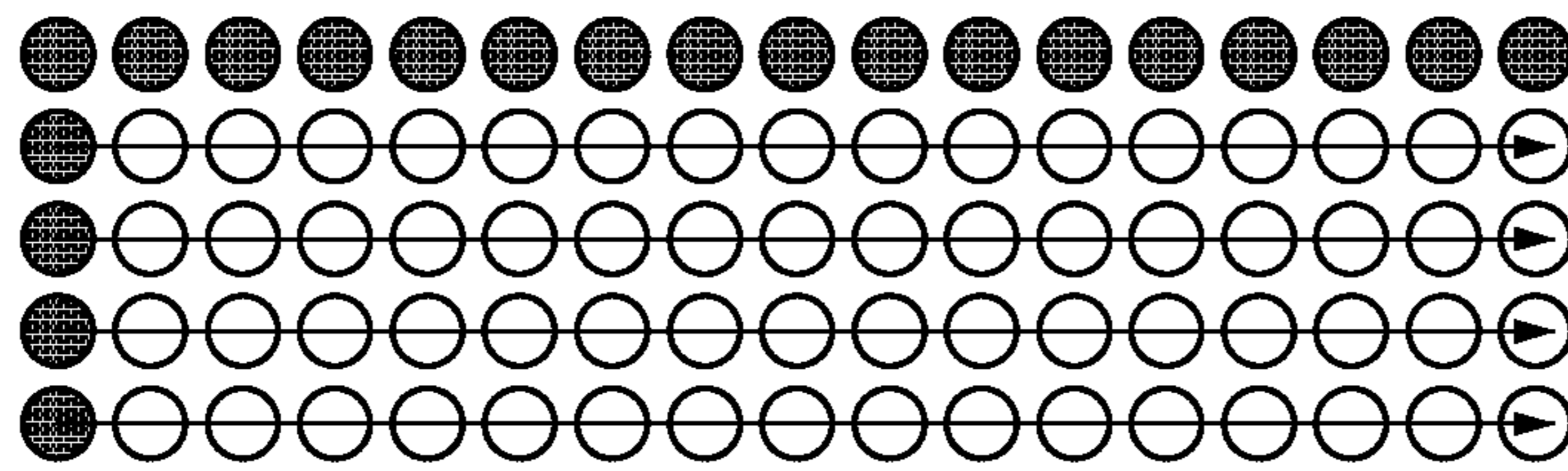
Prediction mode 1
