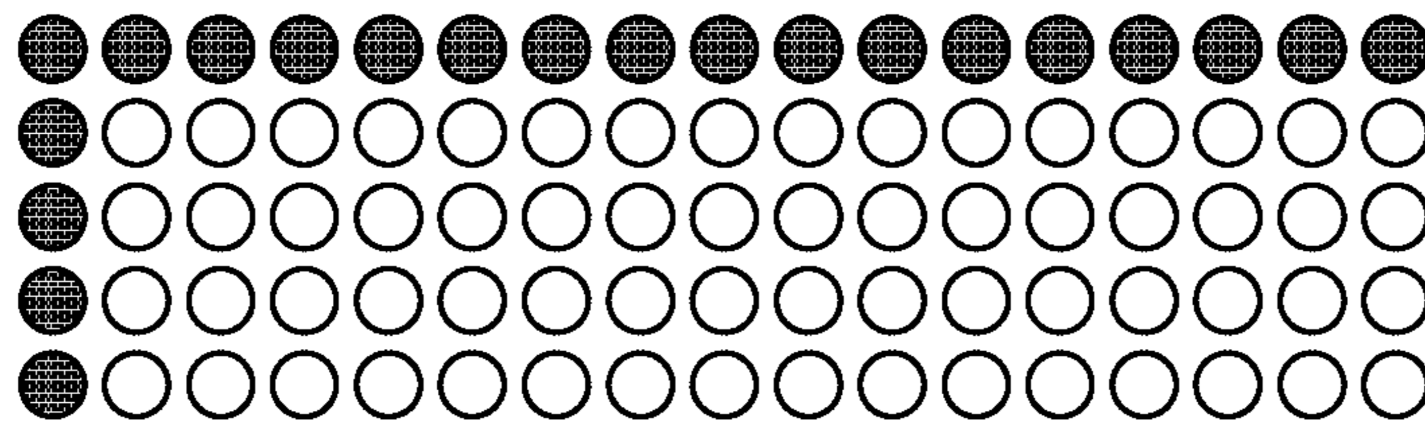
Prediction mode 2
