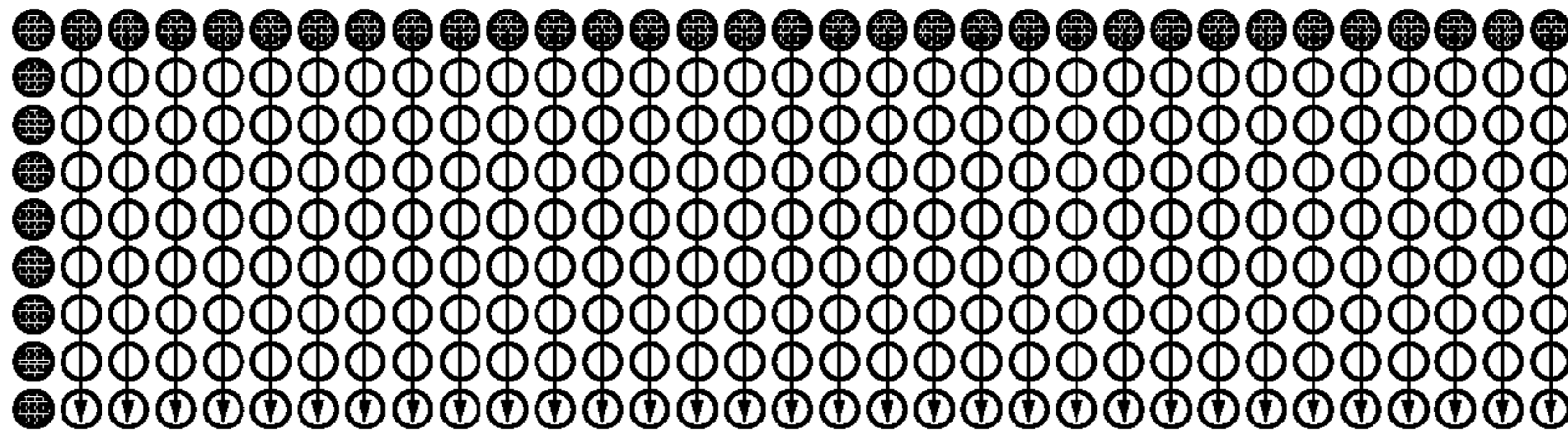
Prediction mode 0
