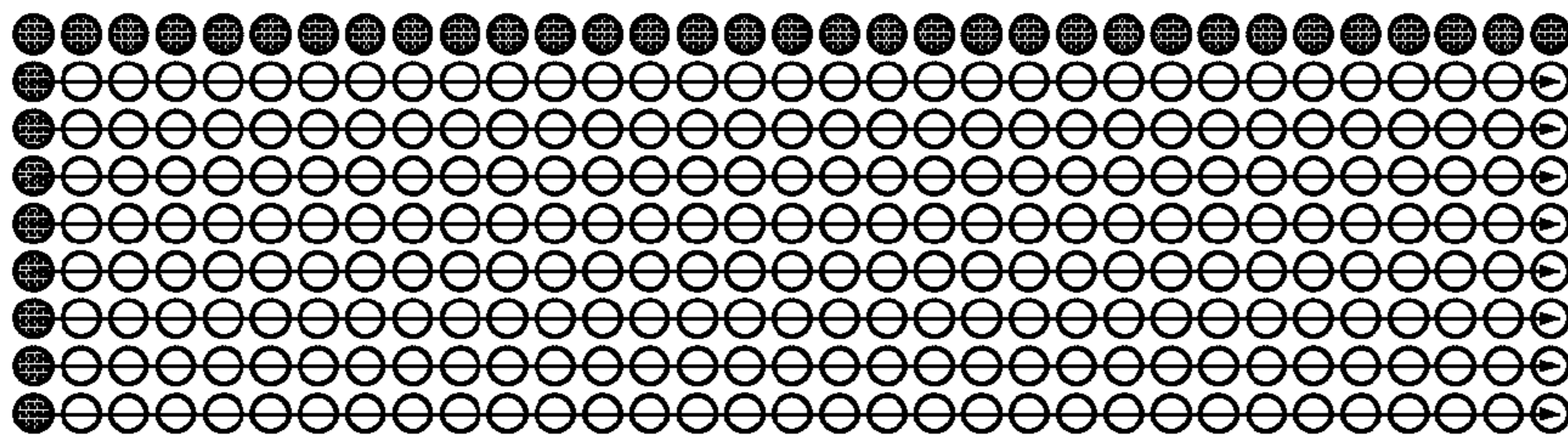
Prediction mode 1
