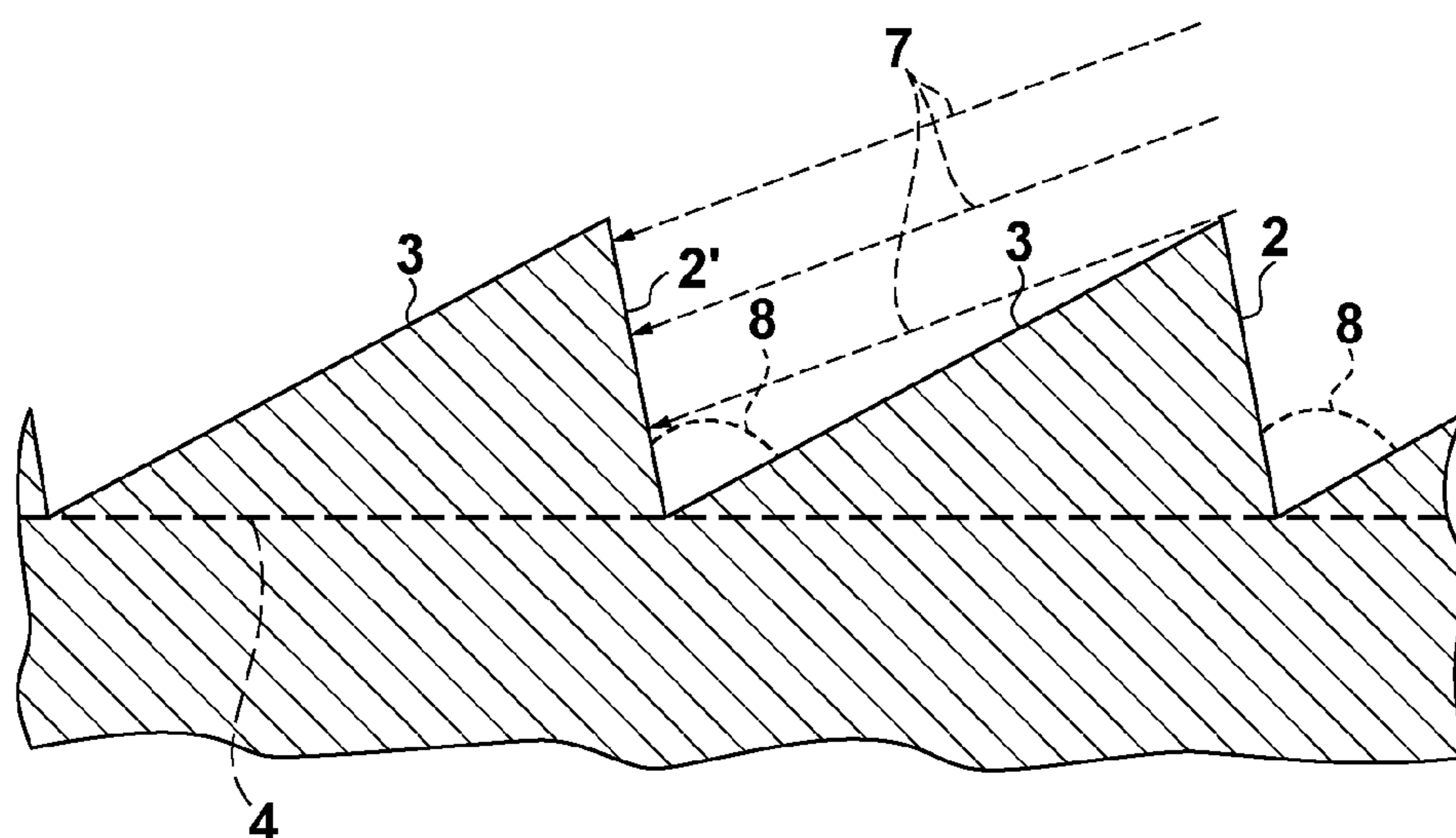
FIG. 2 PRIOR ART
