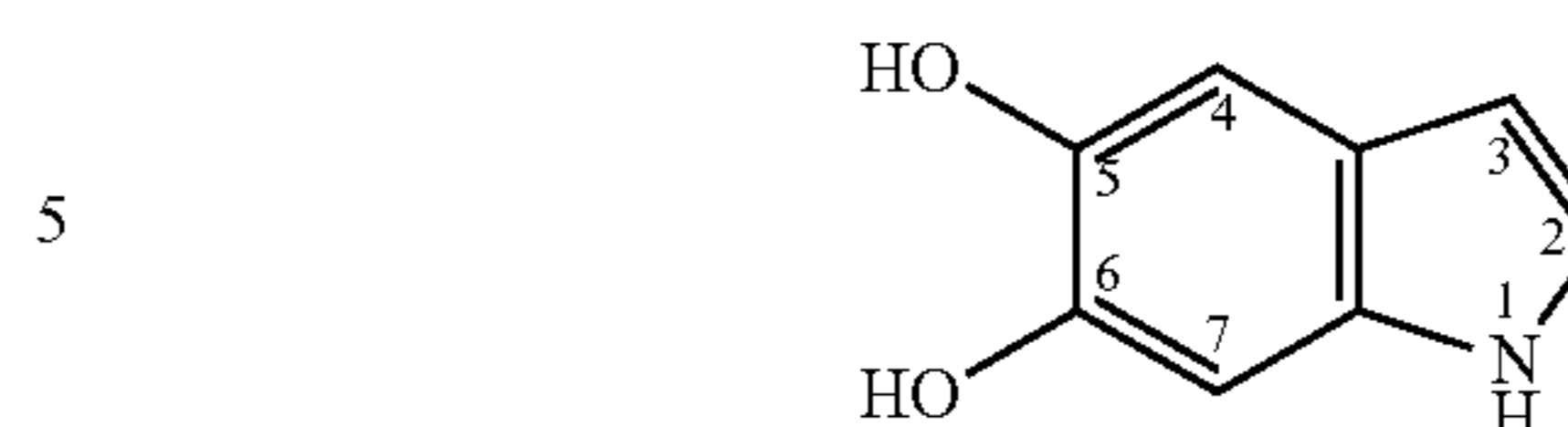
Scheme 2: Chemical structure of 5,6-dihydroxyindole.
