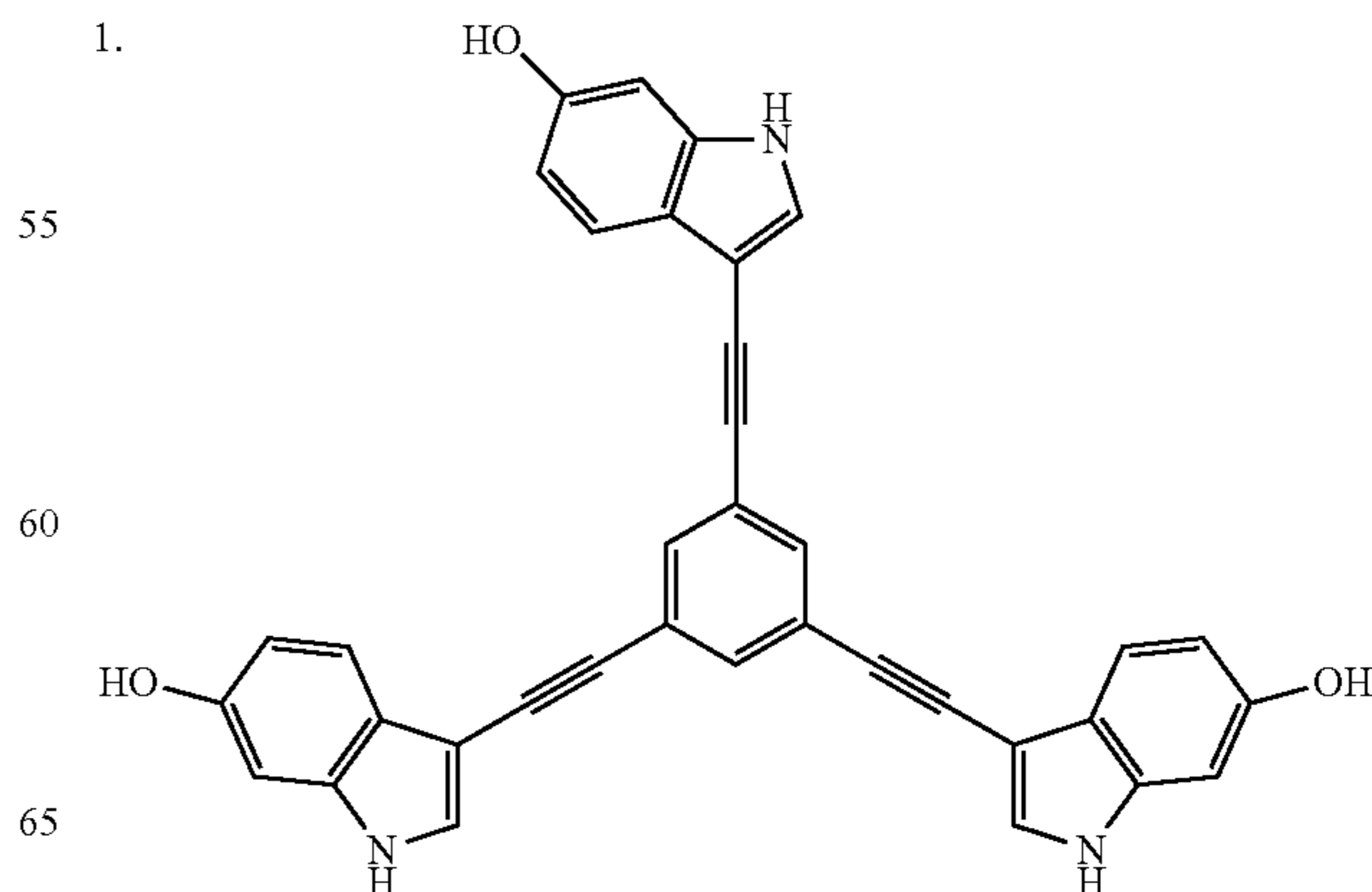
Scheme 1: Exemplary multifunctional organic substrates comprising two, three, or four moieties for polymerization.
