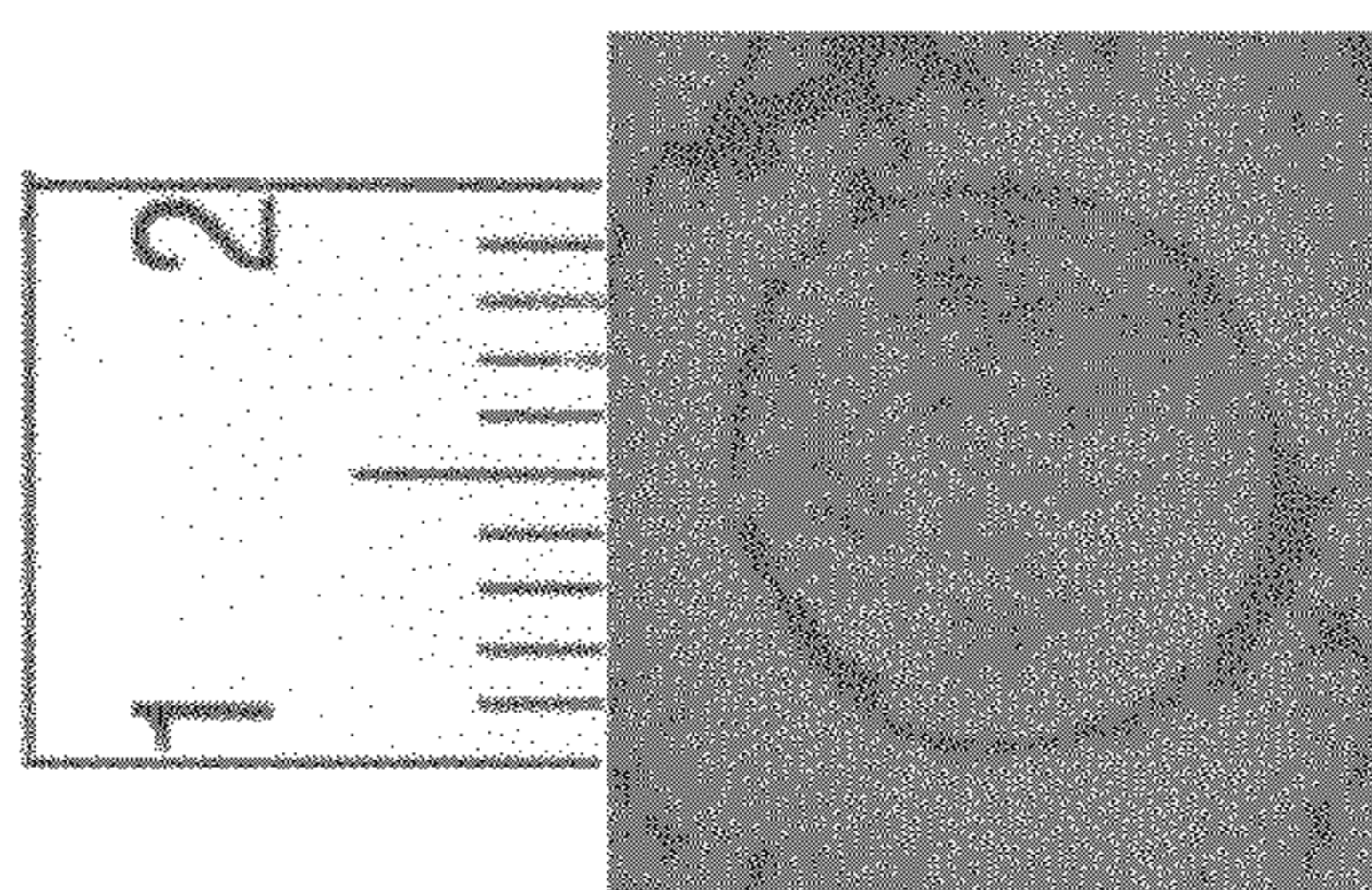
E. coli after 3 days BC - control
