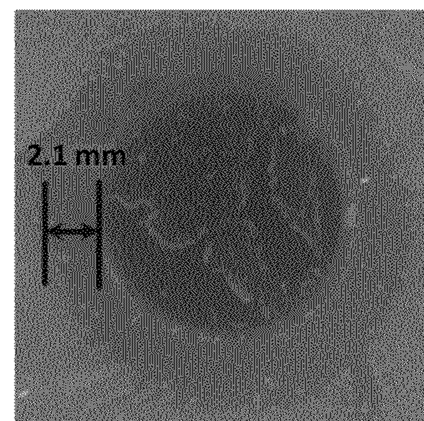
E. coli after 3 days 1 hr - oxidized (BC-Ag)
