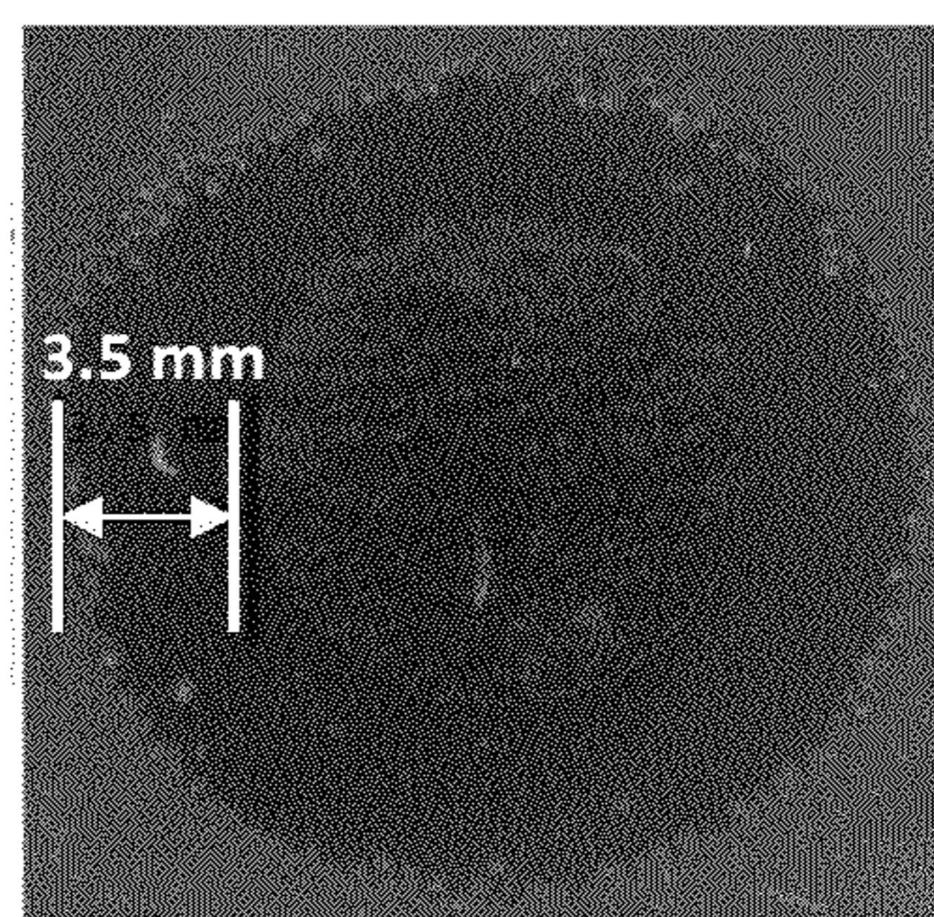
E. coli after 3 days 1 hr oxidized (BC-SP)
