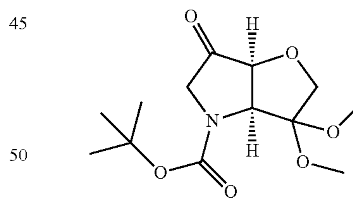
3,3-Dimethoxy-6-oxo-hexahydro-furo[3,2-b]pyrrole-4-carboxylic acid tert-butyl ester (1e)
