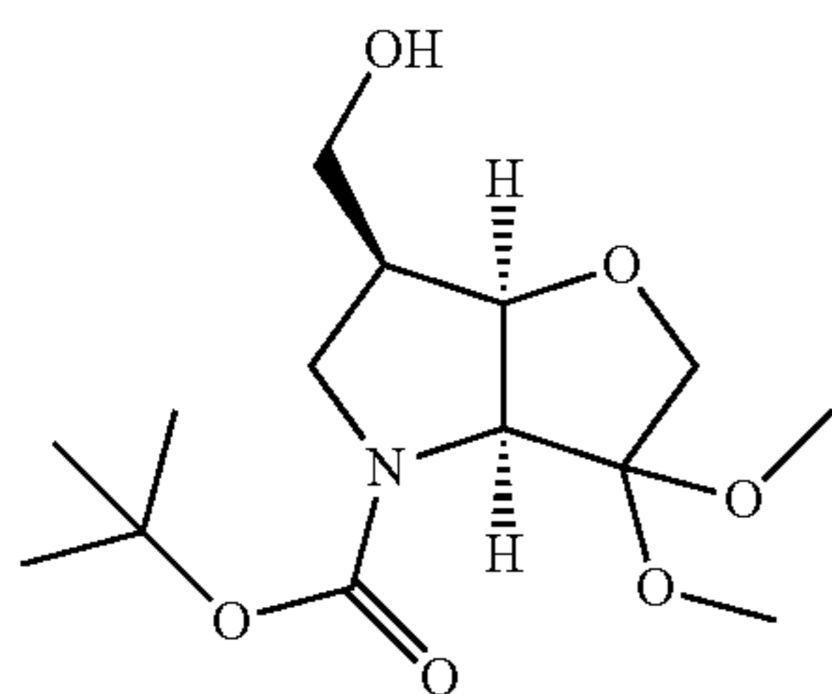
6-Hydroxymethyl-3,3-dimethoxy-hexahydro-furo[3,2-b]pyrrole-4-carboxylic acid tert-butyl ester (1g)
