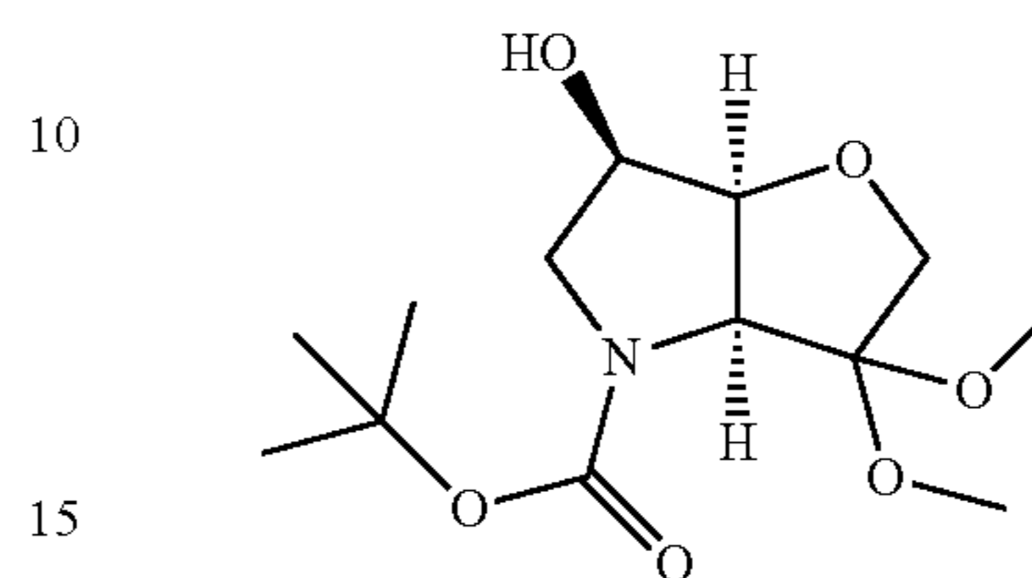
(3aS,6aS)-6R-hydroxy-3,3-dimethoxy-hexahydro-furo[3,2-b]pyrrole-4-carboxylic acid tert-butyl ester (1d)
