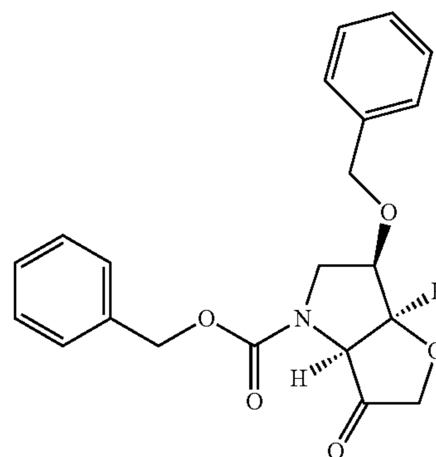
(3 as, 6aS)-6R-benzyloxy-3-oxo-hexahydro-furo[3,2-b]pyrrole-4-carboxylic acid benzyl ester (1a)
