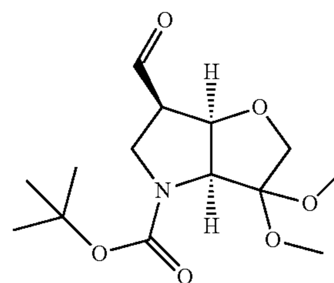
6-Formyl-3,3-dimethoxy-hexahydro-furo[3,2-b]pyrrole-4-carboxylic acid tert-butyl ester
