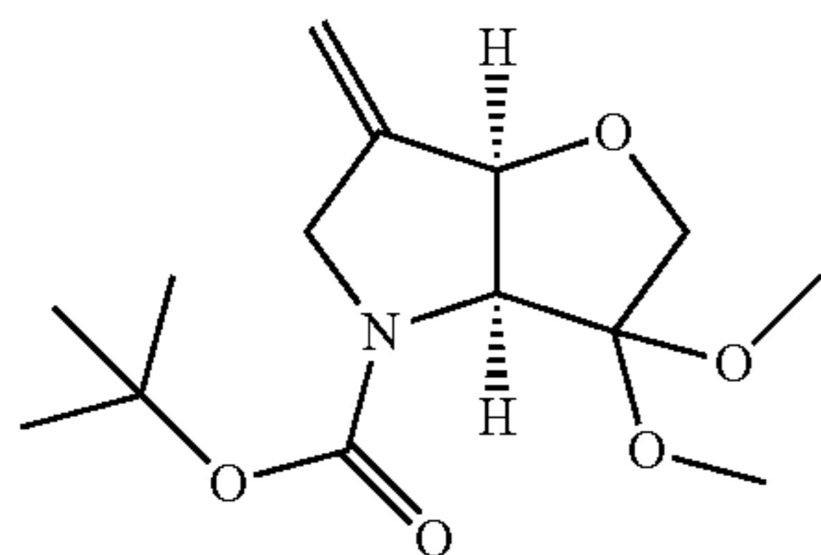
3,3-Dimethoxy-6-methylene-hexahydro-furo[3,2-b]pyrrole-4-carboxylic acid tert-butyl ester (1f)
