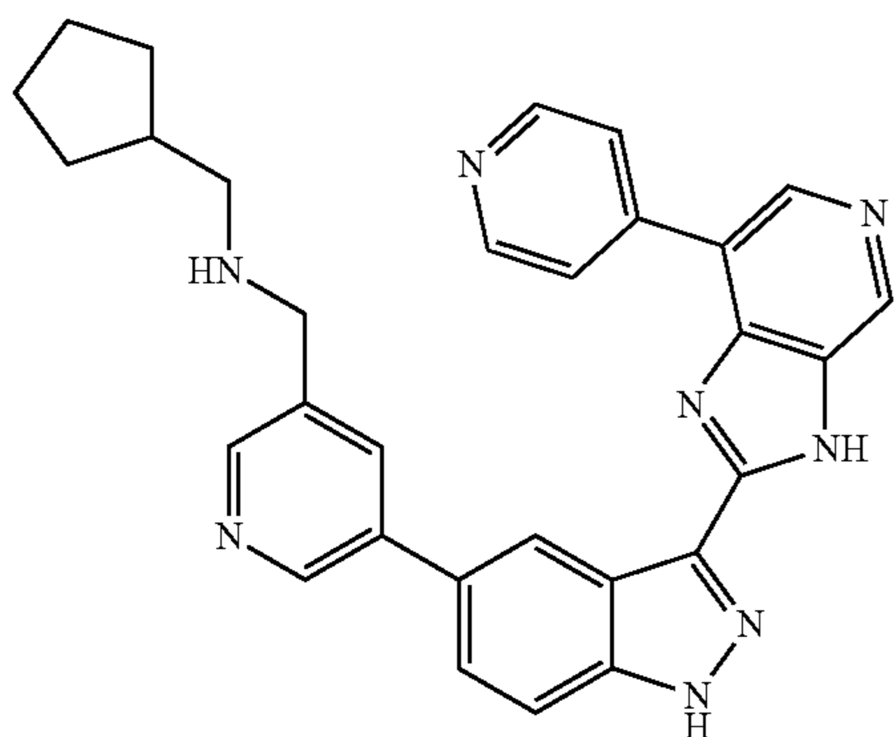
1-Cyclopentyl-N-((5-(3-(7-(pyridin-4-yl)-3H-imidazo[4,5-c]pyridin-2-yl)-1H-indazol-5-yl)pyridin-3-yl)methyl)methanamine 173
