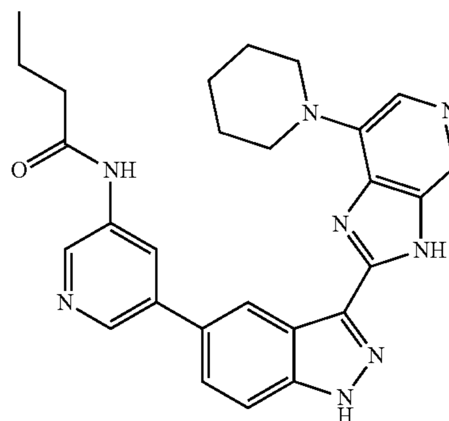
N-(5-(3-(7-(Piperidin-1-yl)-3H-imidazo[4,5-c]pyridin-2-yl)-1H-indazol-5-yl)pyridin-3-yl)butyramide 214
