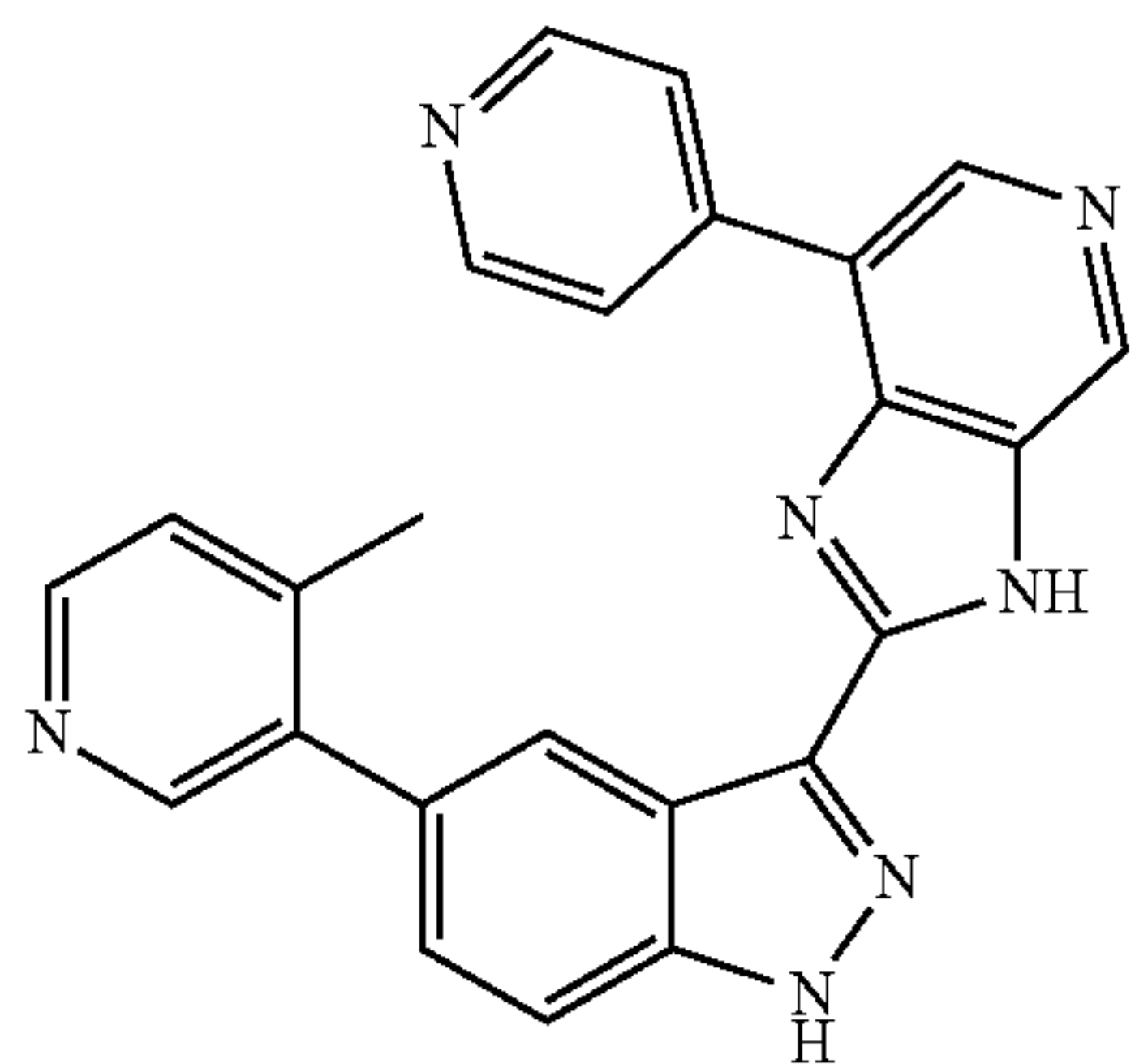
2-(5-(4-Methylpyridin-3-yl)-1H-indazol-3-yl)-7-(pyridin-4-yl)-3H-imidazo[4,5-c]pyridine 154
