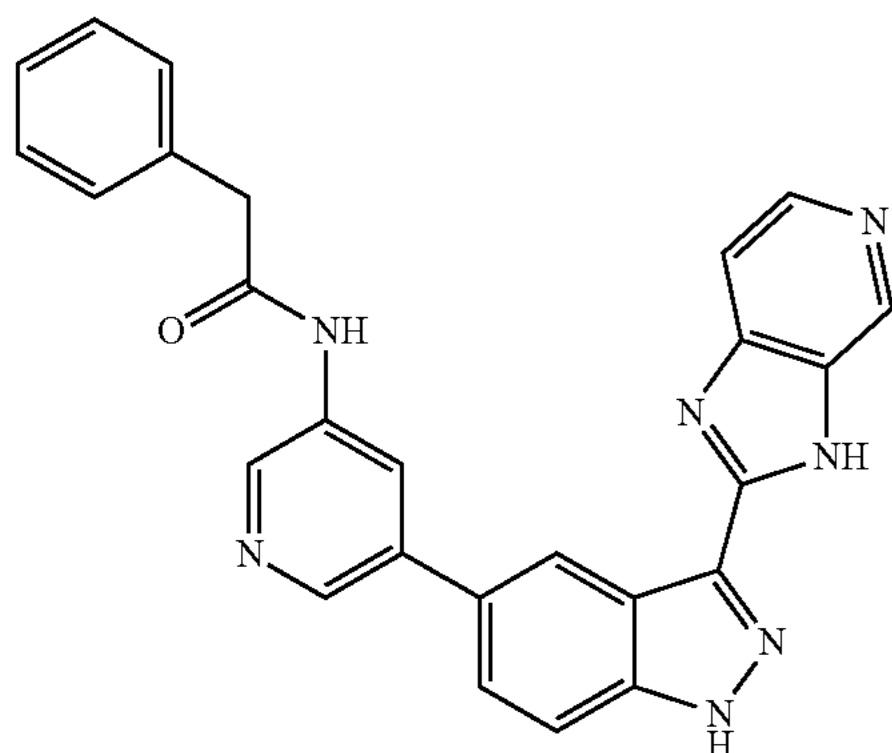
N-(5-(3-(3H-Imidazo[4,5-c]pyridin-2-yl)-1H-indazol-5-yl)pyridin-3-yl)-2-phenylacetamide 274
