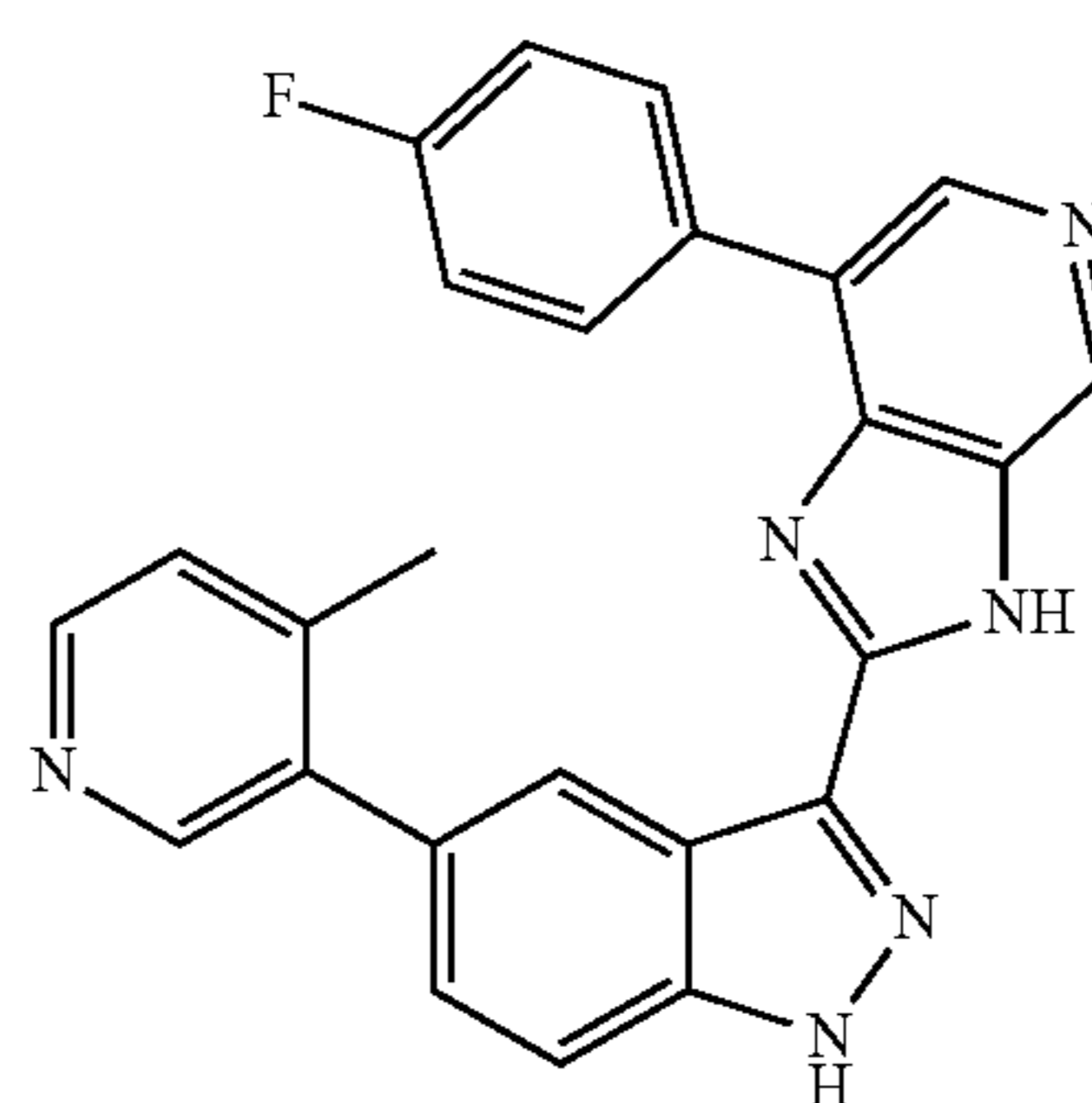
7-(4-Fluorophenyl)-2-(5-(4-methylpyridin-3-yl)-1H-indazol-3-yl)-3H-imidazo[4,5-c]pyridine 99
