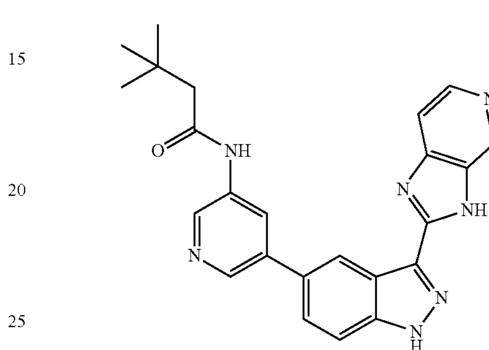
5-(3-(3H-Imidazo[4,5-c]pyridin-2-yl)-1H-indazol-5-yl)pyridin-3-amine 268
