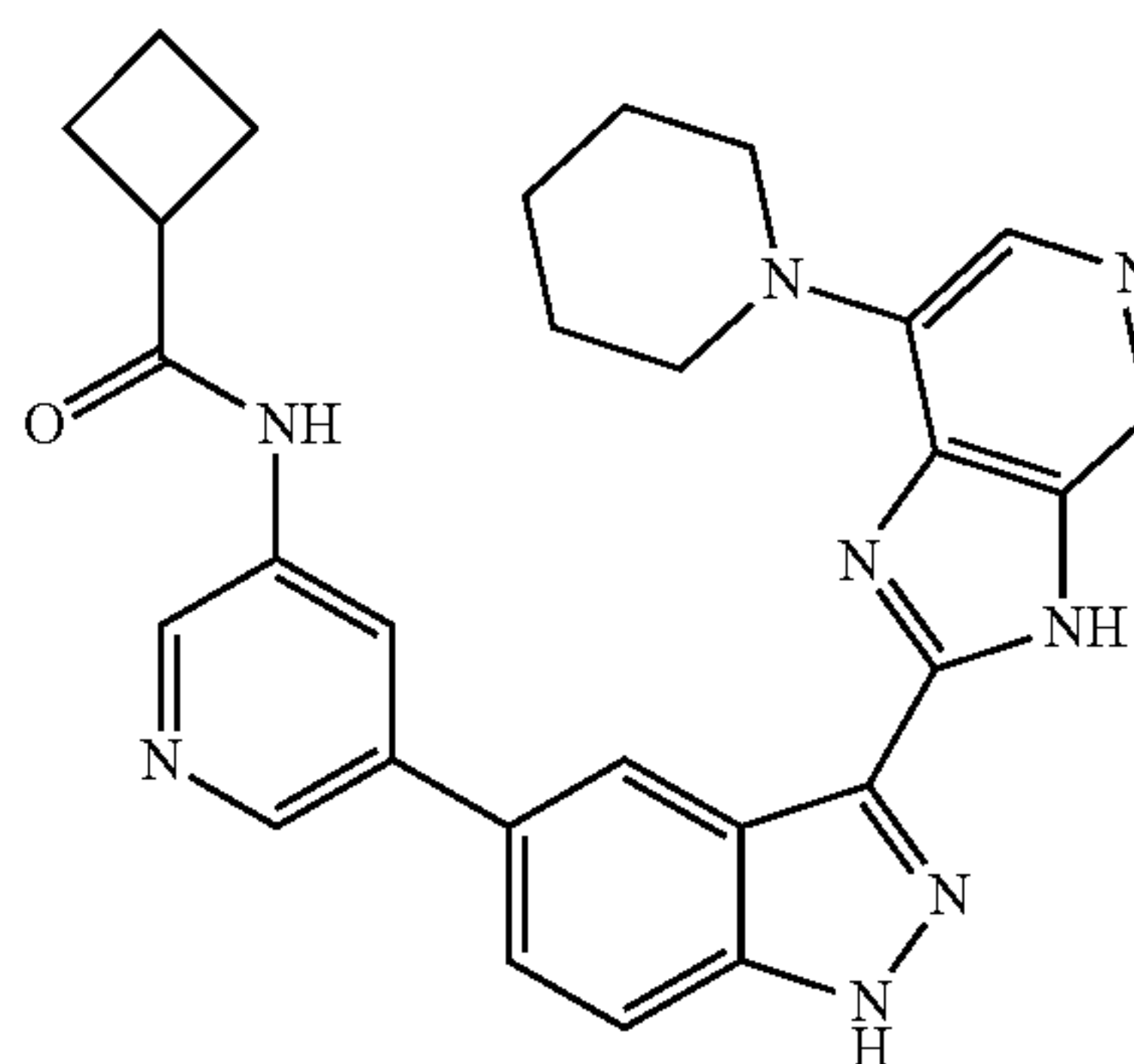
N-(5-(3-(7-(Piperidin-1-yl)-3H-imidazo[4,5-c]pyridin-2-yl)-1H-indazol-5-yl)pyridin-3-yl)cyclobutanecarboxamide 217
