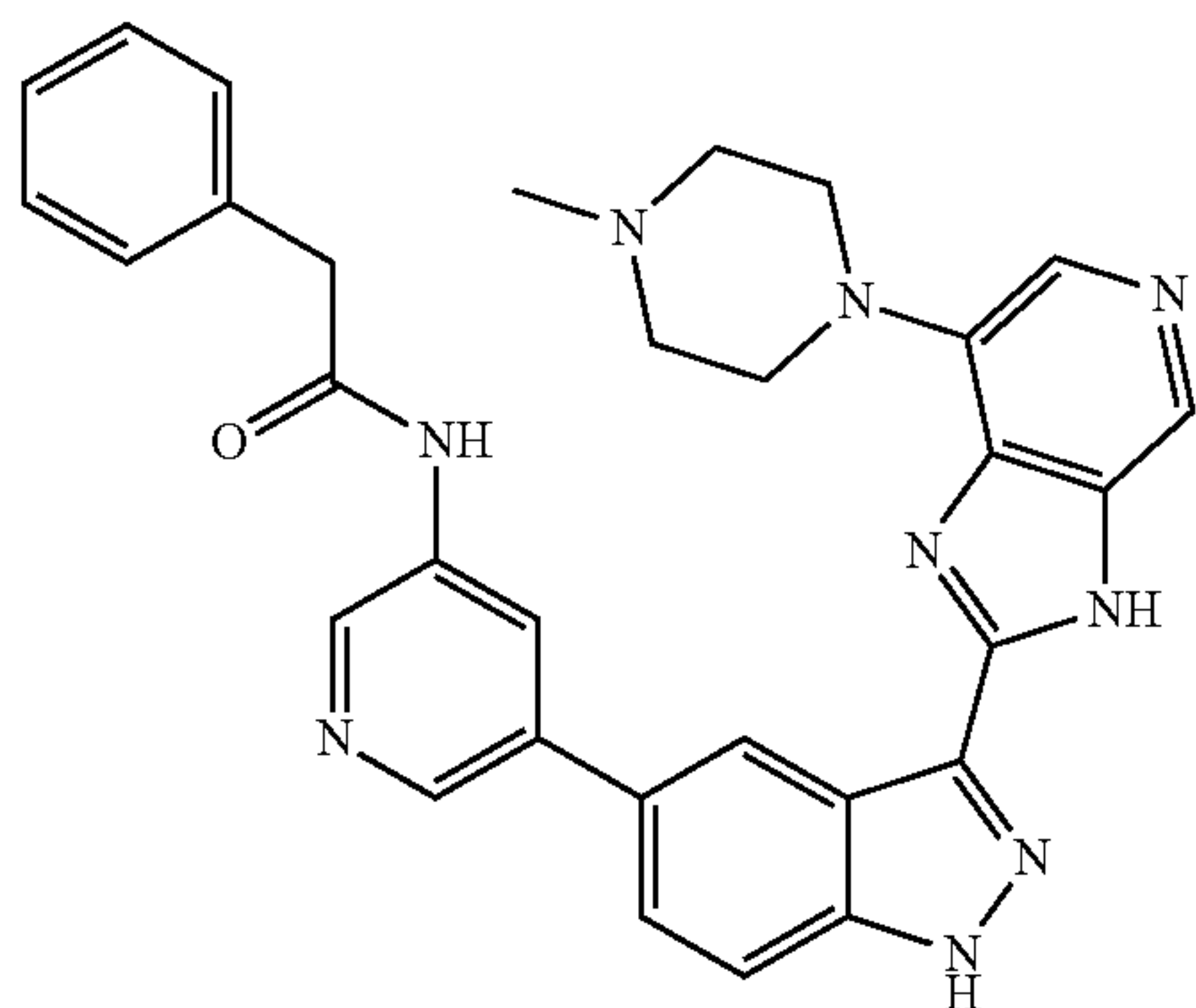
N-(5-(3-(7-(4-Methylpiperazin-1-yl)-3H-imidazo[4,5-c]pyridin-2-yl)-1H-indazol-5-yl)pyridin-3-yl)-2-phenylacetamide 252
