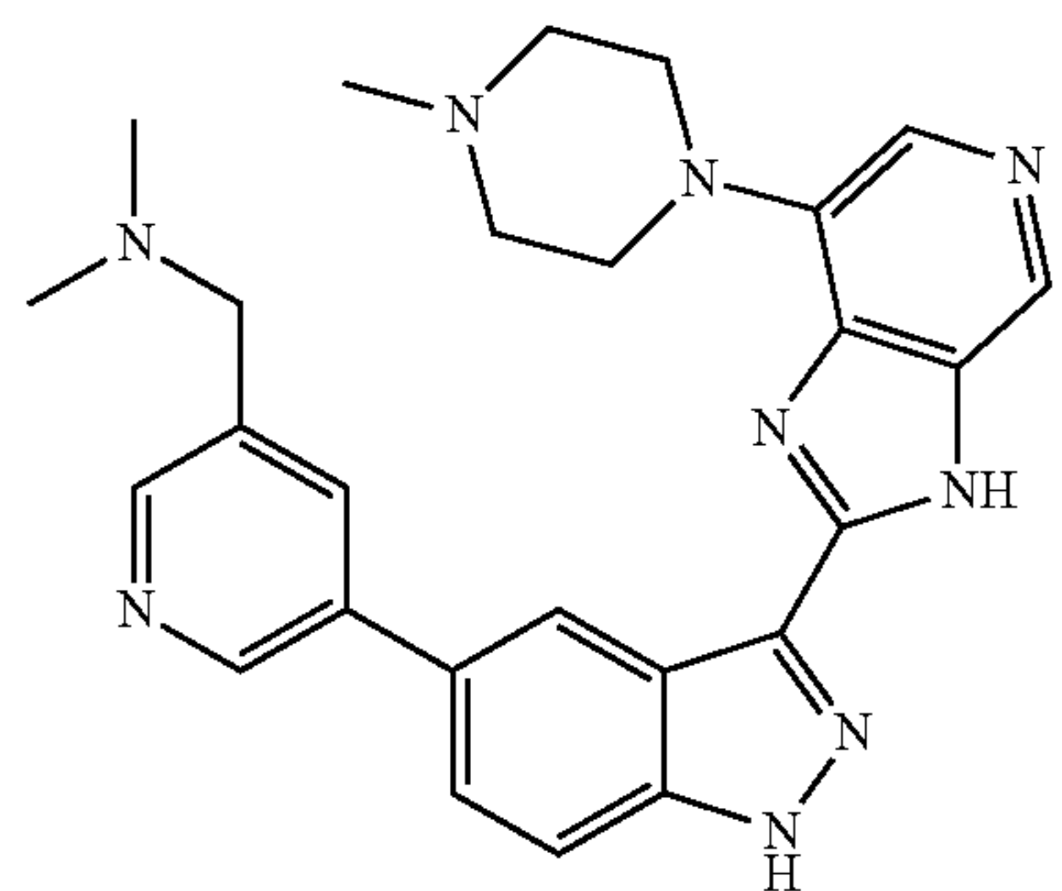
N,N-dimethyl-1-(5-(3-(7-(4-methylpiperazin-1-yl)-3H-imidazo[4,5-c]pyridin-2-yl)-1H-indazol-5-yl)pyridin-3-yl)methanamine 3
