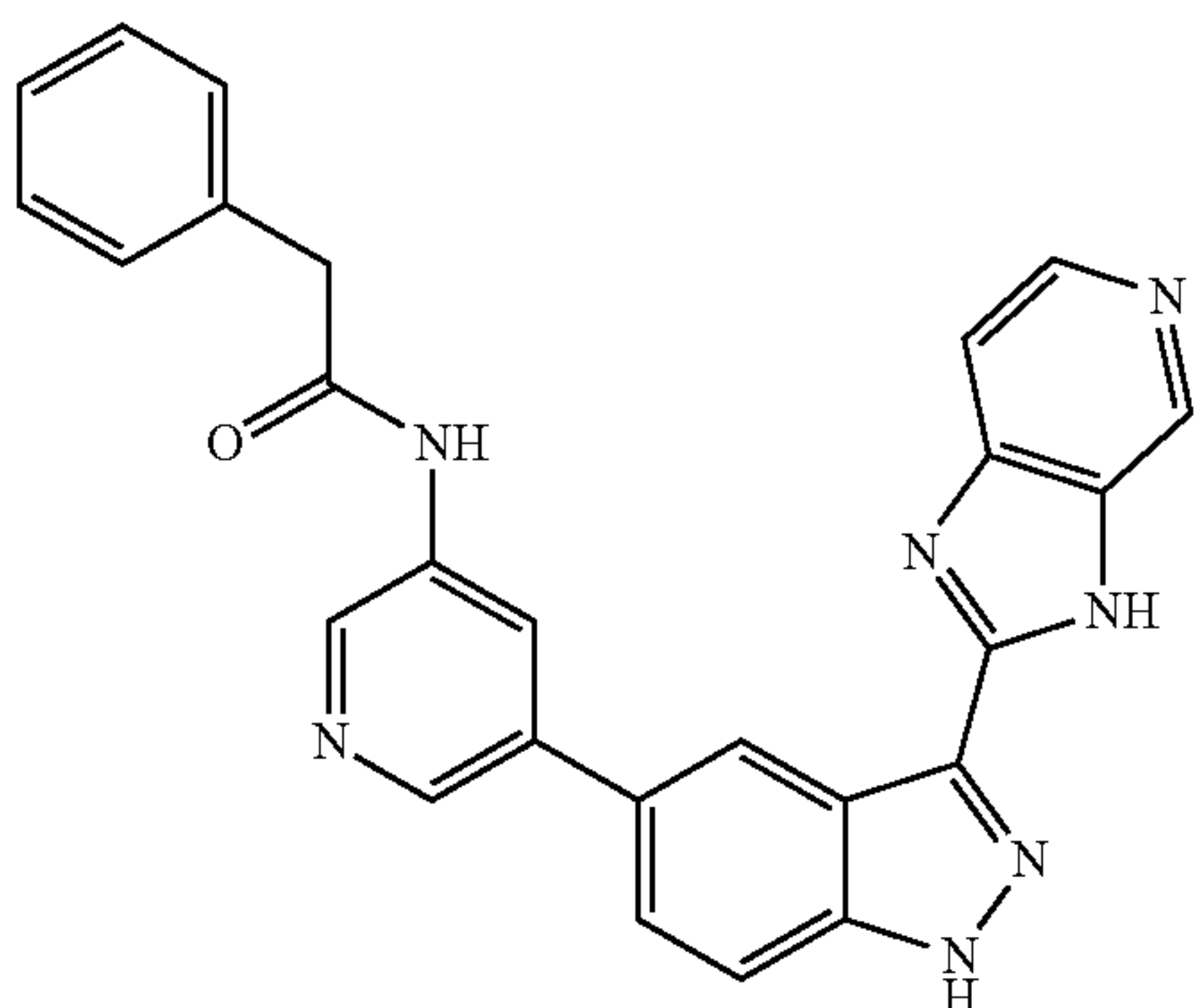
N-(5-(3-(3H-Imidazo[4,5-c]pyridin-2-yl)-1H-indazol-5-yl)pyridin-3-yl)-2-phenylacetamide 274
