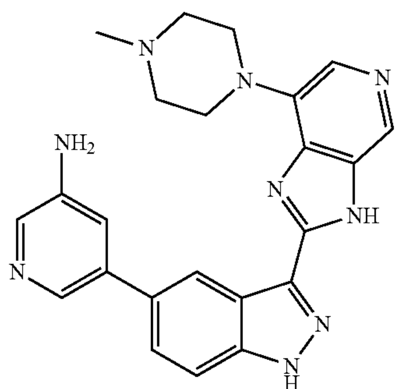
5-(3-(7-(4-Methylpiperazin-1-yl)-3H-imidazo[4,5-c]pyridin-2-yl)-1H-indazol-5-yl)pyridin-3-amine 247
