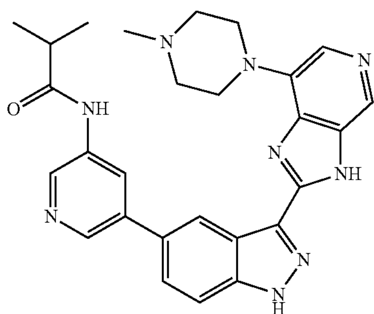
N-(5-(3-(7-(4-methylpiperazin-1-yl)-3H-imidazo[4,5-c]pyridin-2-yl)-1H-indazol-5-yl)pyridin-3-yl)isobutyramide 2
