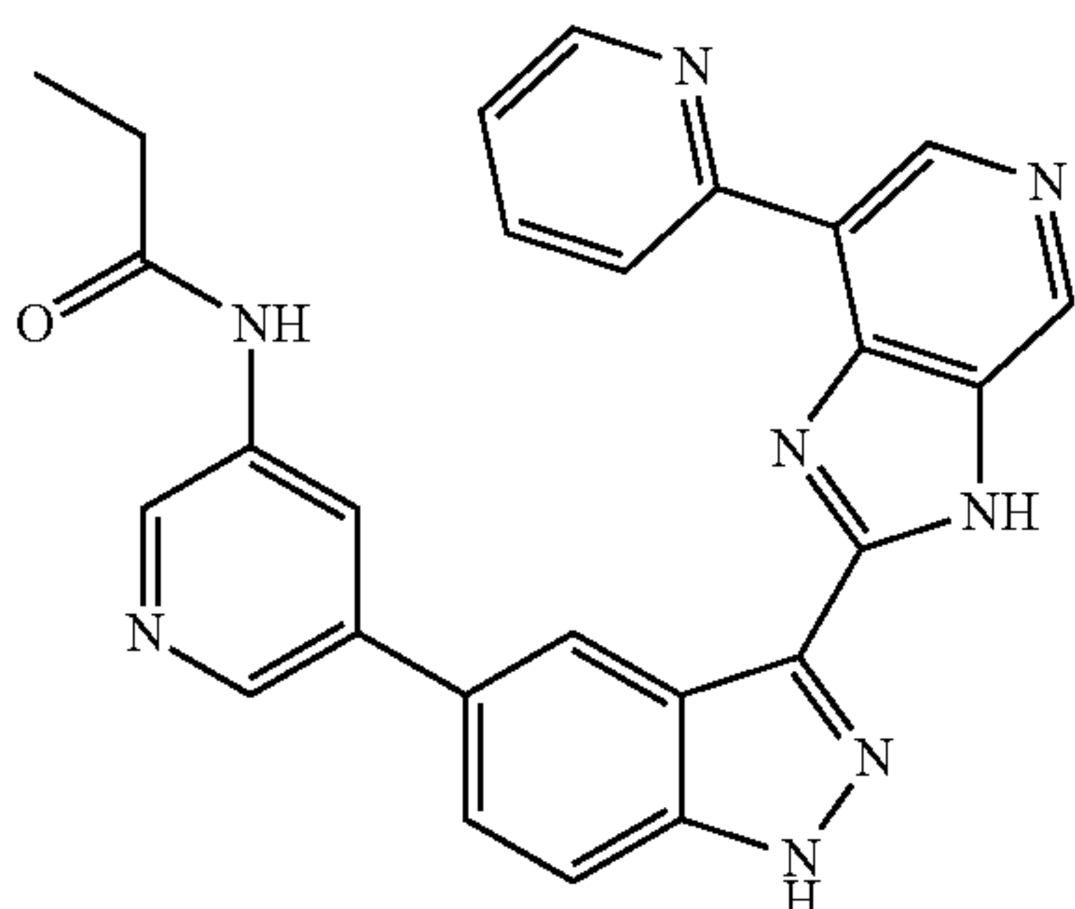
N-(5-(3-(7-(Pyridin-2-yl)-3H-imidazo[4,5-c]pyridin-2-yl)-1H-indazol-5-yl)pyridin-3-yl)propionamide 174
