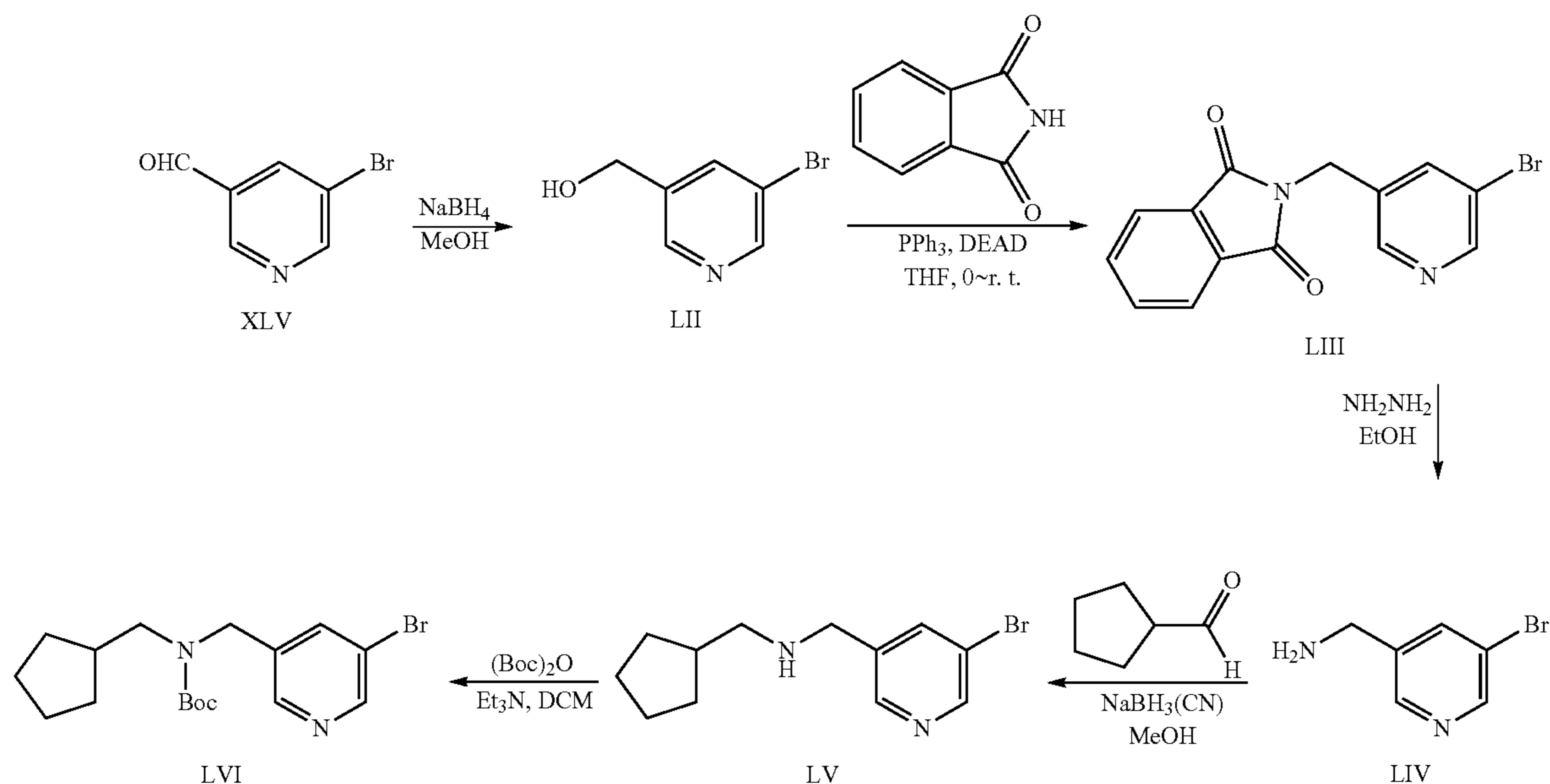
Scheme 11
