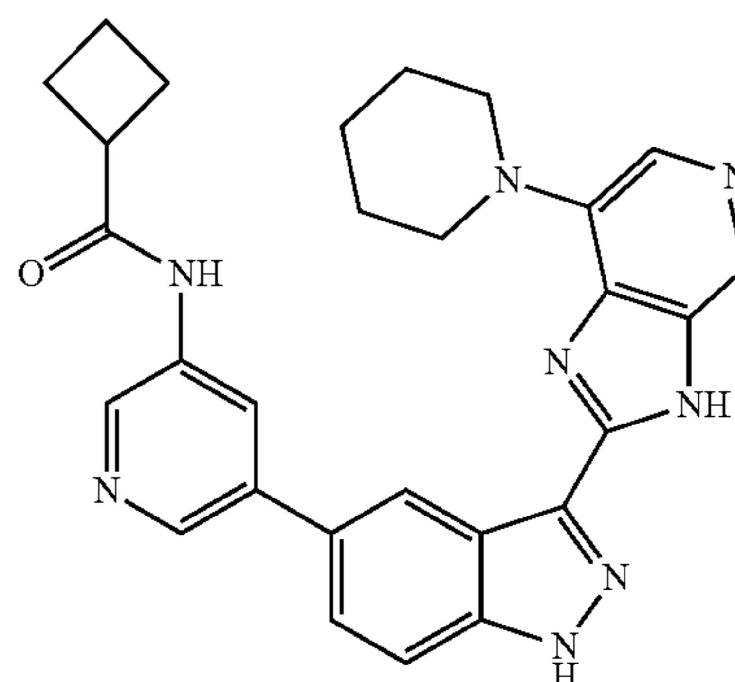
N-(5-(3-(7-(Piperidin-1-yl)-3H-imidazo[4,5-c]pyridin-2-yl)-1H-indazol-5-yl)pyridin-3-yl)cyclobutanecarboxamide 217
