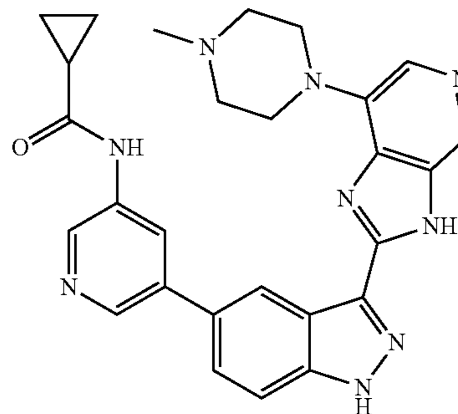
N-(5-(3-(7-(4-Methylpiperazin-1-yl)-3H-imidazo[4,5-c]pyridin-2-yl)-1H-indazol-5-yl)pyridin-3-yl)cyclopropanecarboxamide 260
