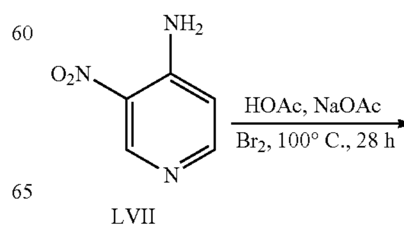
Scheme 12
