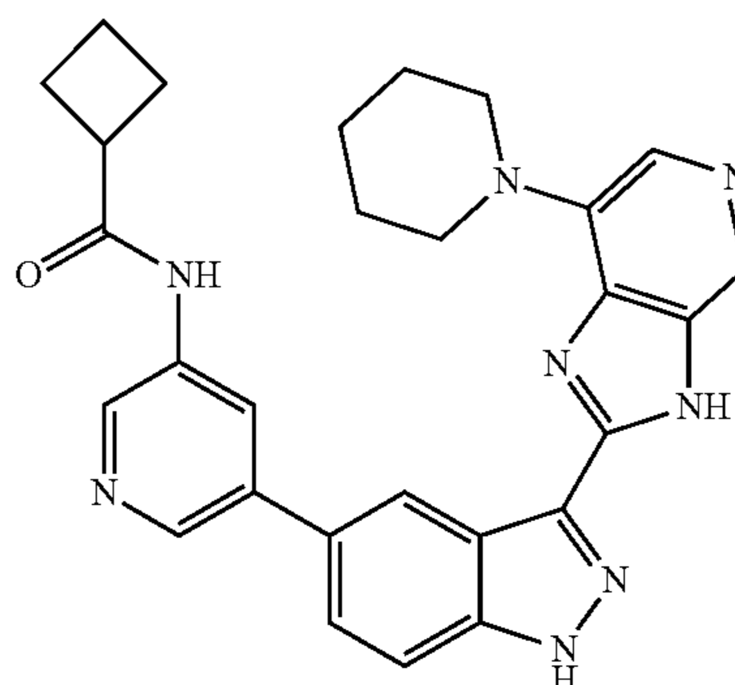
N-(5-(3-(7-(Piperidin-1-yl)-3H-imidazo[4,5-c]pyridin-2-yl)-1H-indazol-5-yl)pyridin-3-yl)cyclobutanecarboxamide 217
