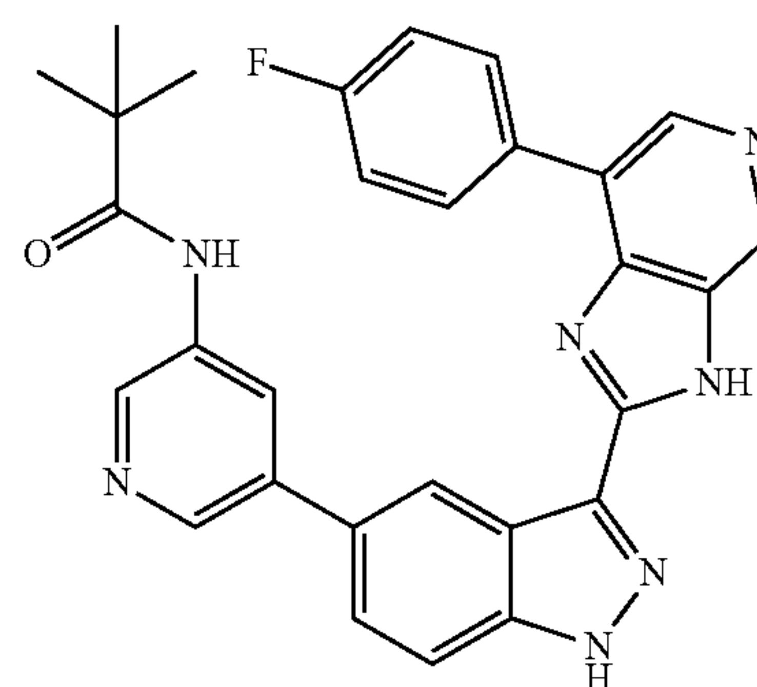
N-(5-(3-(7-(4-Fluorophenyl)-3H-imidazo[4,5-c]pyridin-2-yl)-1H-indazol-5-yl)pyridin-3-yl)pivalamide 102
