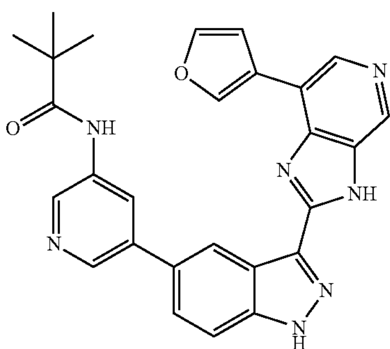
N-(5-(3-(7-(Furan-3-yl)-3H-imidazo[4,5-c]pyridin-2-yl)-1H-indazol-5-yl)pyridin-3-yl)pivalamide 319
