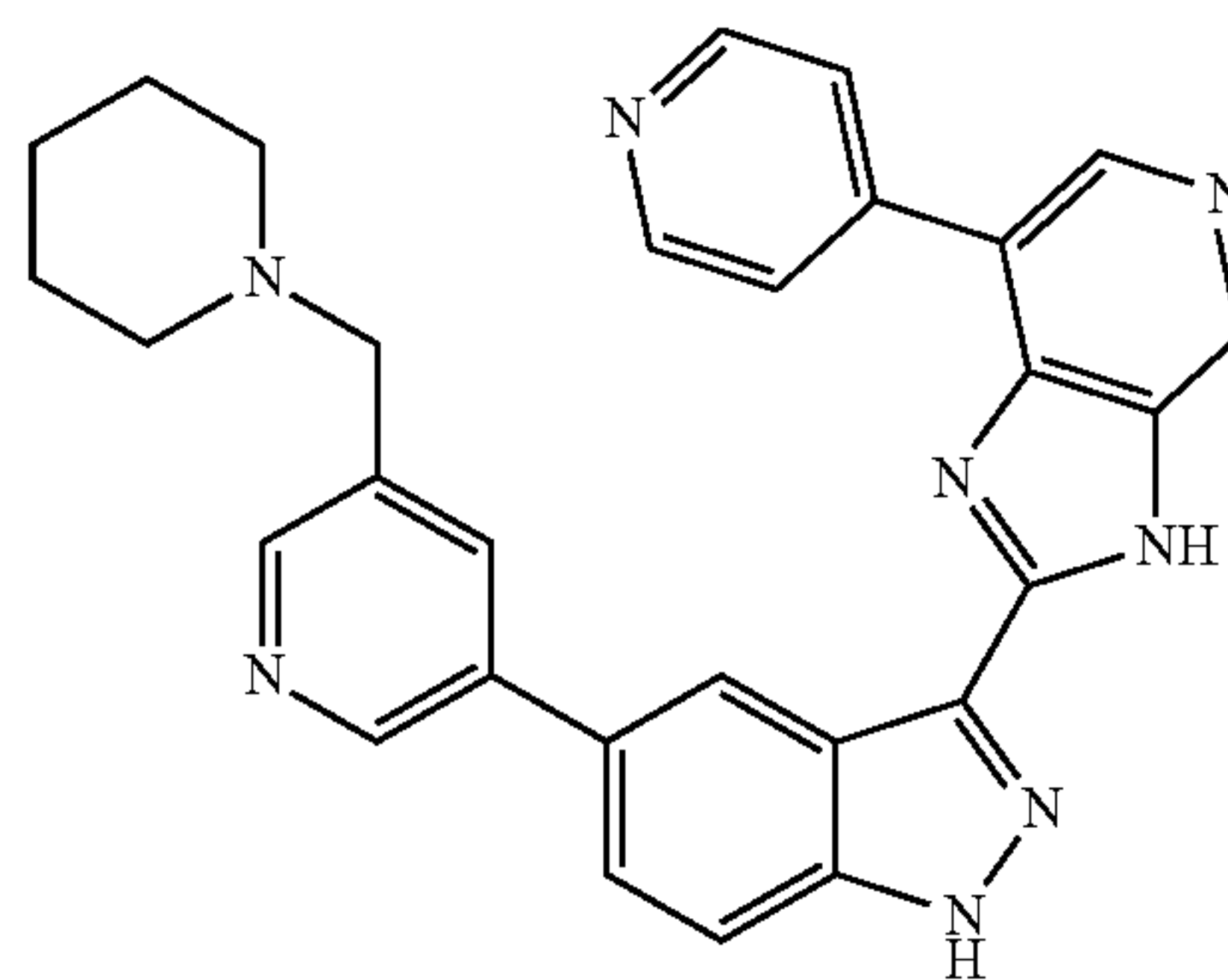
2-(5-(5-(Piperidin-1-ylmethyl)pyridin-3-yl)-1H-indazol-3-yl)-7-(pyridin-4-yl)-3H-imidazo[4,5-c]pyridine 164
