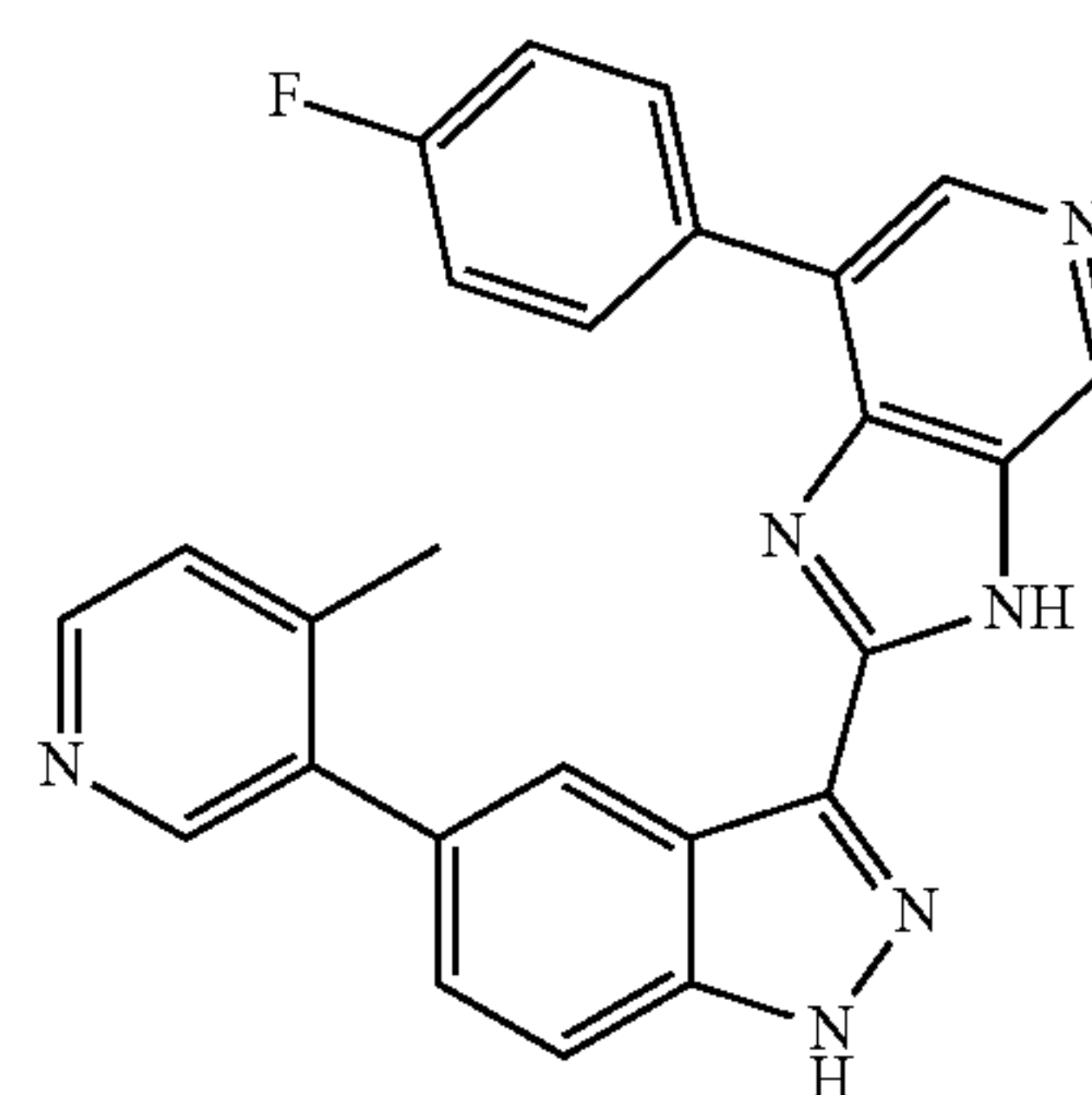
7-(4-Fluorophenyl)-2-(5-(4-methylpyridin-3-yl)-1H-indazol-3-yl)-3H-imidazo[4,5-c]pyridine 99
