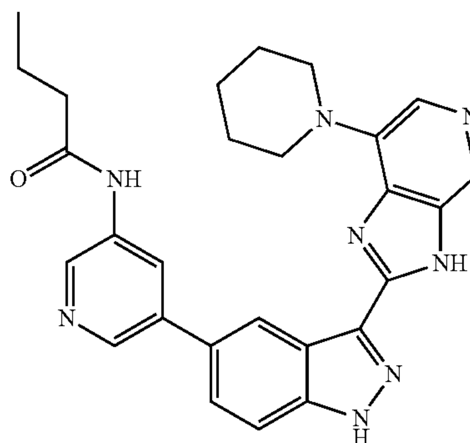
N-(5-(3-(7-(Piperidin-1-yl)-3H-imidazo[4,5-c]pyridin-2-yl)-1H-indazol-5-yl)pyridin-3-yl)butyramide 214
