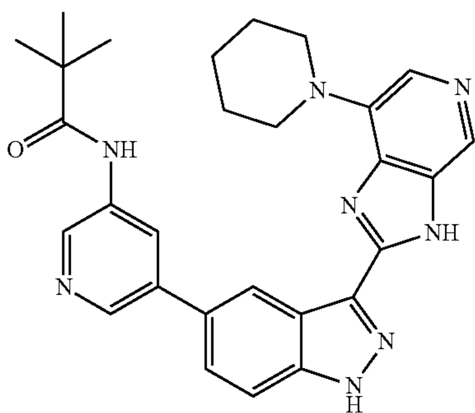
N-(5-(3-(7-(Piperidin-1-yl)-3H-imidazo[4,5-c]pyridin-2-yl)-1H-indazol-5-yl)pyridin-3-yl)pivalamide 205
