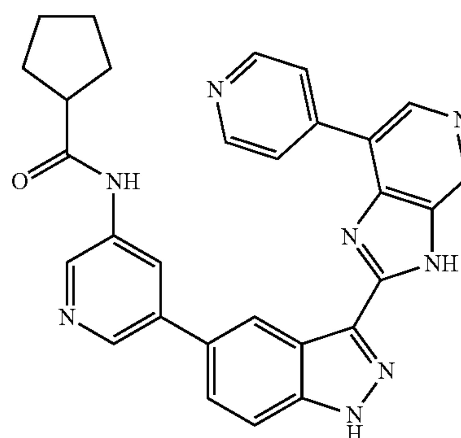
N-(5-(3-(7-(Pyridin-4-yl)-3H-imidazo[4,5-c]pyridin-2-yl)-1H-indazol-5-yl)pyridin-3-yl)cyclopentanecarboxamide 170
