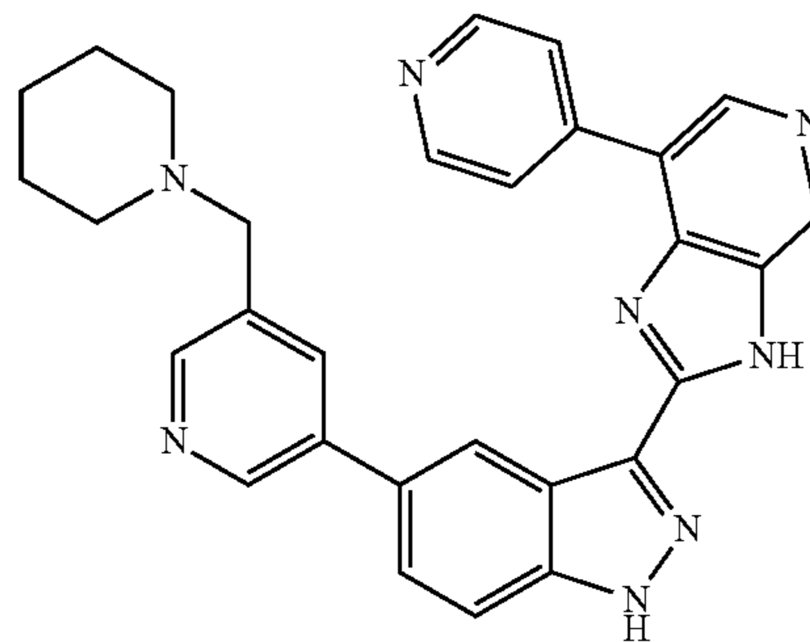
2-(5-(5-(Piperidin-1-ylmethyl)pyridin-3-yl)-1H-indazol-3-yl)-7-(pyridin-4-yl)-3H-imidazo[4,5-c]pyridine 164
