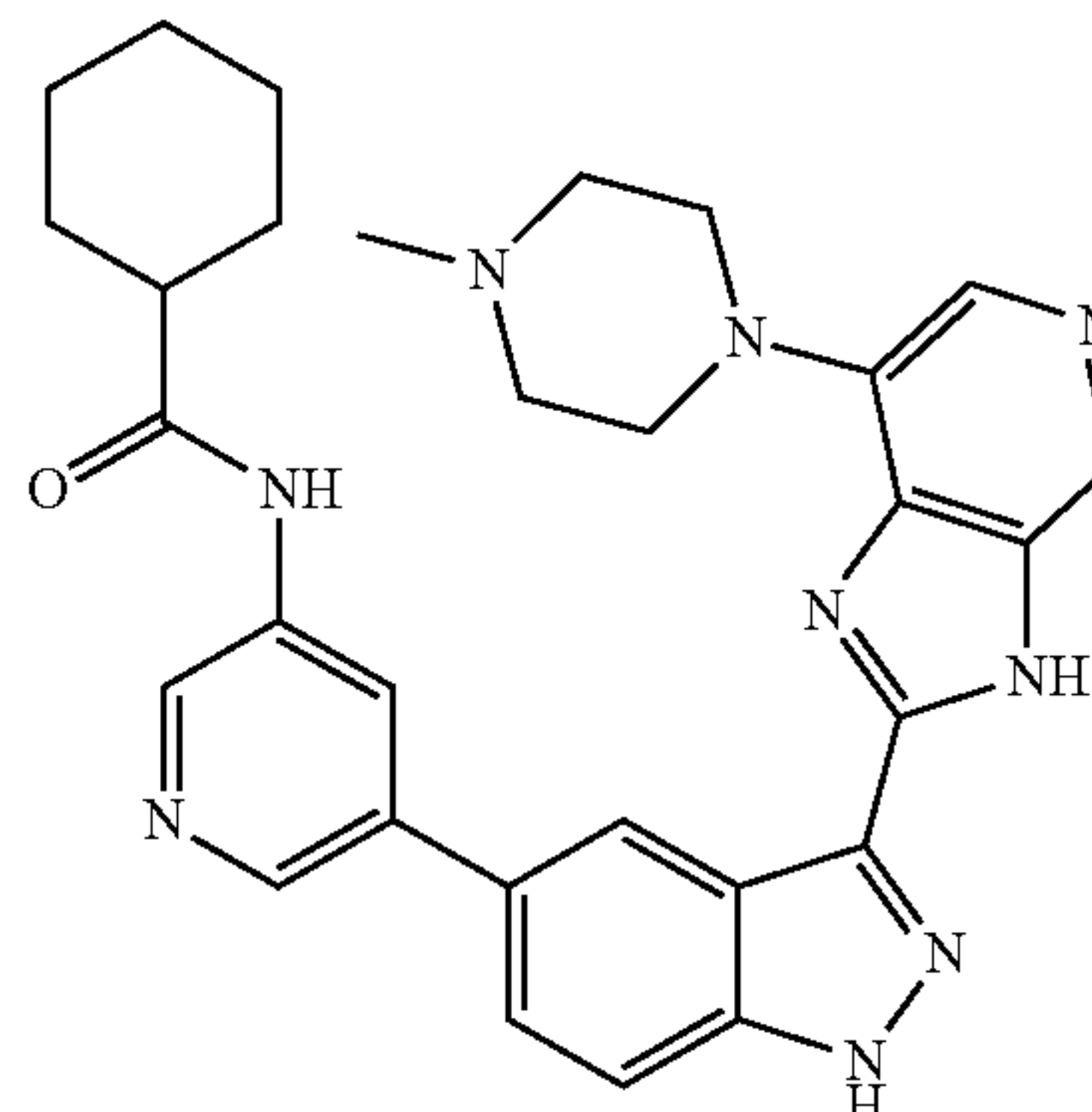
N-(5-(3-(7-(4-Methylpiperazin-1-yl)-3H-imidazo[4,5-c]pyridin-2-yl)-1H-indazol-5-yl)pyridin-3-yl)cyclohexanecarboxamide 263
