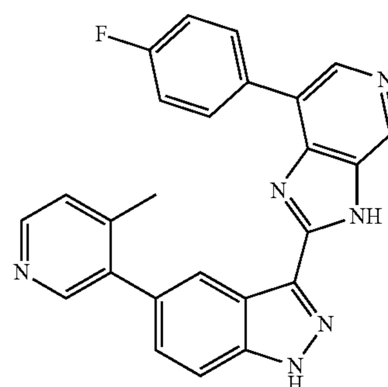
7-(4-Fluorophenyl)-2-(5-(4-methylpyridin-3-yl)-1H-indazol-3-yl)-3H-imidazo[4,5-c]pyridine 99
