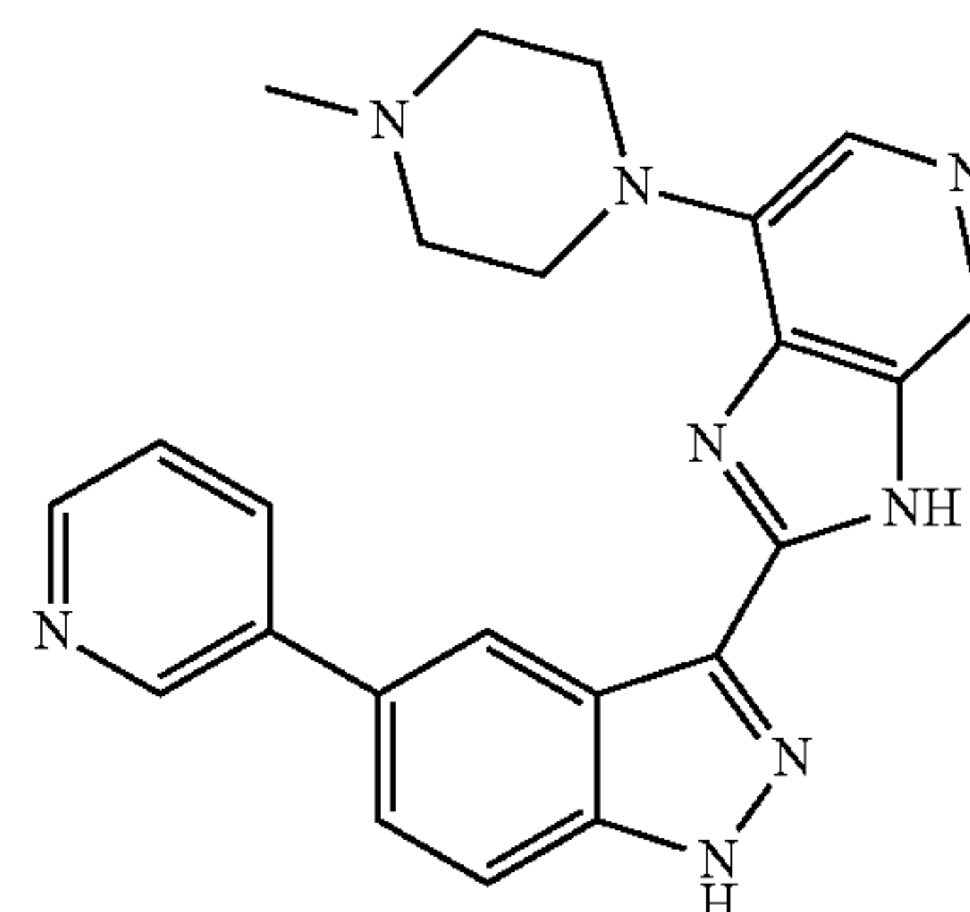
7-(4-methylpiperazin-1-yl)-2-(5-(pyridin-3-yl)-1H-indazol-3-yl)-3H-imidazo[4,5-c]pyridine 4
