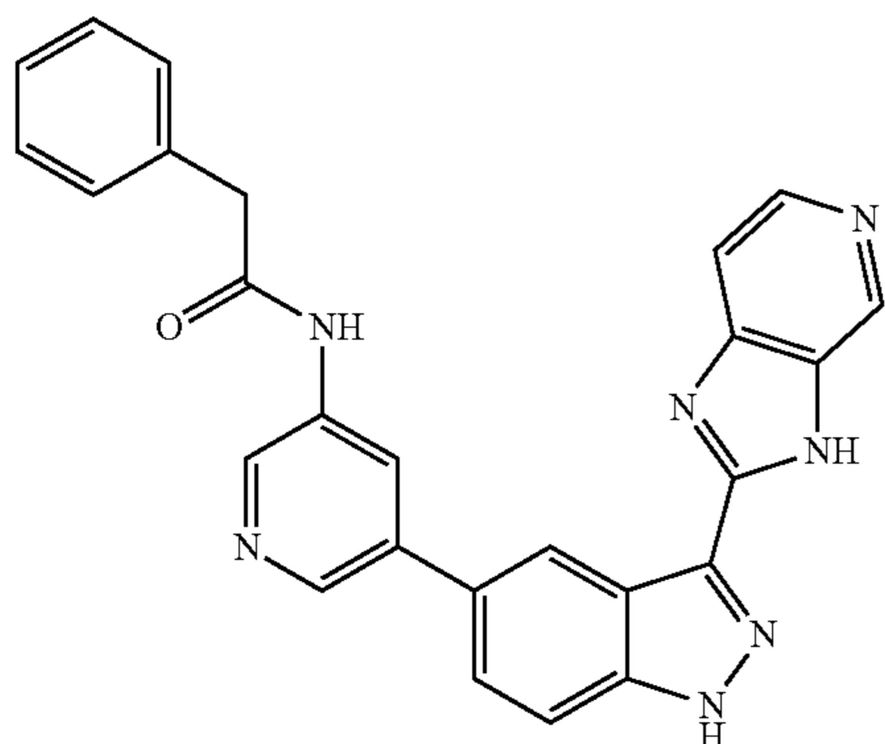
N-(5-(3-(3H-Imidazo[4,5-c]pyridin-2-yl)-1H-indazol-5-yl)pyridin-3-yl)-2-phenylacetamide 274
