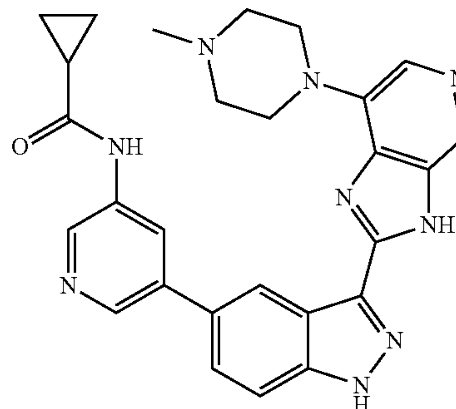
N-(5-(3-(7-(4-Methylpiperazin-1-yl)-3H-imidazo[4,5-c]pyridin-2-yl)-1H-indazol-5-yl)pyridin-3-yl)cyclopropanecarboxamide 260
