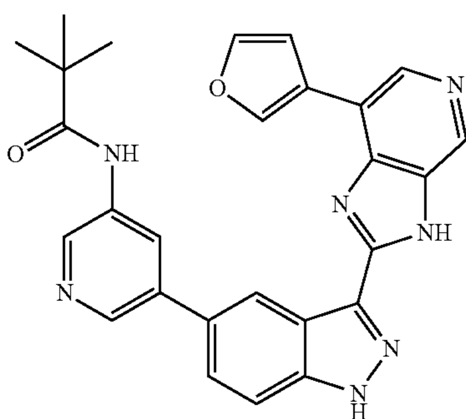
N-(5-(3-(7-(Furan-3-yl)-3H-imidazo[4,5-c]pyridin-2-yl)-1H-indazol-5-yl)pyridin-3-yl)pivalamide 319
