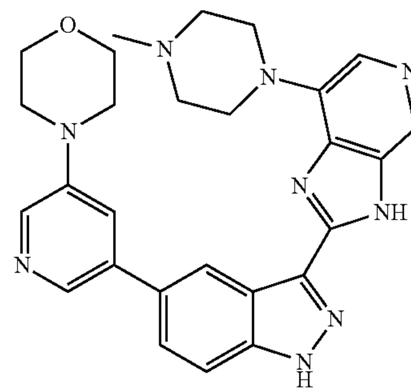
4-(5-(3-(7-(4-methylpiperazin-1-yl)-3H-imidazo[4,5-c]pyridin-2-yl)-1H-indazol-5-yl)pyridin-3-yl)morpholine 5
