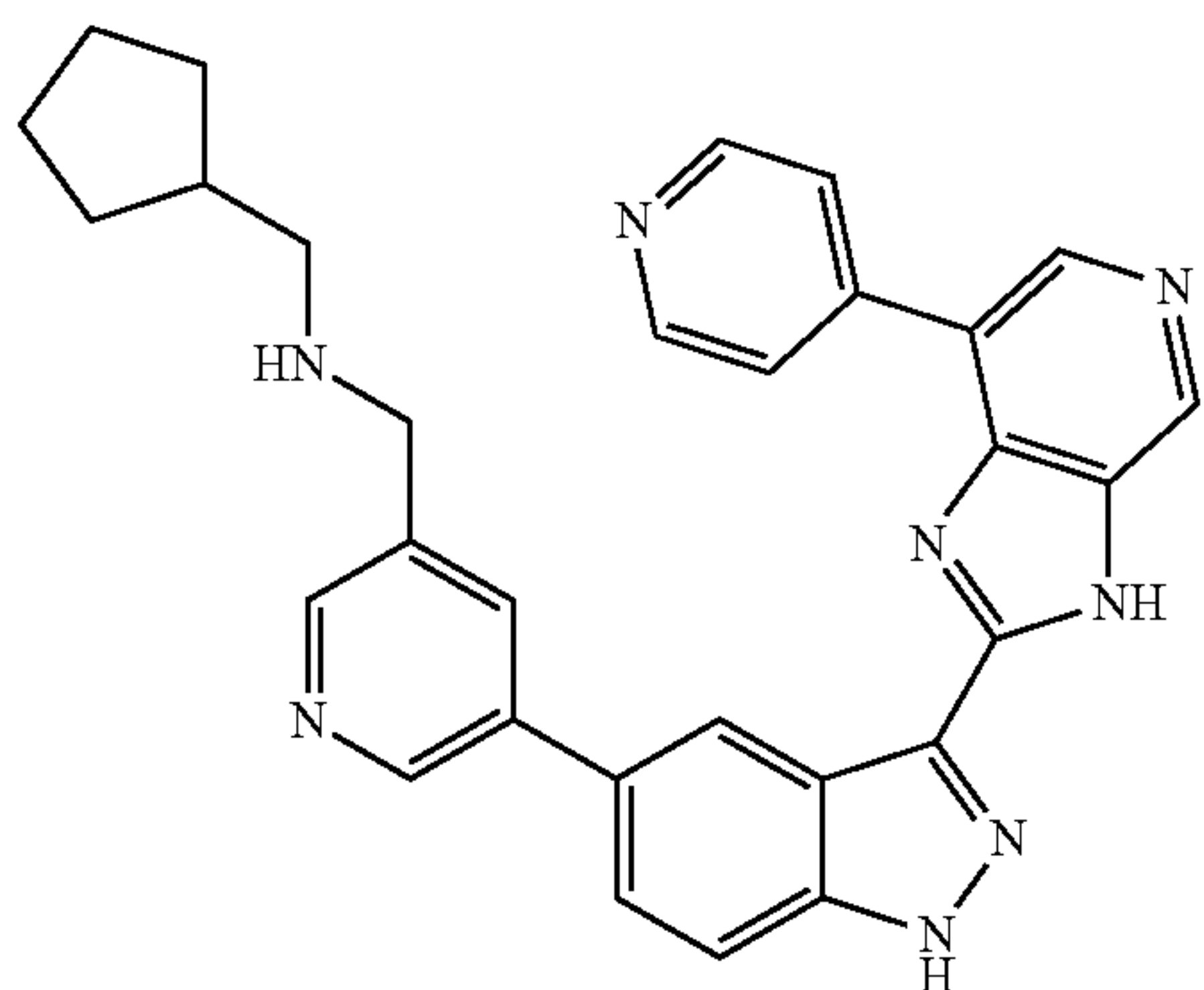
1-Cyclopentyl-N-((5-(3-(7-(pyridin-4-yl)-3H-imidazo[4,5-c]pyridin-2-yl)-1H-indazol-5-yl)pyridin-3-yl)methyl)methanamine 173
