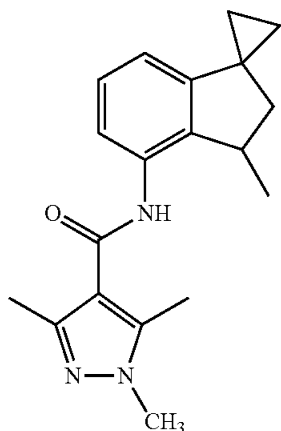
1,3,5-trimethyl-N-(3'-methyl-2',3'-dihydrospiro[cyclopropane-1,1'-inden]-4'-yl)-1H-pyrazole-4-carboxamide
