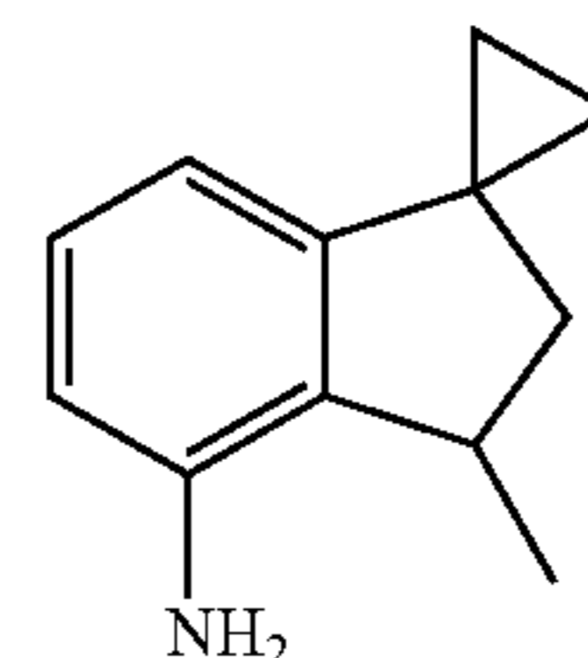
3'-methyl-2',3'-dihydrospiro[cyclopropane-1,1'-inden]-4'-amine (example III-a-16)
