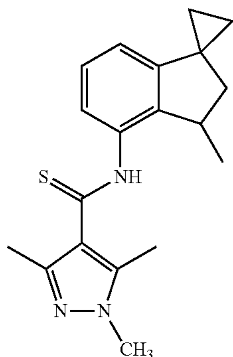
1,3,5-trimethyl-N-(3'-methyl-2',3'-dihydrospiro[cyclopropane-1,1'-inden]-4'-yl)-1H-pyrazole-4-carbothioamide
