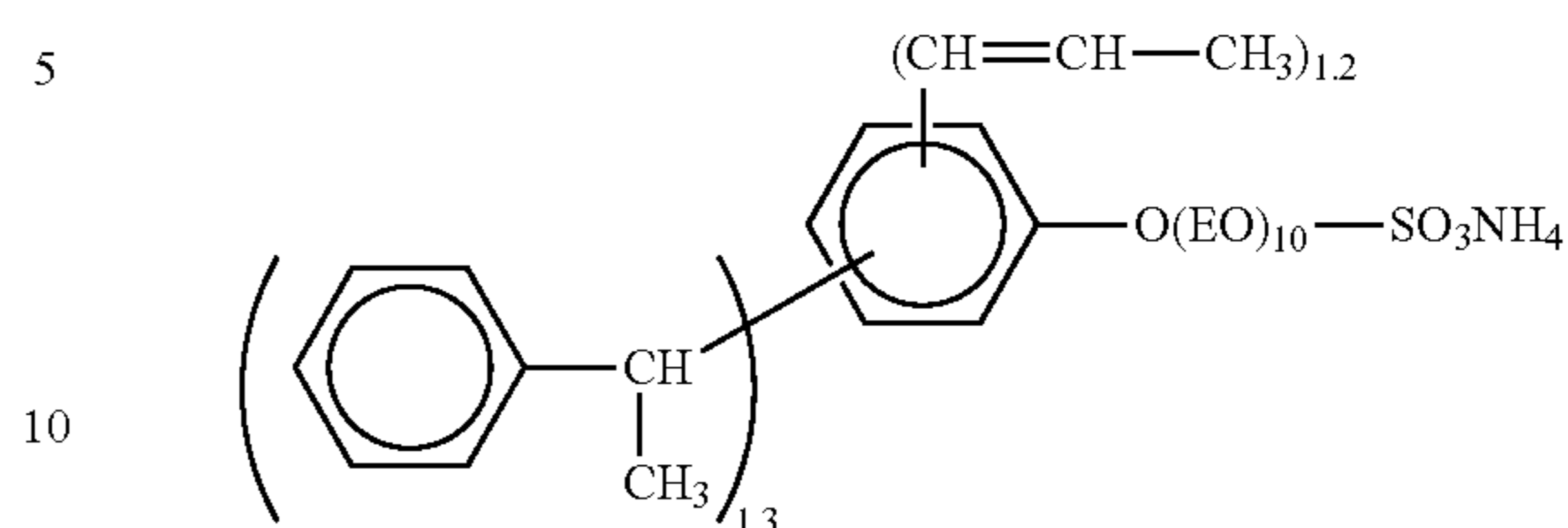
Synthesis Example 4
