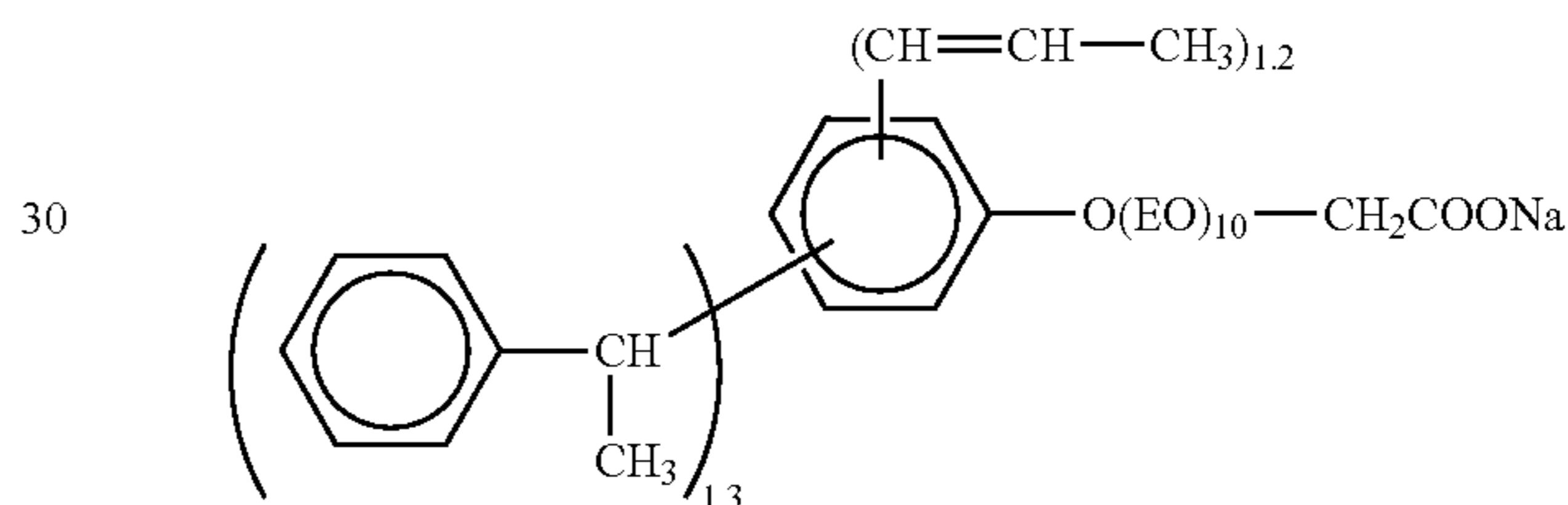
Synthesis Example 5
