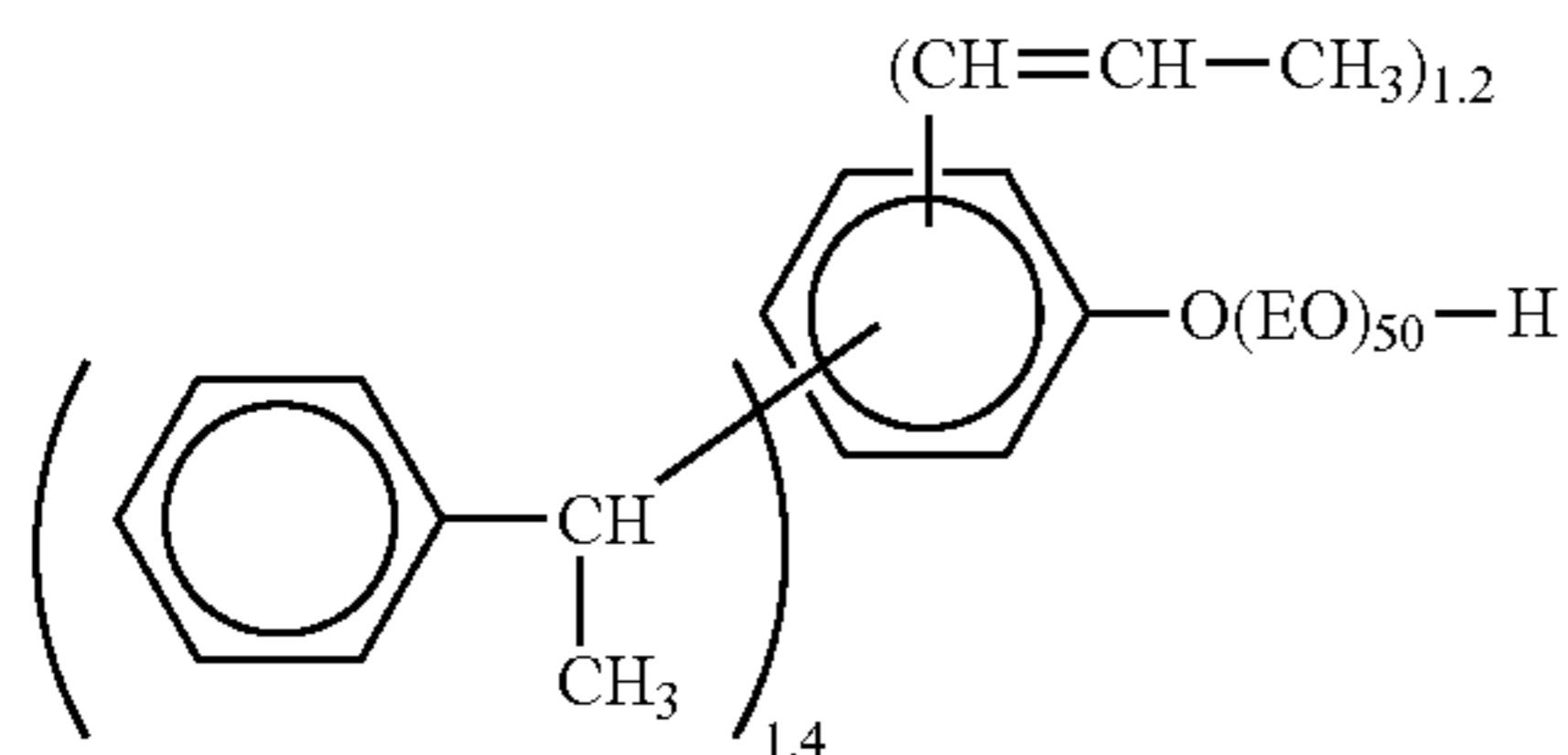
Synthesis Example 13
