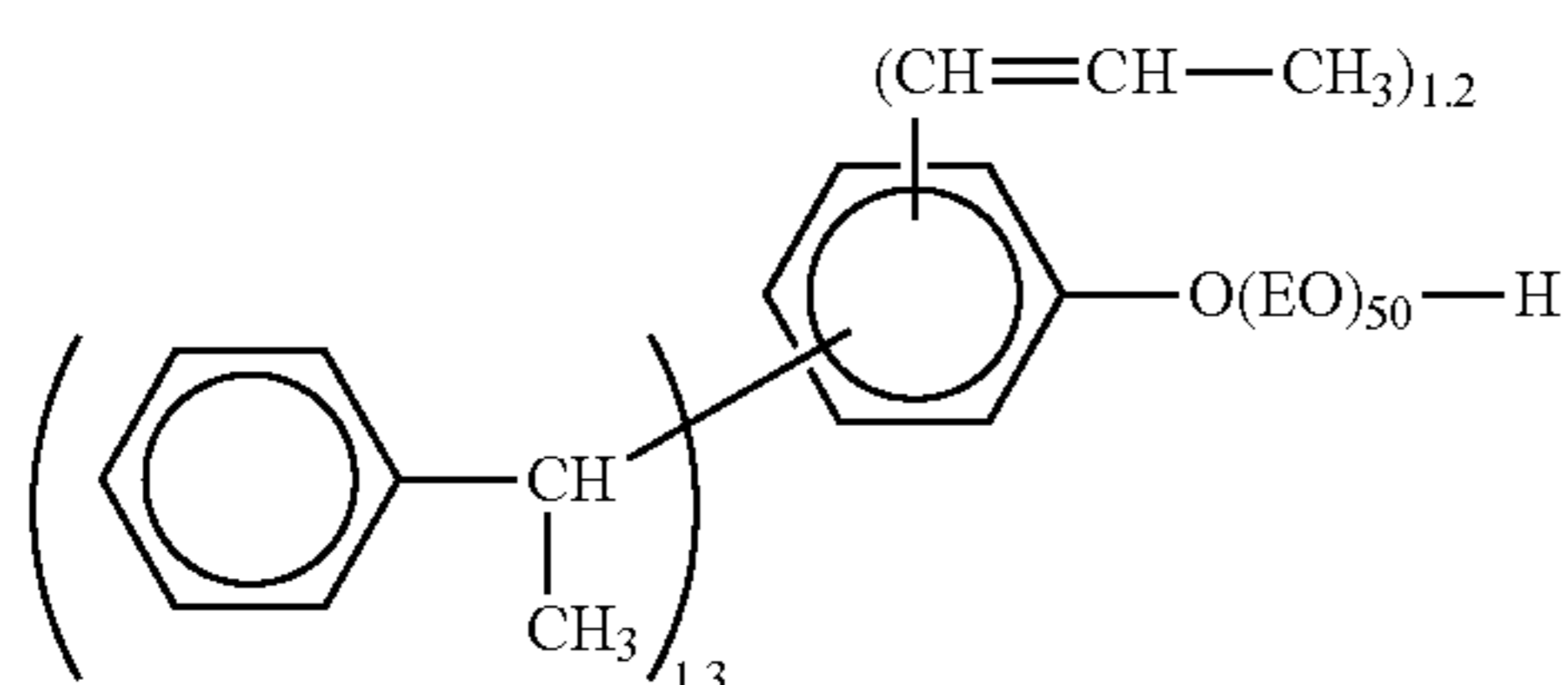
Synthesis Example 3
