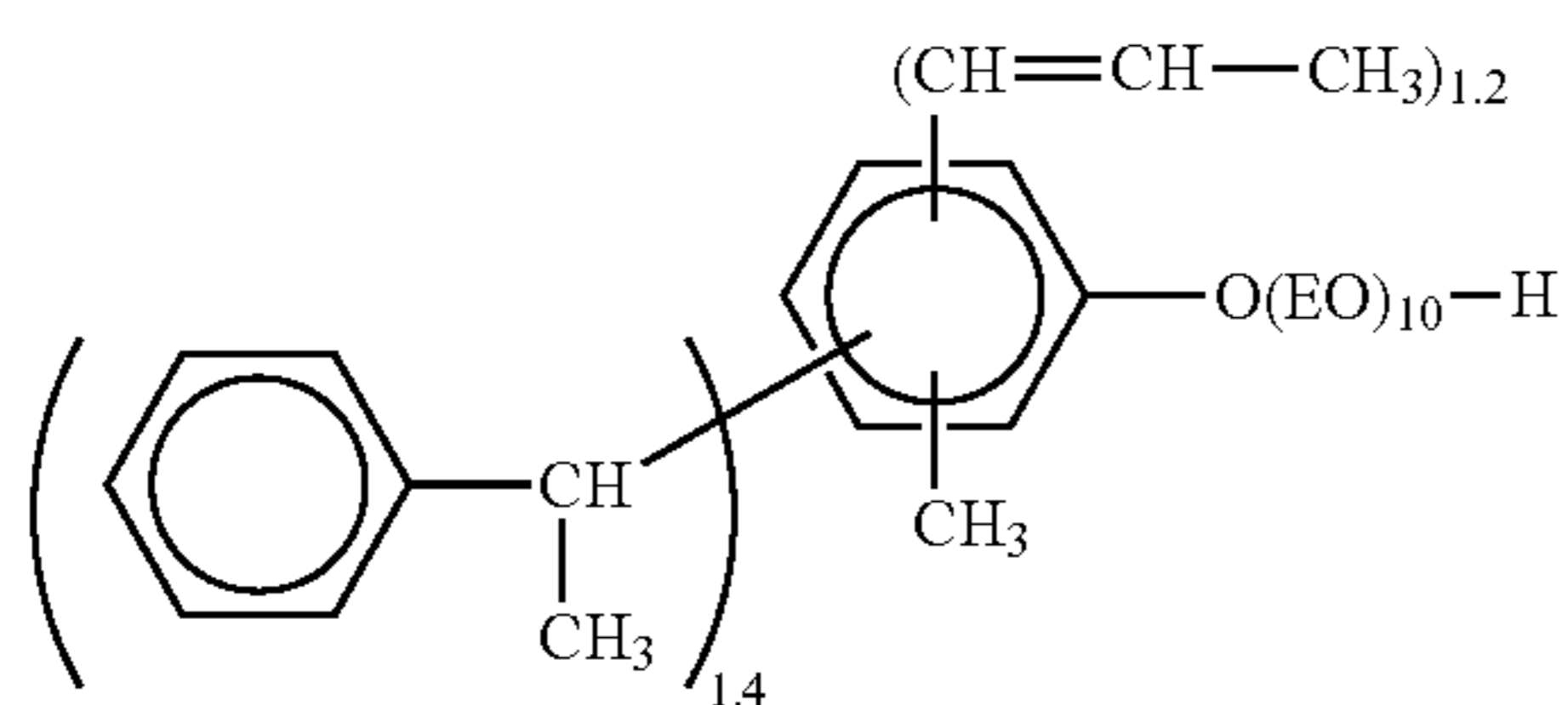
Synthesis Example 12
