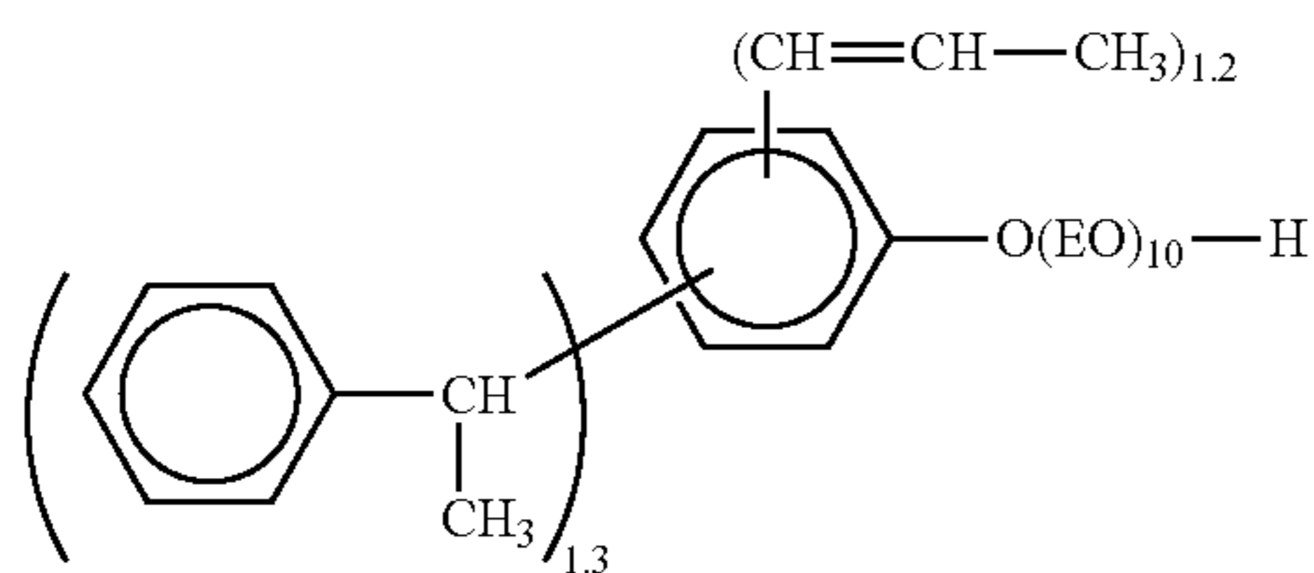
Synthesis Example 2
