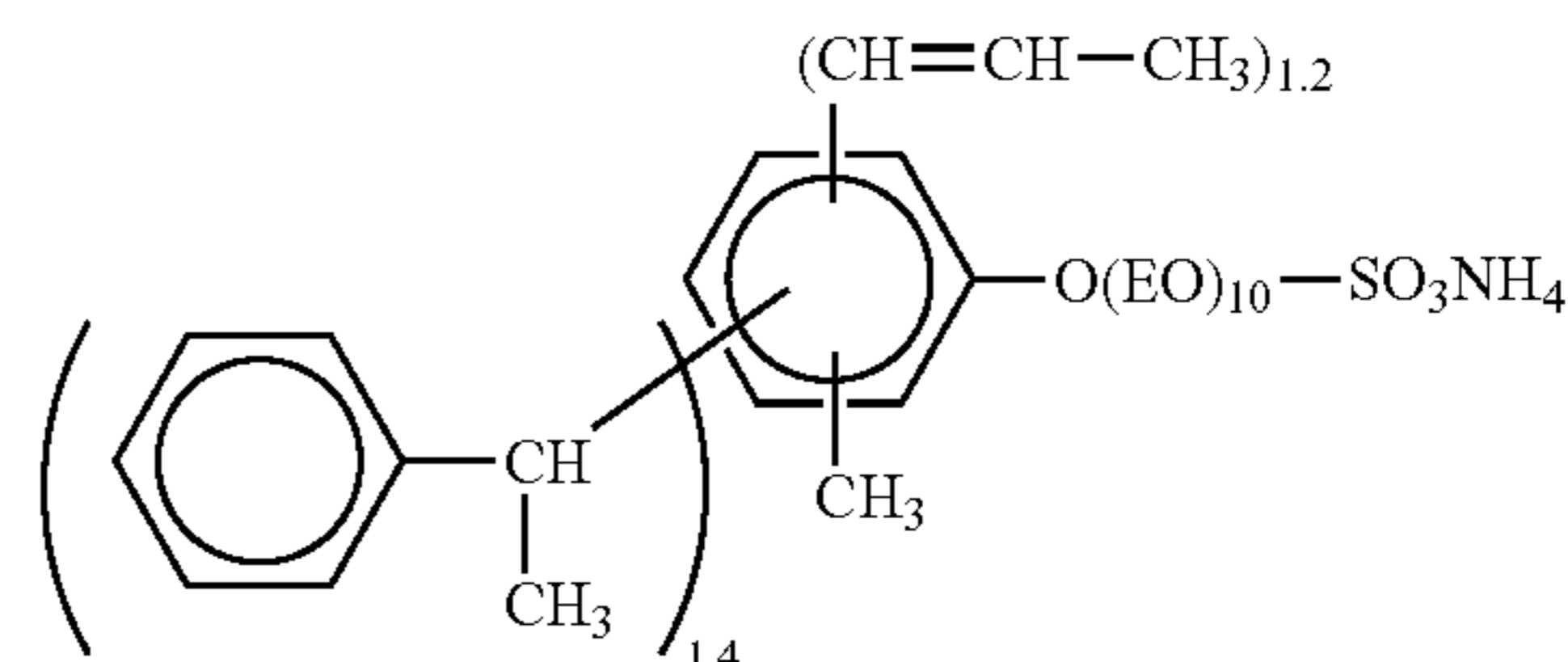
Synthesis Example 14
