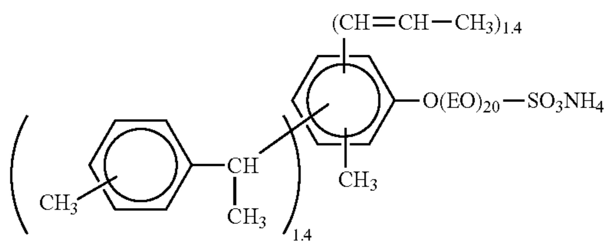
Synthesis Example 17
