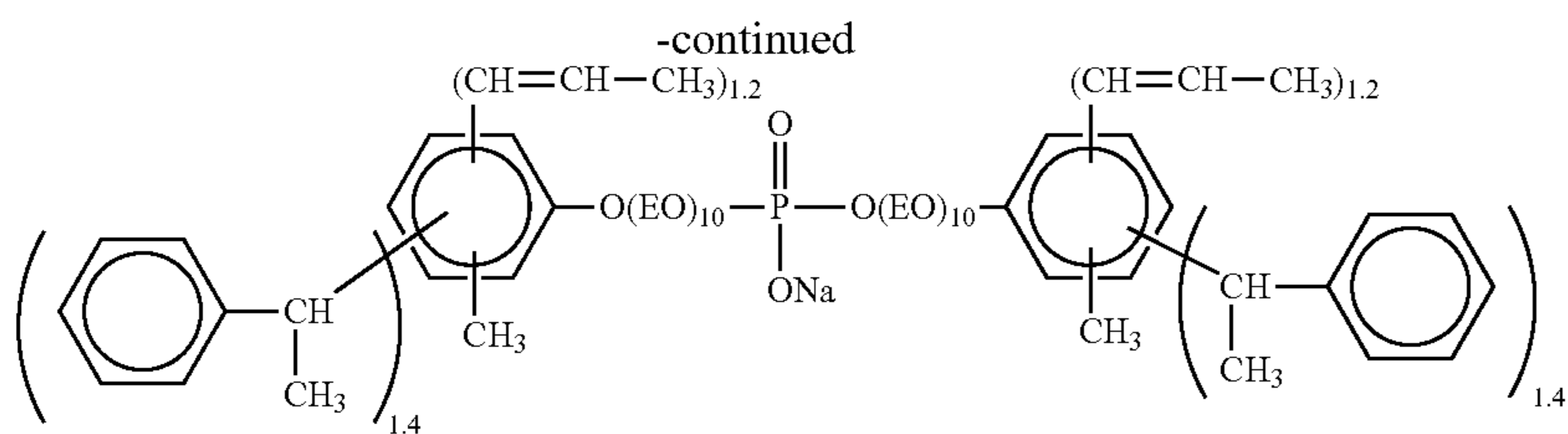
Synthesis Example 16
