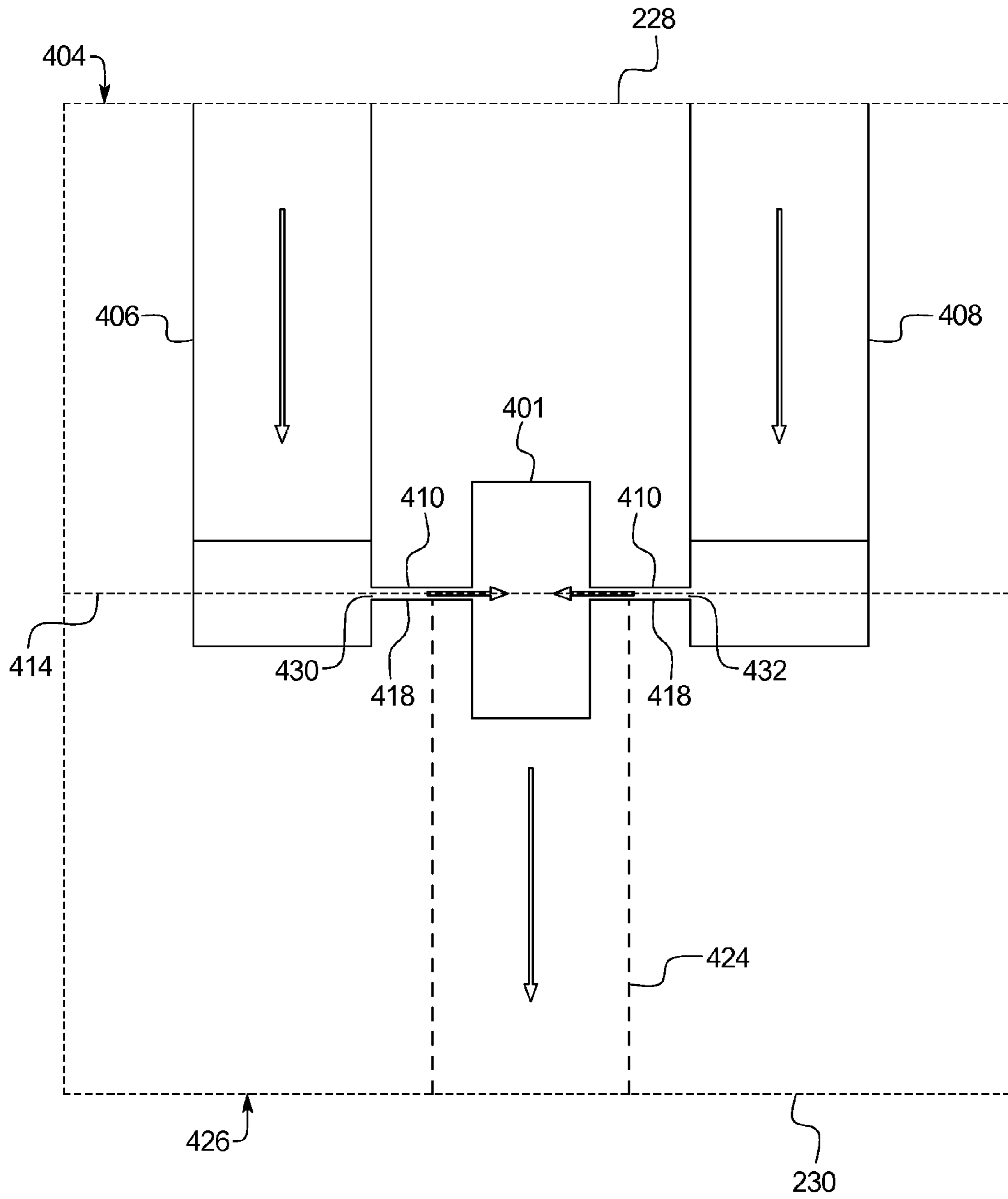
FIG. 9 (PRIOR ART)
